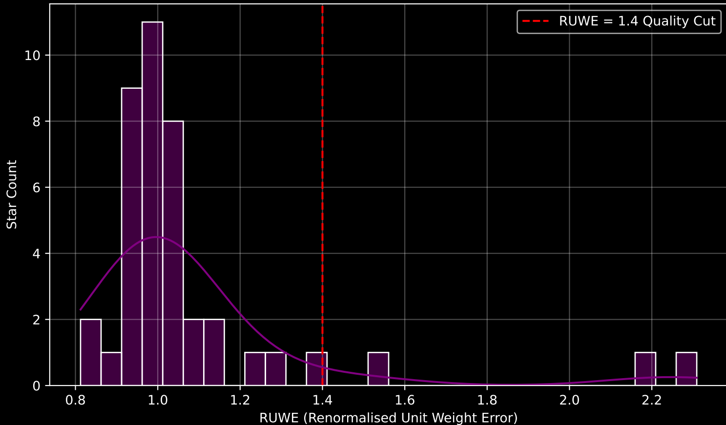
Gaia Cluster: [UPK_219] RUWE Distribution (n= 41)
