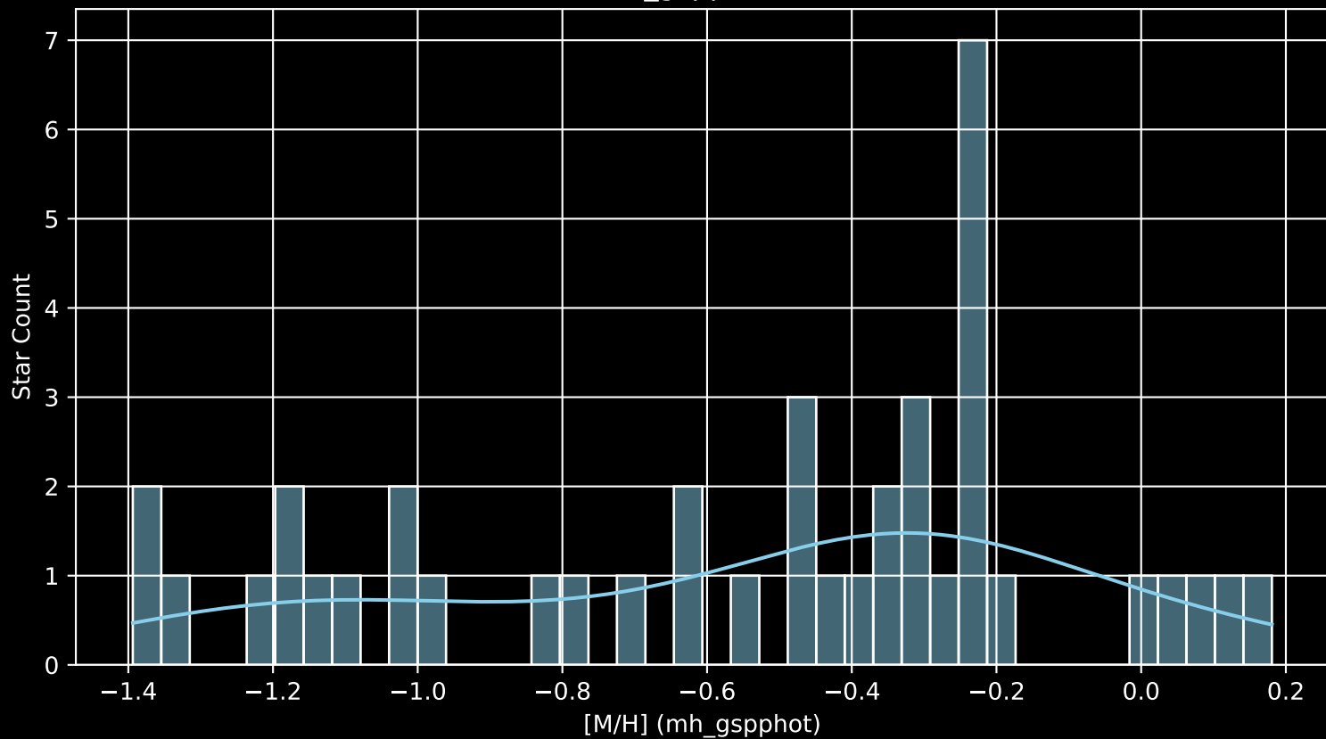
Gaia Cluster: [UPK_219 [M/H] (mh_gspphot) (n= 41)
