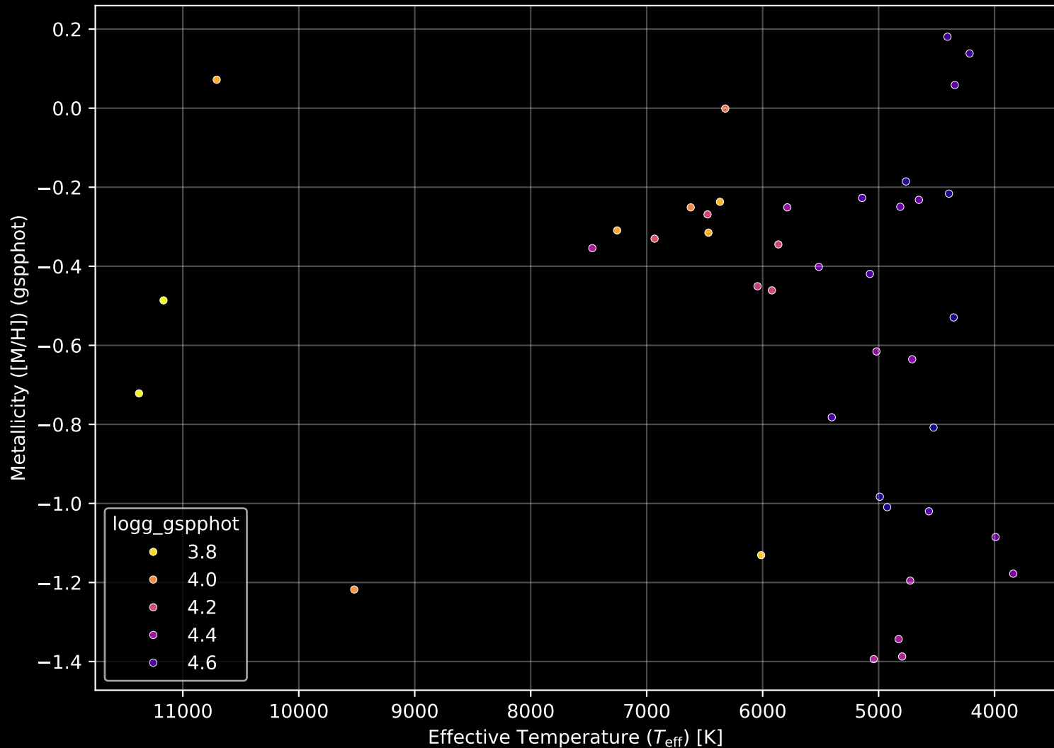
Gaia Cluster: [UPK_219] Stellar Population Parameters (n= 41)
