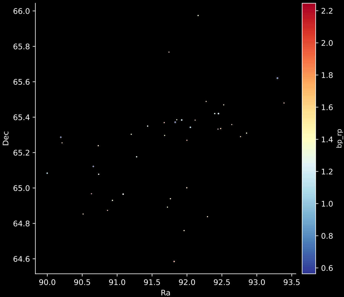
Gaia Cluster: [UPK_219] Stars: 41
