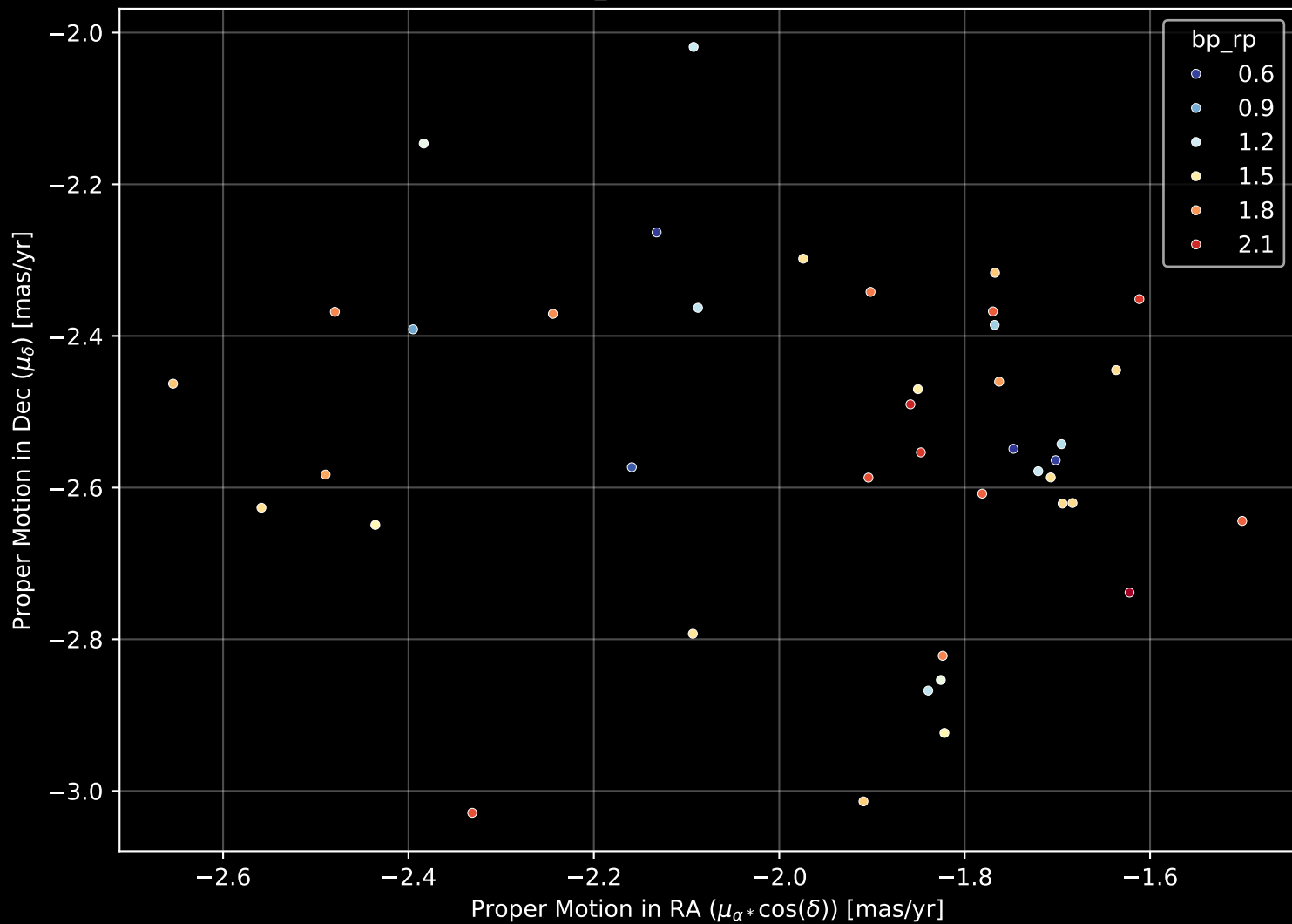
Gaia Cluster: [UPK_219] Proper Motion Diagram (n= 41)
