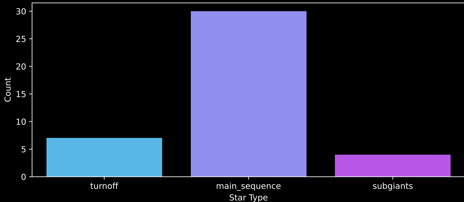
Gaia Cluster: [UPK_219] Count plot of Star Type
