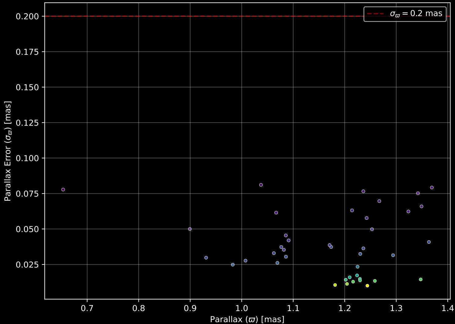
Gaia Cluster: [UPK 219] Parallax Quality (n= 41)
