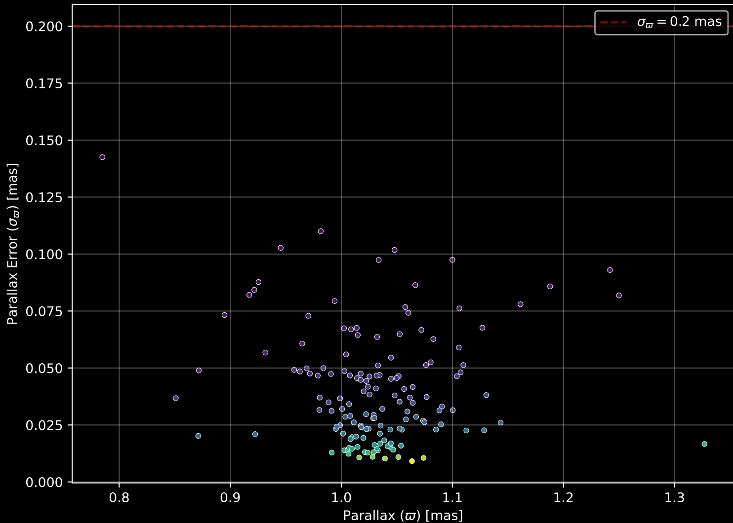
Gaia Cluster: [UPK_220] Parallax Quality (n= 148)
