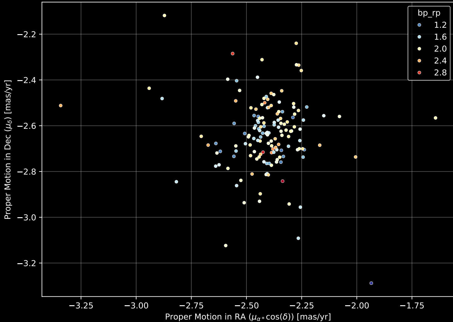
Gaia Cluster: [UPK_220] Proper Motion Diagram (n= 148)
