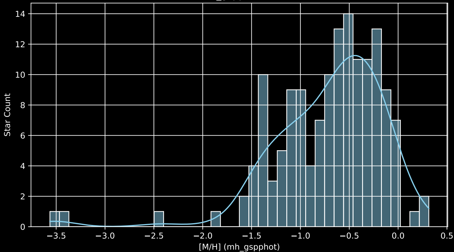
Gaia Cluster: [UPK_220 [M/H] (mh_gspphot) (n= 148)
