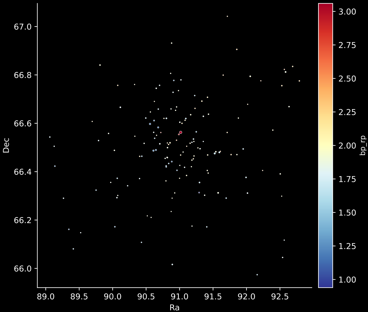
Gaia Cluster: [UPK_220] Stars: 148
