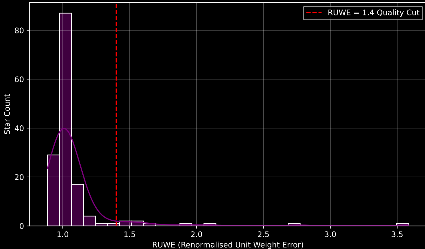
Gaia Cluster: [UPK_220] RUWE Distribution (n= 148)
