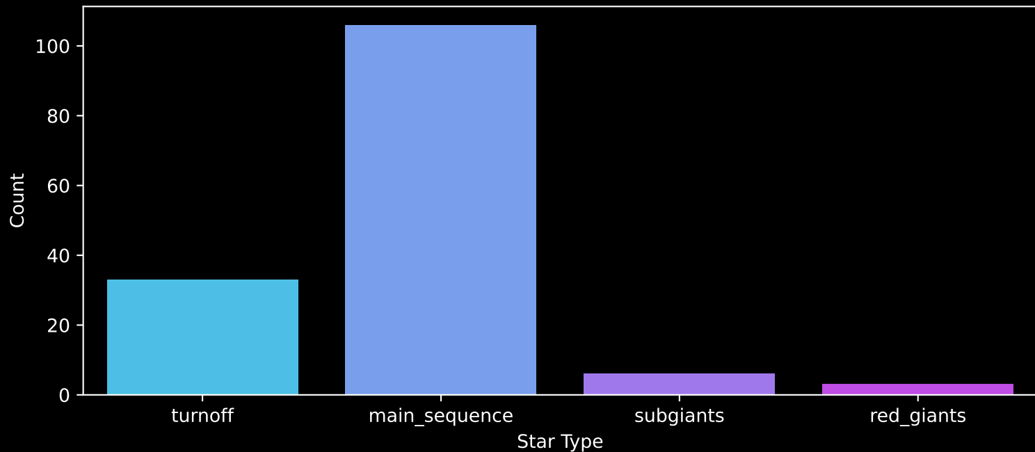
Gaia Cluster: [UPK_220] Count plot of Star Type
