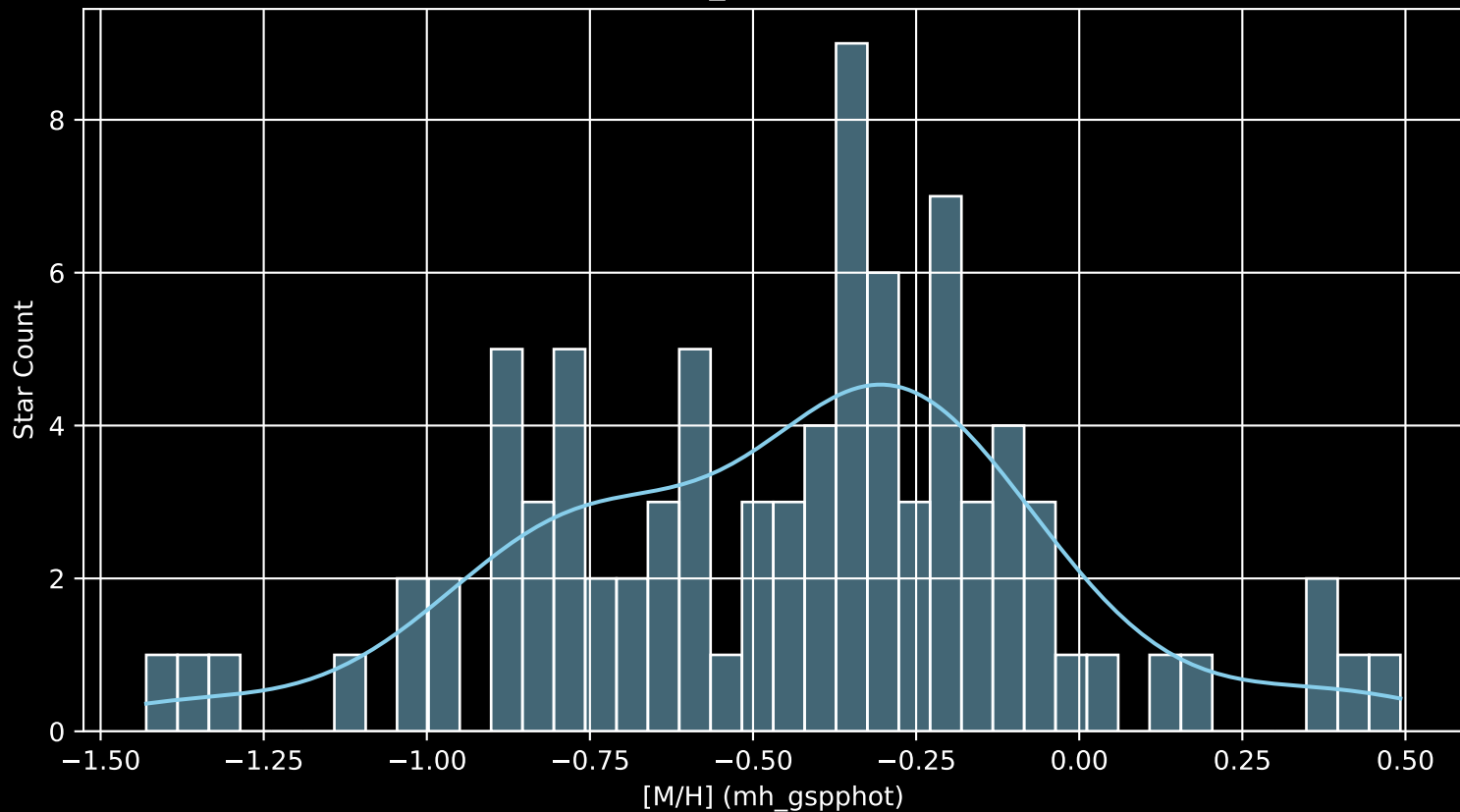
Gaia Cluster: [UPK_237 [M/H] (mh_gspphot) (n= 87)
