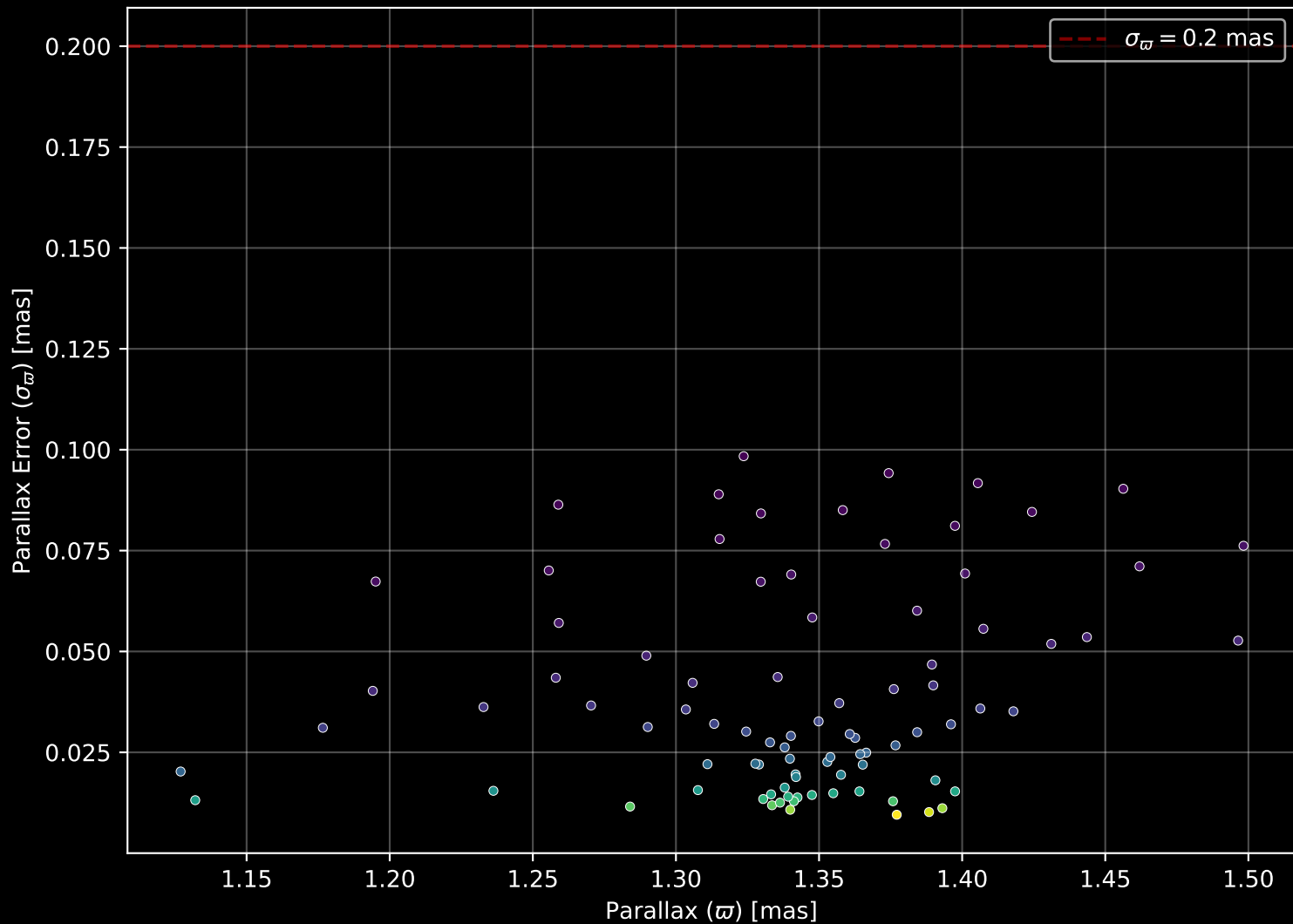
Gaia Cluster: [UPK_237] Parallax Quality (n= 88)
