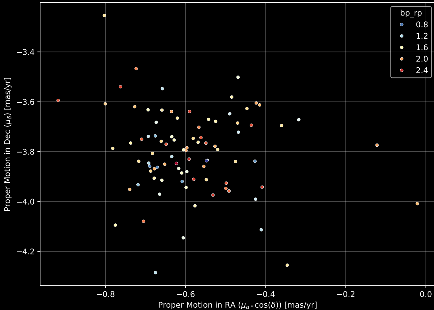
Gaia Cluster: [UPK_237] Proper Motion Diagram (n= 88)
