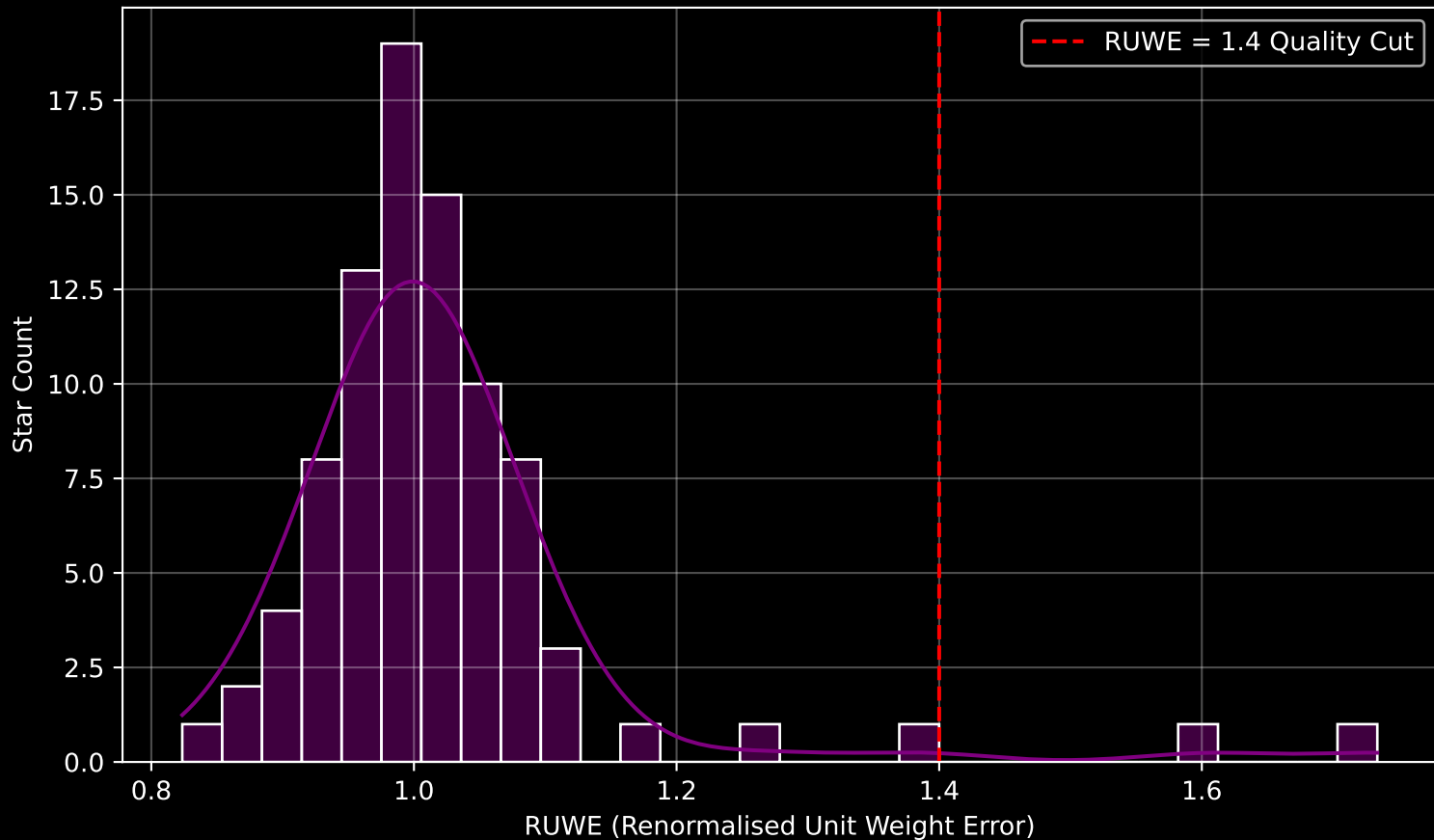
Gaia Cluster: [UPK_237] RUWE Distribution (n= 88)
