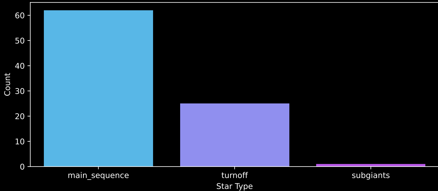
Gaia Cluster: [UPK_237] Count plot of Star Type
