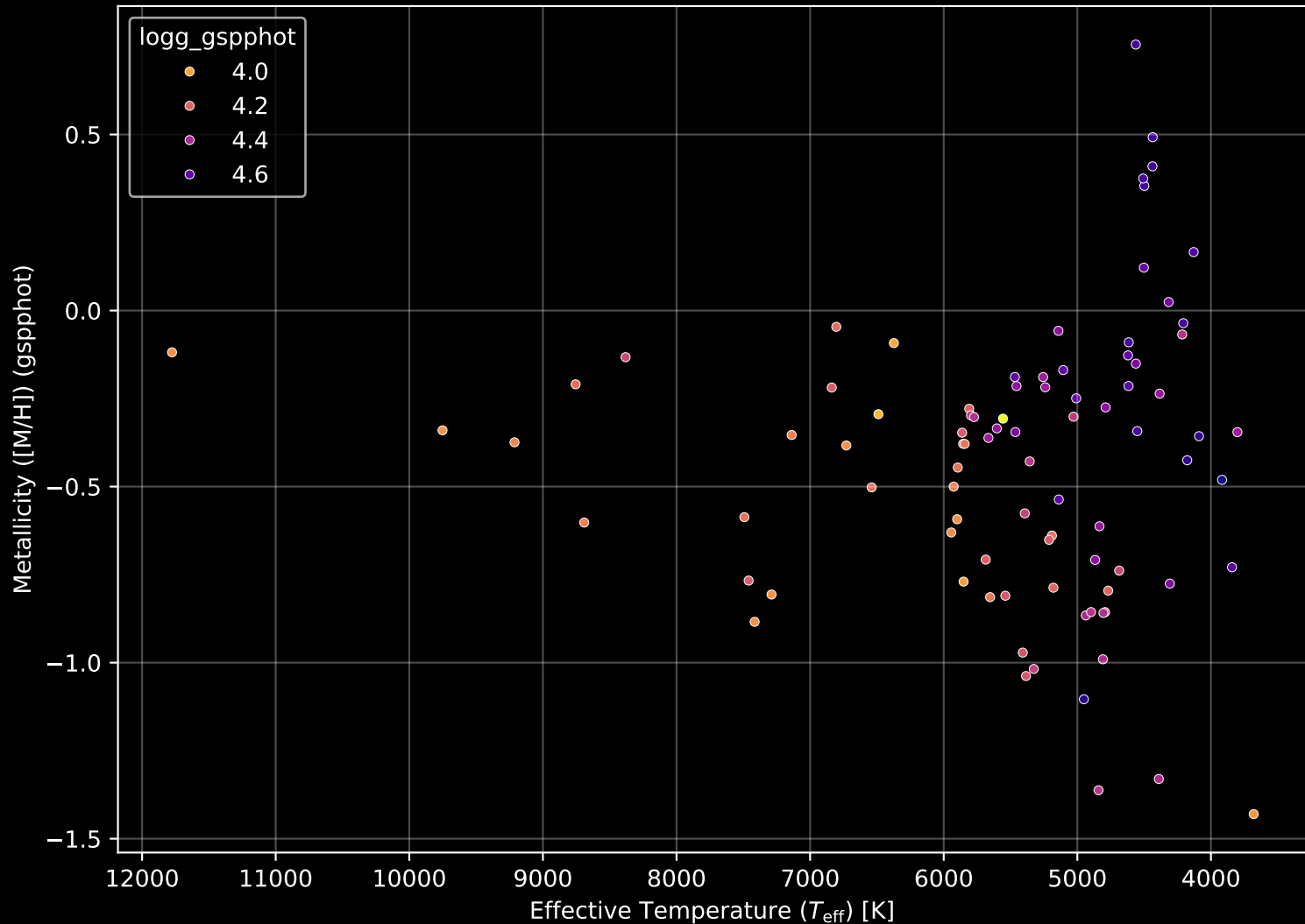
Gaia Cluster: [UPK_237] Stellar Population Parameters (n= 88)
