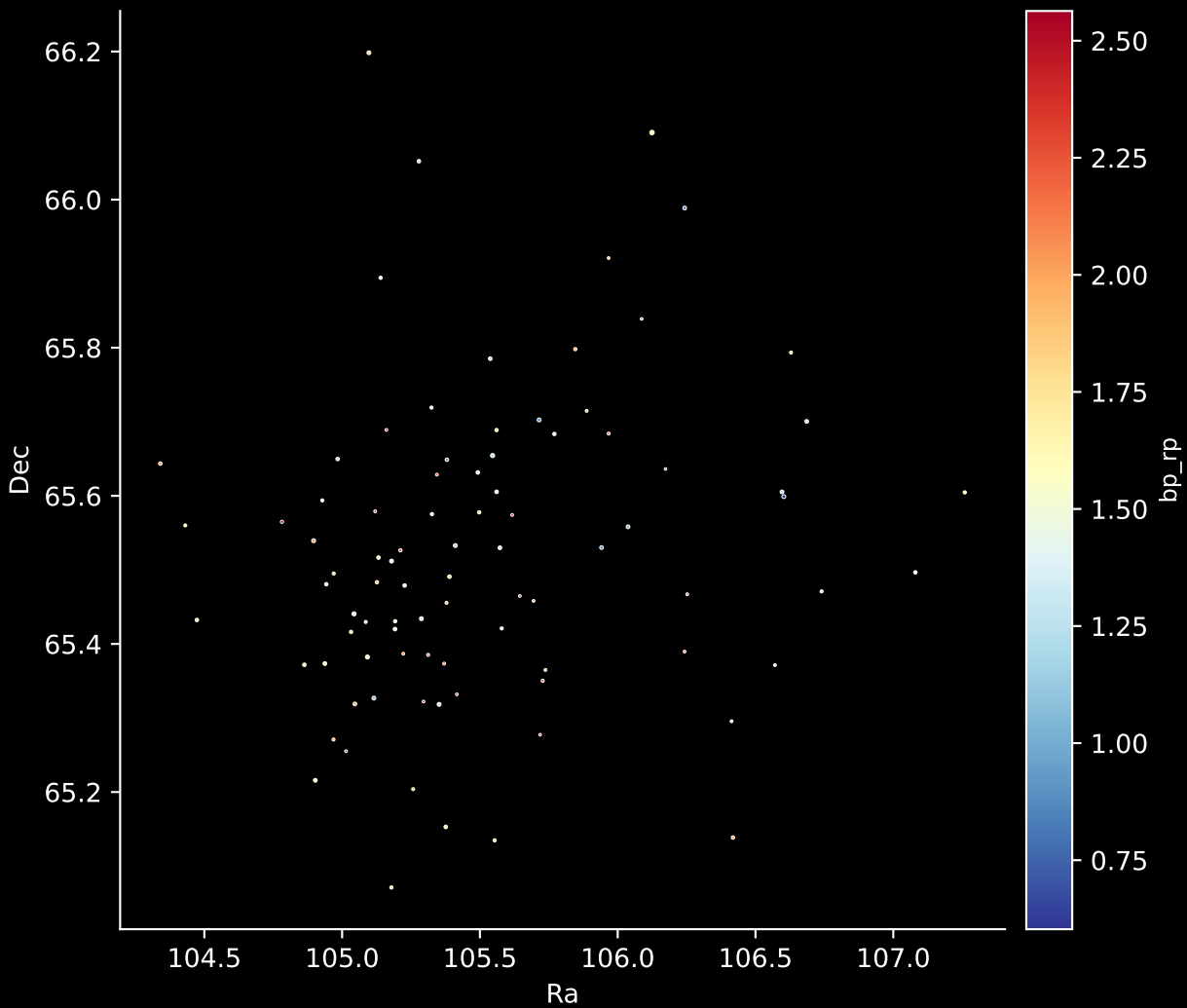
Gaia Cluster: [UPK_237] Stars: 88
