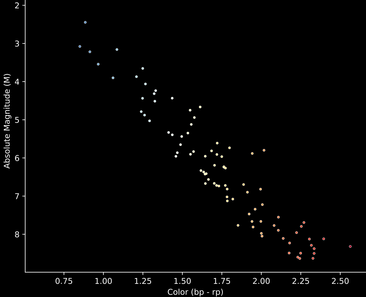
Gaia Cluster: [UPK_237] Stars (n= 88) Hertzsprung-Russel Diagram
