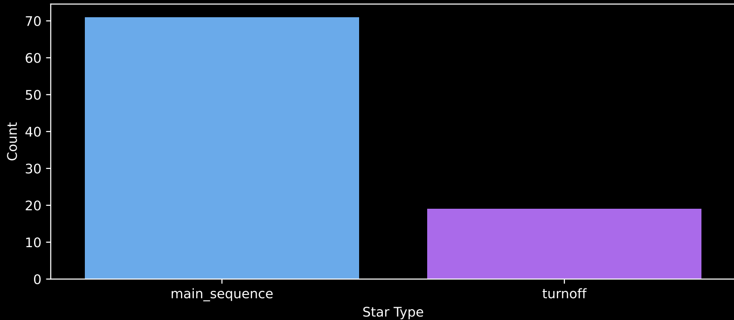
Gaia Cluster: [UPK_24] Count plot of Star Type
