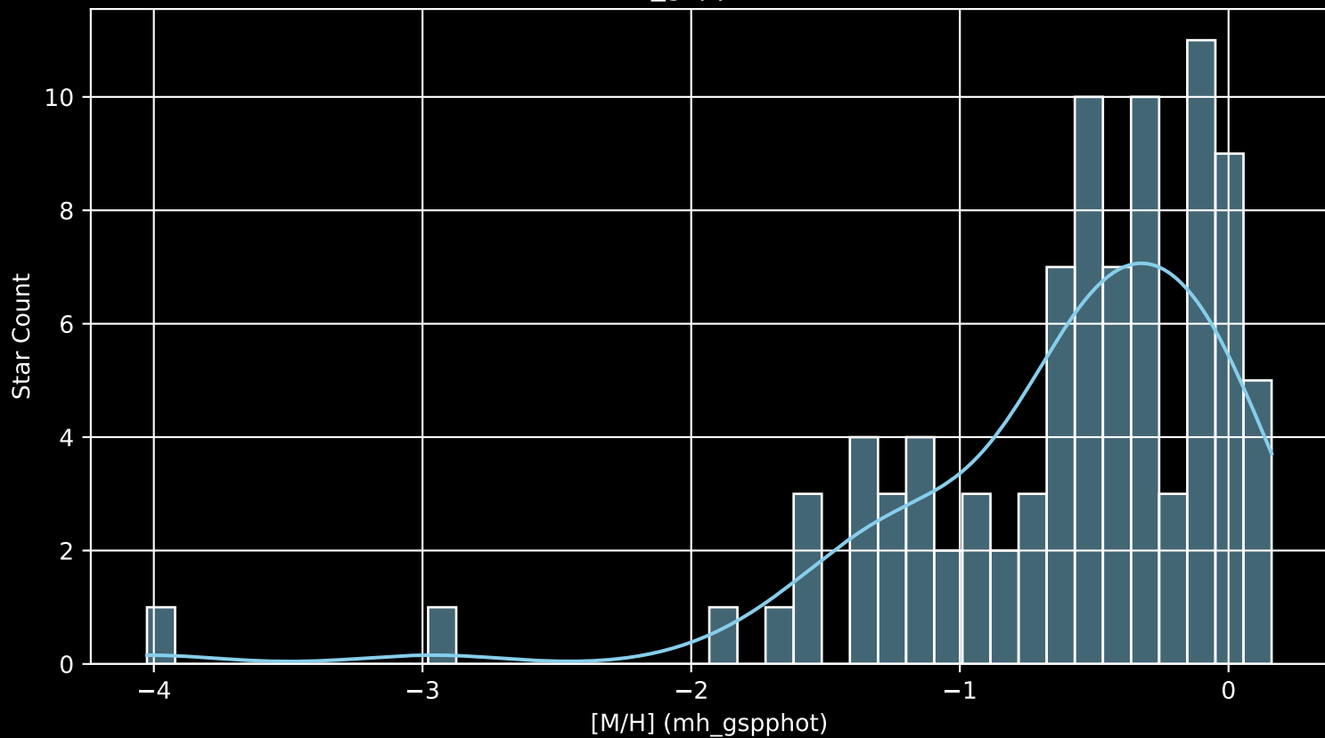
Gaia Cluster: [UPK_24 [M/H] (mh_gspphot) (n= 90)
