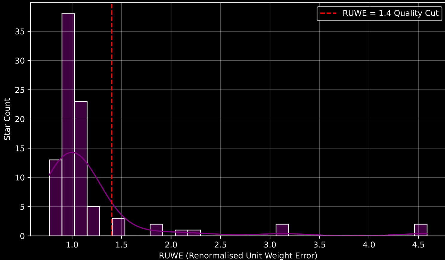
Gaia Cluster: [UPK_24] RUWE Distribution (n= 90)
