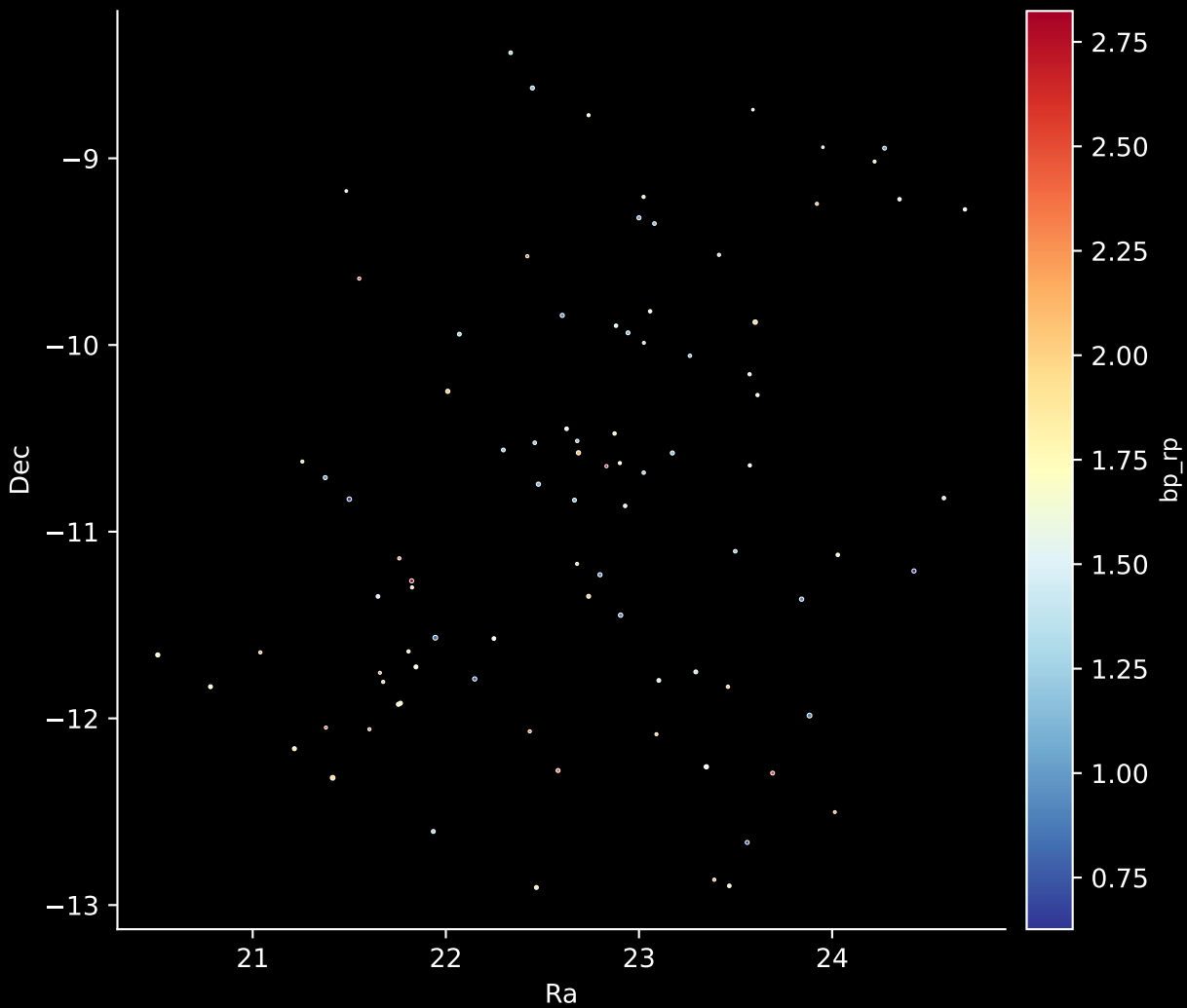
Gaia Cluster: [UPK_24] Stars: 90
