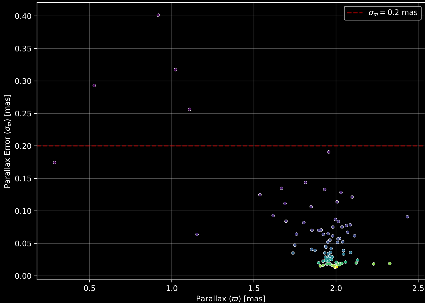
Gaia Cluster: [UPK_24] Parallax Quality (n= 90)
