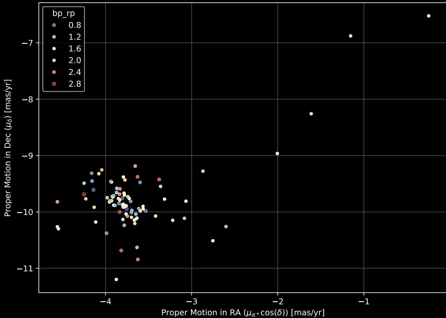
Gaia Cluster: [UPK_24] Proper Motion Diagram (n= 90)
