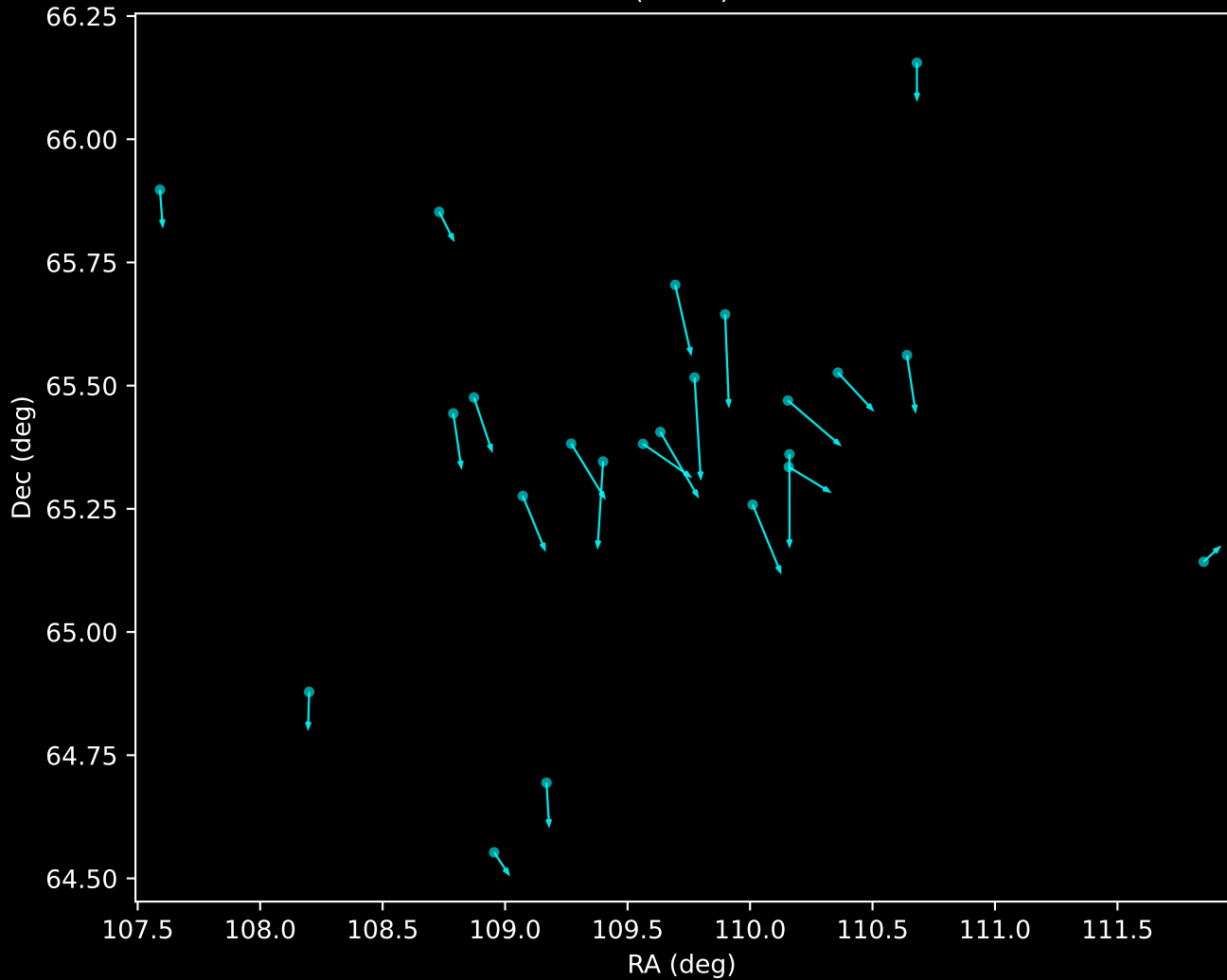
Gaia DR3 Noise Stream Proper Motion Vectors (n=23)
