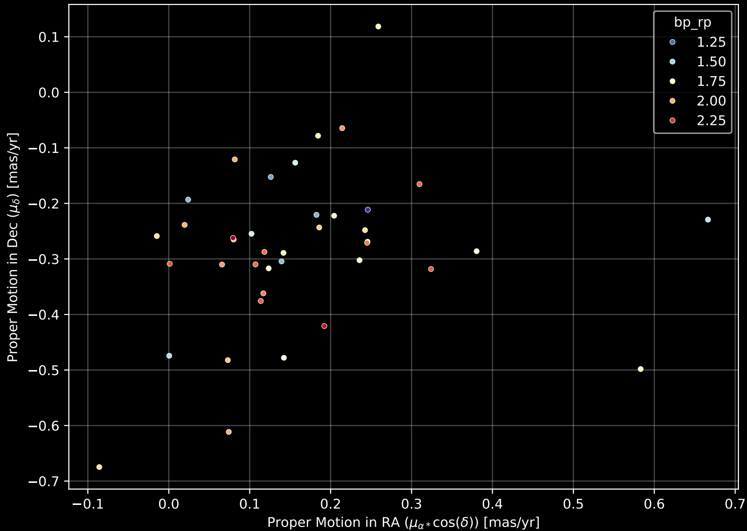
Gaia Cluster: [UPK_241] Proper Motion Diagram (n= 40)
