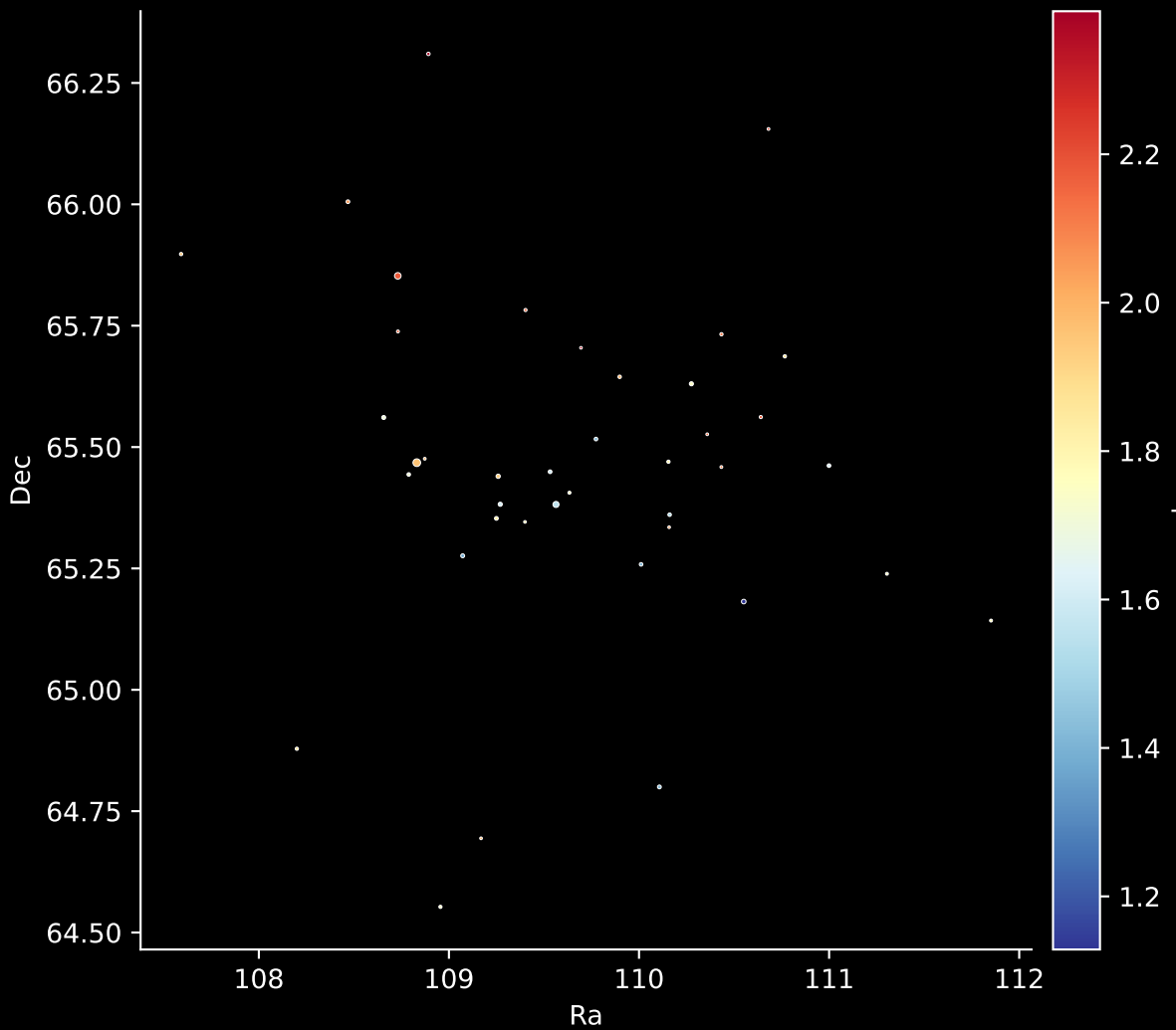
Gaia Cluster: [UPK_241] Stars: 40
