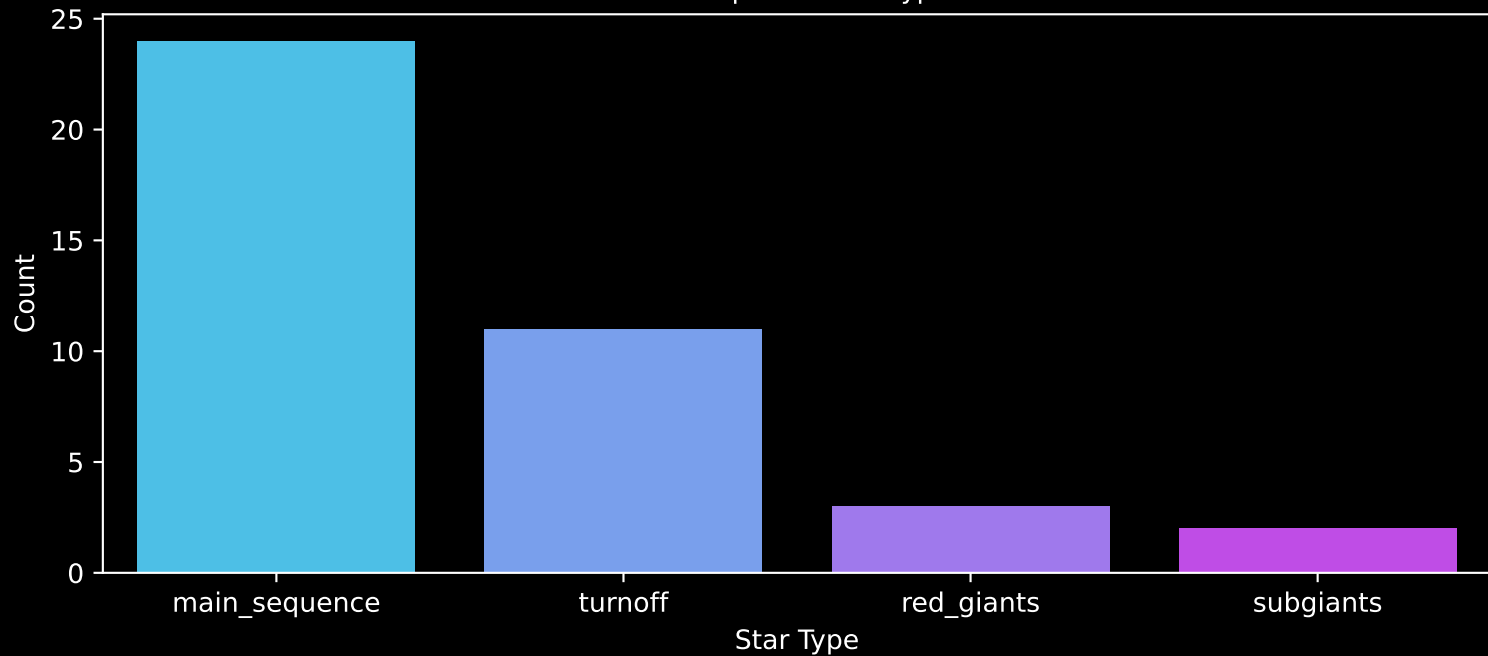
Gaia Cluster: [UPK_241] Count plot of Star Type
