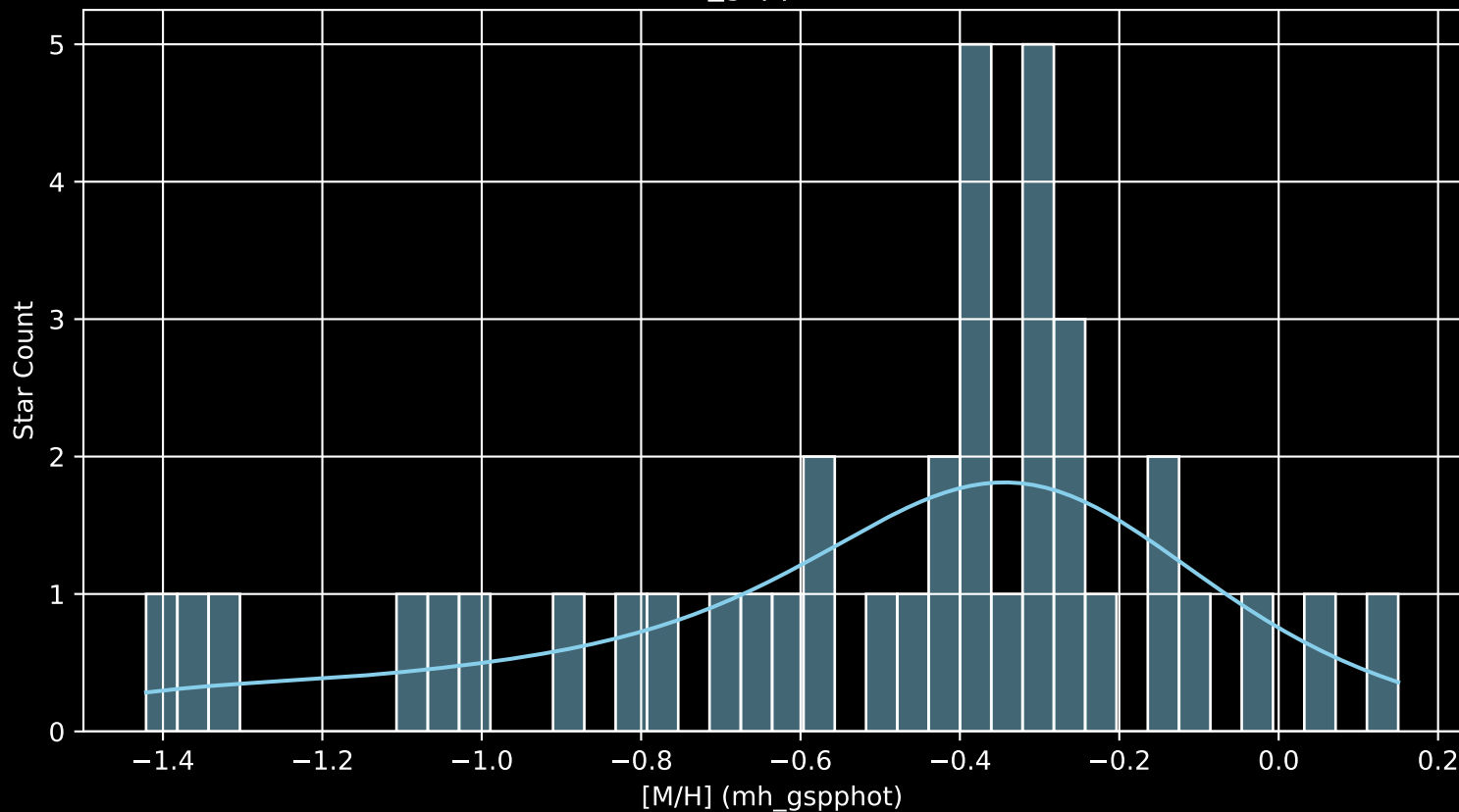
Gaia Cluster: [UPK_241 [M/H] (mh_gspphot) (n= 39)
