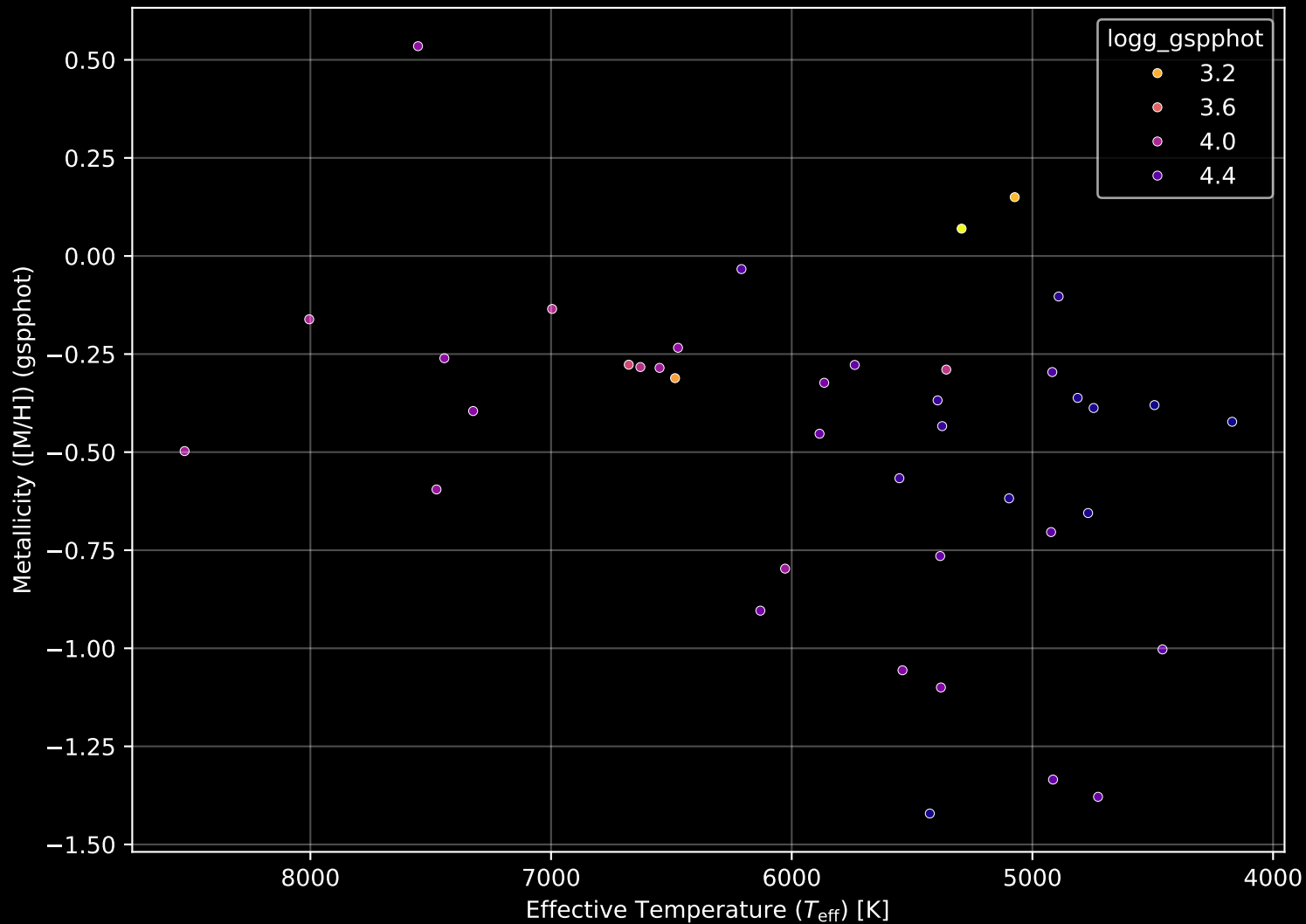
Gaia Cluster: [UPK_241] Stellar Population Parameters (n= 40)
