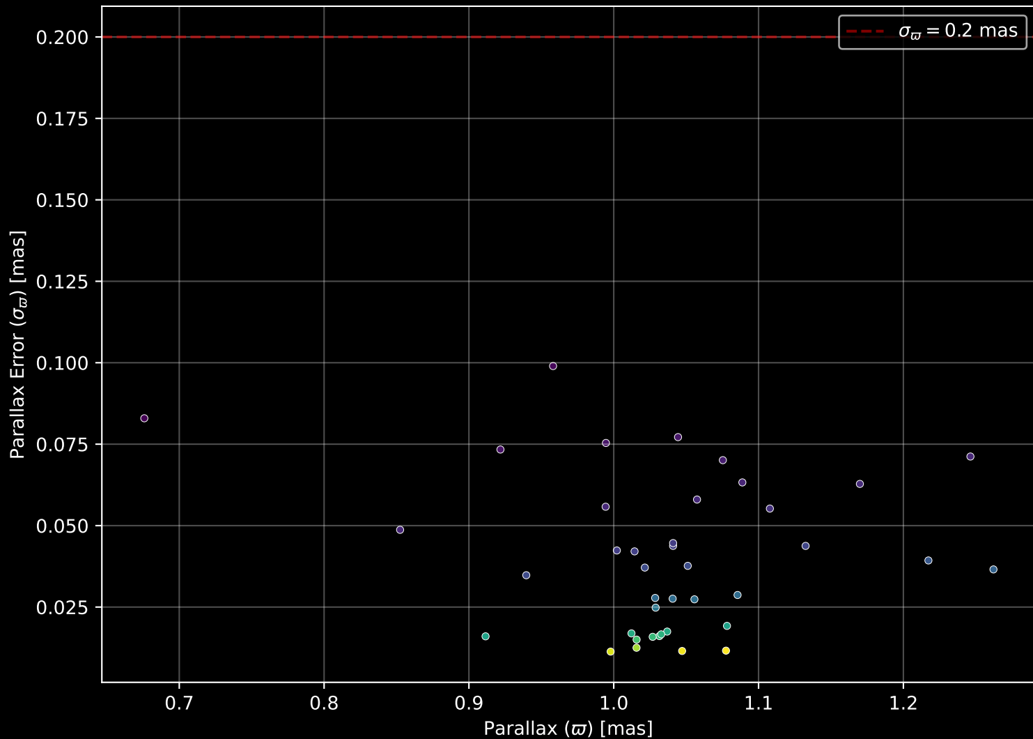
Gaia Cluster: [UPK_241] Parallax Quality (n= 40)
