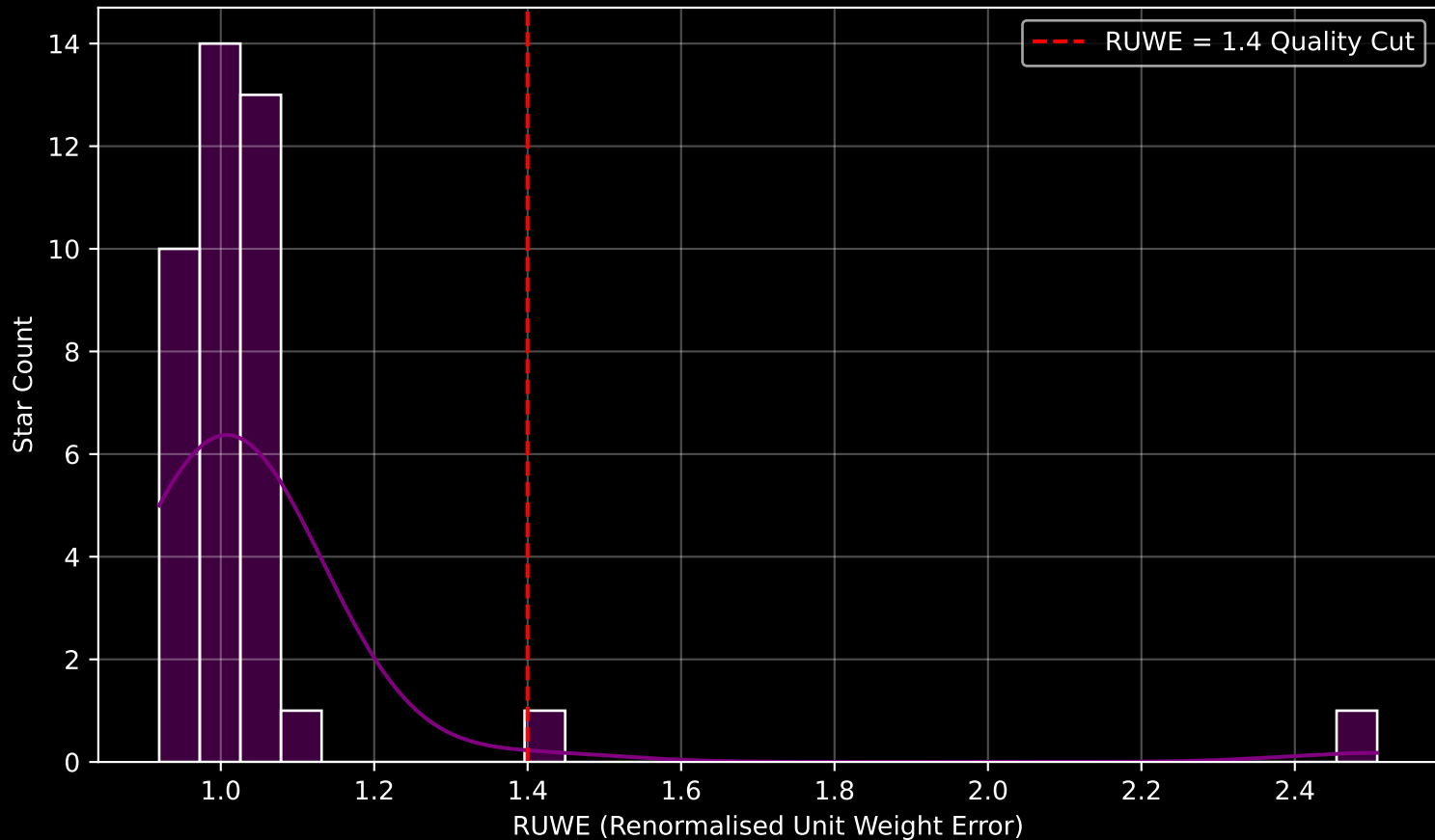
Gaia Cluster: [UPK_241] RUWE Distribution (n= 40)
