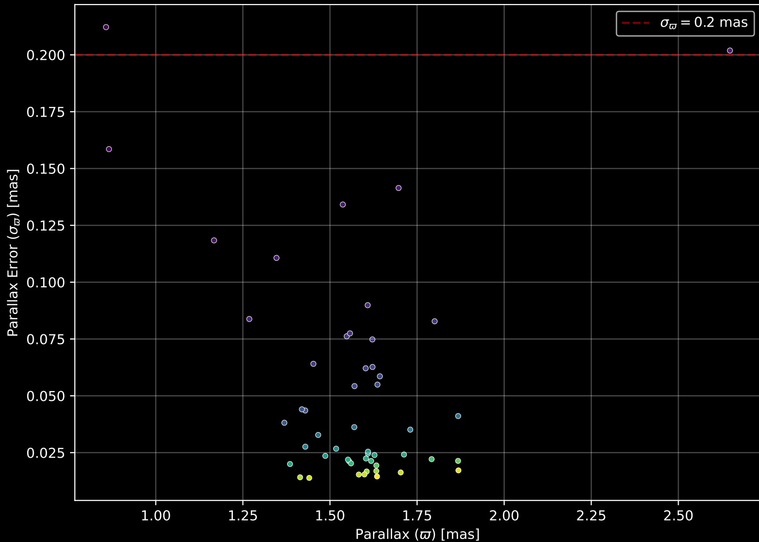
Gaia Cluster: [UPK_25] Parallax Quality (n= 51)
