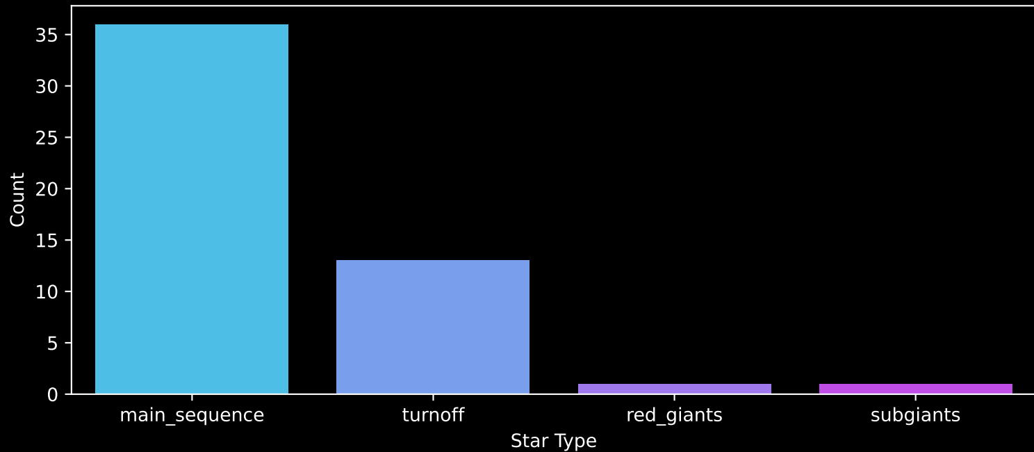
Gaia Cluster: [UPK_25] Count plot of Star Type
