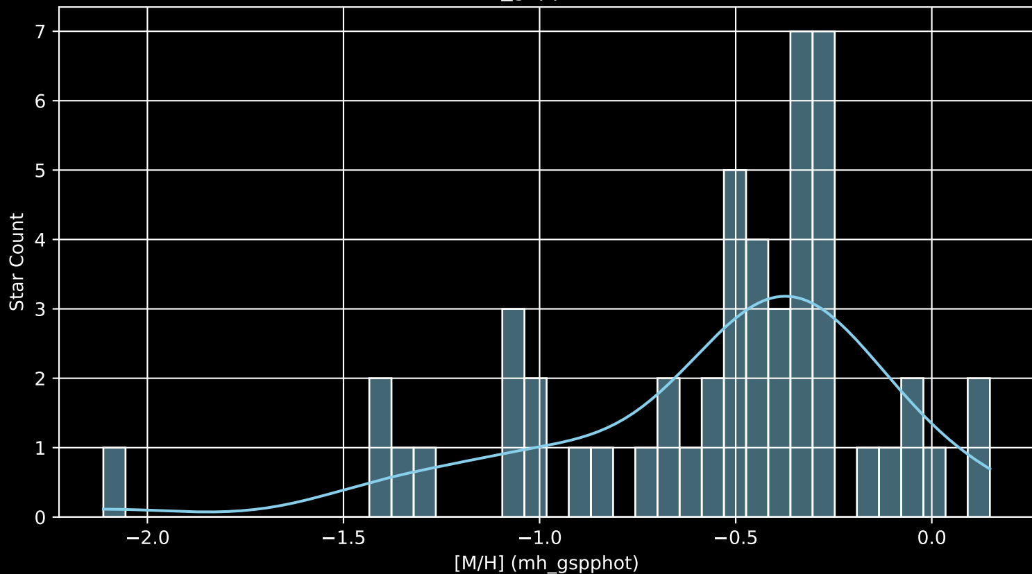
Gaia Cluster: [UPK_25 [M/H] (mh_gspphot) ( \bar{n}= 51 )
