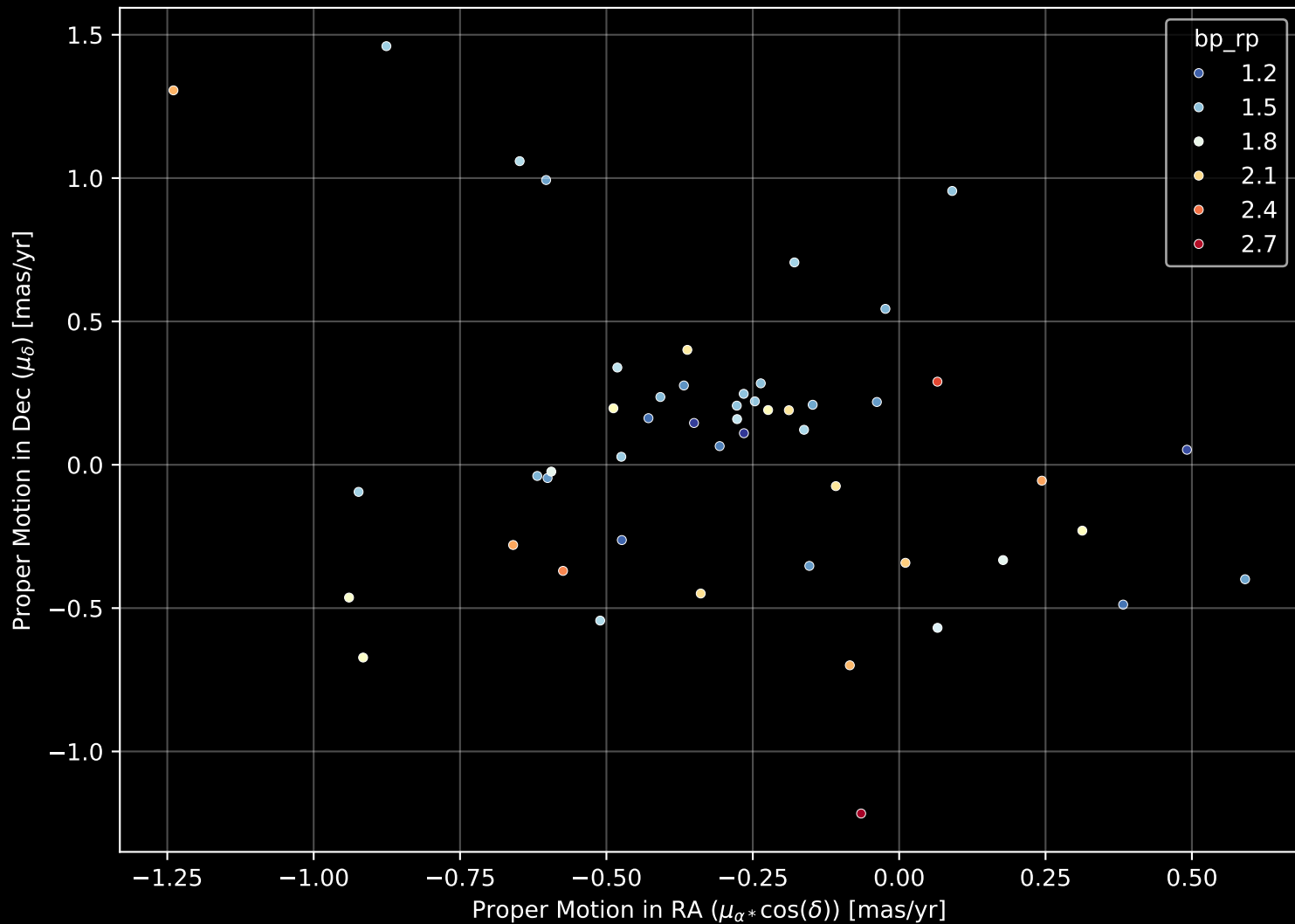
Gaia Cluster: [UPK_25] Proper Motion Diagram (n= 51)
