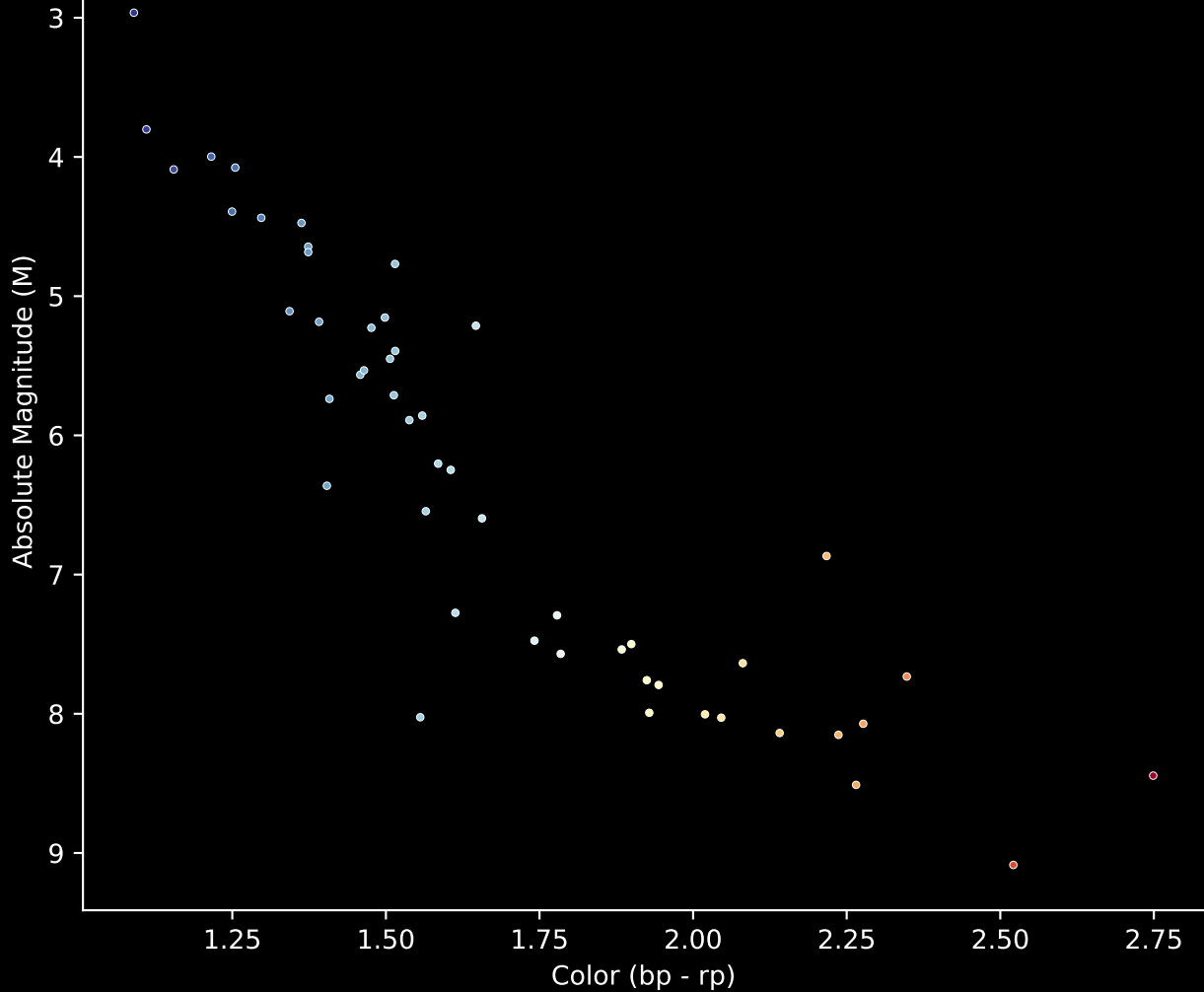
Gaia Cluster: [UPK_25] Stars (n= 51) Hertzsprung-Russel Diagram
