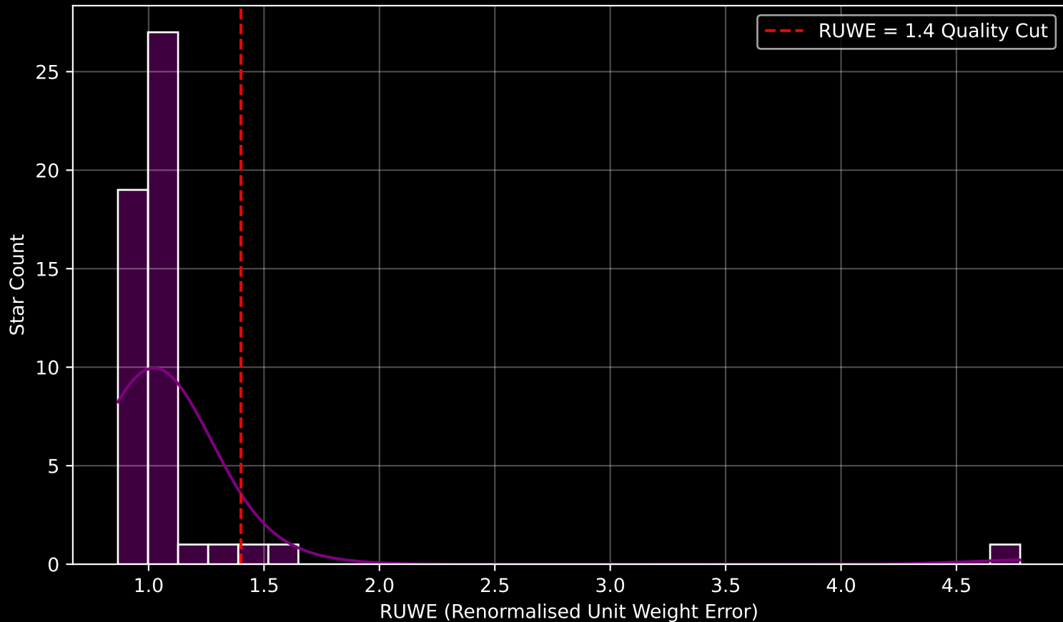
Gaia Cluster: [UPK_25] RUWE Distribution (n= 51)
