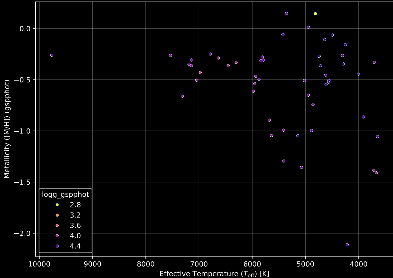
Gaia Cluster: [UPK_25] Stellar Population Parameters (n= 51)
