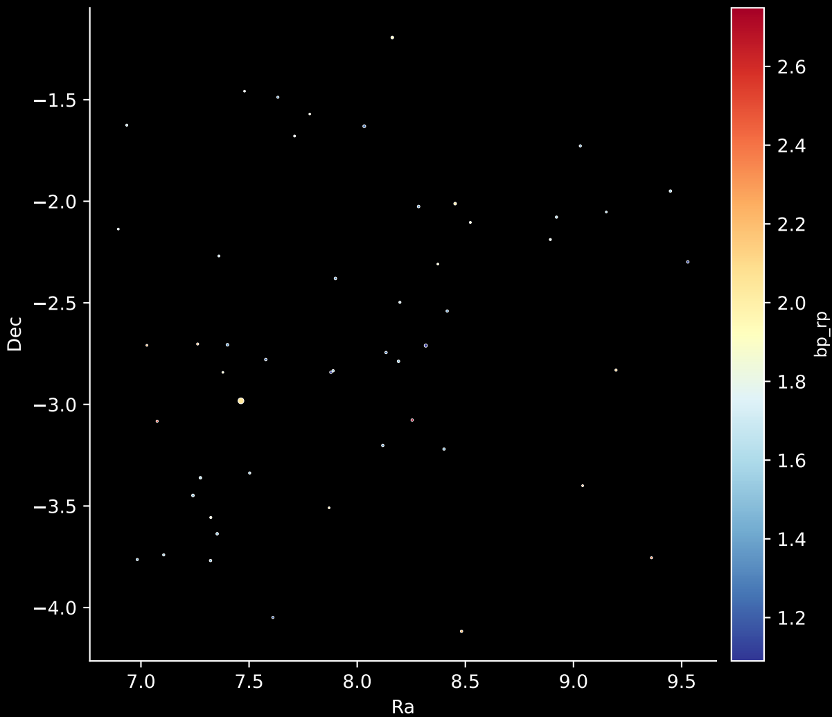
Gaia Cluster: [UPK_25] Stars: 51
