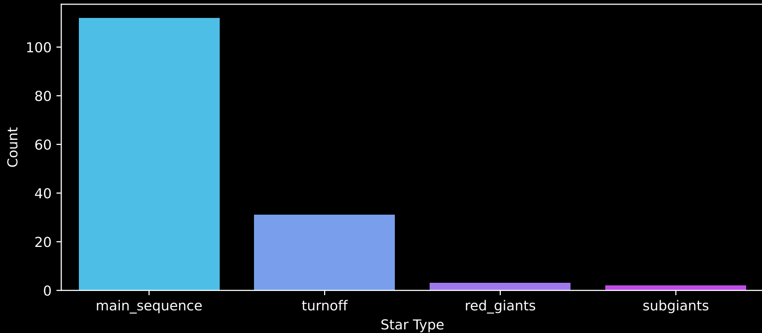
Gaia Cluster: [UPK_26] Count plot of Star Type
