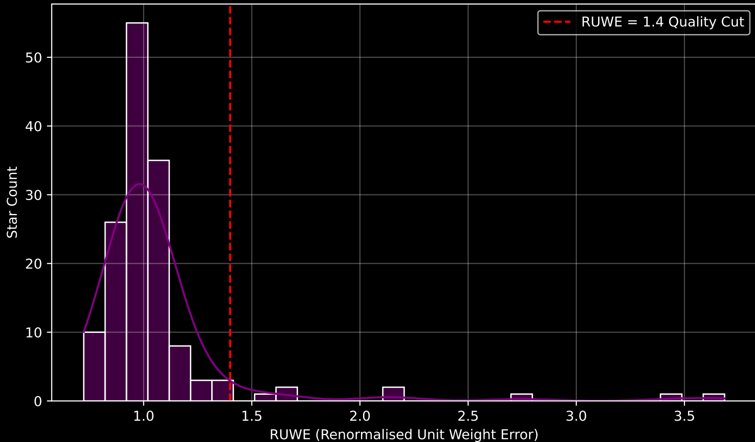
Gaia Cluster: [UPK_26] RUWE Distribution (n= 148)
