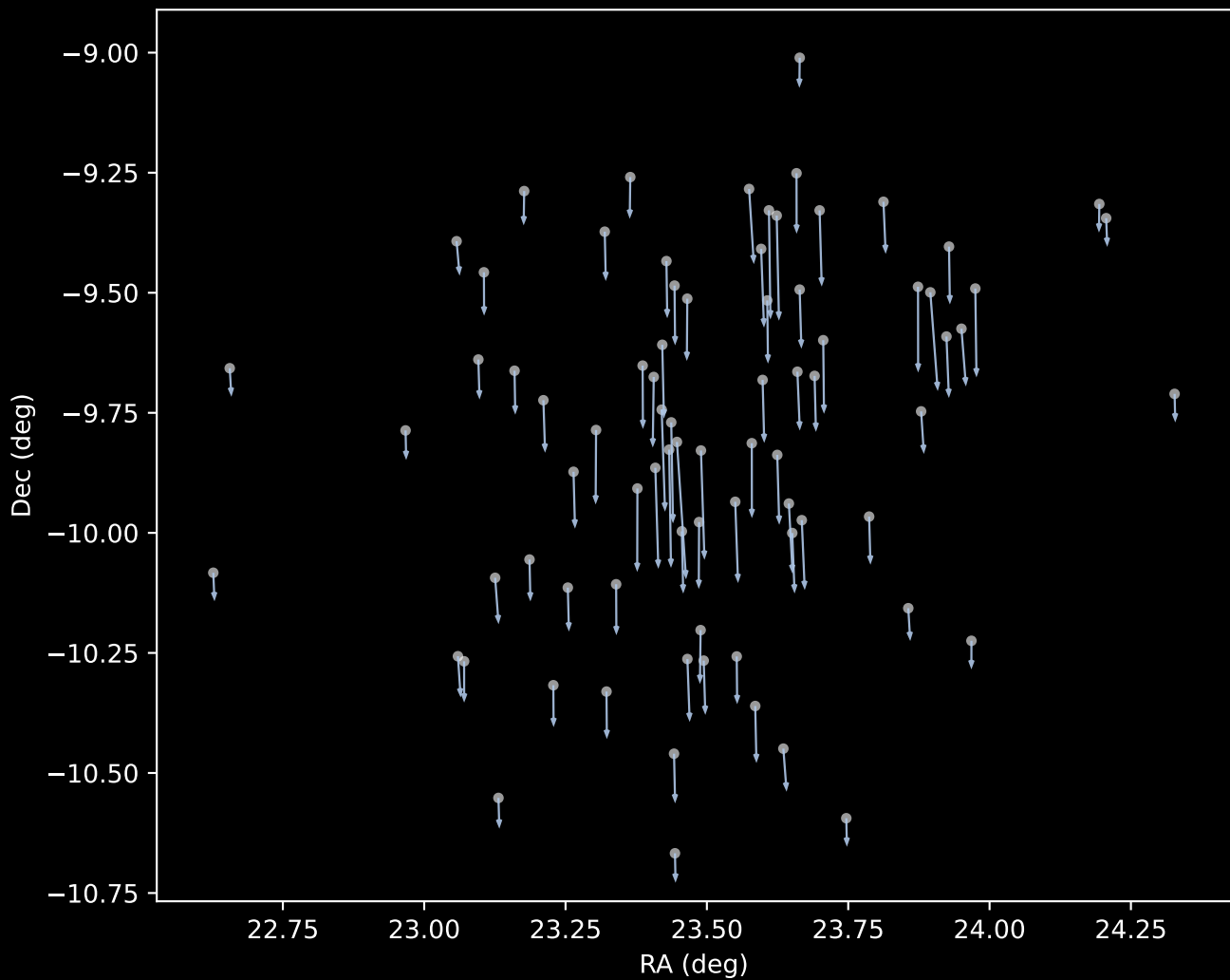
Gaia DR3 Cluster 1 Proper Motion Vectors (n=79)
