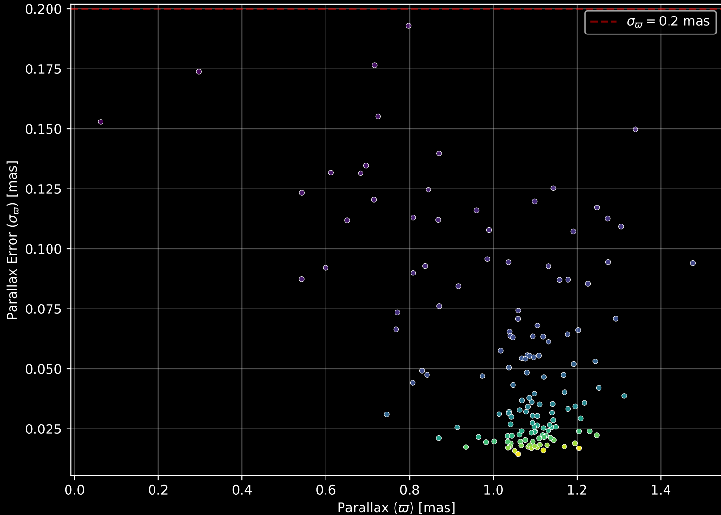
Gaia Cluster: [UPK_26] Parallax Quality (n= 148)
