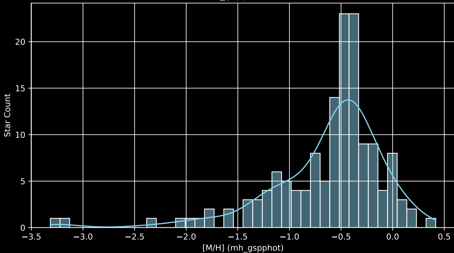
Gaia Cluster: [UPK_26 [M/H] (mh_gspphot) (n= 148)
