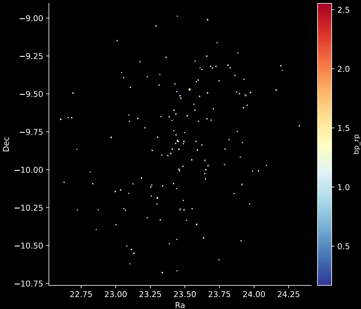
Gaia Cluster: [UPK_26] Stars: 148
