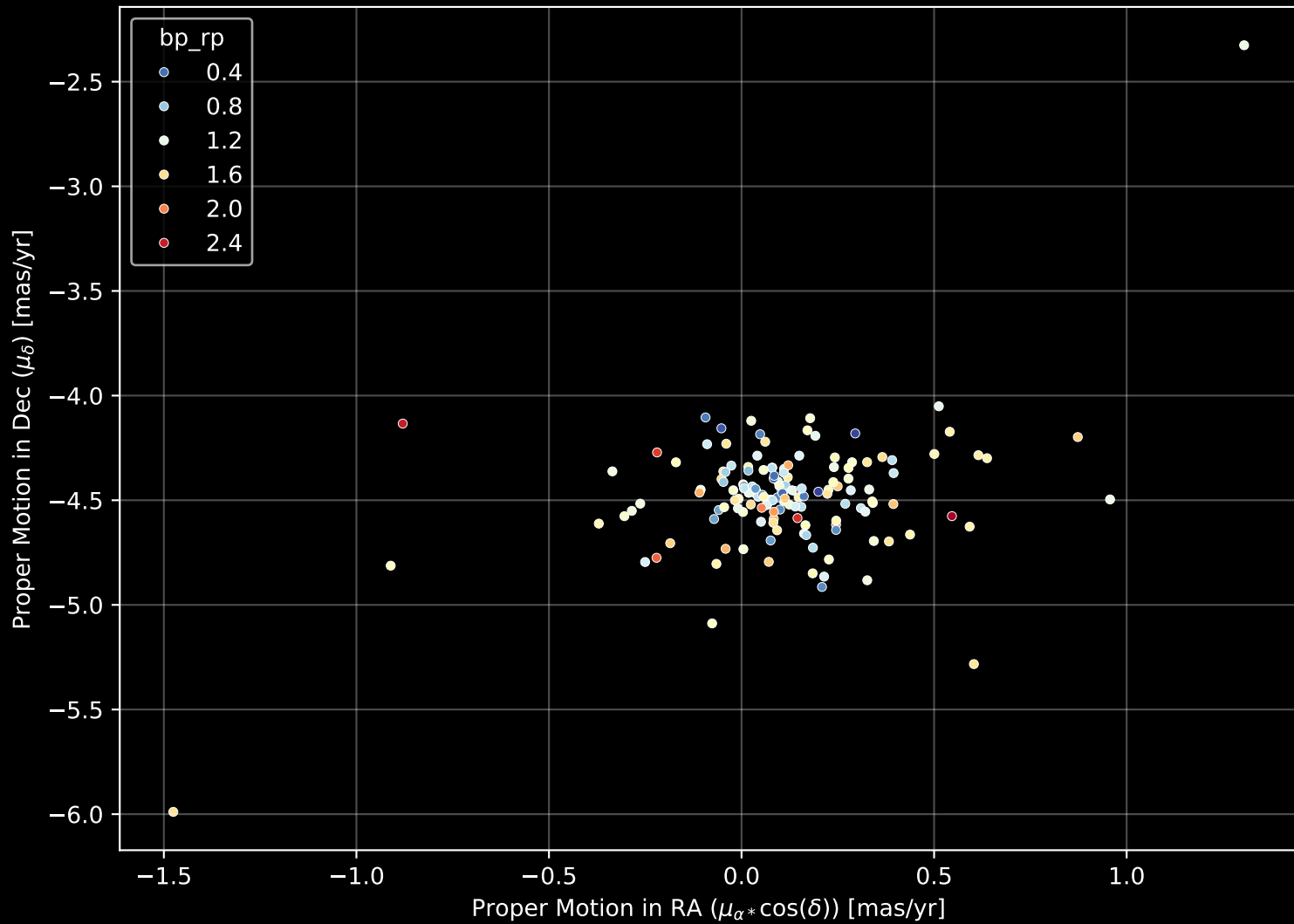
Gaia Cluster: [UPK_26] Proper Motion Diagram (n= 148)
