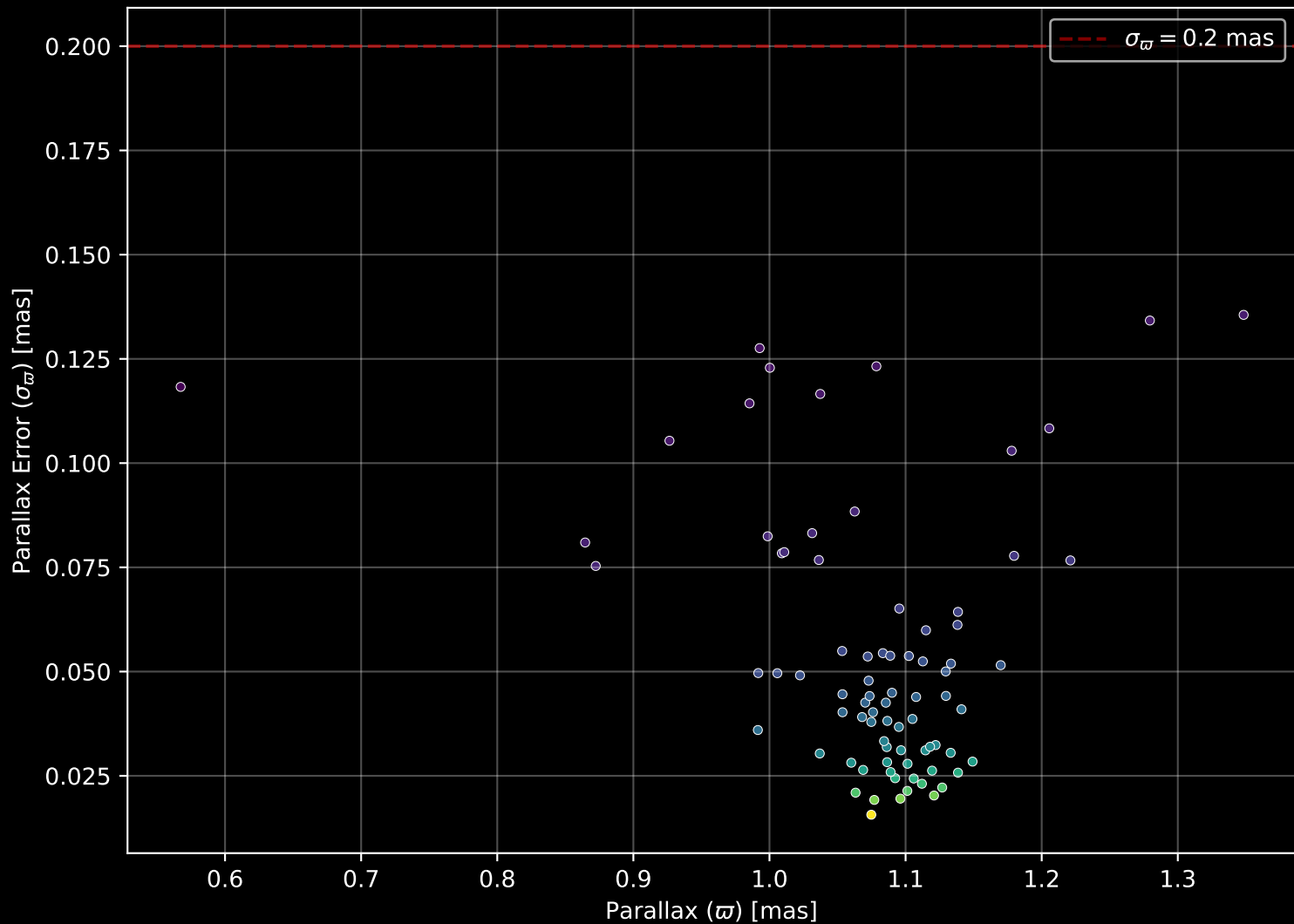
Gaia Cluster: [UPK_27] Parallax Quality (n= 80)
