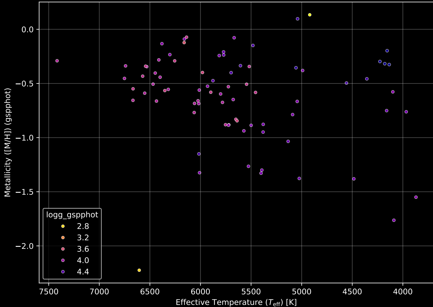
Gaia Cluster: [UPK_27] Stellar Population Parameters (n= 80)
