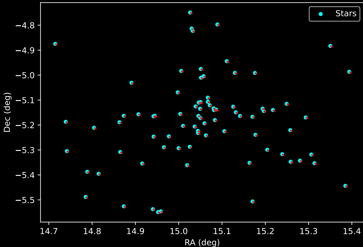
Gaia Cluster: [UPK_27] Proper Motion Vectors for Gaia Star Field (n= 80)
