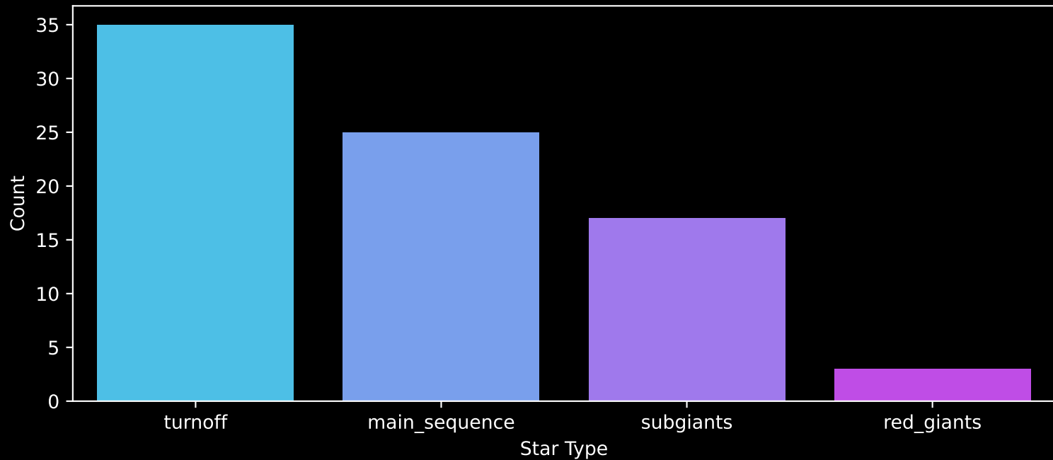
Gaia Cluster: [UPK_27] Count plot of Star Type
