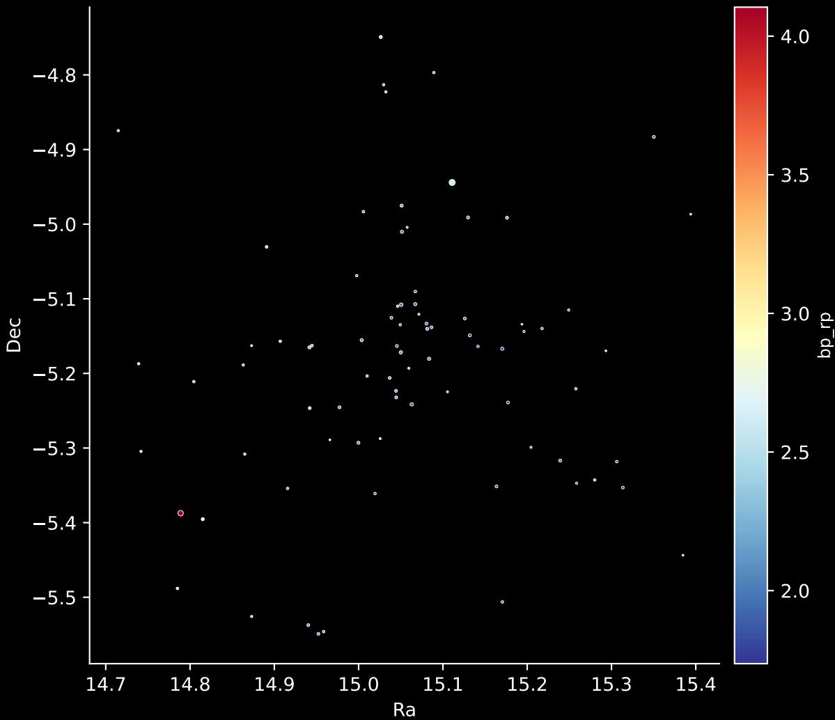
Gaia Cluster: [UPK_27] Stars: 80
