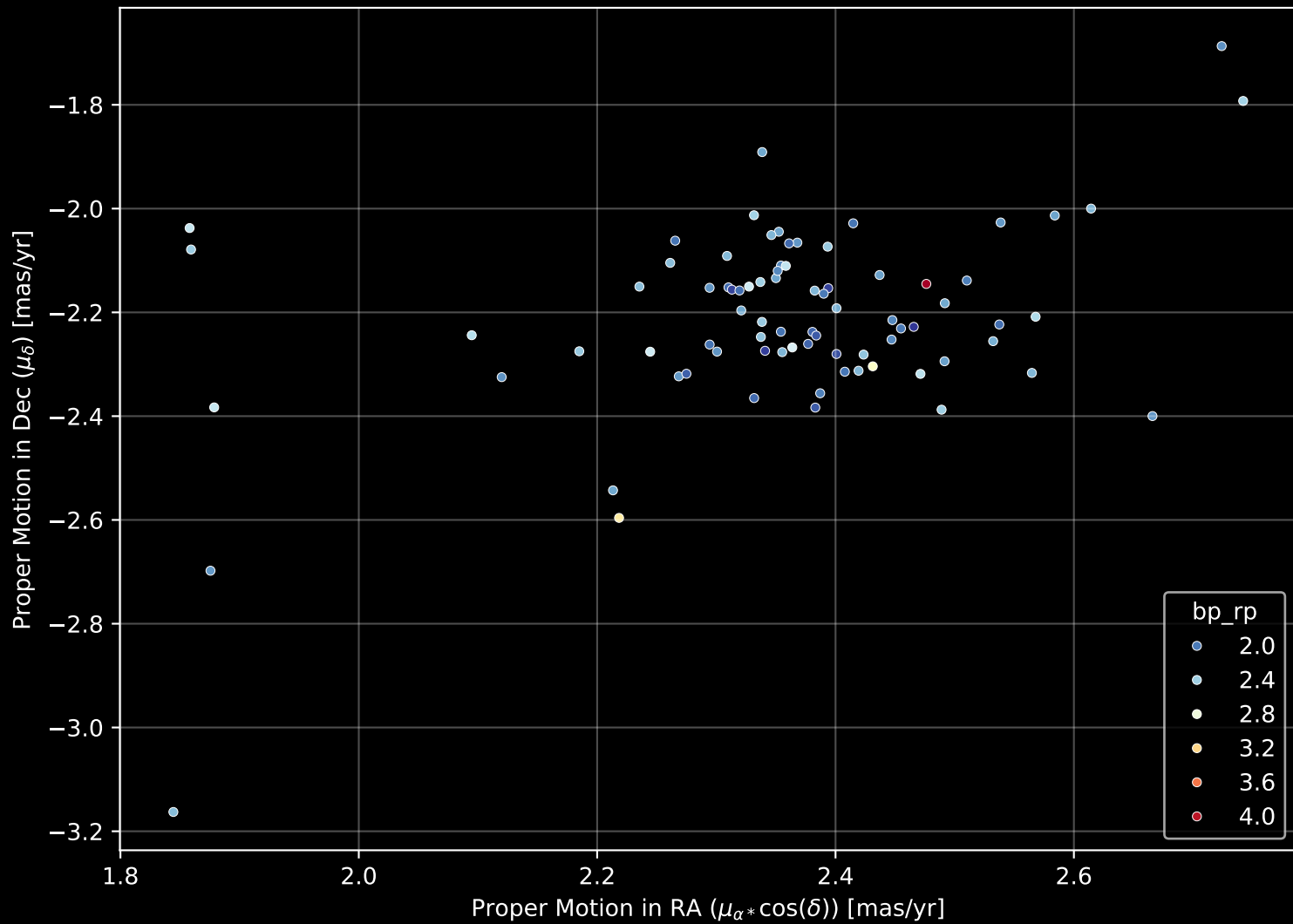
Gaia Cluster: [UPK_27] Proper Motion Diagram (n= 80)
