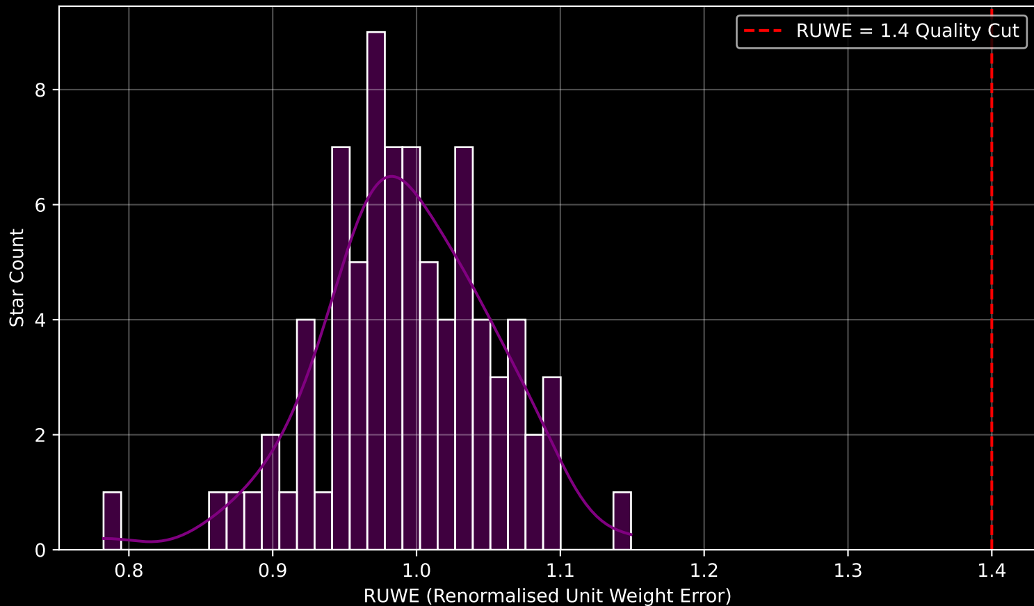
Gaia Cluster: [UPK_27] RUWE Distribution (n= 80)
