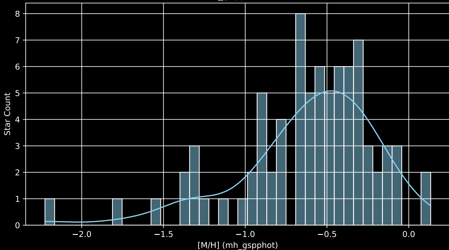
Gaia Cluster: [UPK_27 [M/H] (mh_gspphot) (n= 80)
