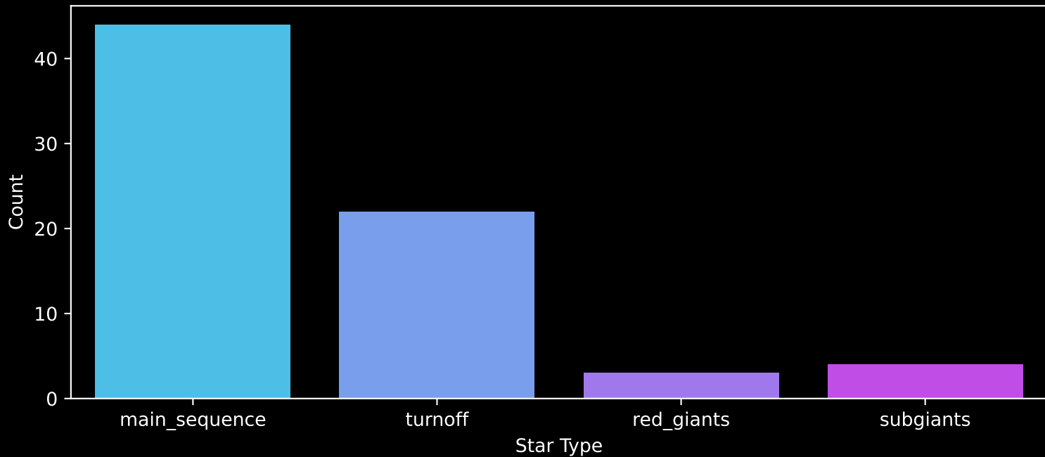
Gaia Cluster: [UPK_29] Count plot of Star Type
