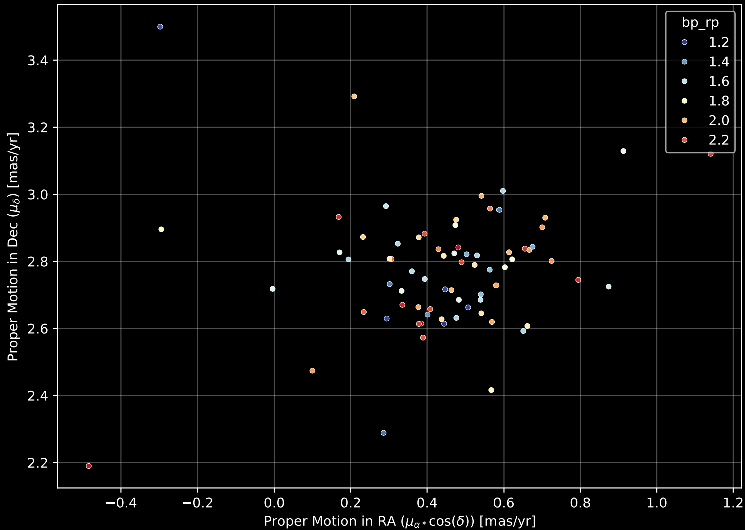
Gaia Cluster: [UPK_29] Proper Motion Diagram (n= 73)
