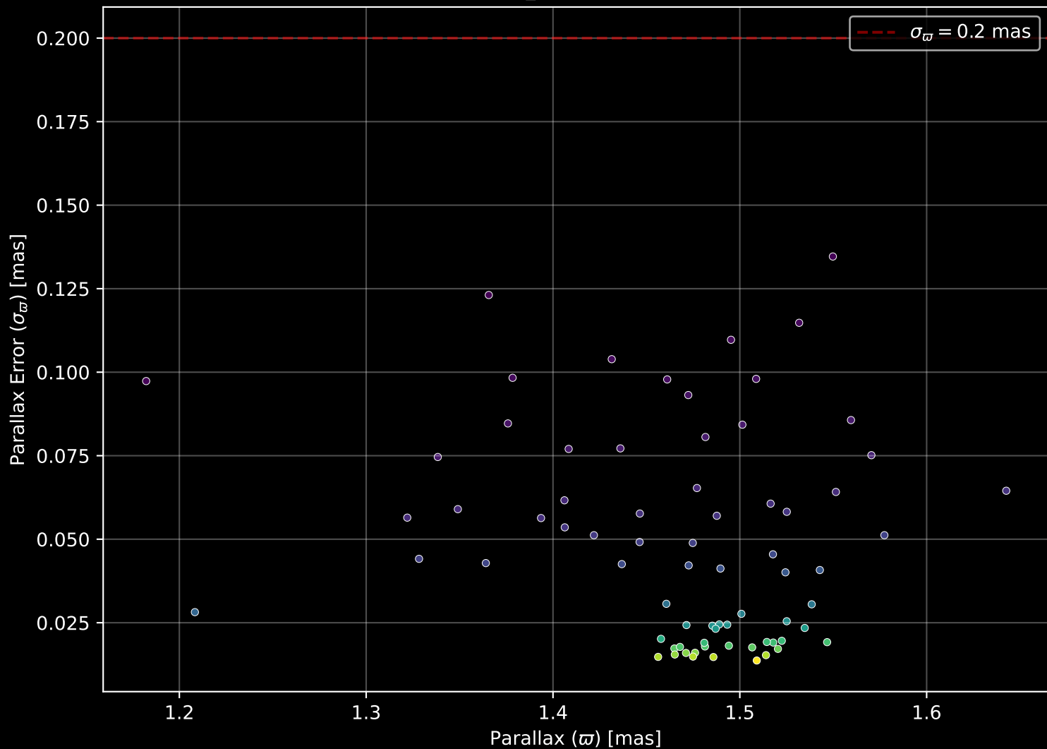
Gaia Cluster: [UPK_29] Parallax Quality (n= 73)
