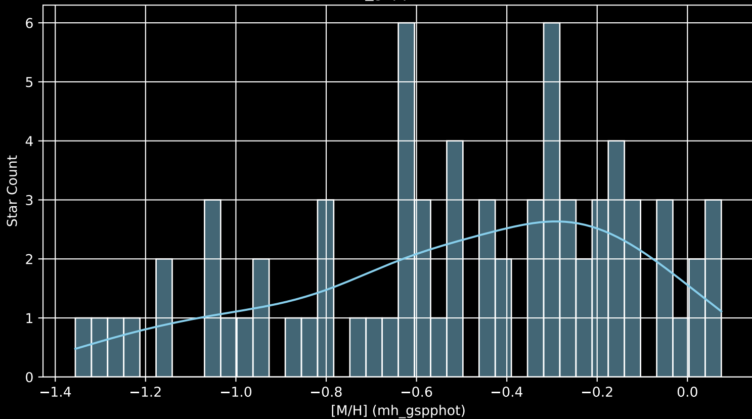
Gaia Cluster: [UPK_29 [M/H] (mh_gspphot) (n= 73)
