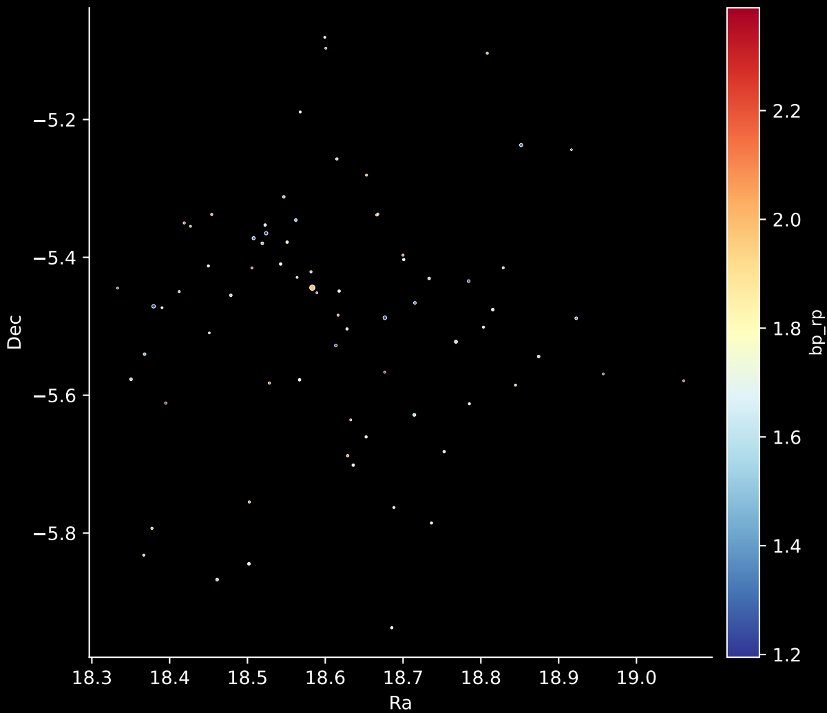
Gaia Cluster: [UPK_29] Stars: 73
