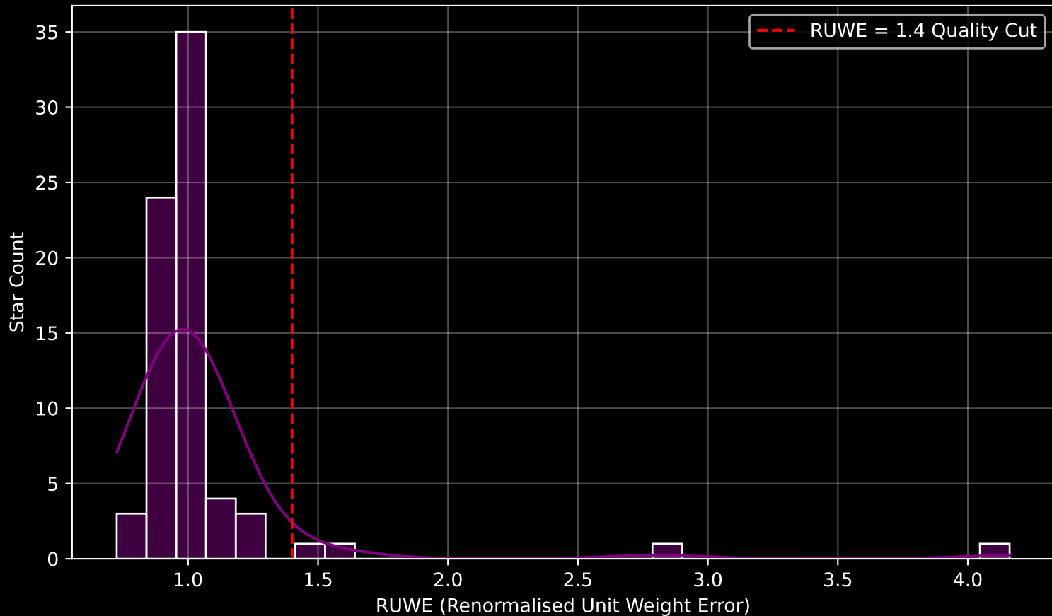
Gaia Cluster: [UPK_29] RUWE Distribution (n= 73)
