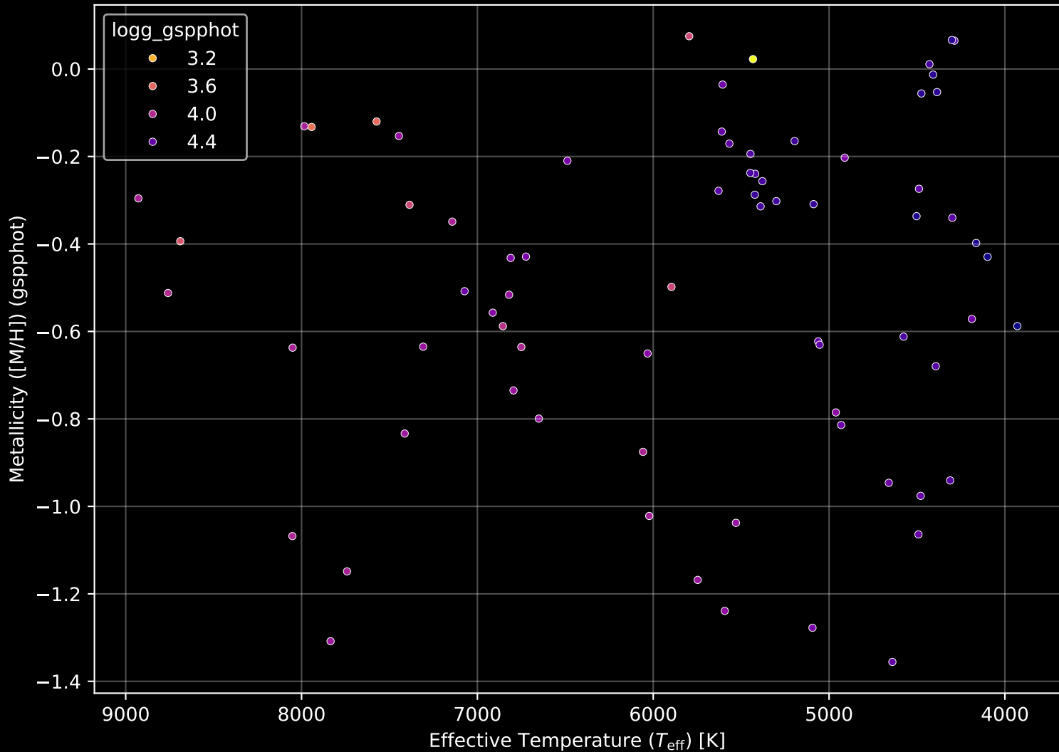
Gaia Cluster: [UPK_29] Stellar Population Parameters (n= 73)
