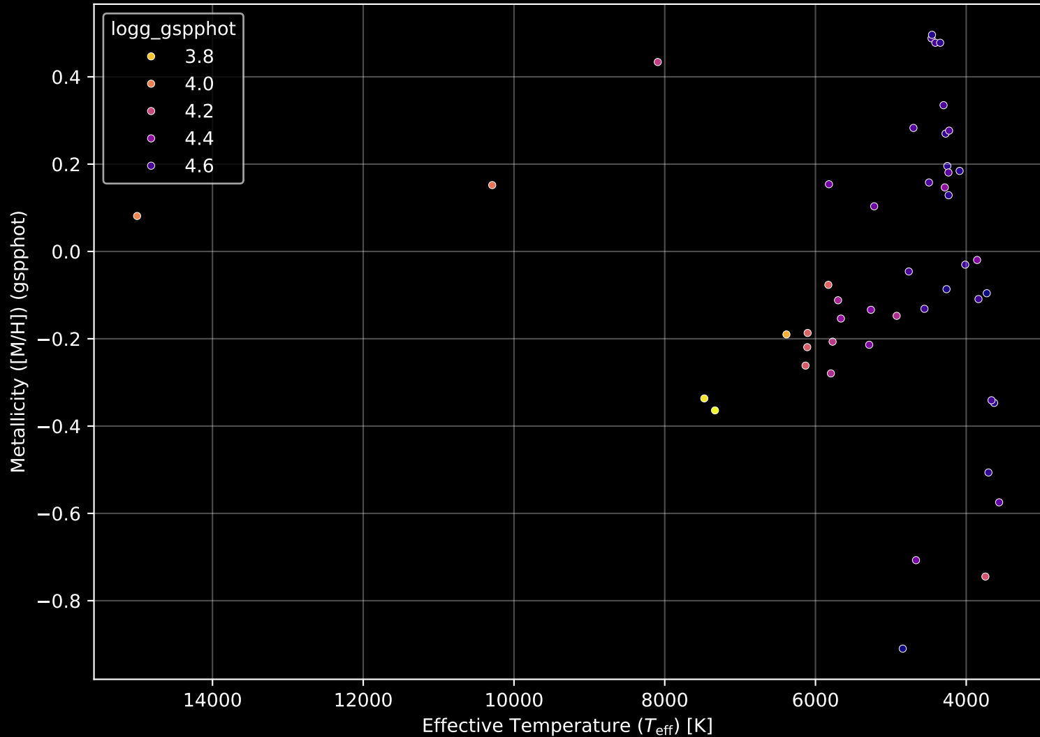
Gaia Cluster: [UPK_292] Stellar Population Parameters (n= 47)
