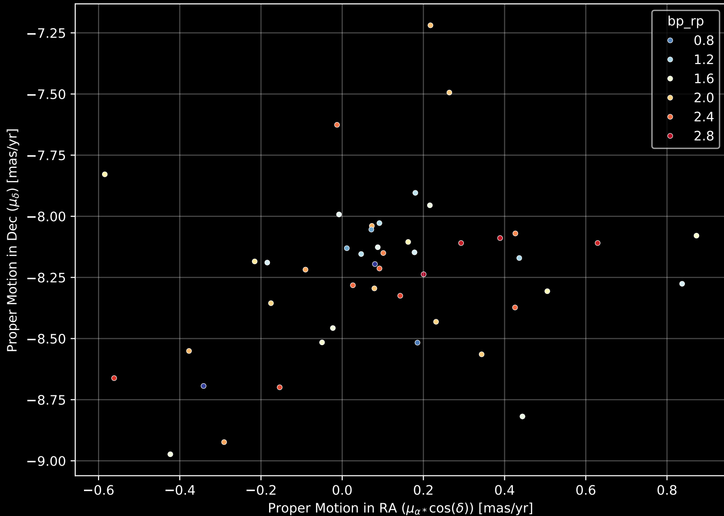
Gaia Cluster: [UPK_292] Proper Motion Diagram (n= 47)
