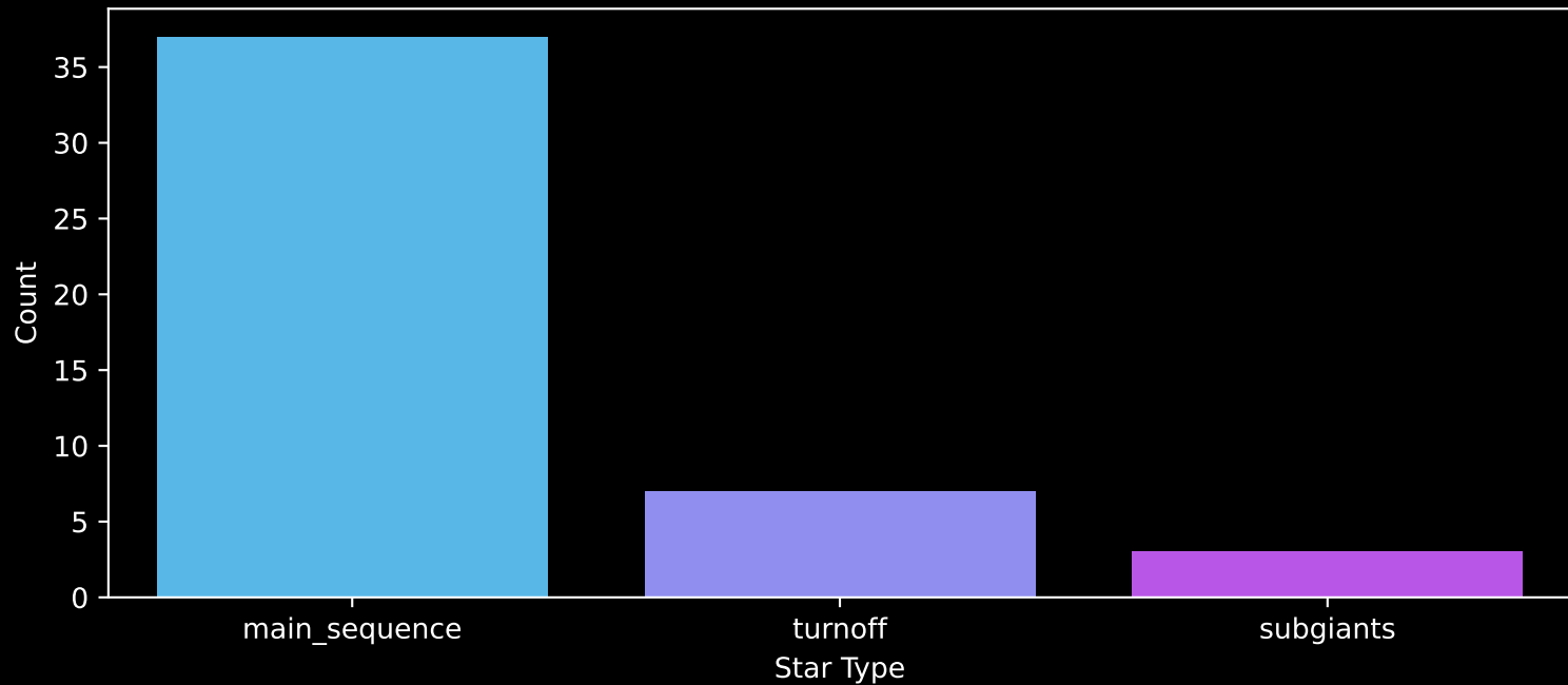
Gaia Cluster: [UPK_292] Count plot of Star Type
