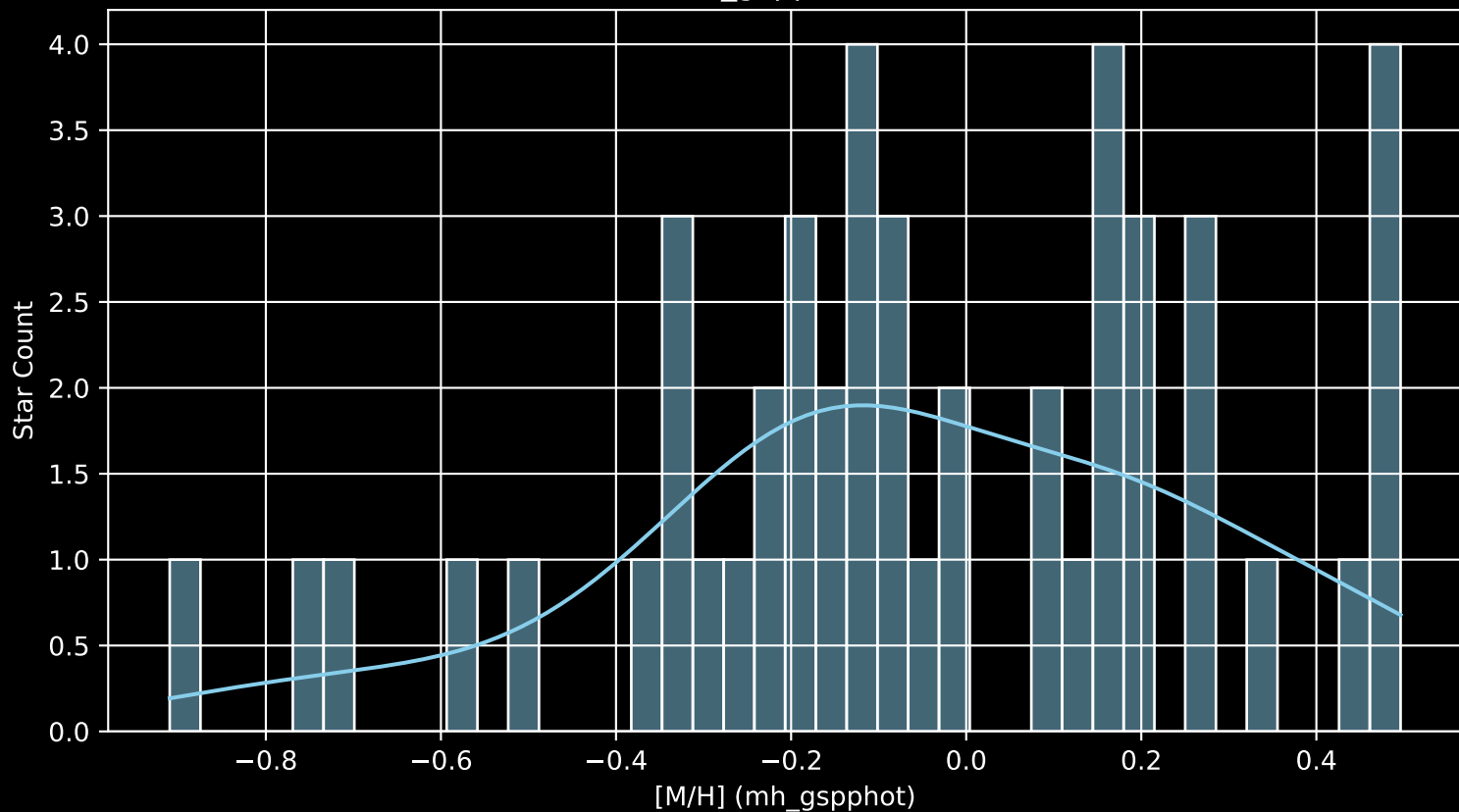
Gaia Cluster: [UPK_292 [M/H] (mh_gspphot) (n= 47)
