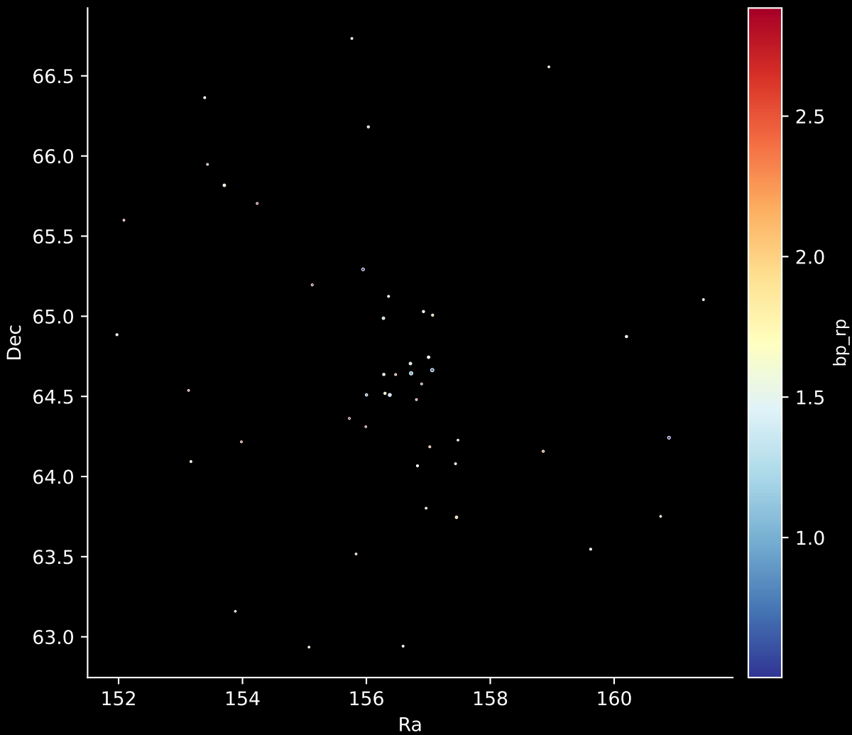
Gaia Cluster: [UPK_292] Stars: 47
