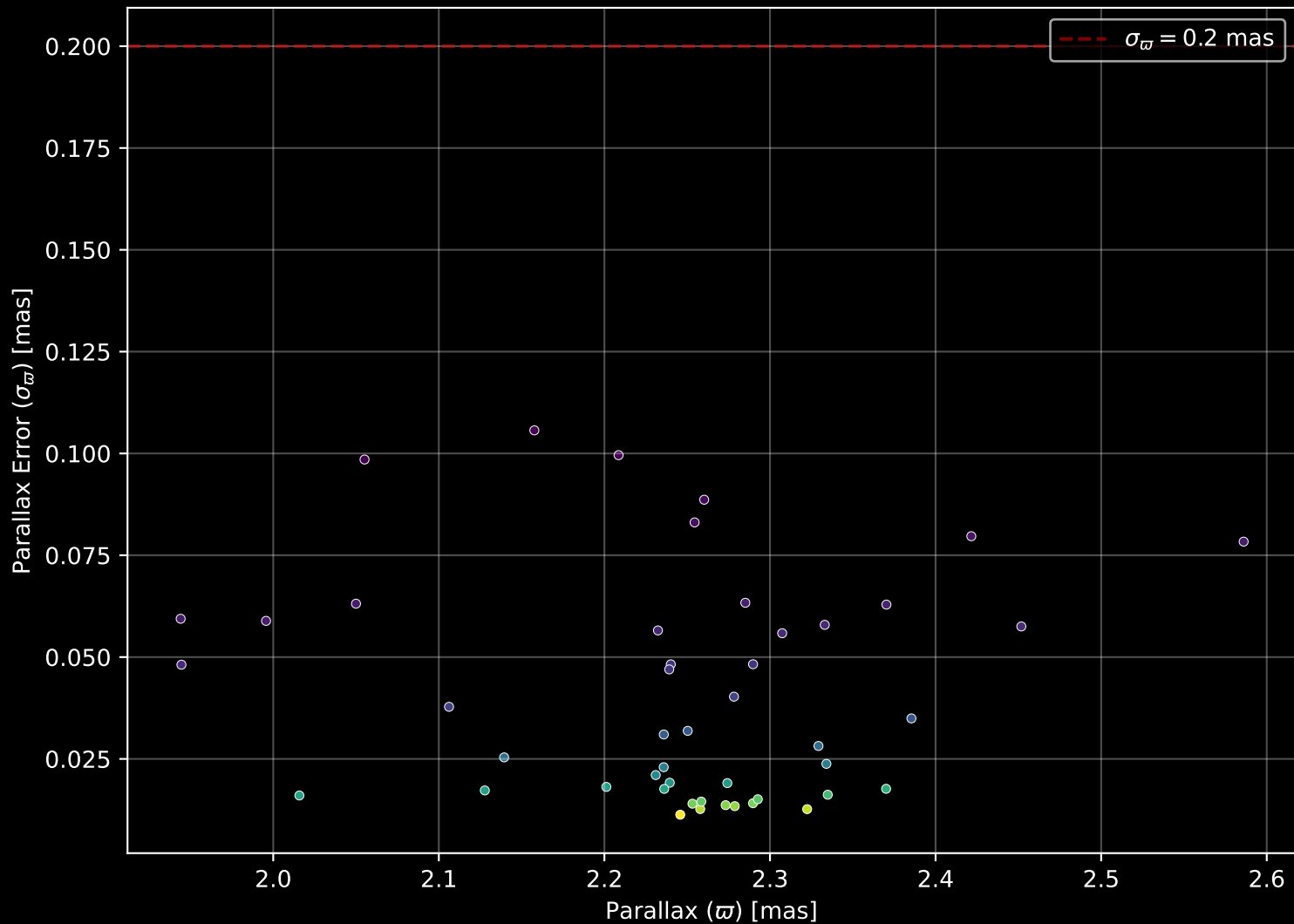
Gaia Cluster: [UPK_292] Parallax Quality (n= 47)
