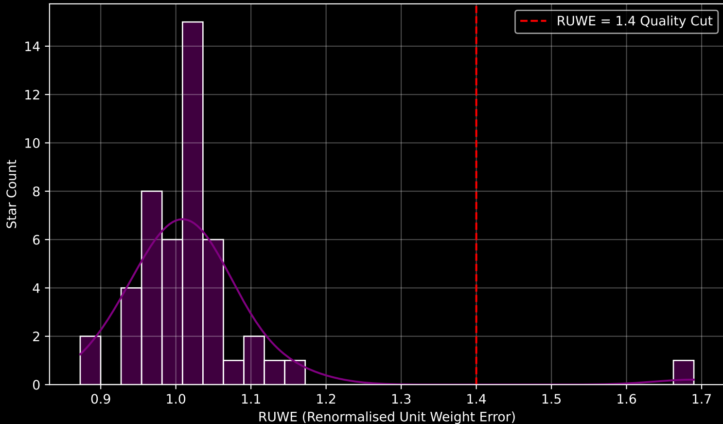
Gaia Cluster: [UPK_292] RUWE Distribution (n= 47)
