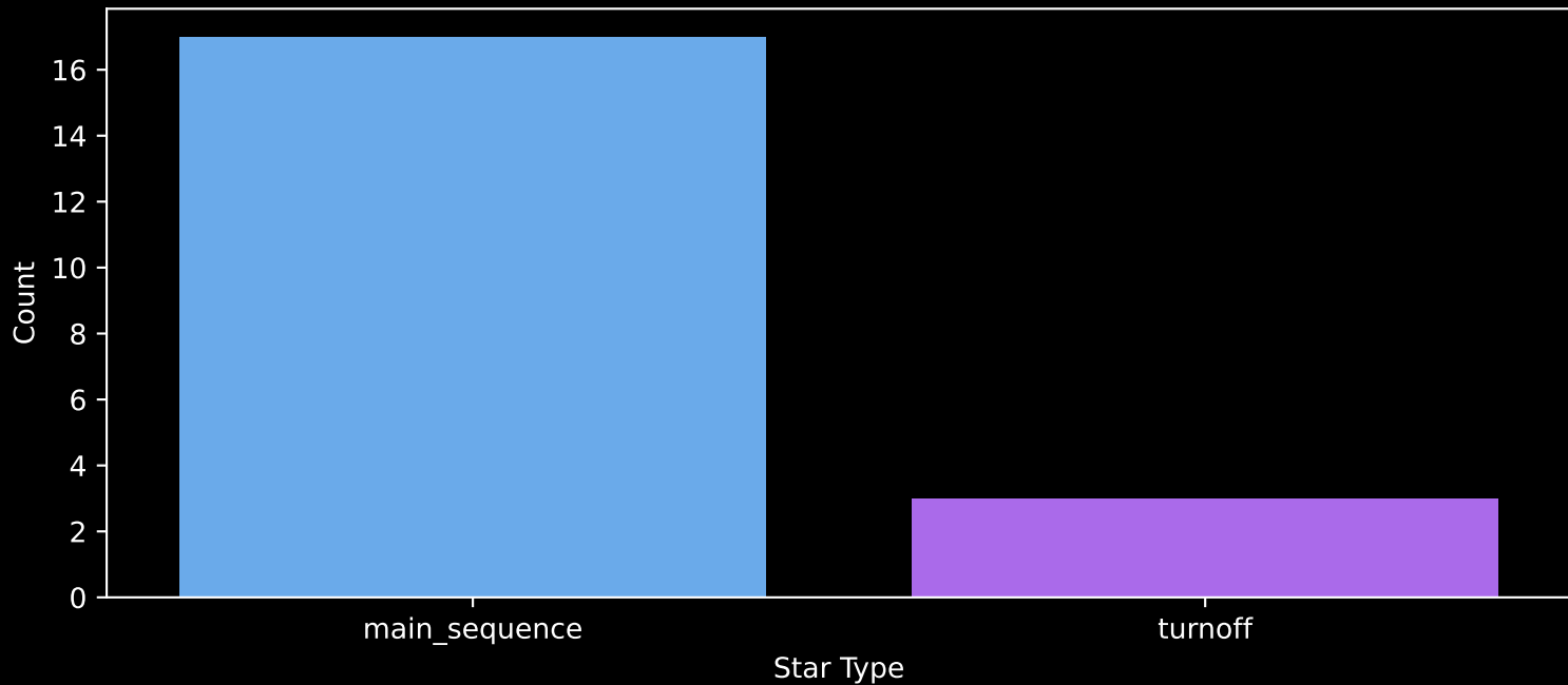
Gaia Cluster: [UPK_303] Count plot of Star Type
