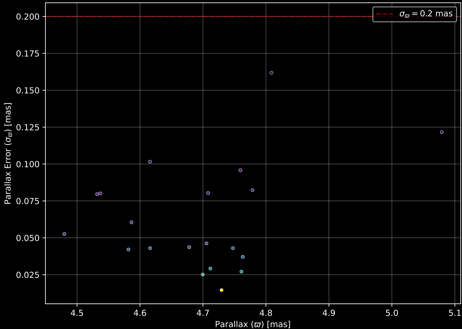
Gaia Cluster: [UPK_303] Parallax Quality (n= 20)
