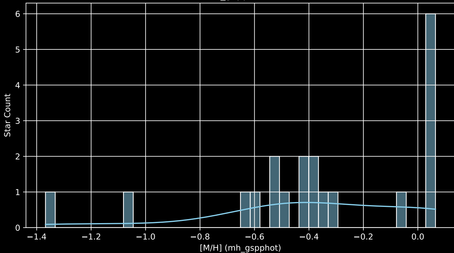
Gaia Cluster: [UPK_303 [M/H] (mh_gspphot) (n= 20)
