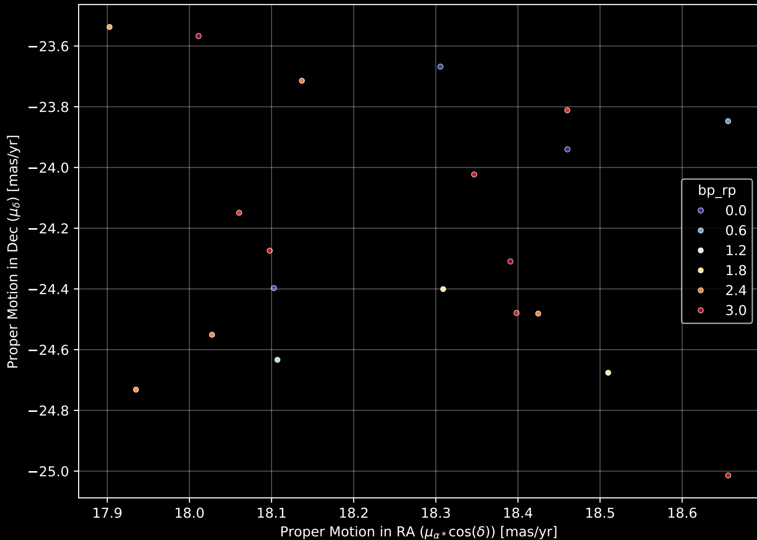
Gaia Cluster: [UPK_303] Proper Motion Diagram (n= 20)
