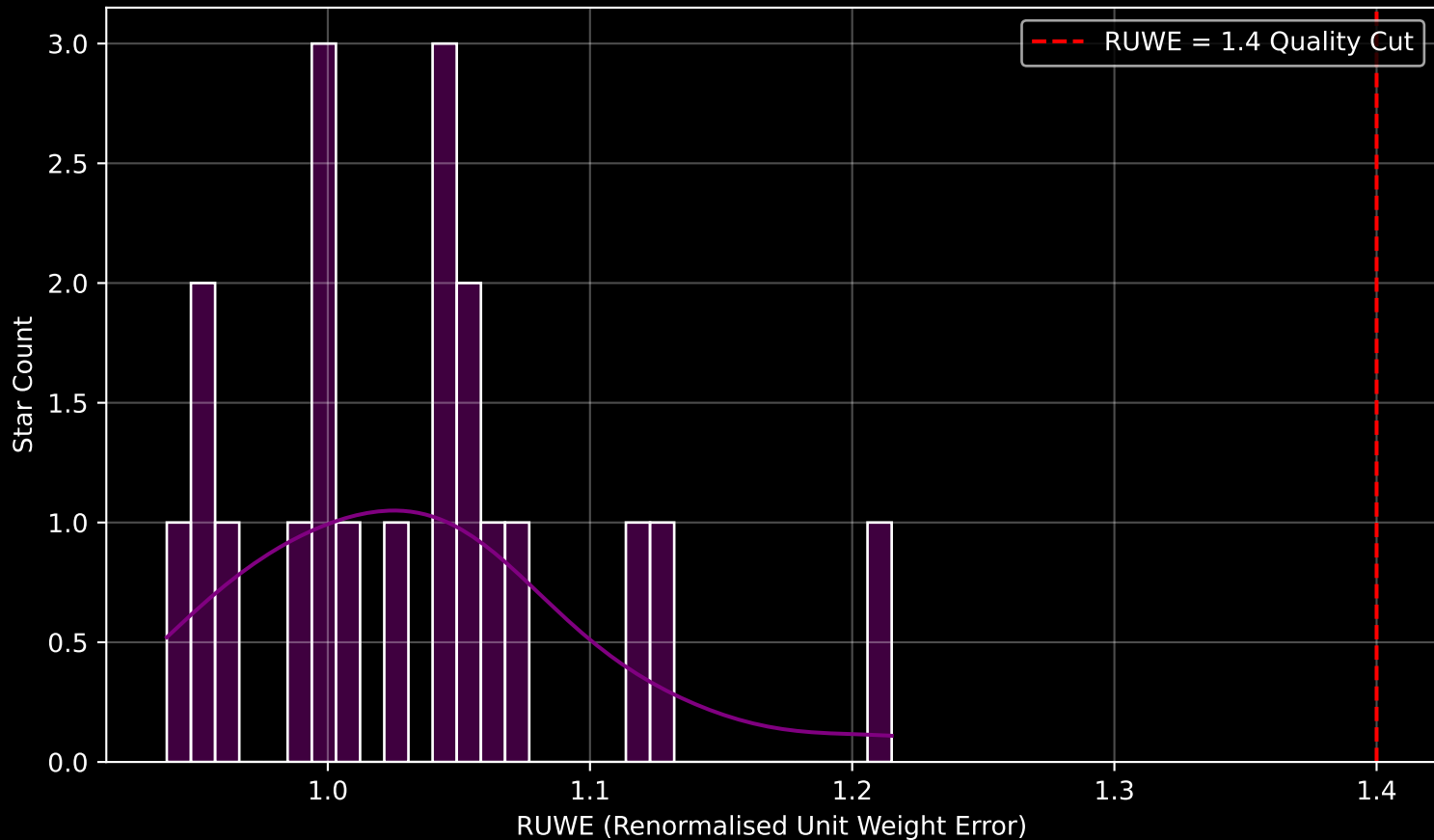
Gaia Cluster: [UPK_303] RUWE Distribution (n= 20)
