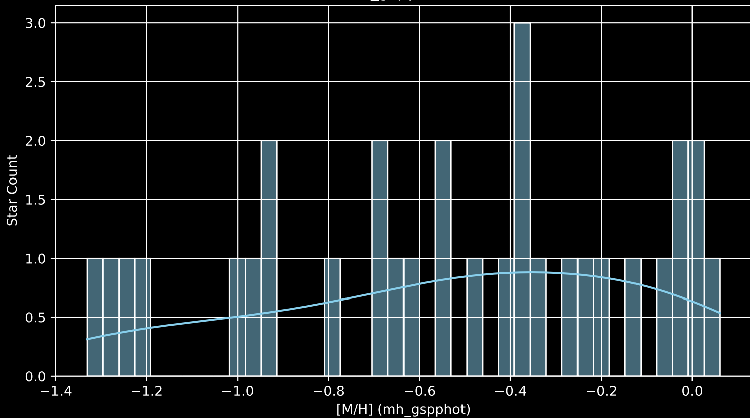
Gaia Cluster: [UPK_33 [M/H] (mh_gspphot) (n= 31)
