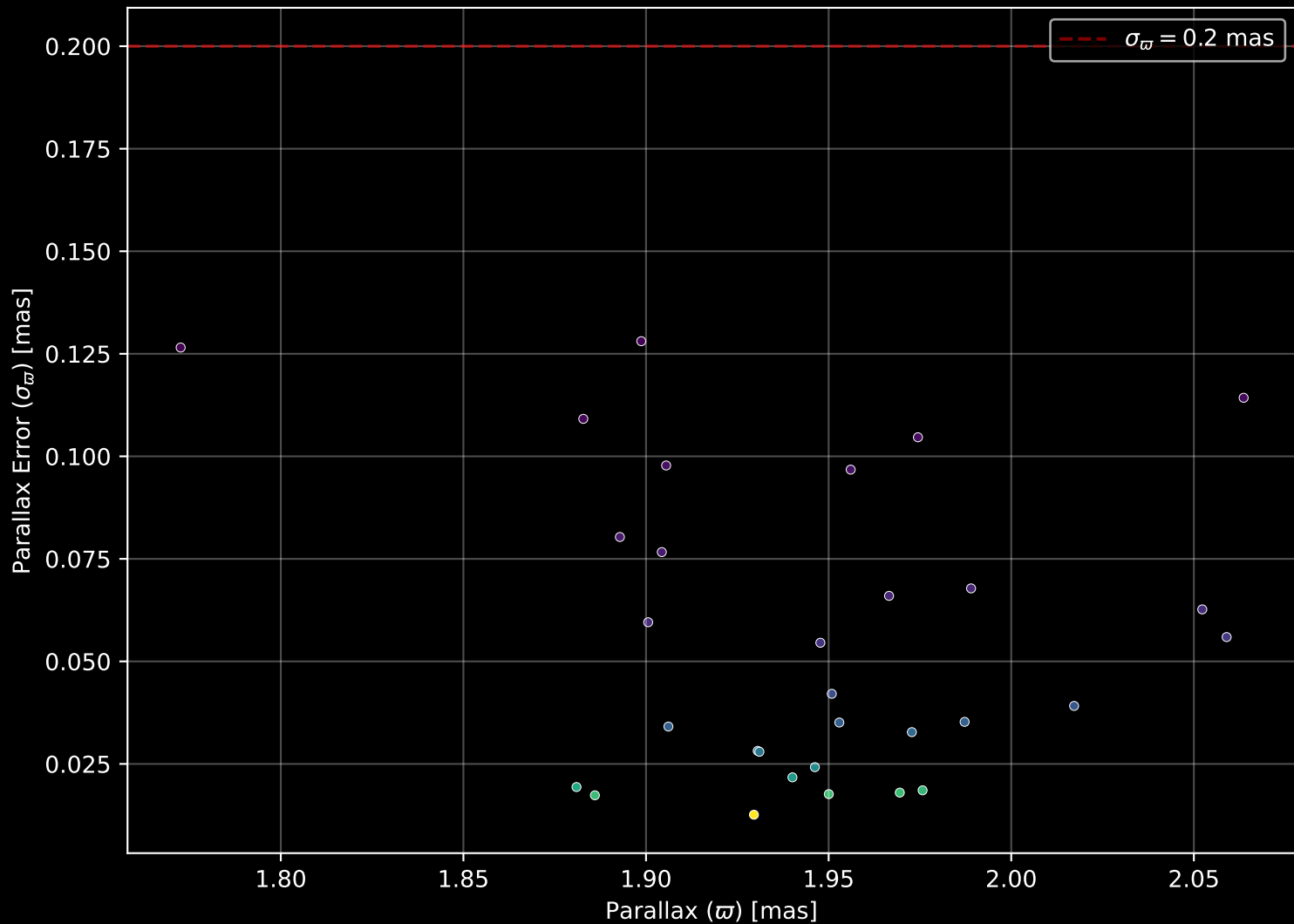
Gaia Cluster: [UPK_33] Parallax Quality (n= 31)
