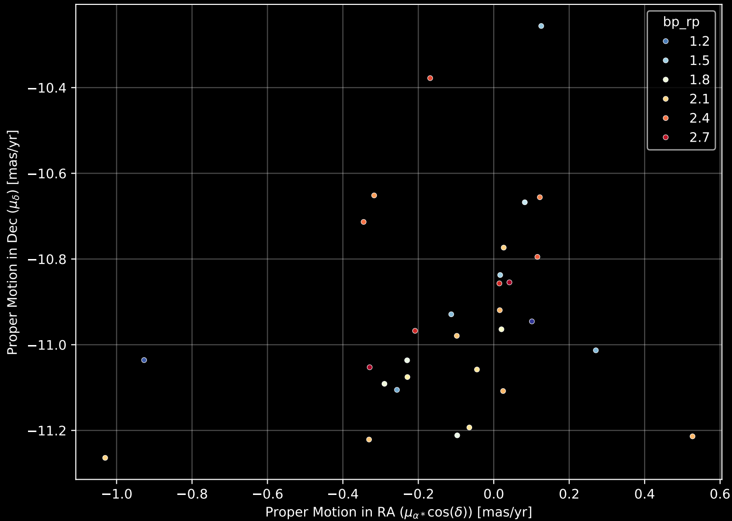
Gaia Cluster: [UPK_33] Proper Motion Diagram (n= 31)
