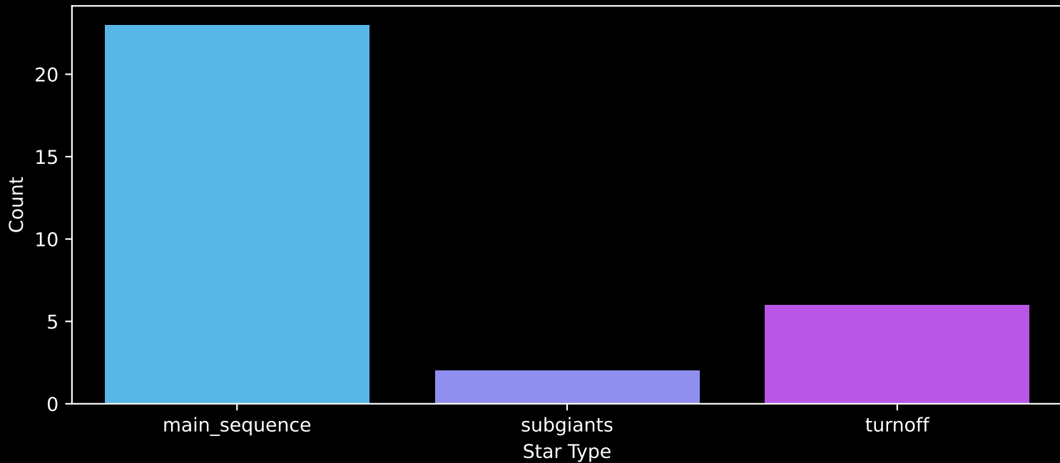
Gaia Cluster: [UPK_33] Count plot of Star Type
