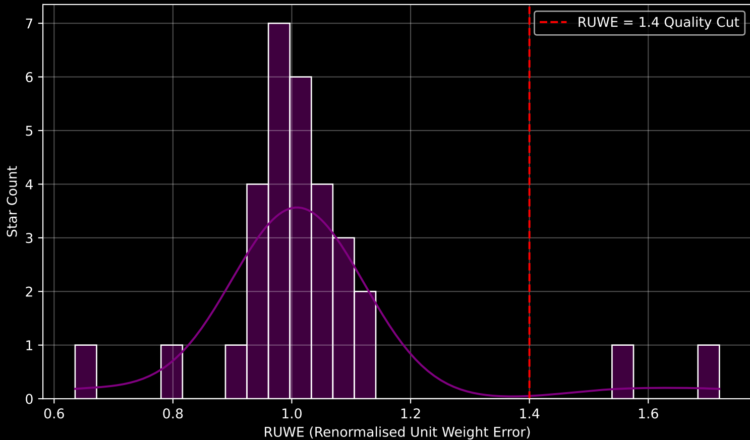
Gaia Cluster: [UPK_33] RUWE Distribution (n= 31)
