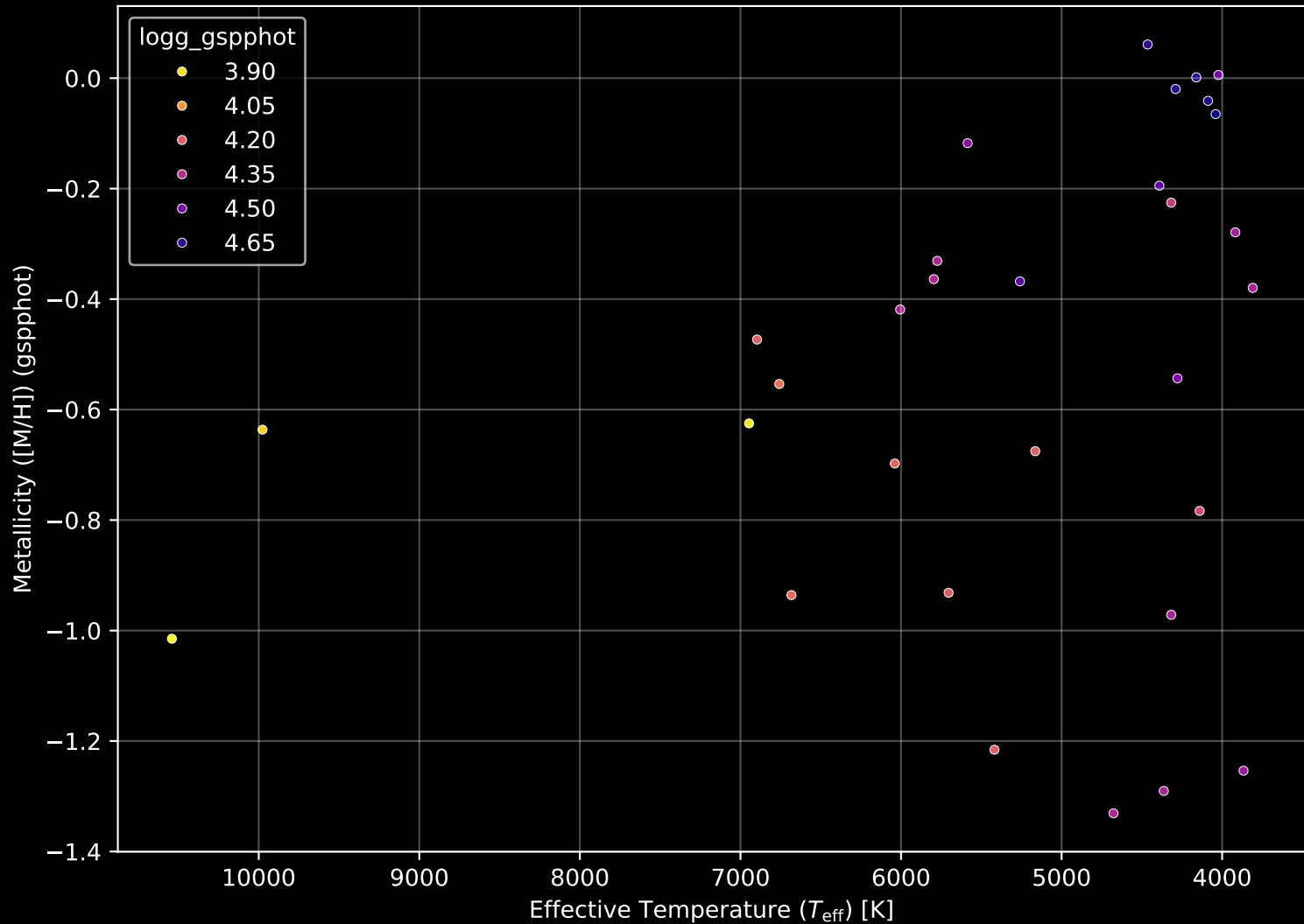
Gaia Cluster: [UPK_33] Stellar Population Parameters (n= 31)
