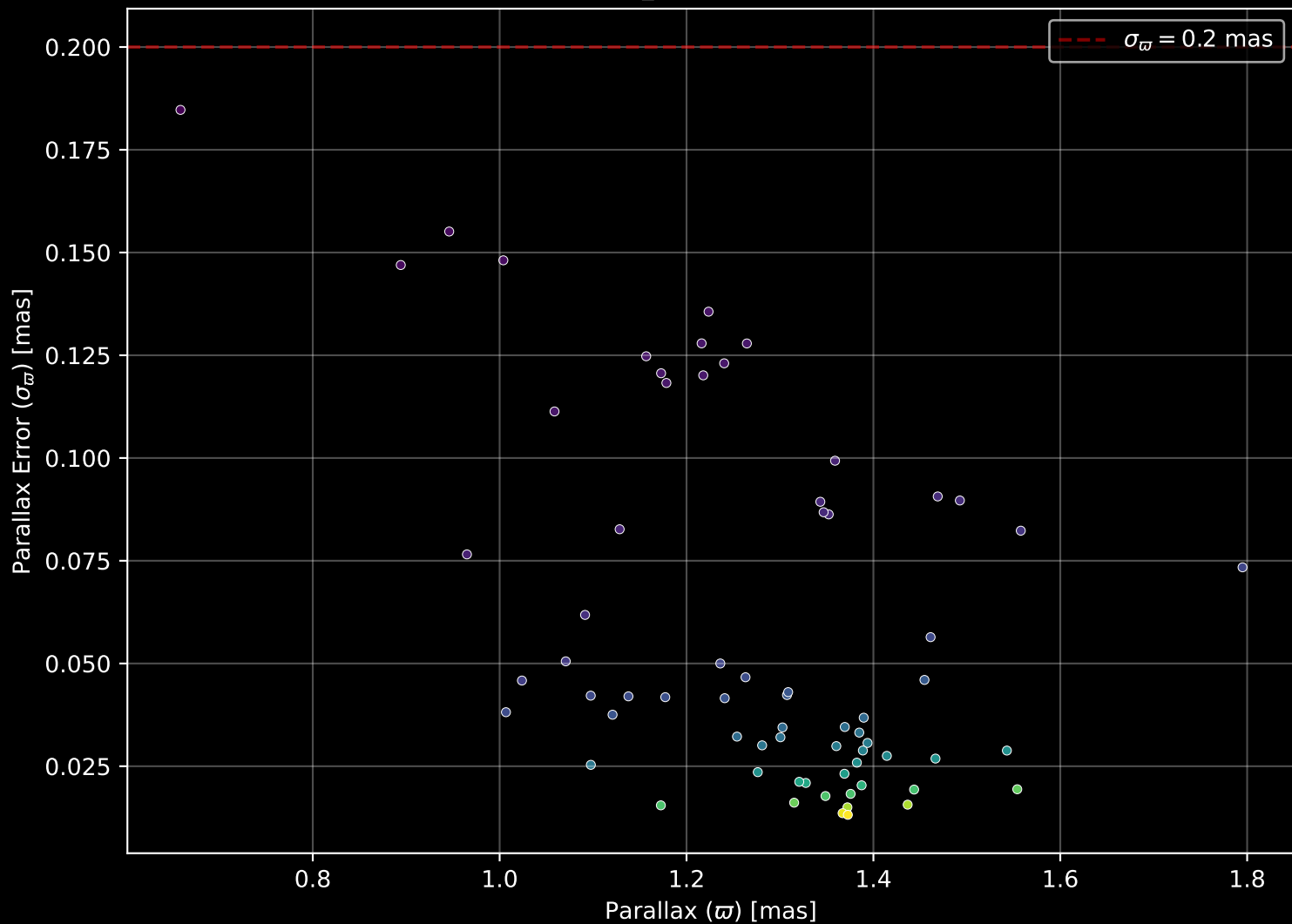
Gaia Cluster: [UPK_369] Parallax Quality (n= 68)
