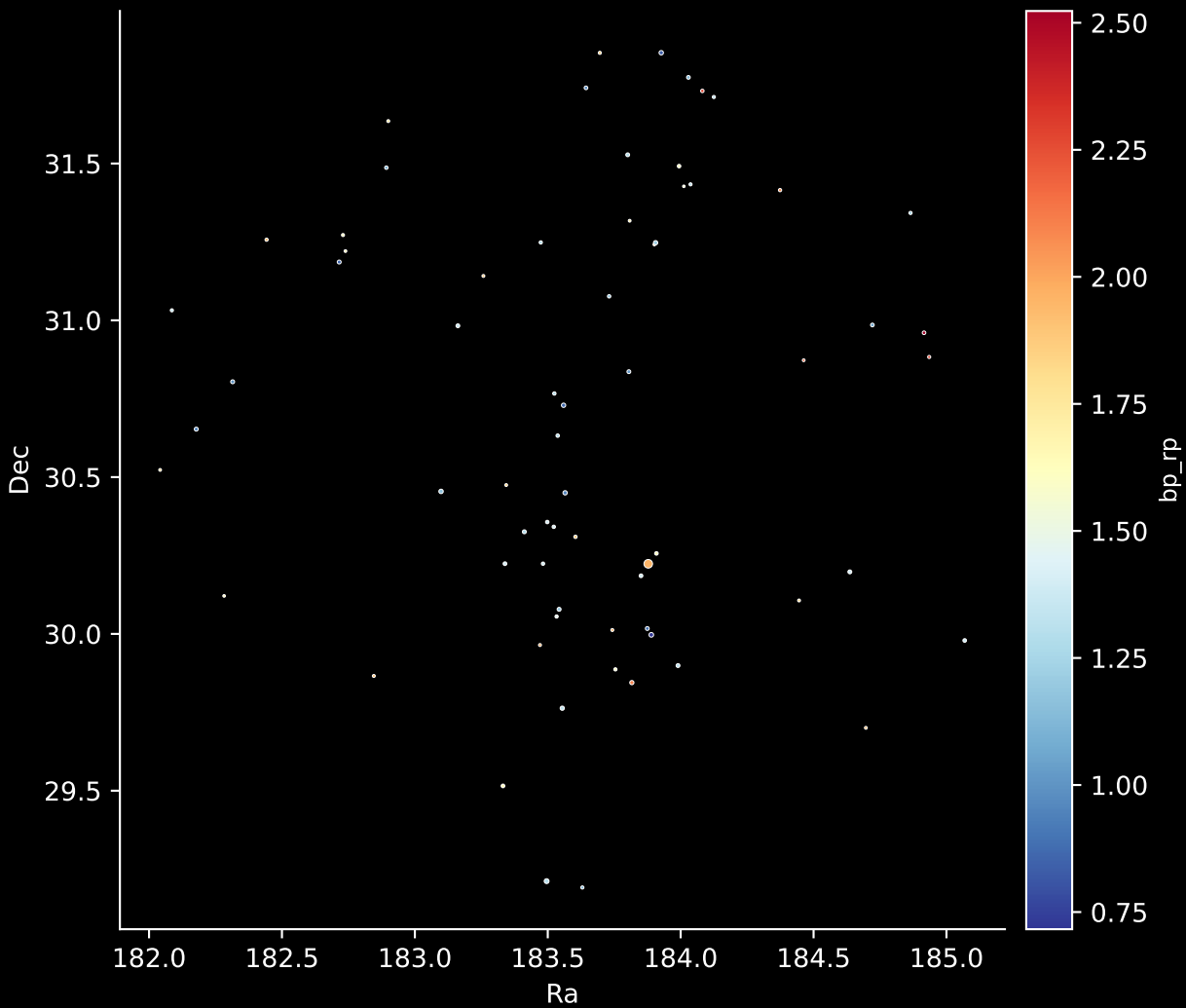
Gaia Cluster: [UPK_369] Stars: 68
