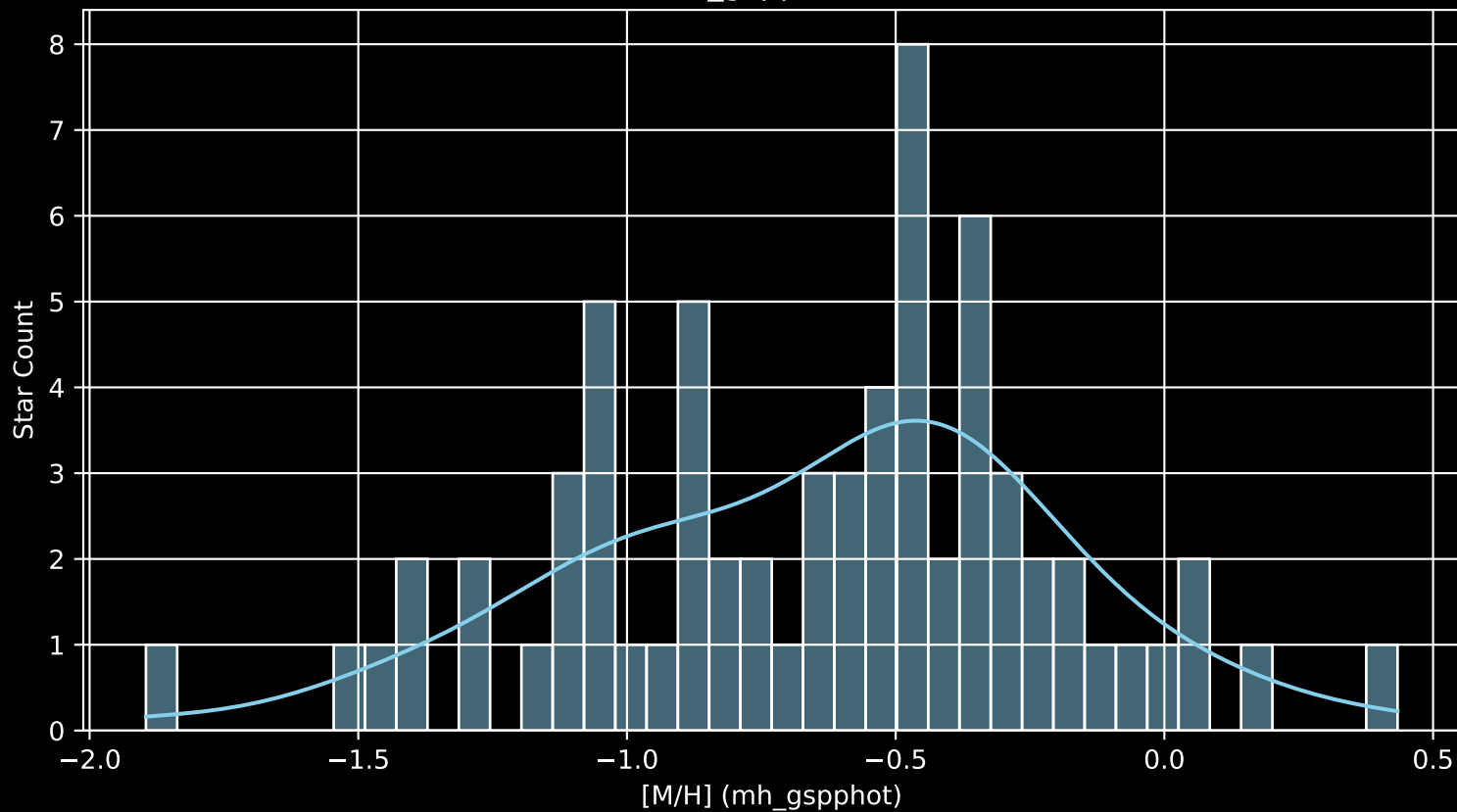
Gaia Cluster: [UPK_369 [M/H] (mh_gspphot) (n= 68)
