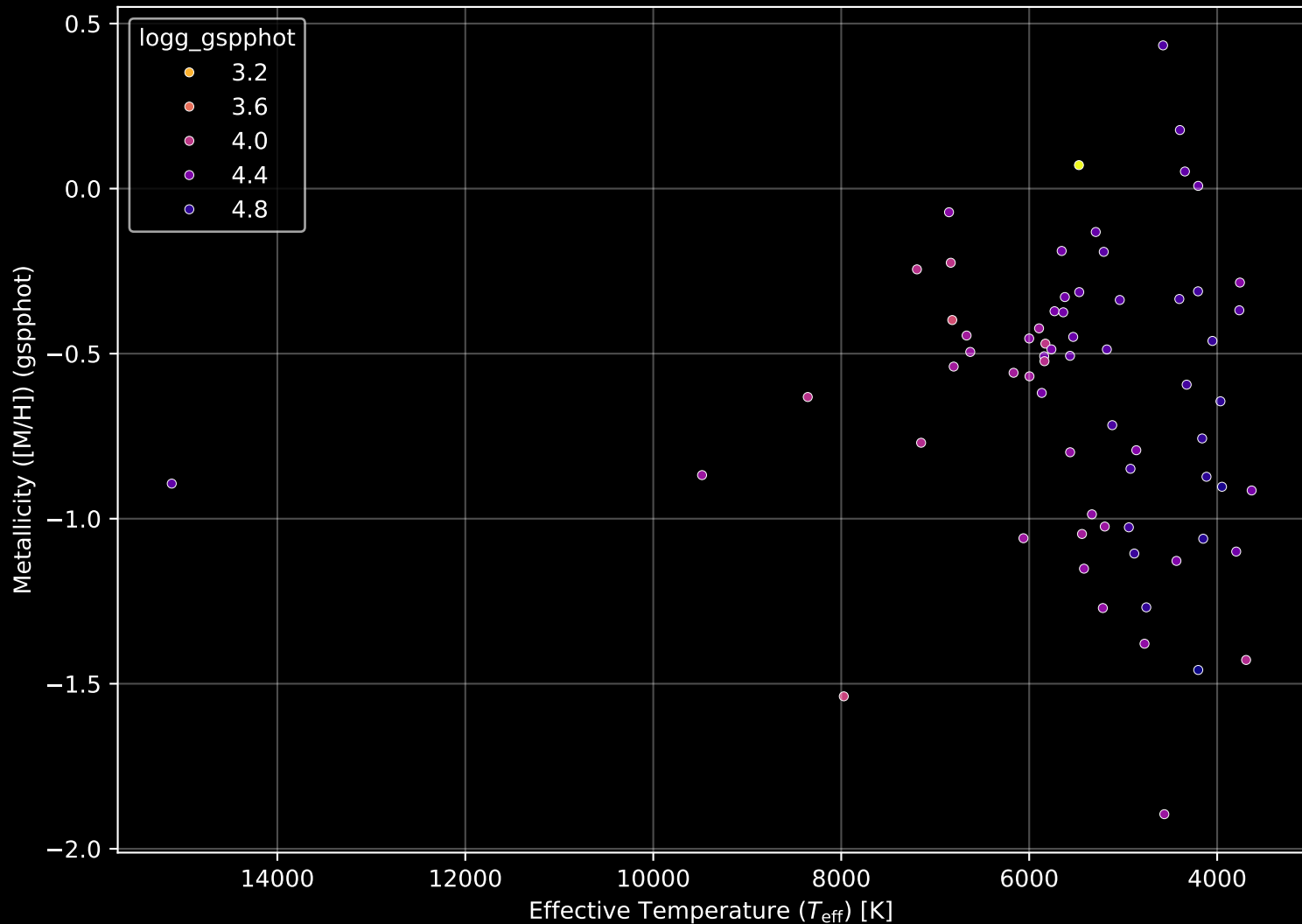
Gaia Cluster: [UPK_369] Stellar Population Parameters (n= 68)
