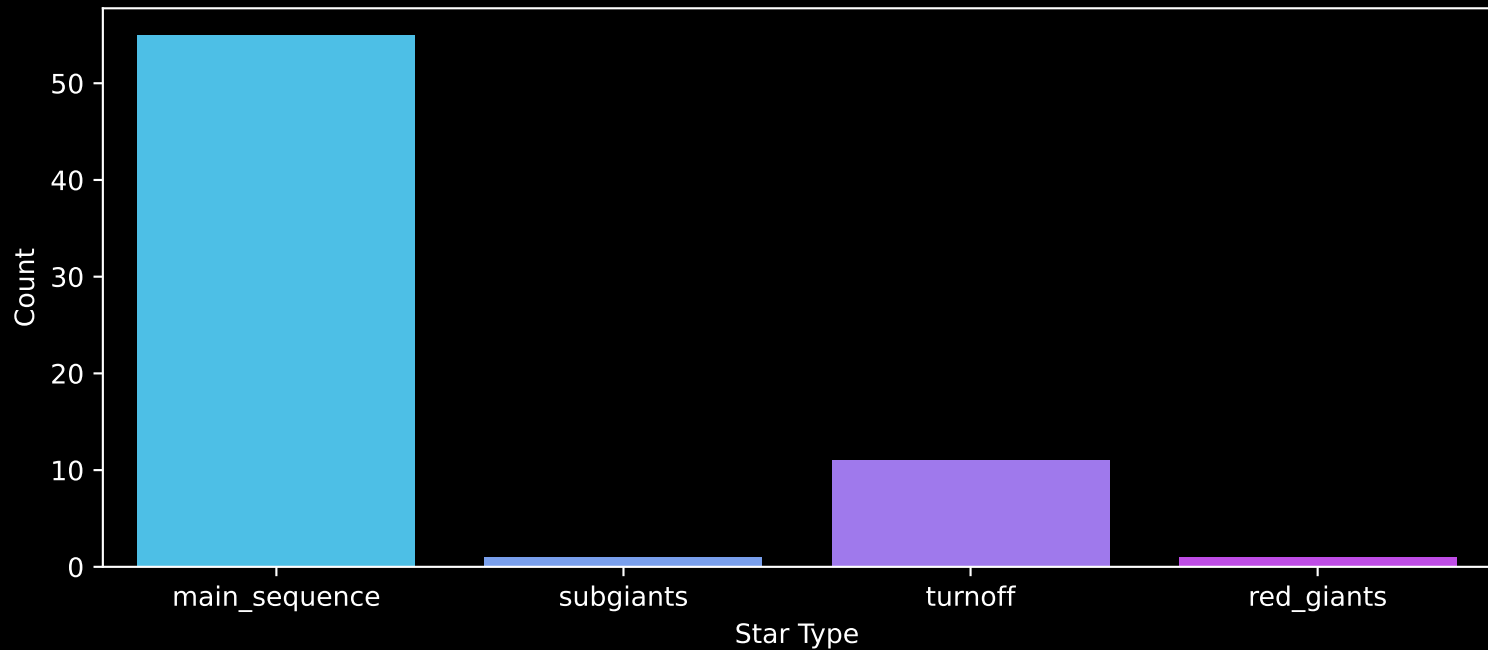
Gaia Cluster: [UPK_369] Count plot of Star Type
