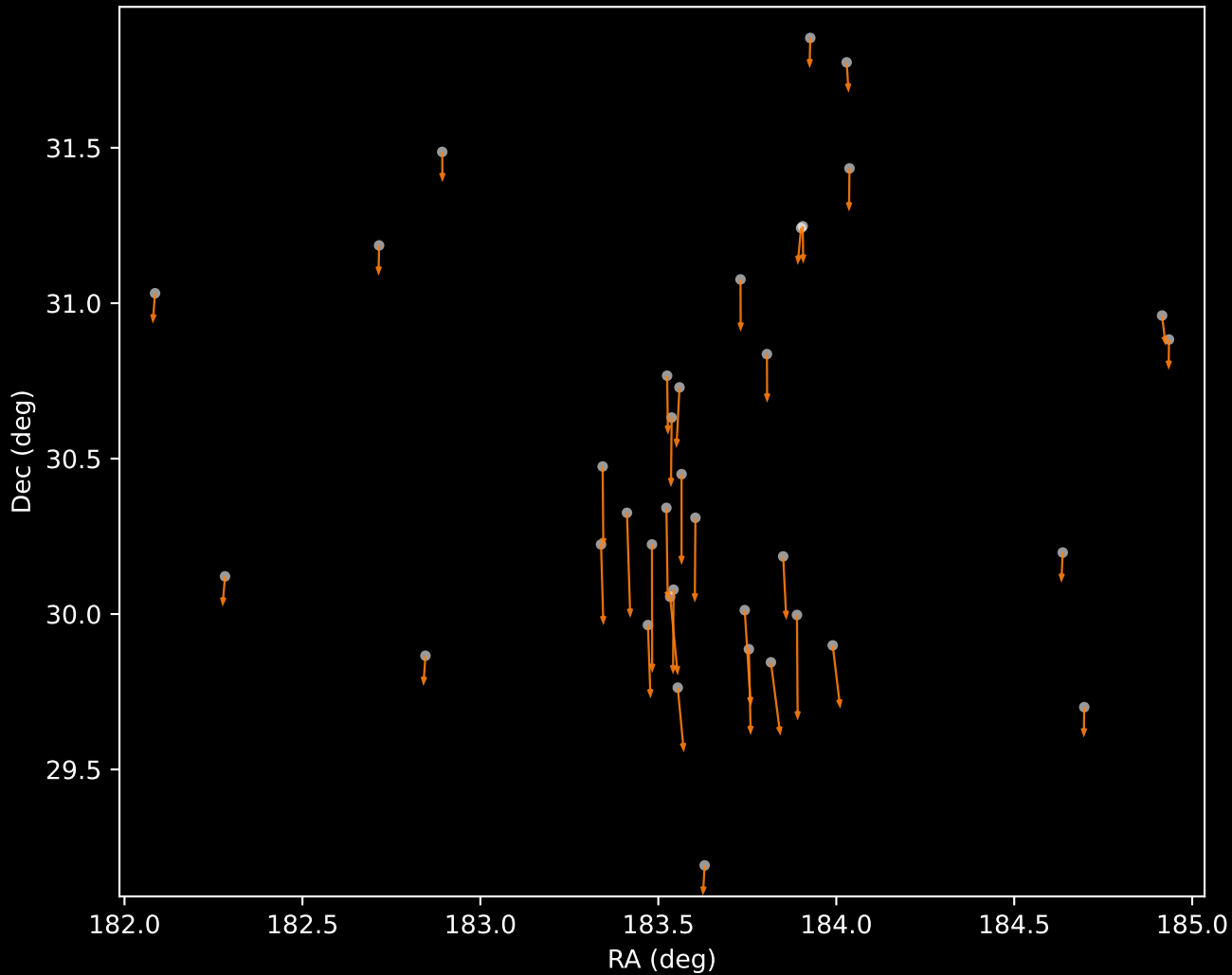
Gaia DR3 Cluster 2 Proper Motion Vectors (n=37)
