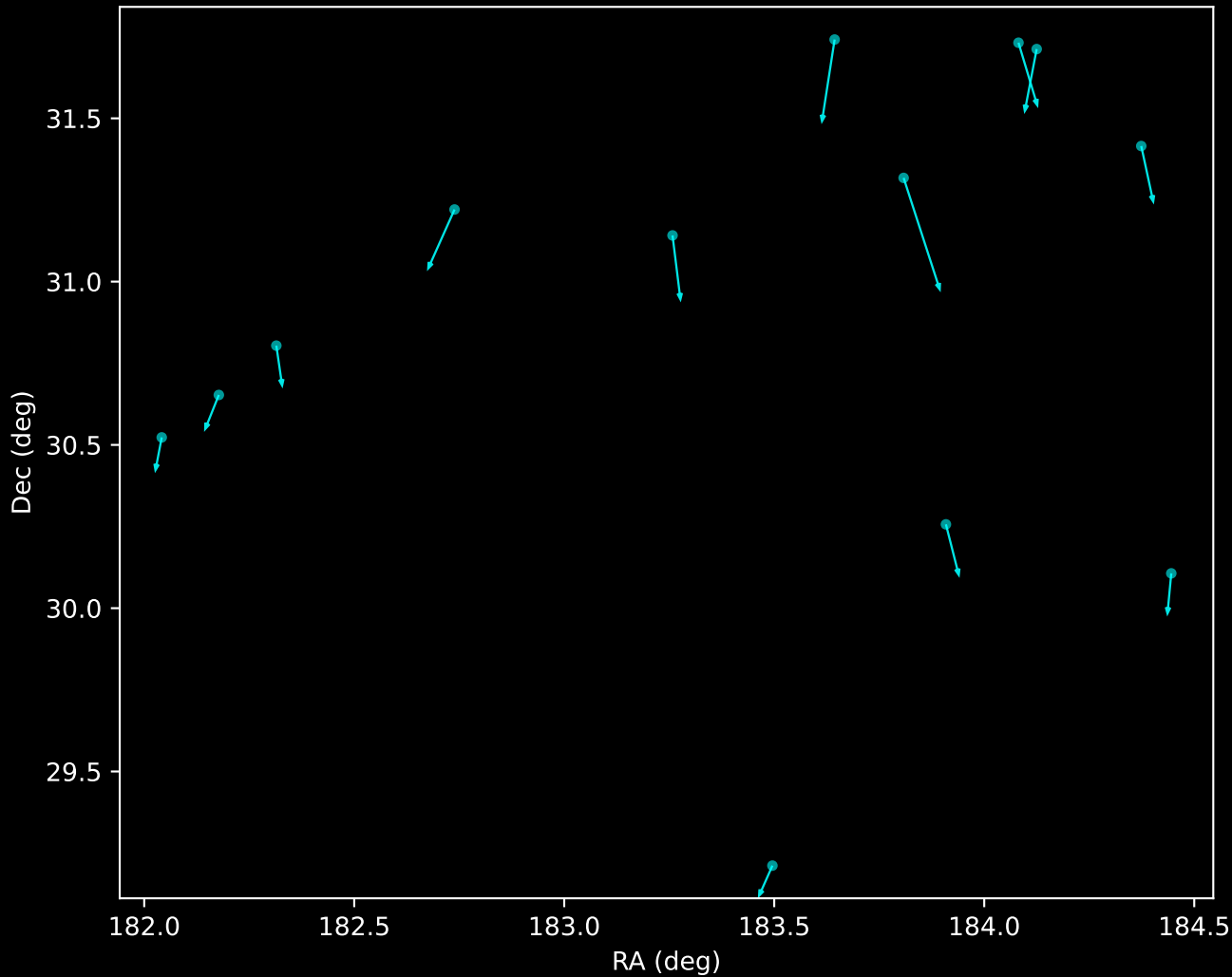
Gaia DR3 Noise Stream Proper Motion Vectors (n=13)
