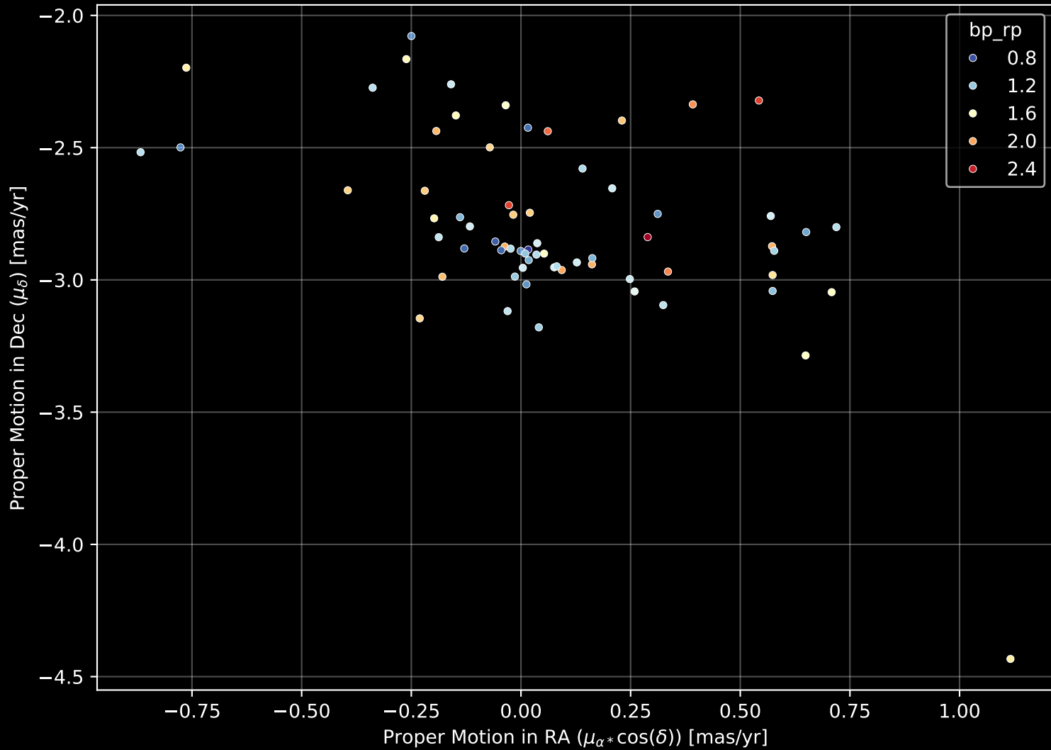
Gaia Cluster: [UPK_369] Proper Motion Diagram (n= 68)
