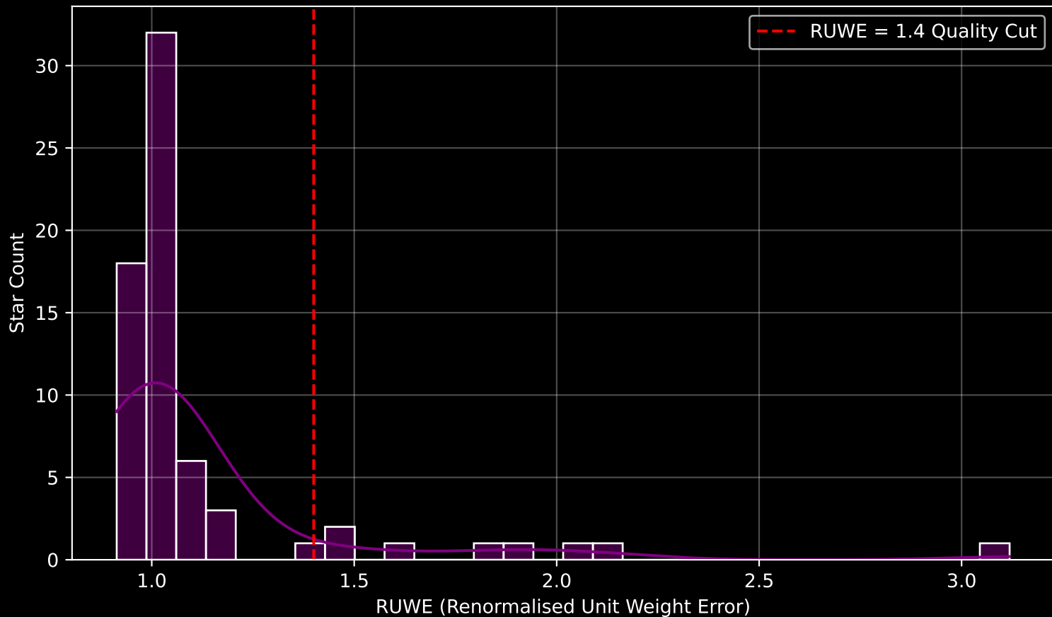
Gaia Cluster: [UPK_369] RUWE Distribution (n= 68)
