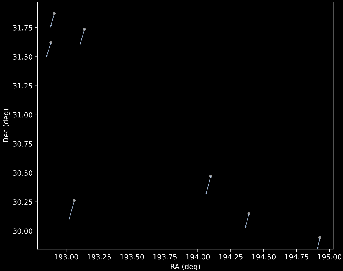
Gaia DR3 Cluster 1 Proper Motion Vectors (n=7)
