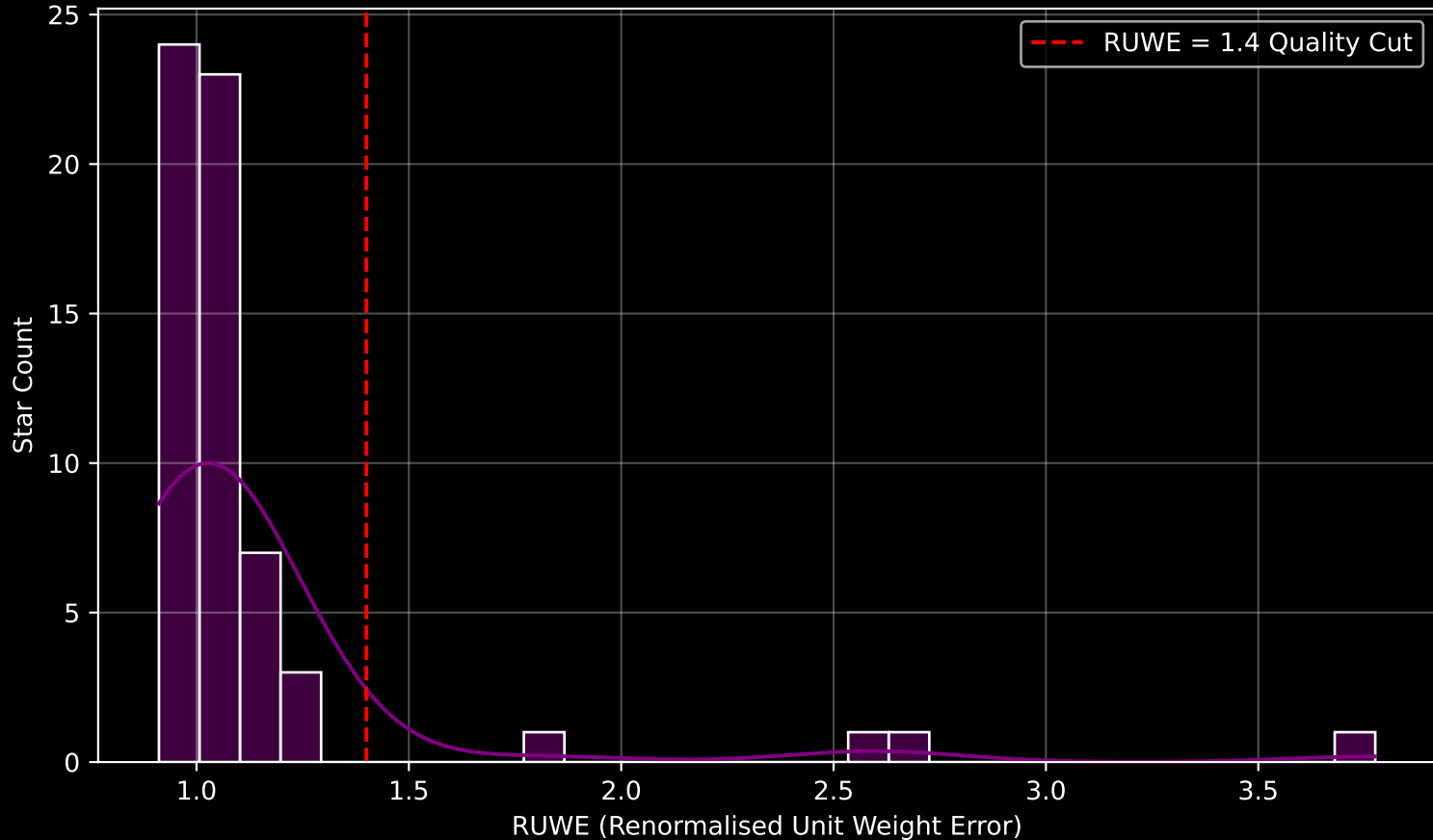
Gaia Cluster: [UPK_379] RUWE Distribution (n= 61)
