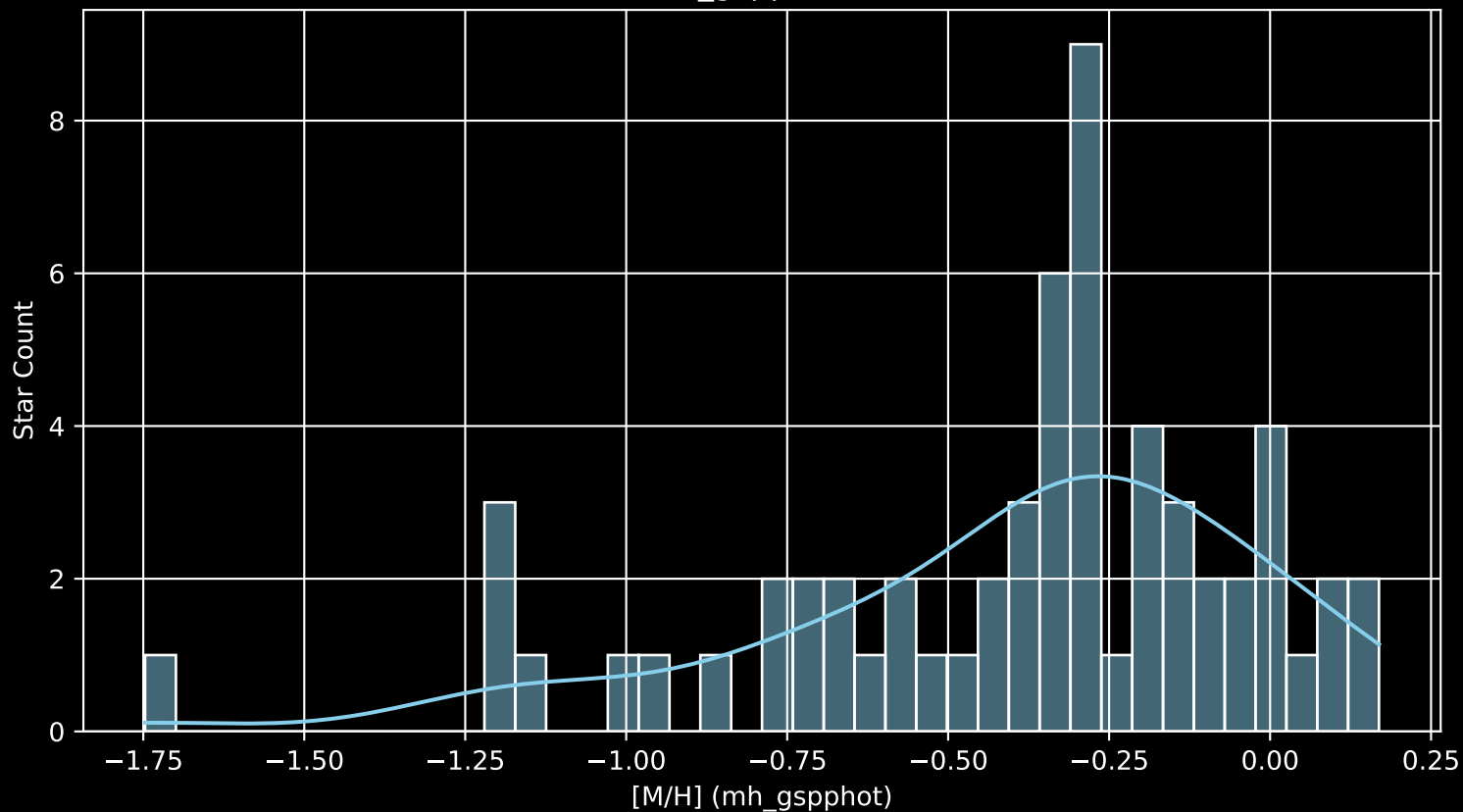
Gaia Cluster: [UPK_379 [M/H] (mh_gspphot) (n= 60)
