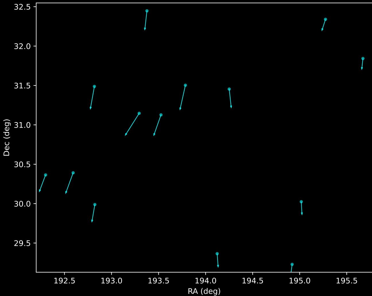
Gaia DR3 Noise Stream Proper Motion Vectors (n=14)
