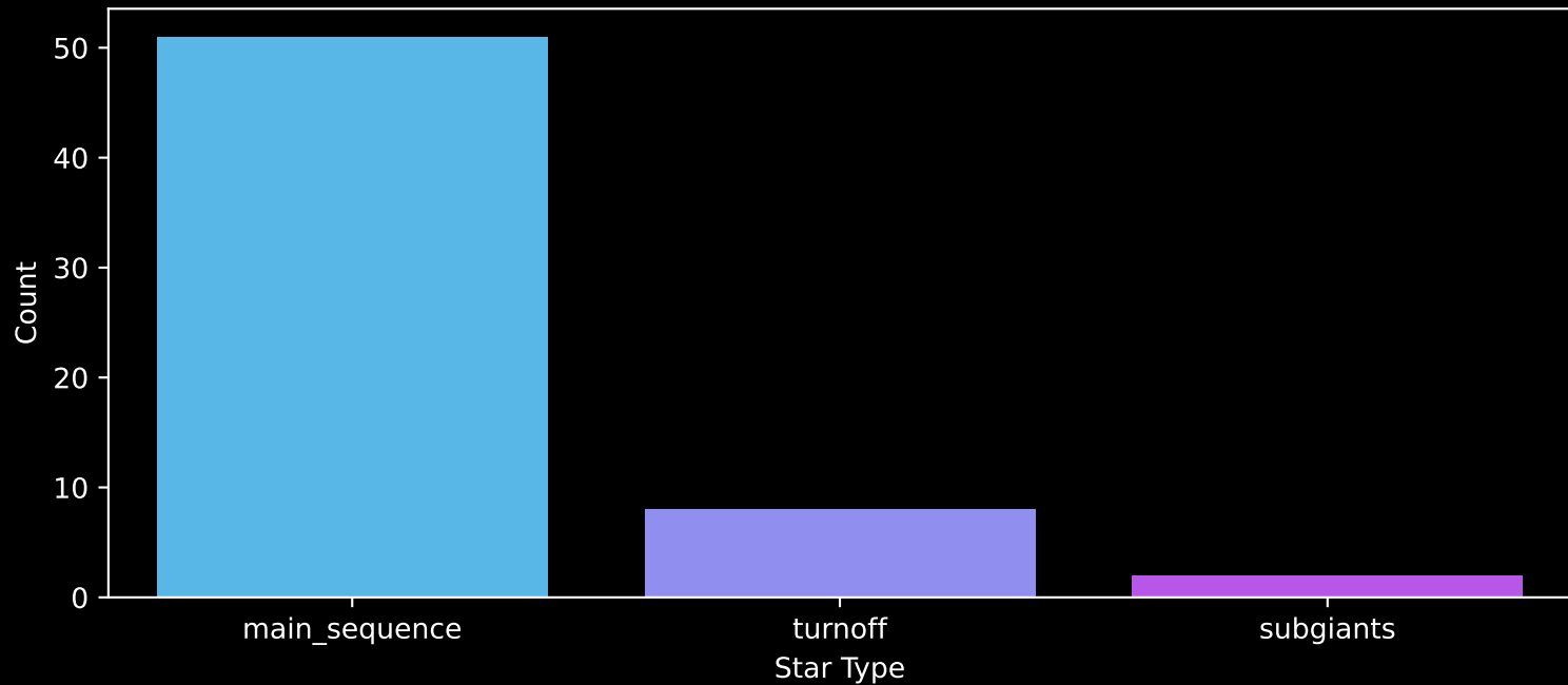
Gaia Cluster: [UPK_379] Count plot of Star Type
