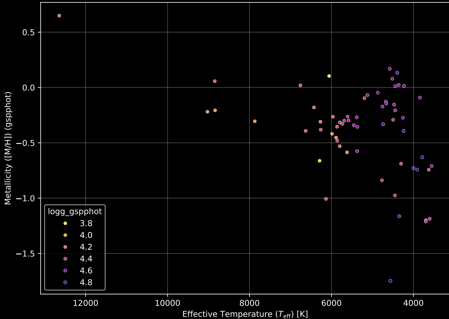
Gaia Cluster: [UPK_379] Stellar Population Parameters (n= 61)
