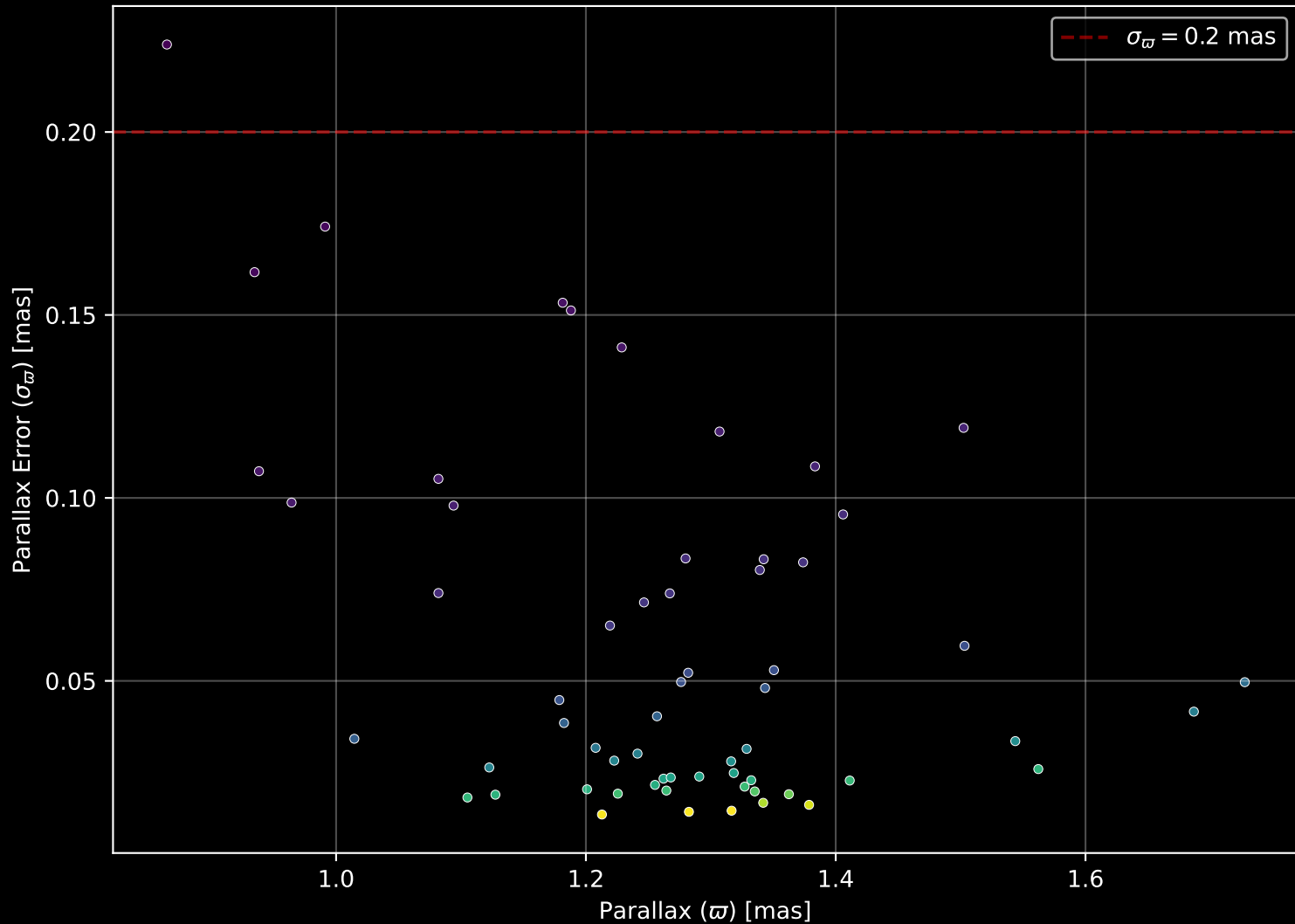
Gaia Cluster: [UPK_379] Parallax Quality (n= 61)
