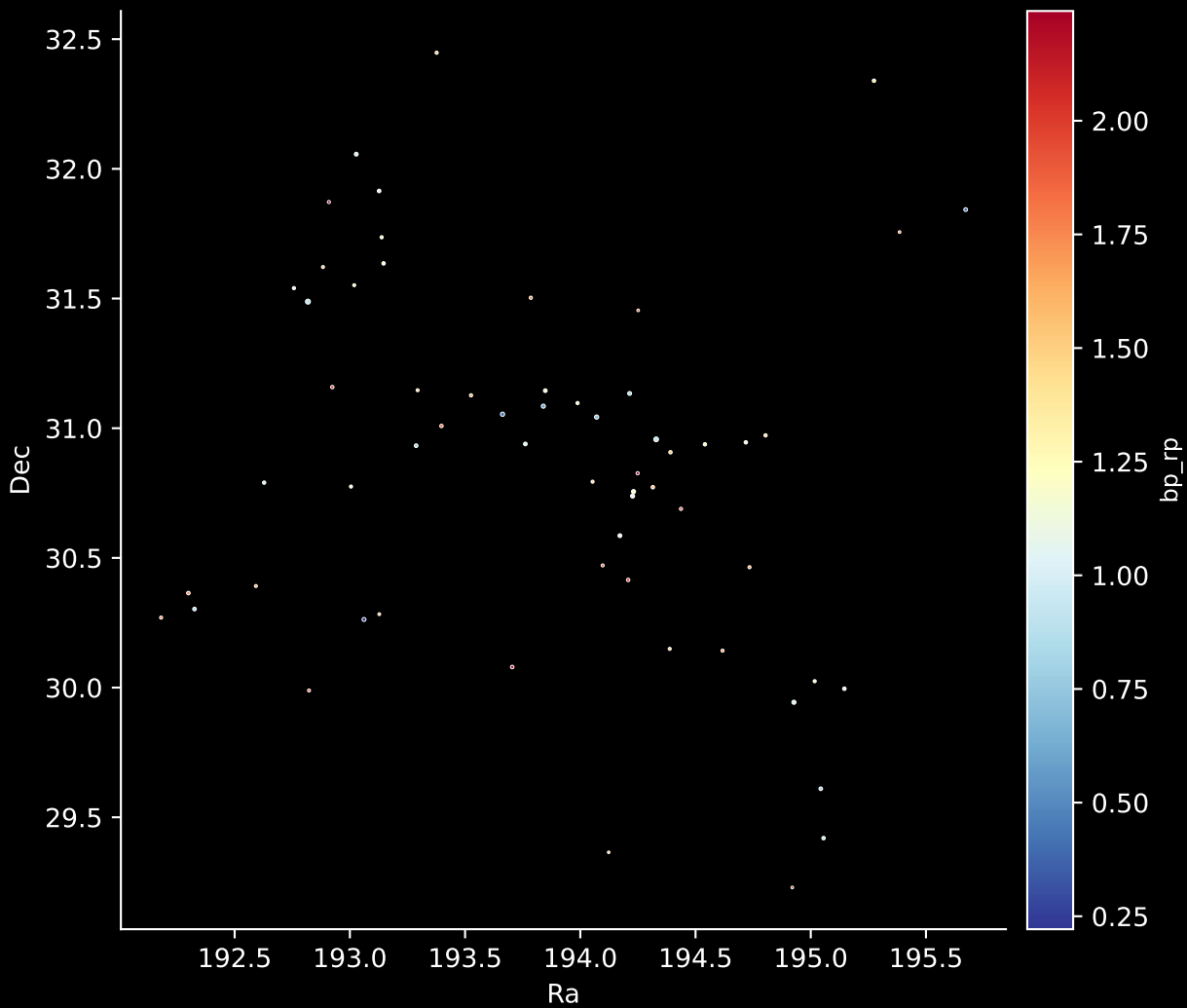
Gaia Cluster: [UPK_379] Stars: 61
