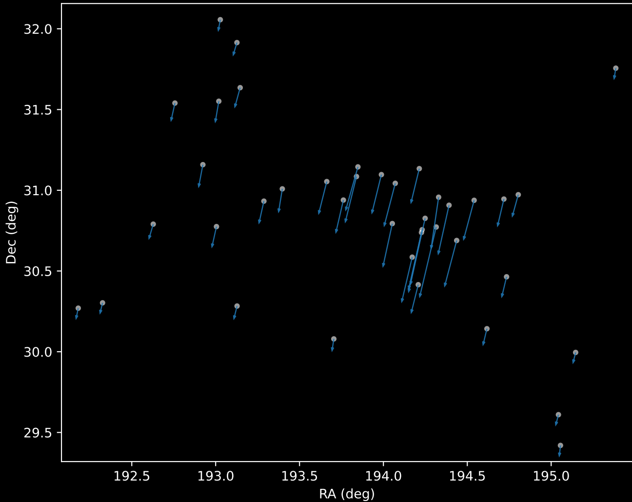
Gaia DR3 Cluster 0 Proper Motion Vectors (n=40)
