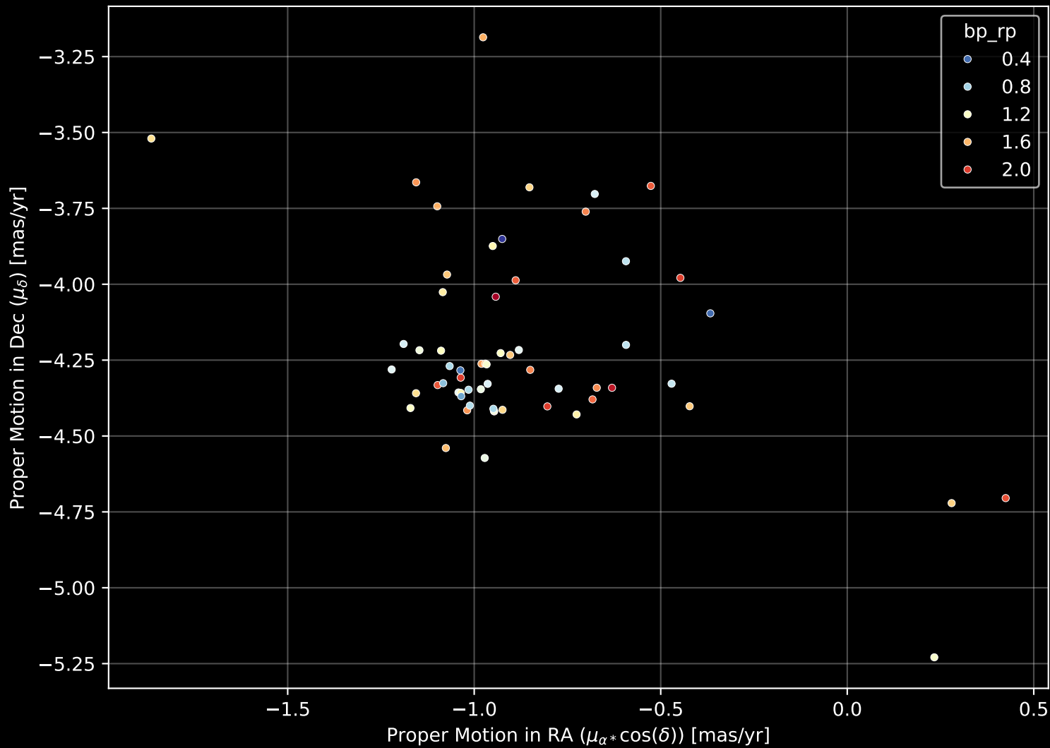
Gaia Cluster: [UPK_379] Proper Motion Diagram (n= 61)
