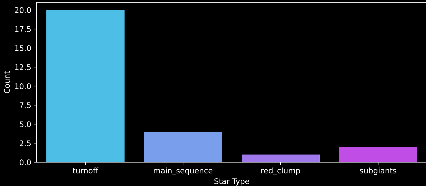
Gaia Cluster: [UPK_38] Count plot of Star Type
