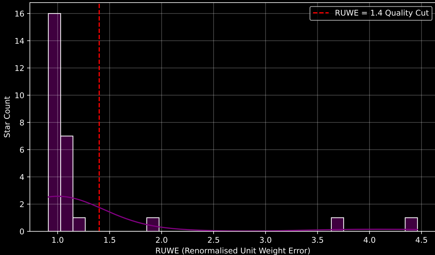
Gaia Cluster: [UPK_38] RUWE Distribution (n= 27)
