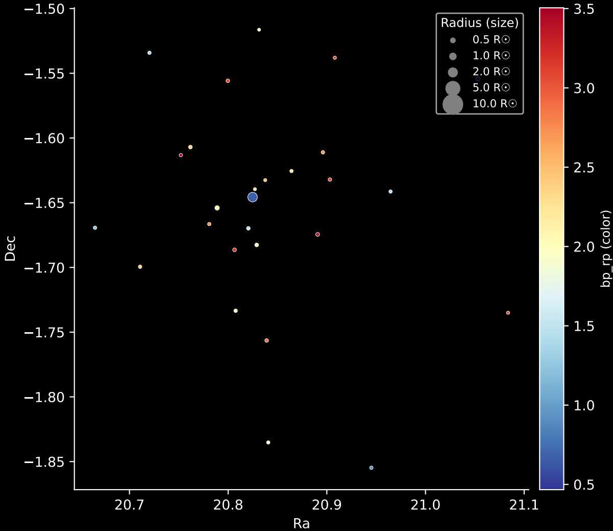
Gaia Cluster: [UPK_38] Stars: 27
