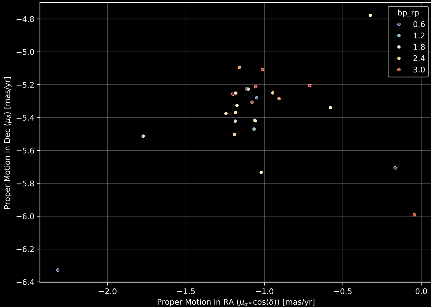
Gaia Cluster: [UPK_38] Proper Motion Diagram (n= 27)
