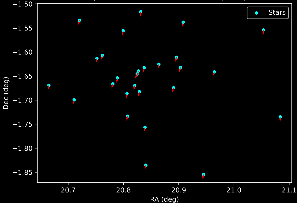
Gaia Cluster: [UPK_38] Proper Motion Vectors for Gaia Star Field (n= 27)
