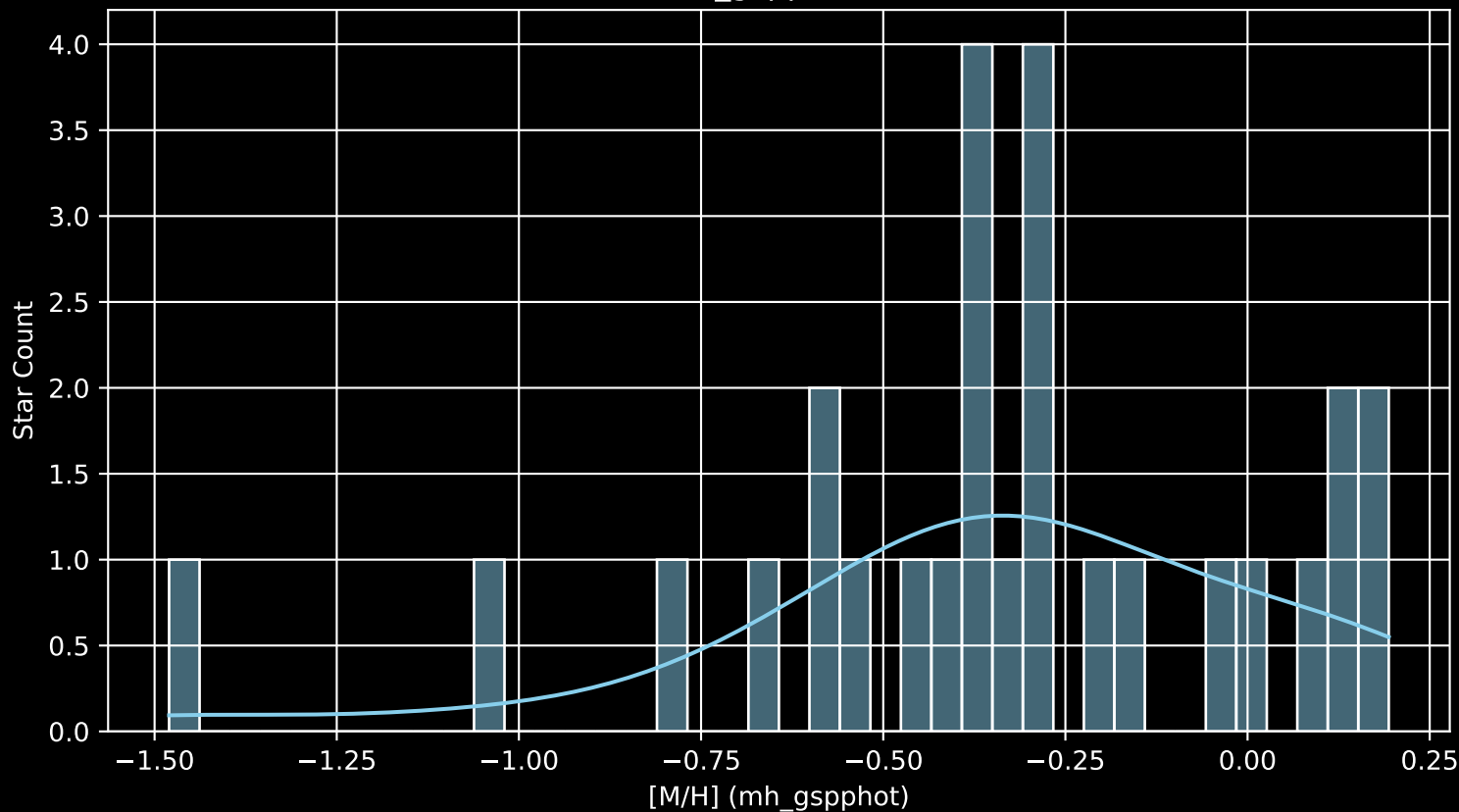
Gaia Cluster: [UPK_38 [M/H] (mh_gspphot) (n= 27)
