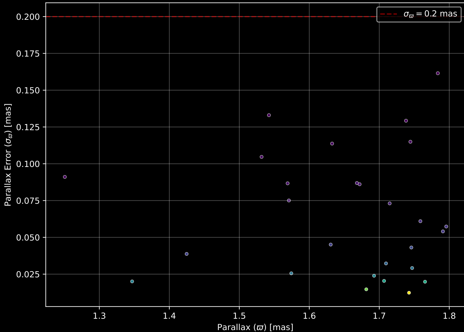
Gaia Cluster: [UPK_38] Parallax Quality (n= 27)
