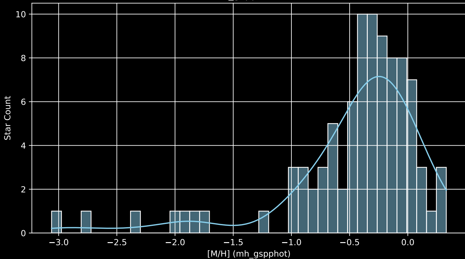
Gaia Cluster: [UPK_381 [M/H] (mh_gspphot) (n= 91)
