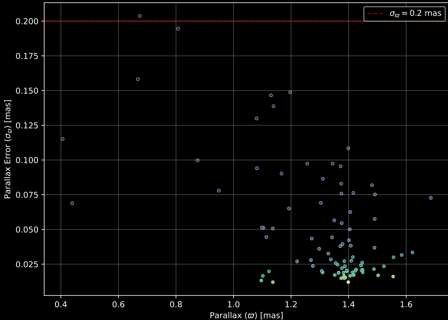
Gaia Cluster: [UPK_381] Parallax Quality (n= 91)
