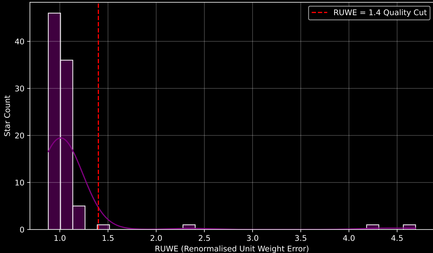
Gaia Cluster: [UPK_381] RUWE Distribution (n= 91)
