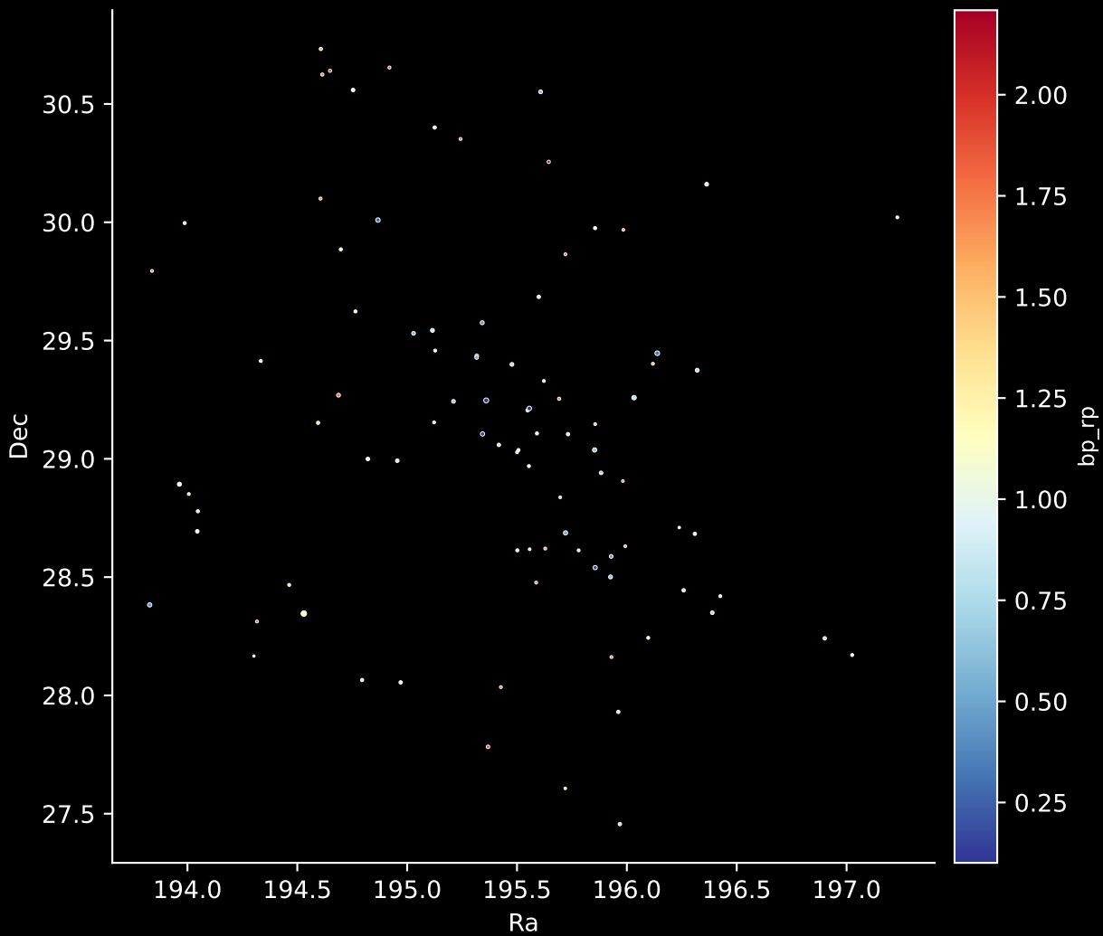
Gaia Cluster: [UPK_381] Stars: 91
