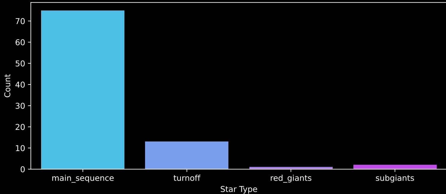
Gaia Cluster: [UPK_381] Count plot of Star Type
