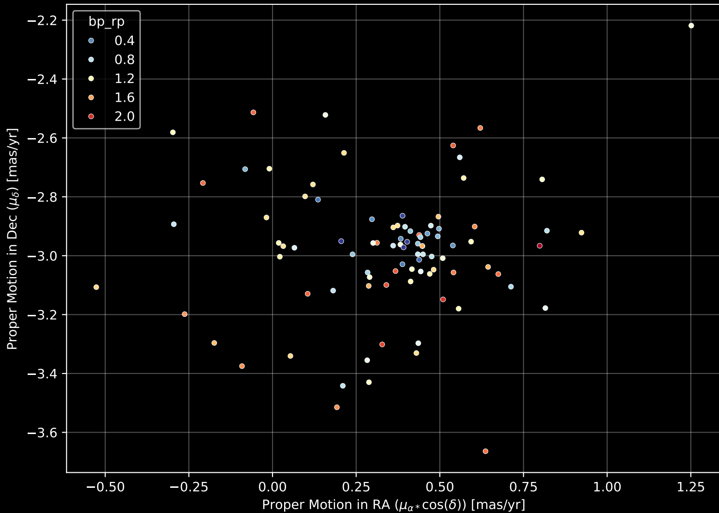
Gaia Cluster: [UPK_381] Proper Motion Diagram (n= 91)
