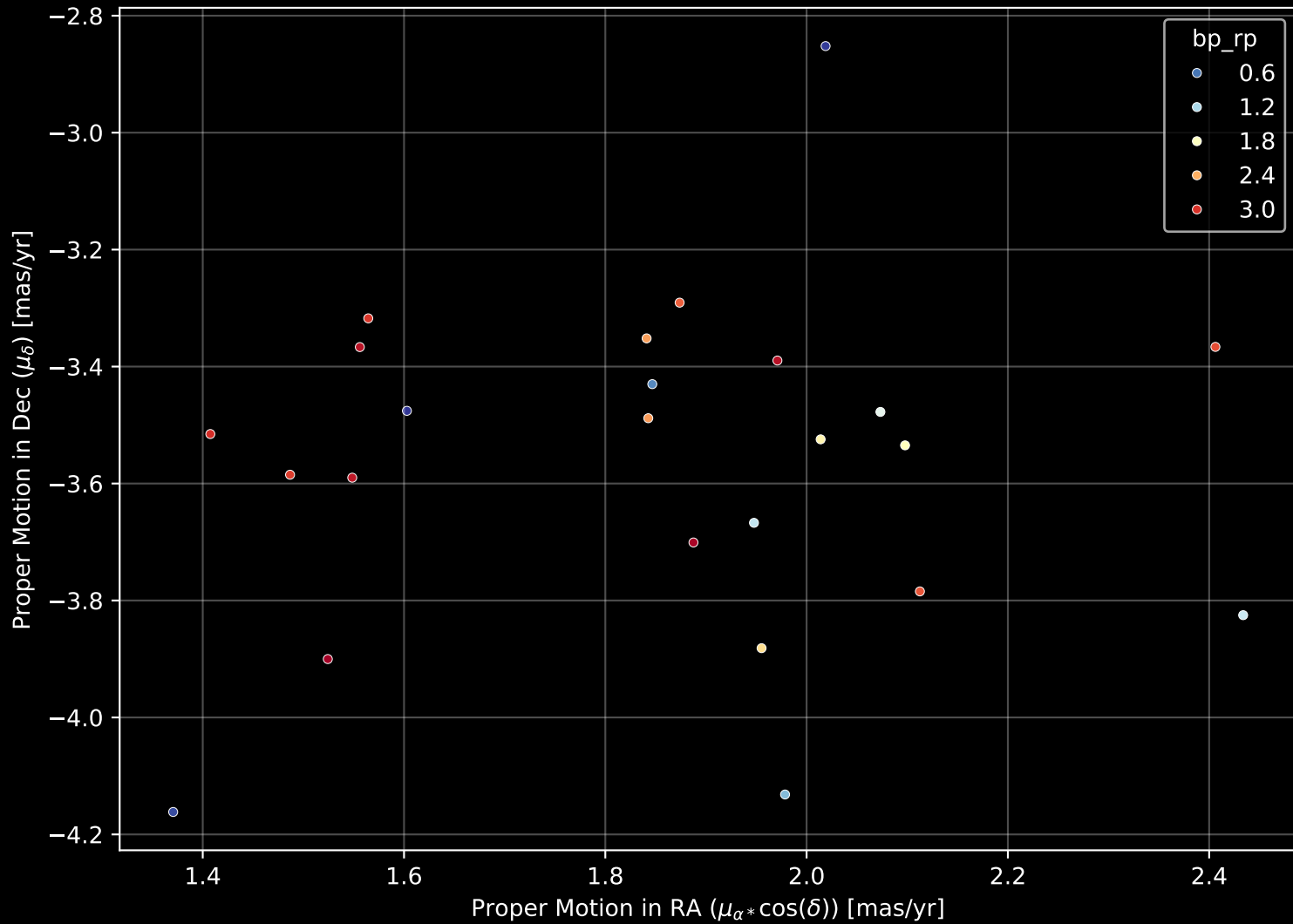
Gaia Cluster: [UPK_385] Proper Motion Diagram (n= 24)
