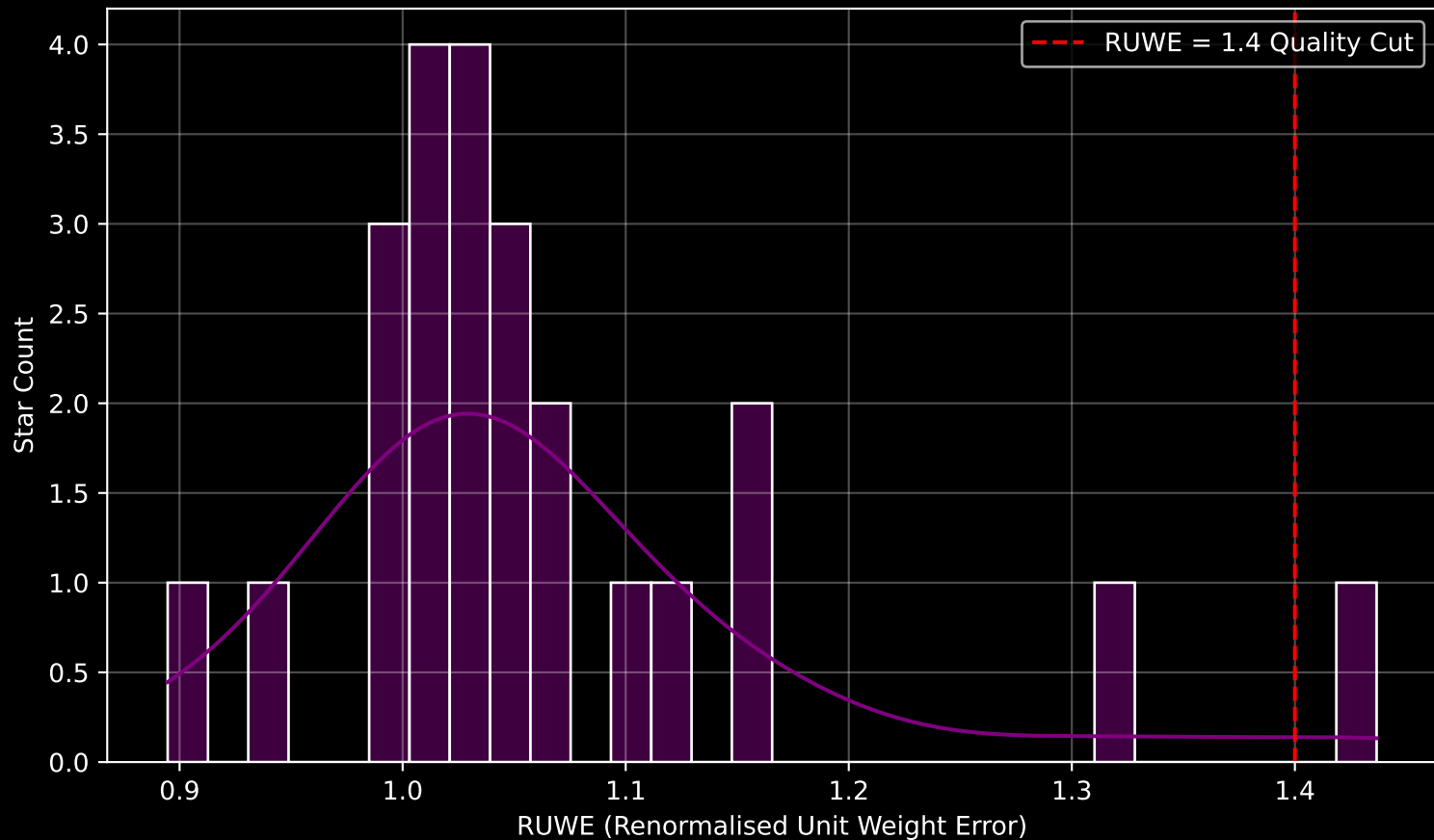
Gaia Cluster: [UPK_385] RUWE Distribution (n= 24)
