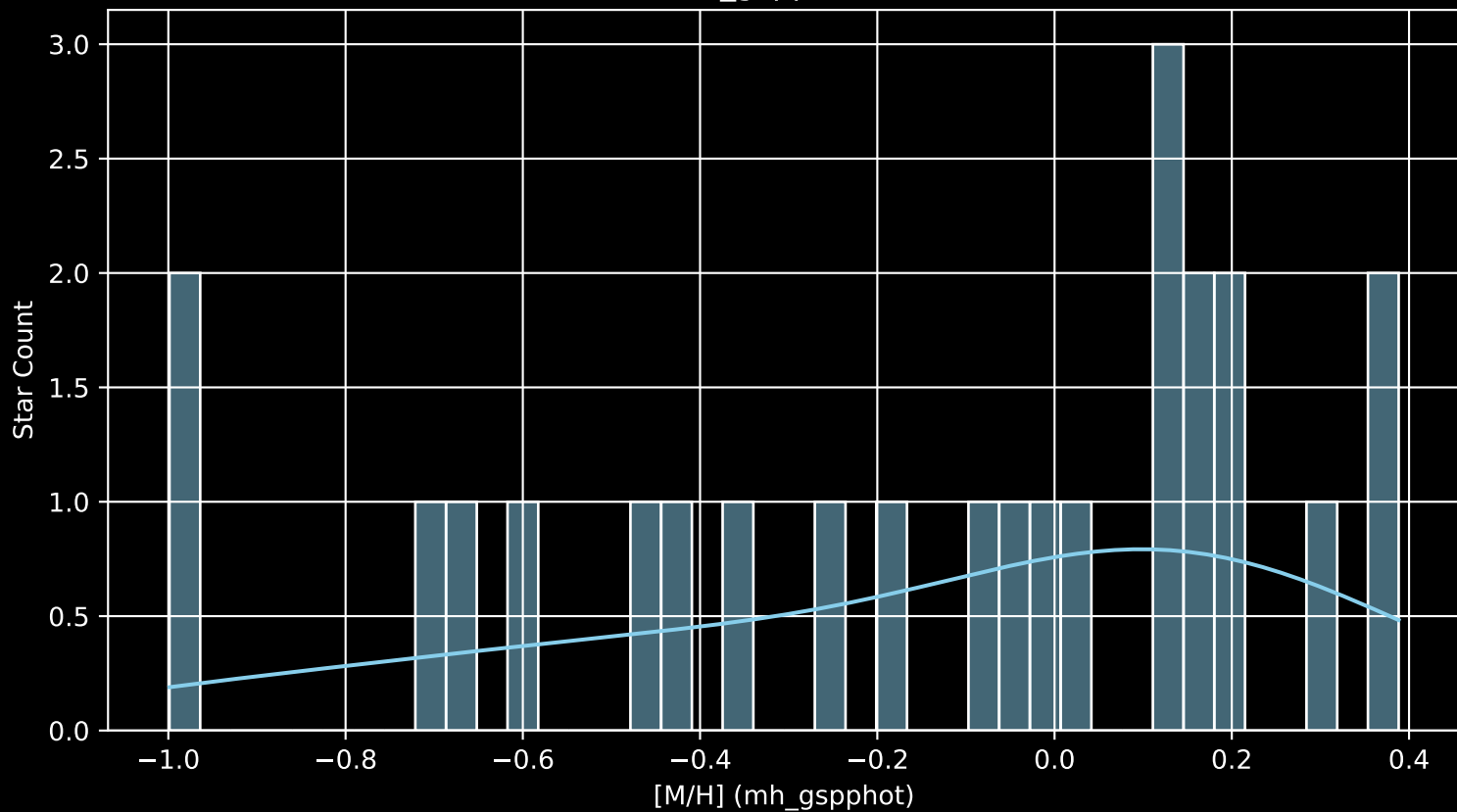
Gaia Cluster: [UPK_385 [M/H] (mh_gspphot) (n= 24)
