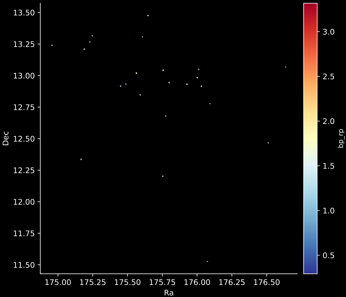
Gaia Cluster: [UPK_385] Stars: 24
