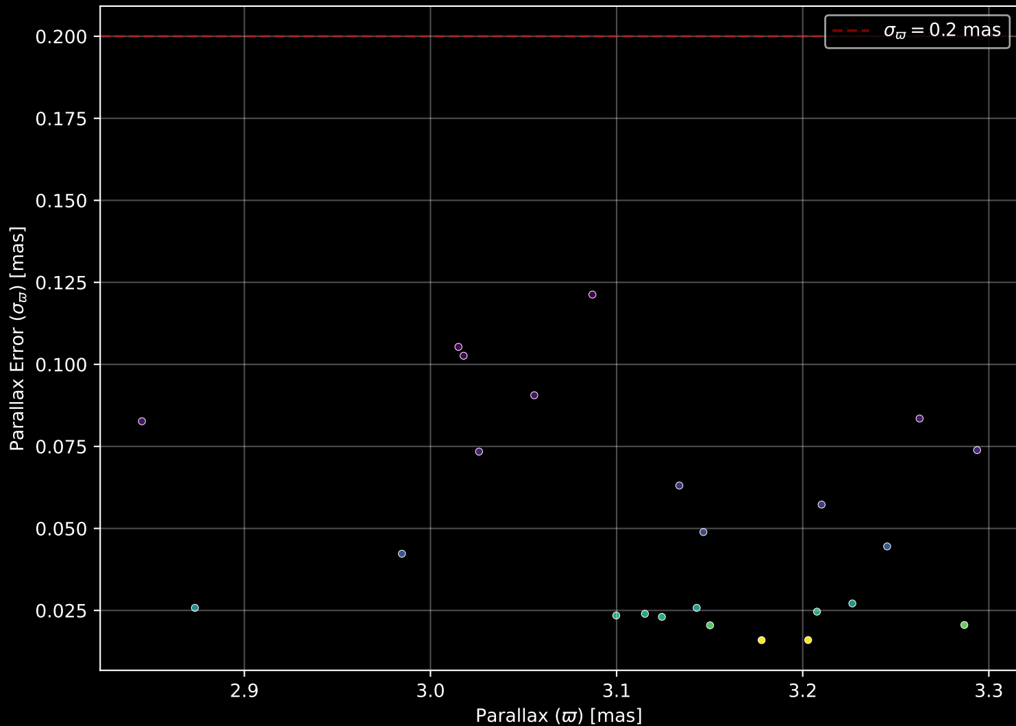
Gaia Cluster: [UPK_385] Parallax Quality (n= 24)
