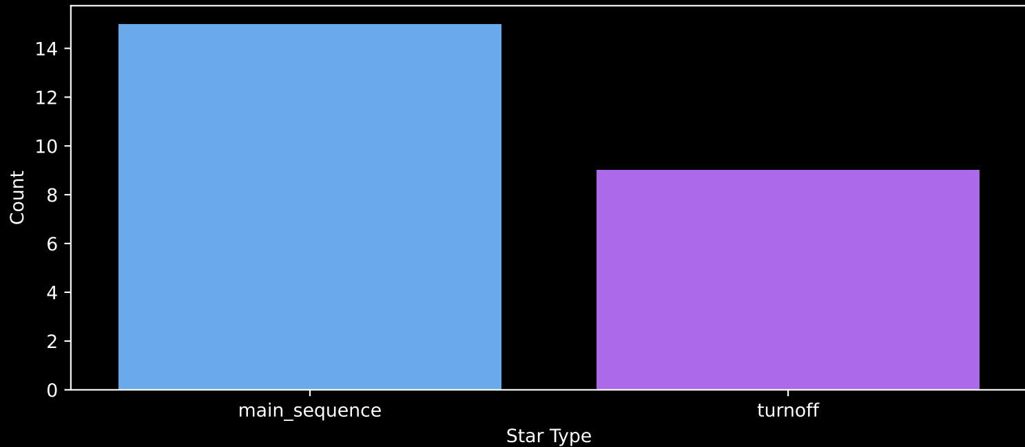
Gaia Cluster: [UPK_385] Count plot of Star Type
