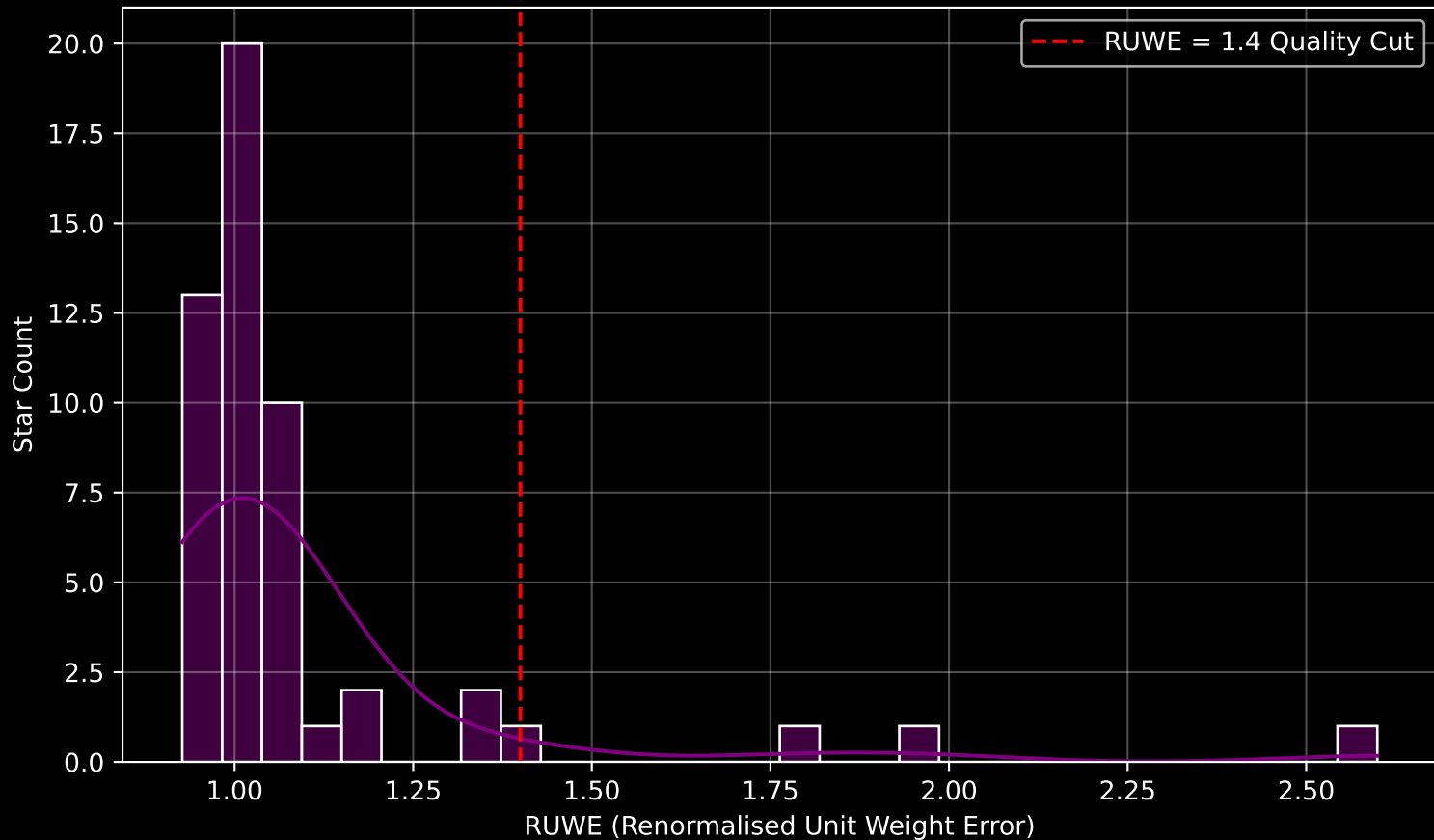
Gaia Cluster: [UPK_394] RUWE Distribution (n= 52)
