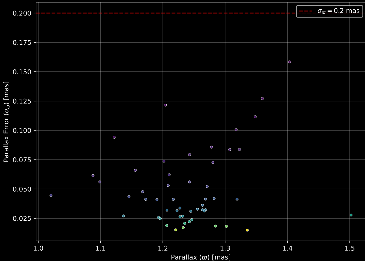
Gaia Cluster: [UPK_394] Parallax Quality (n= 52)
