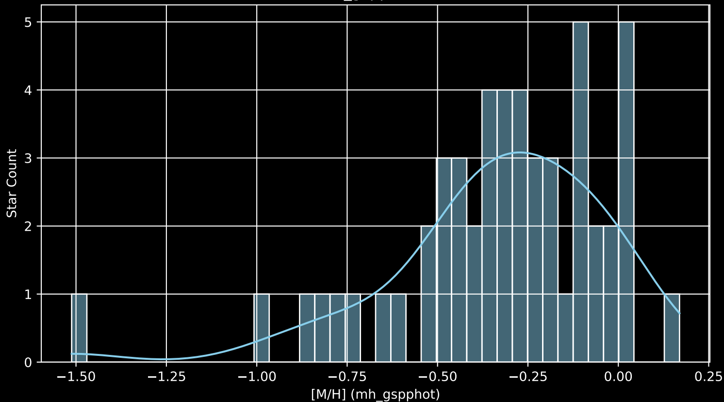
Gaia Cluster: [UPK_394 [M/H] (mh_gspphot) (n= 52)
