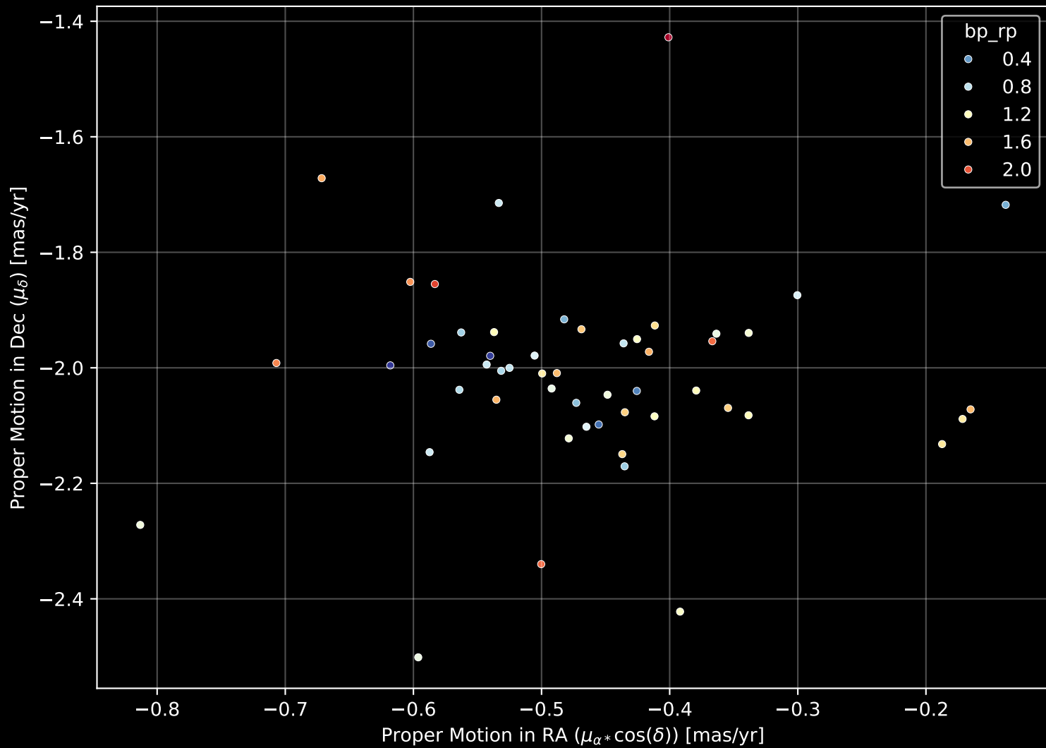
Gaia Cluster: [UPK_394] Proper Motion Diagram (n= 52)
