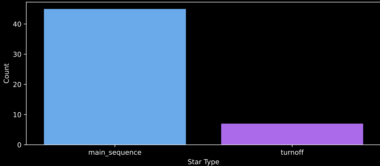
Gaia Cluster: [UPK_394] Count plot of Star Type
