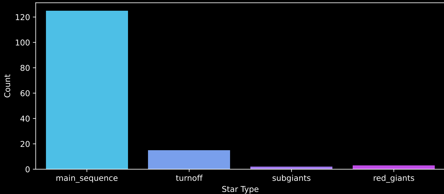
Gaia Cluster: [UPK_431] Count plot of Star Type
