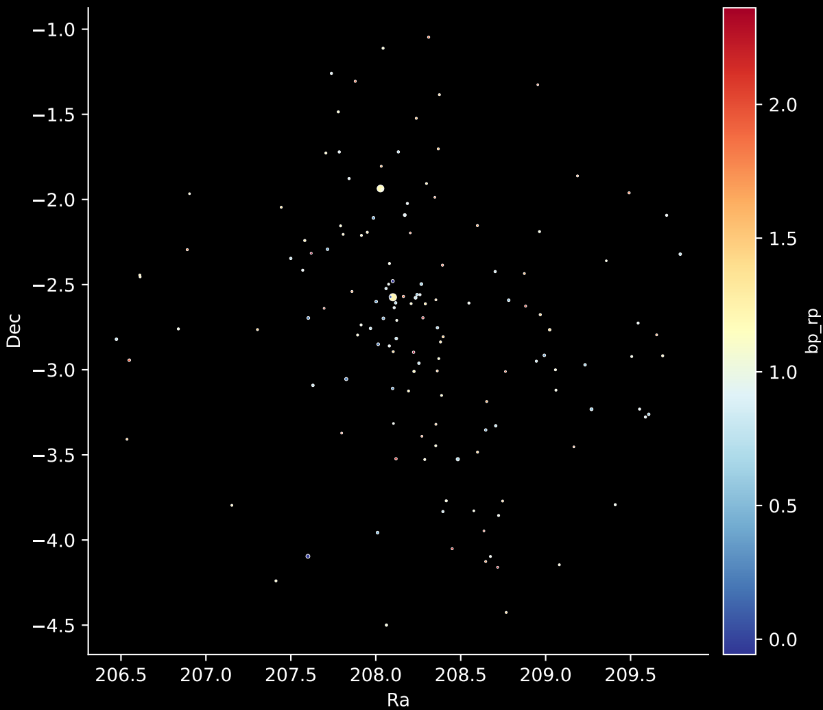
Gaia Cluster: [UPK_431] Stars: 145
