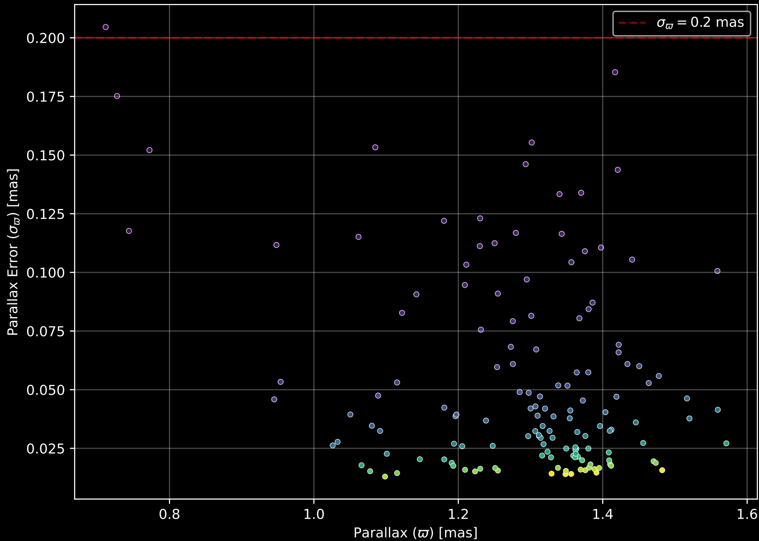
Gaia Cluster: [UPK_431] Parallax Quality (n= 145)
