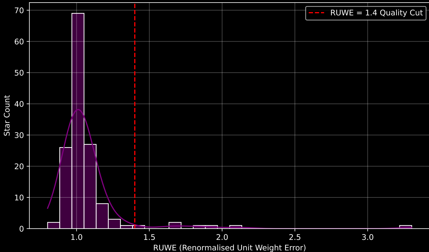
Gaia Cluster: [UPK_431] RUWE Distribution (n= 143)
