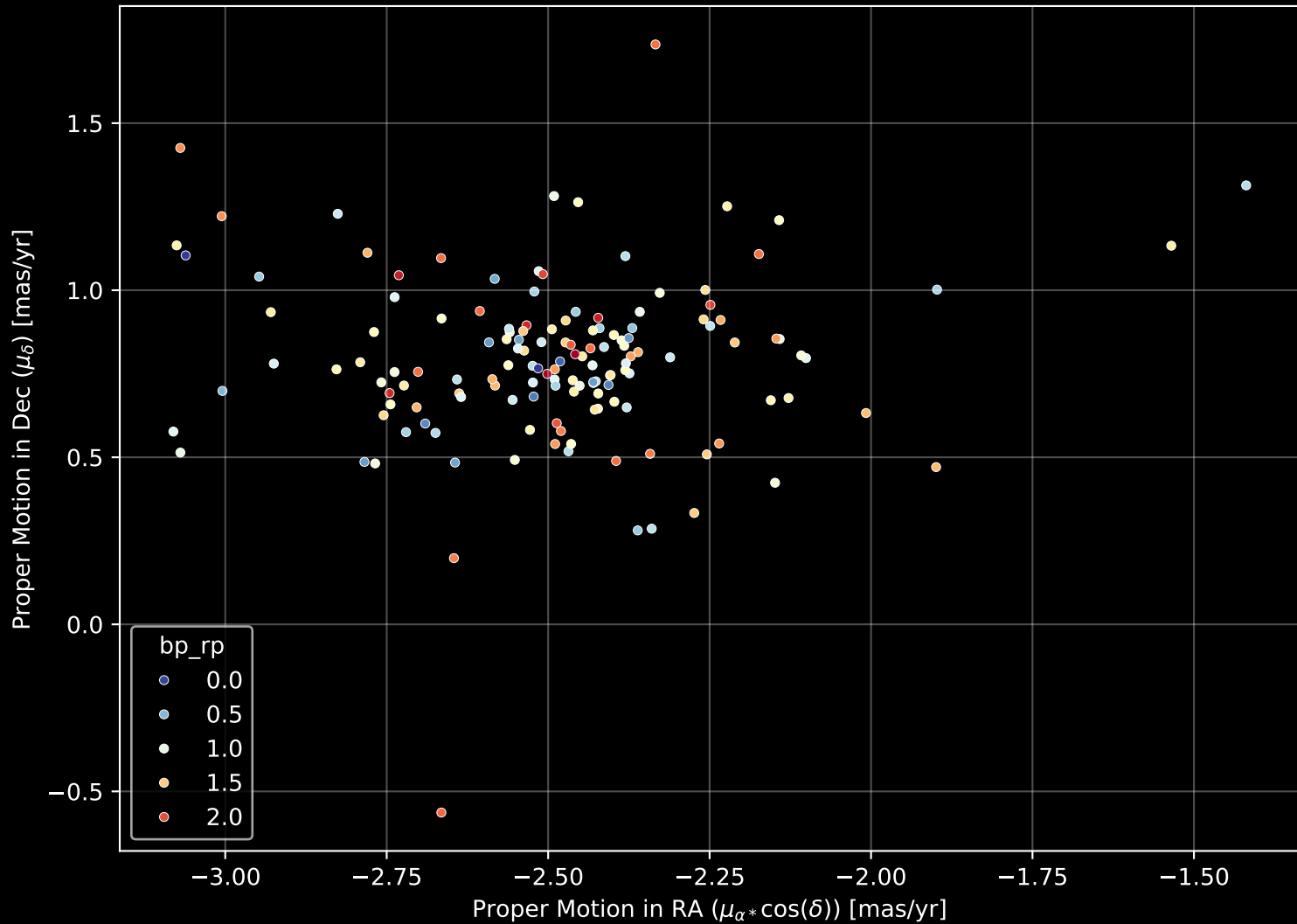
Gaia Cluster: [UPK_431] Proper Motion Diagram (n= 145)
