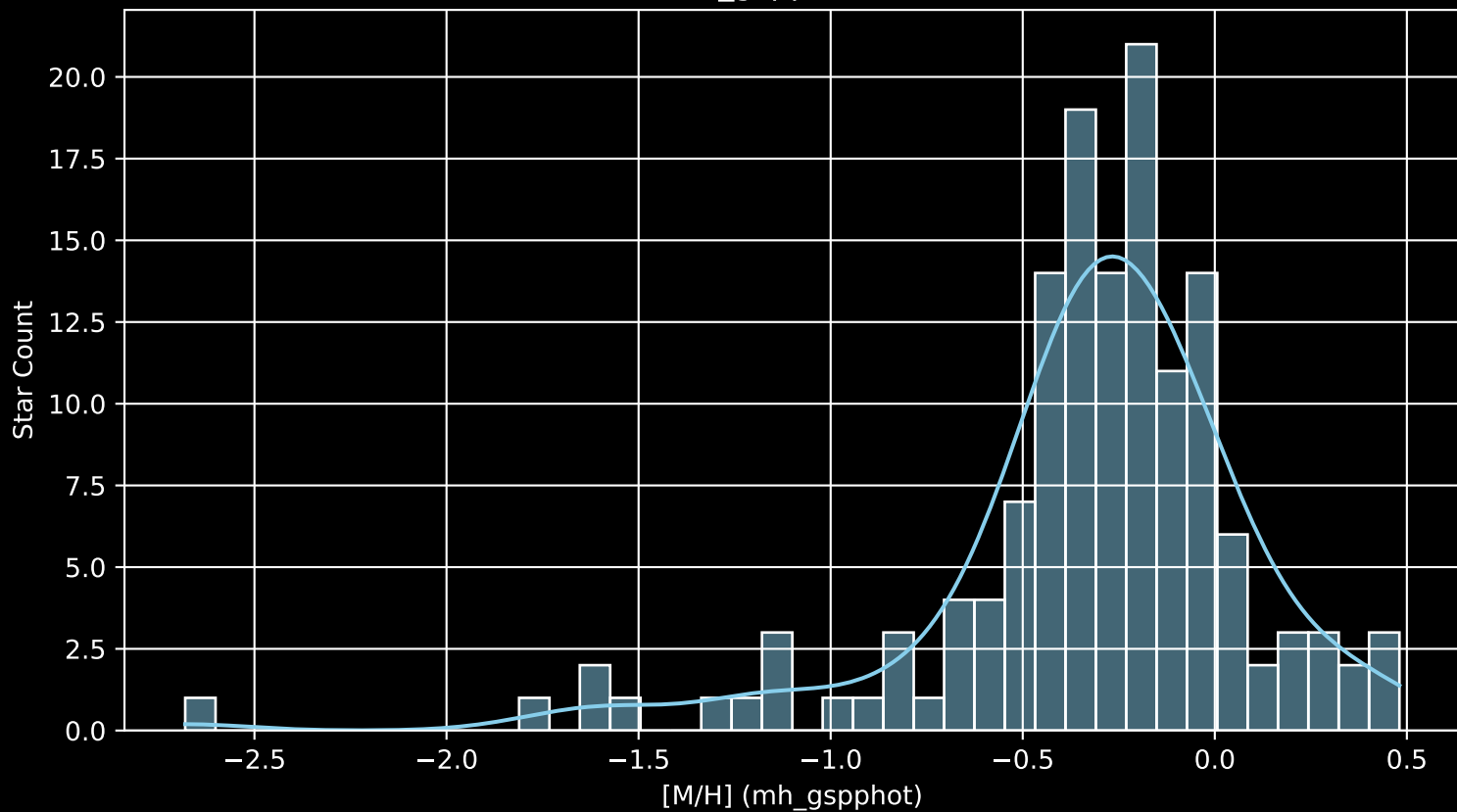
Gaia Cluster: [UPK_431 [M/H] (mh_gspphot) (n= 143)
