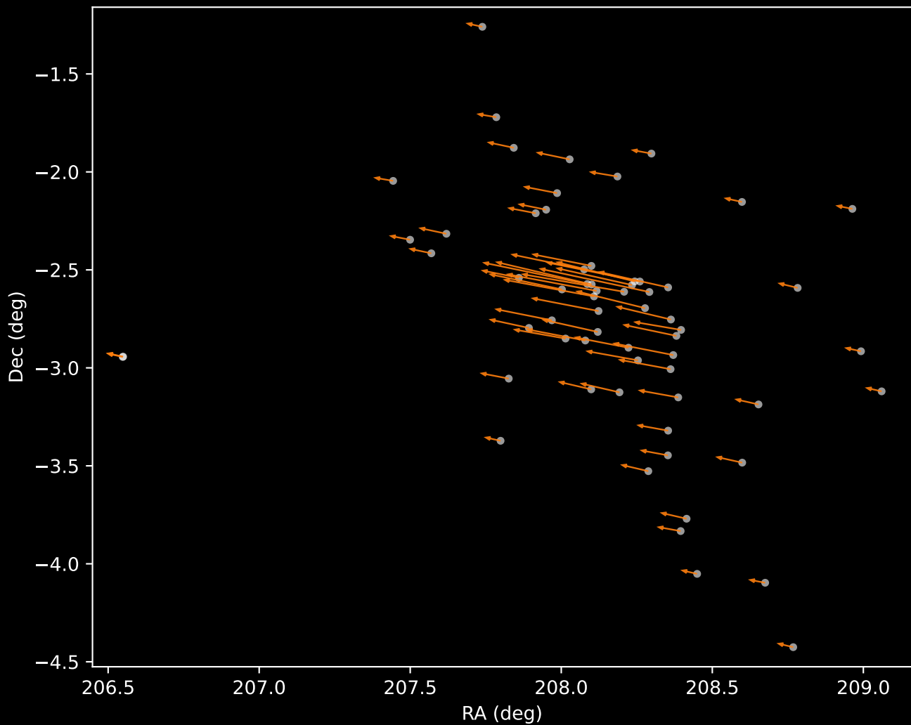
Gaia DR3 Cluster 2 Proper Motion Vectors (n=63)
