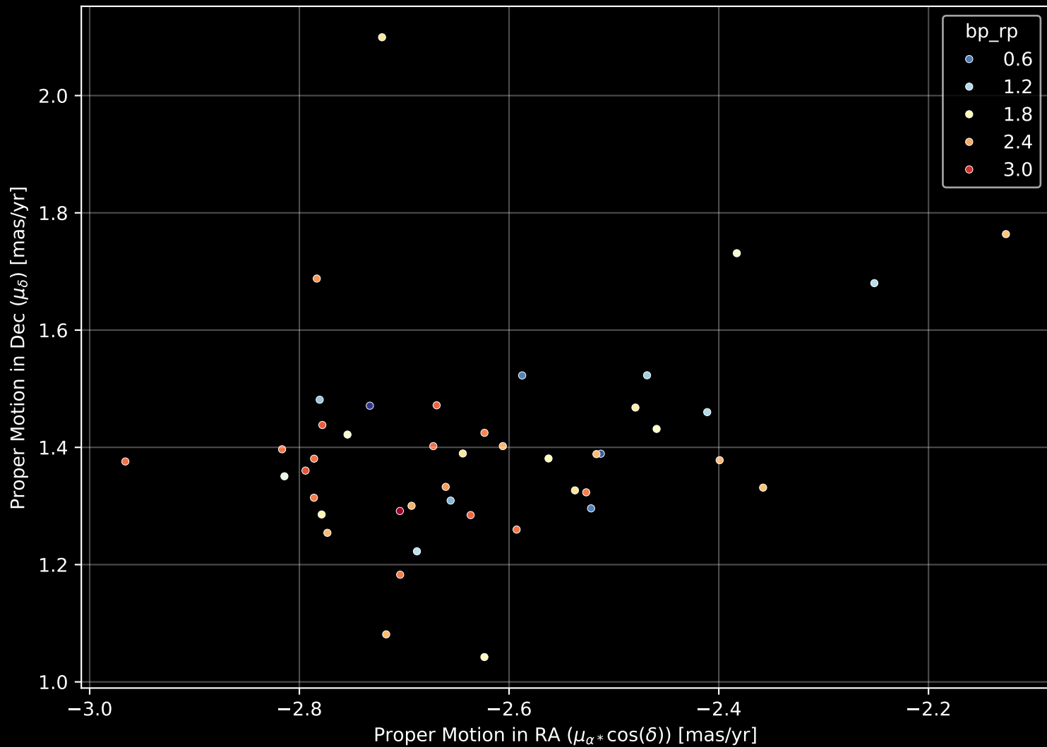
Gaia Cluster: [UPK_445] Proper Motion Diagram (n= 45)
