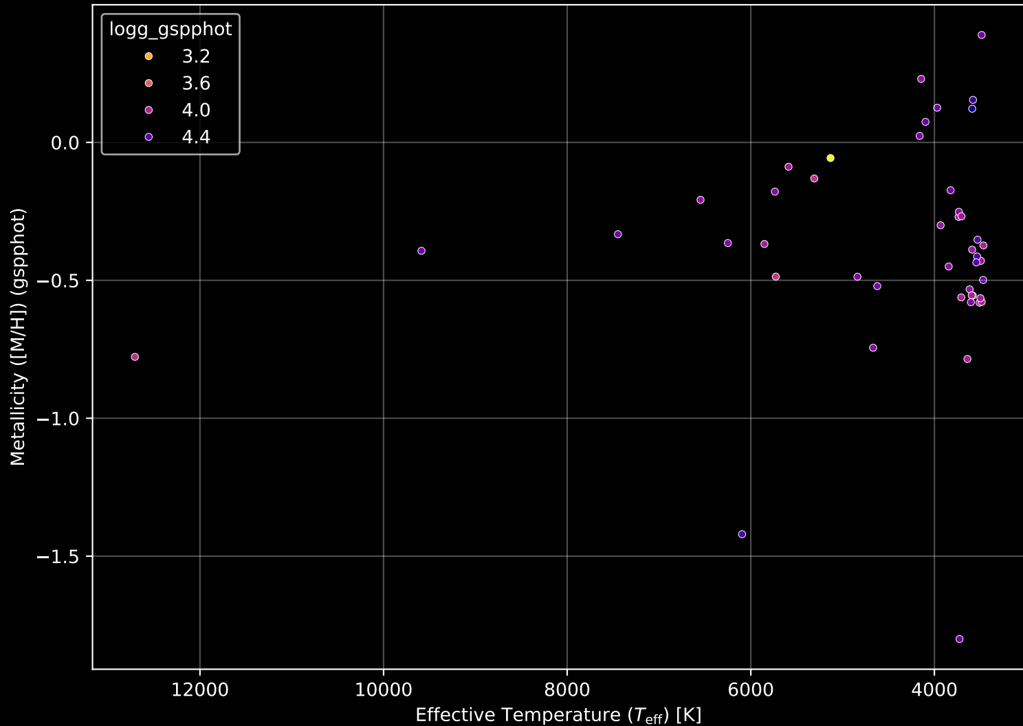
Gaia Cluster: [UPK_445] Stellar Population Parameters (n= 45)
