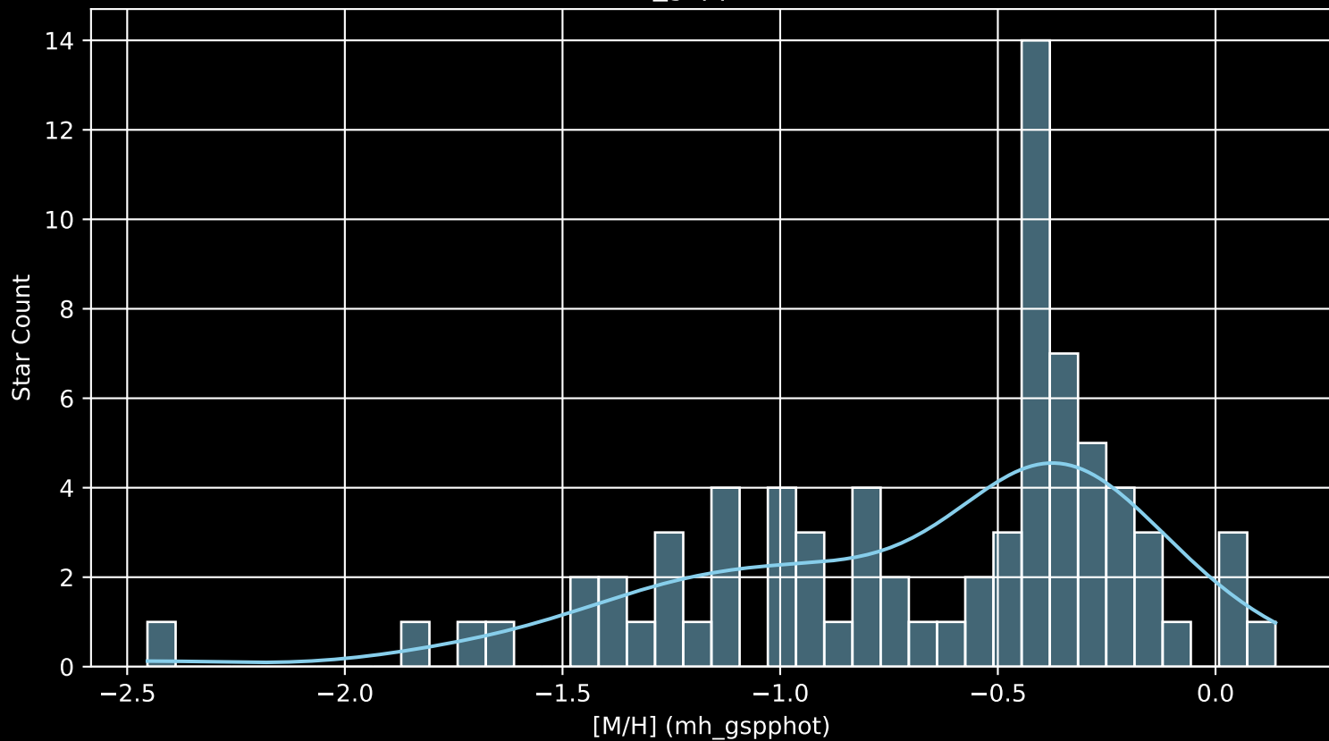
Gaia Cluster: [UPK_45 [M/H] (mh_gspphot) (n= 76)
