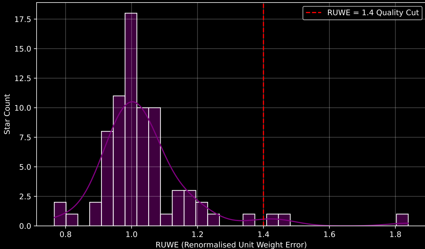
Gaia Cluster: [UPK_45] RUWE Distribution (n= 76)
