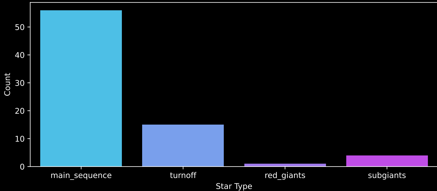
Gaia Cluster: [UPK_45] Count plot of Star Type
