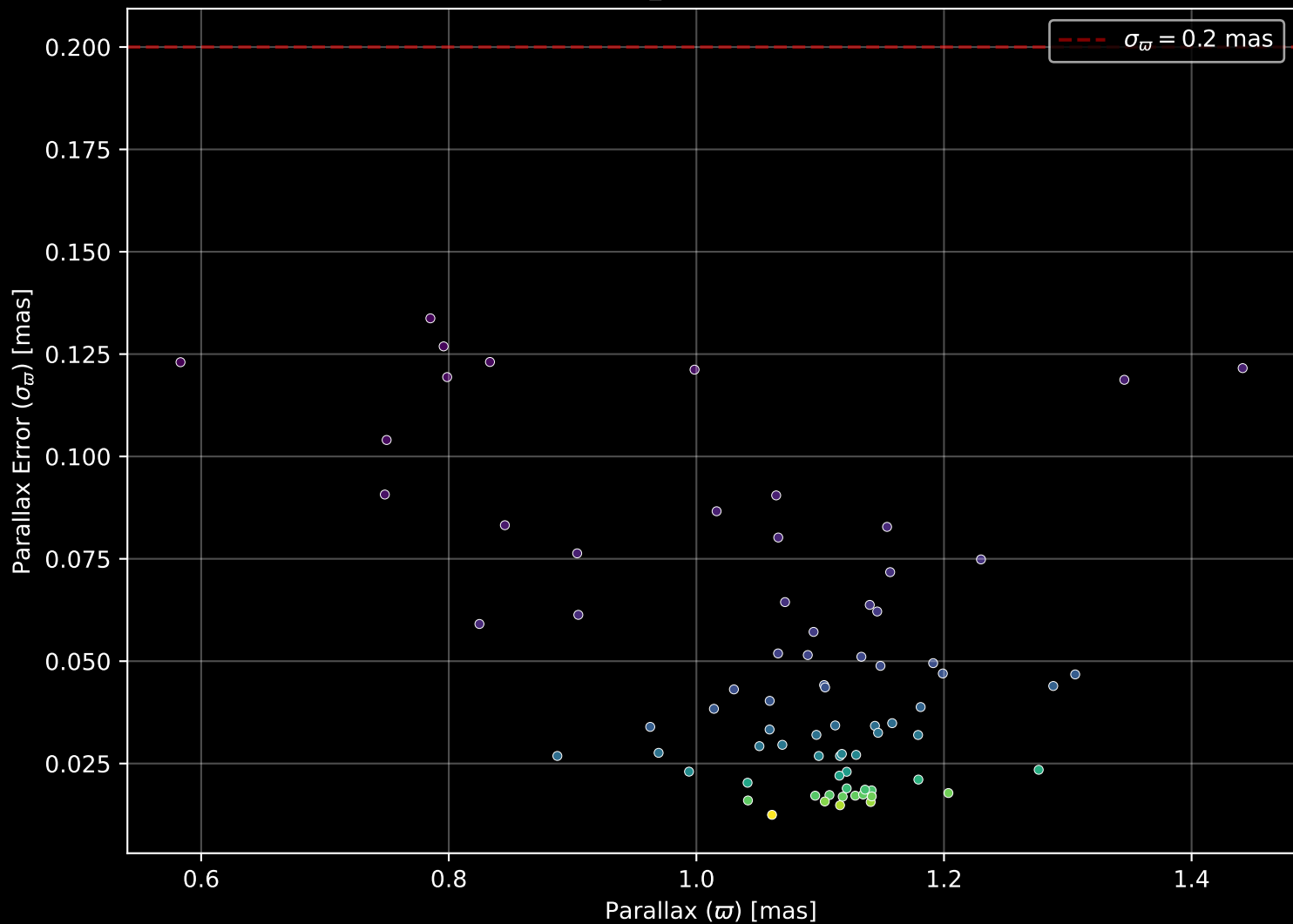
Gaia Cluster: [UPK_45] Parallax Quality (n= 76)
