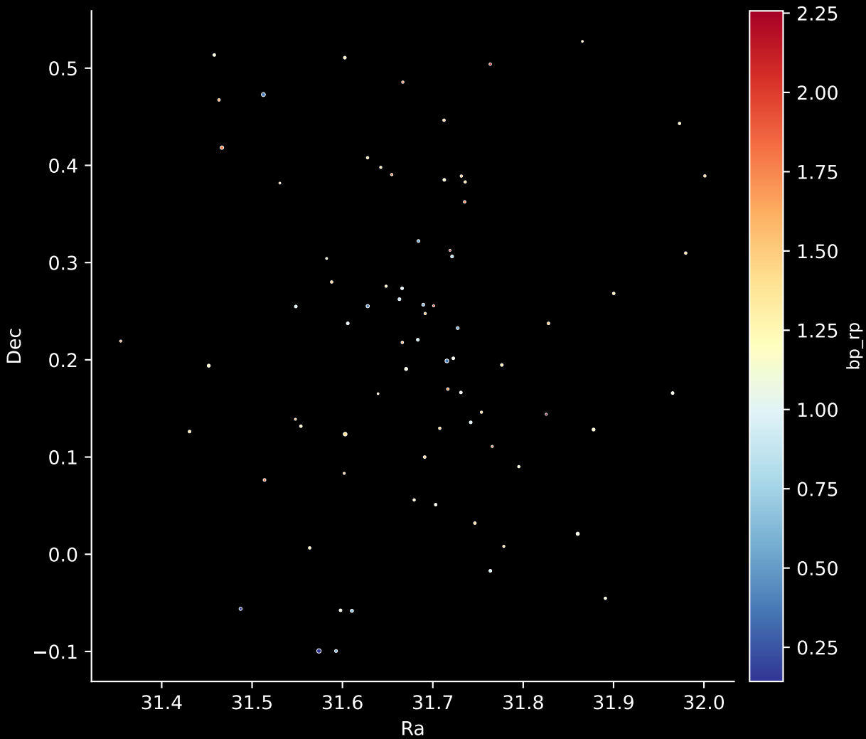
Gaia Cluster: [UPK_45] Stars: 76
