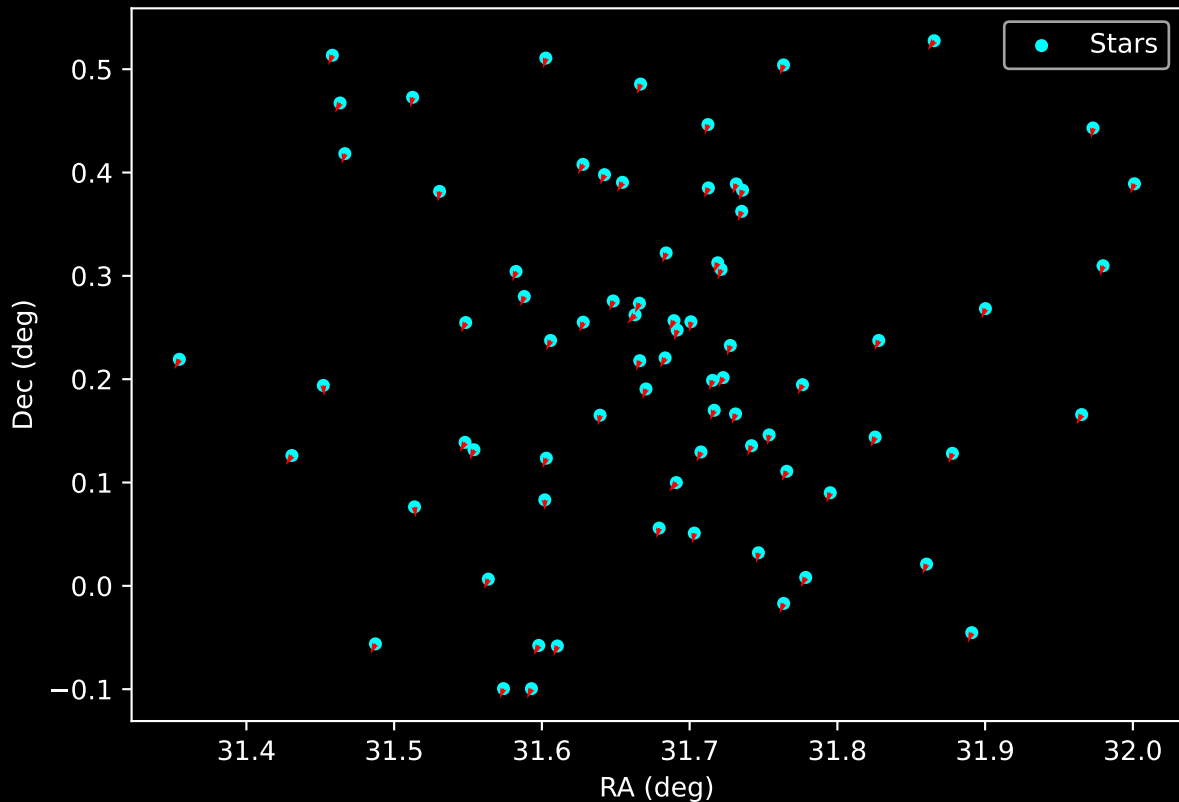
Gaia Cluster: [UPK_45] Proper Motion Vectors for Gaia Star Field (n= 76)
