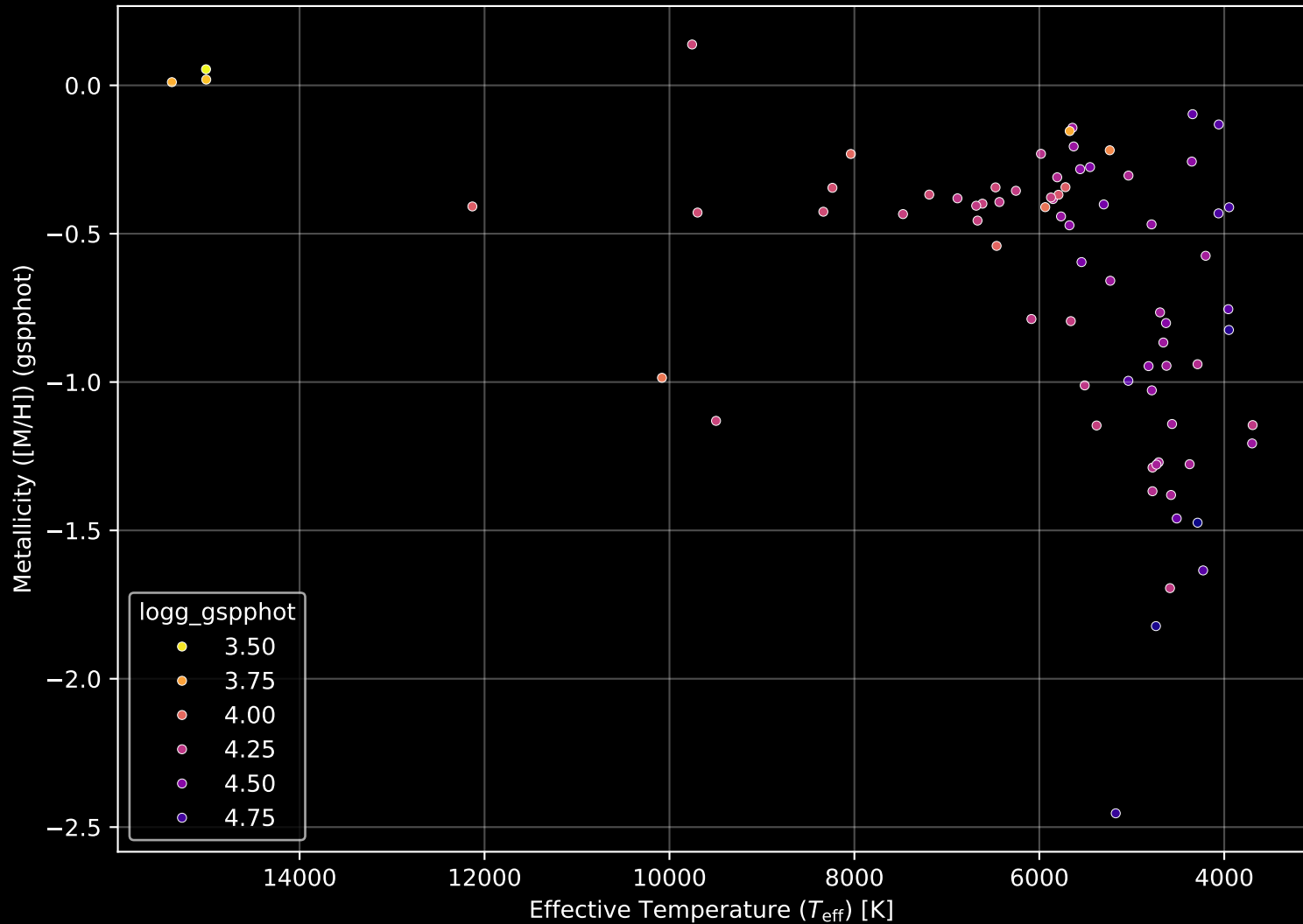
Gaia Cluster: [UPK_45] Stellar Population Parameters (n= 76)
