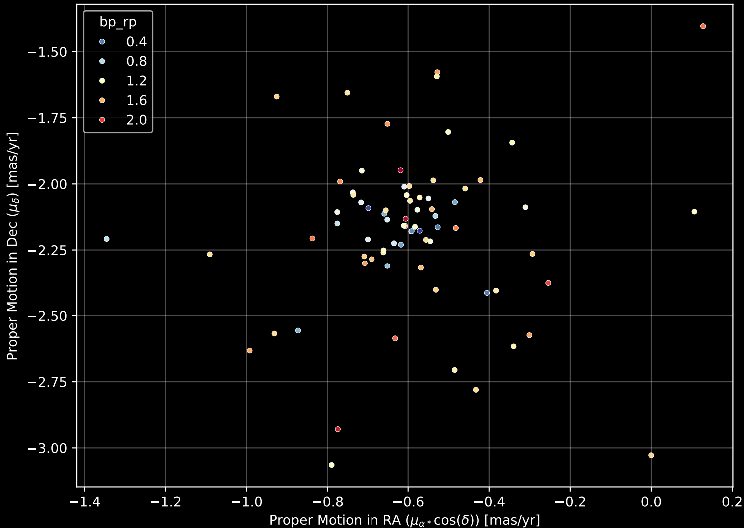
Gaia Cluster: [UPK_45] Proper Motion Diagram (n= 76)
