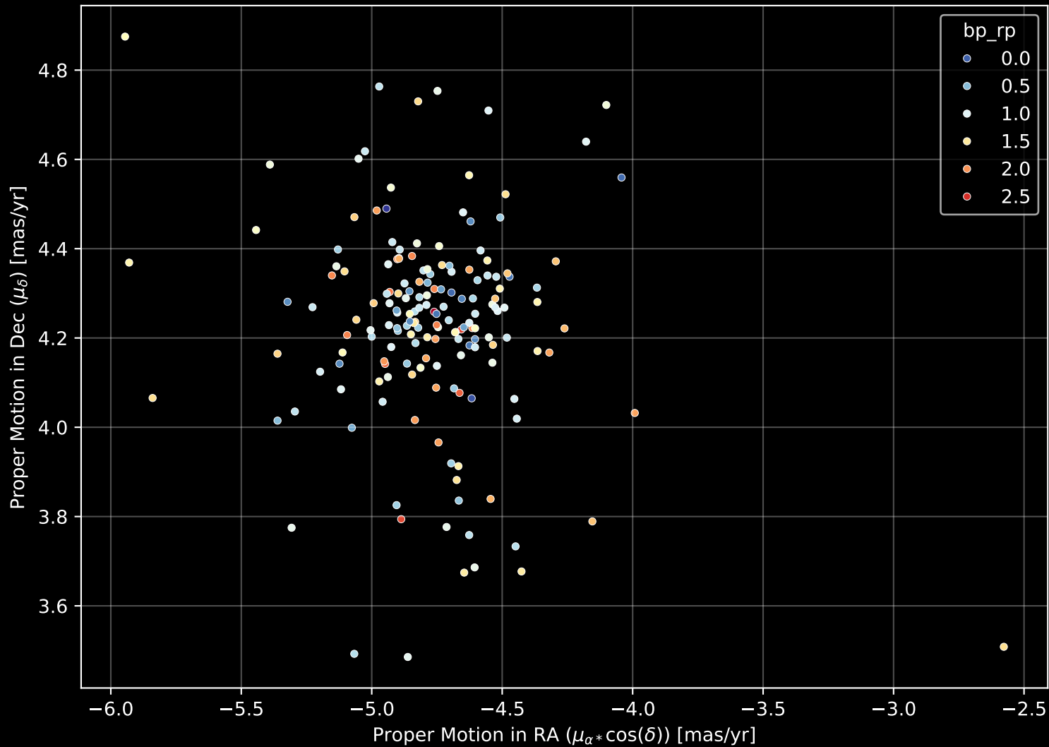
Gaia Cluster: [UPK_470] Proper Motion Diagram (n= 172)
