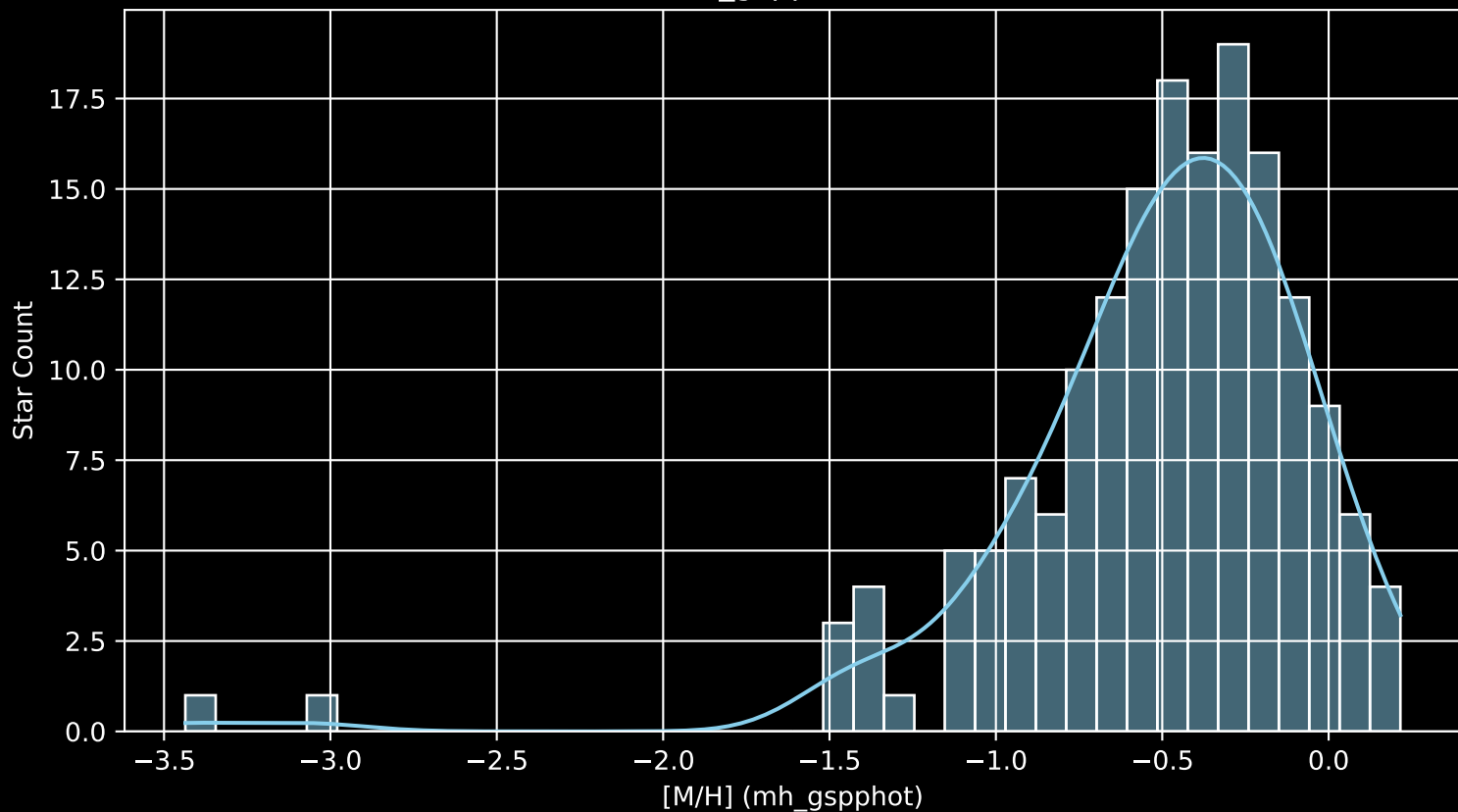
Gaia Cluster: [UPK_470 [M/H] (mh_gspphot) (n= 170)
