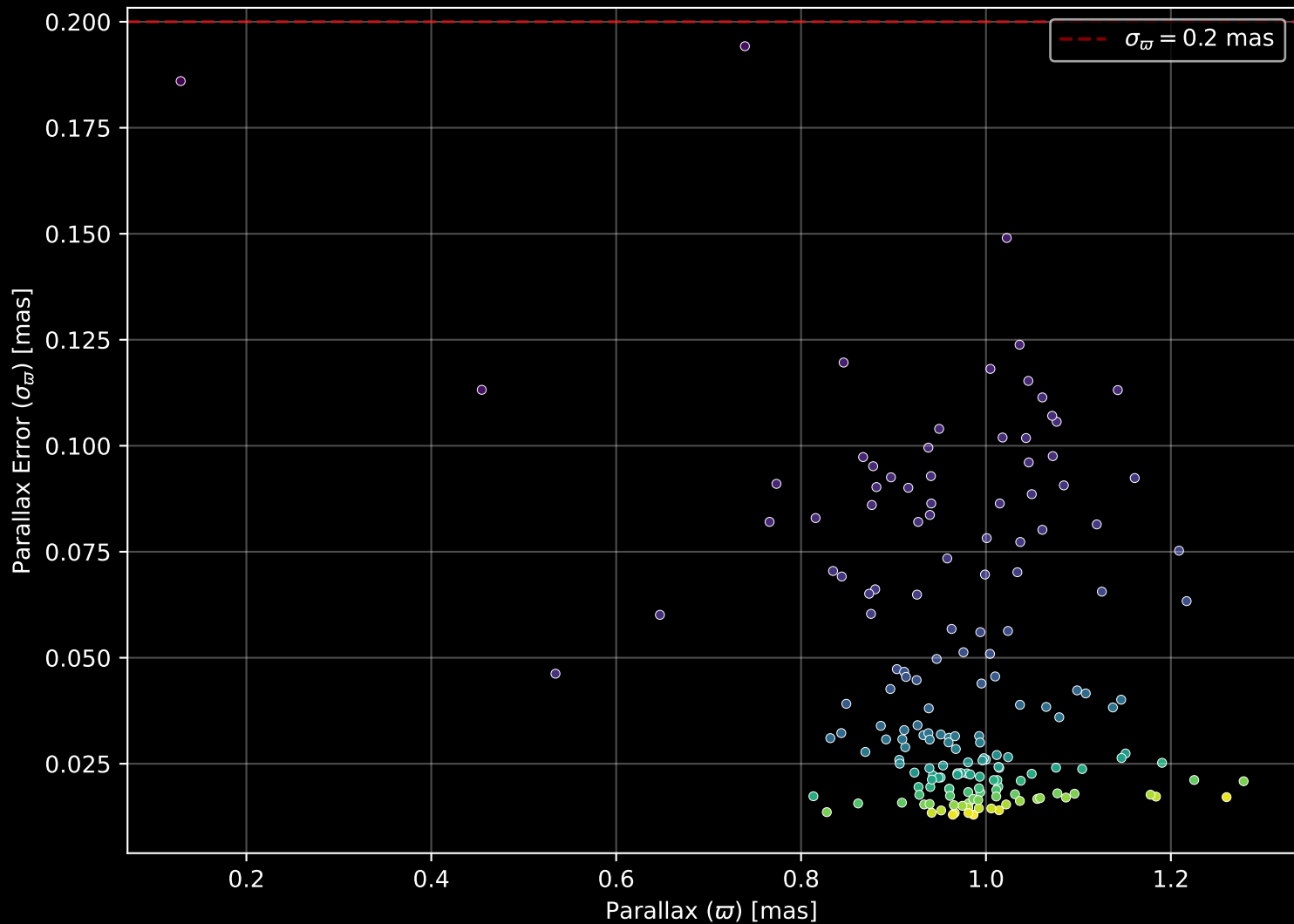
Gaia Cluster: [UPK_470] Parallax Quality (n= 172)
