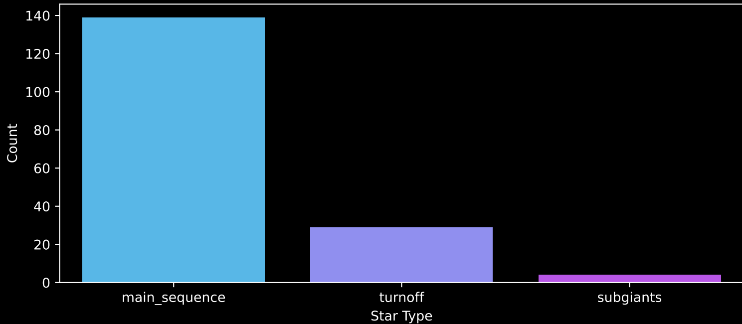
Gaia Cluster: [UPK_470] Count plot of Star Type
