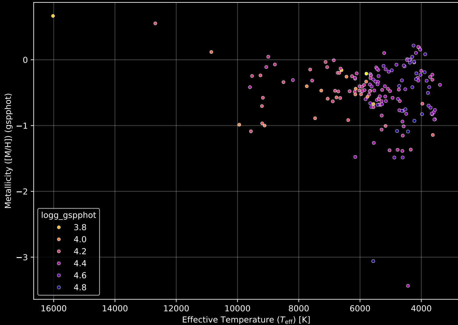
Gaia Cluster: [UPK_470] Stellar Population Parameters (n= 172)
