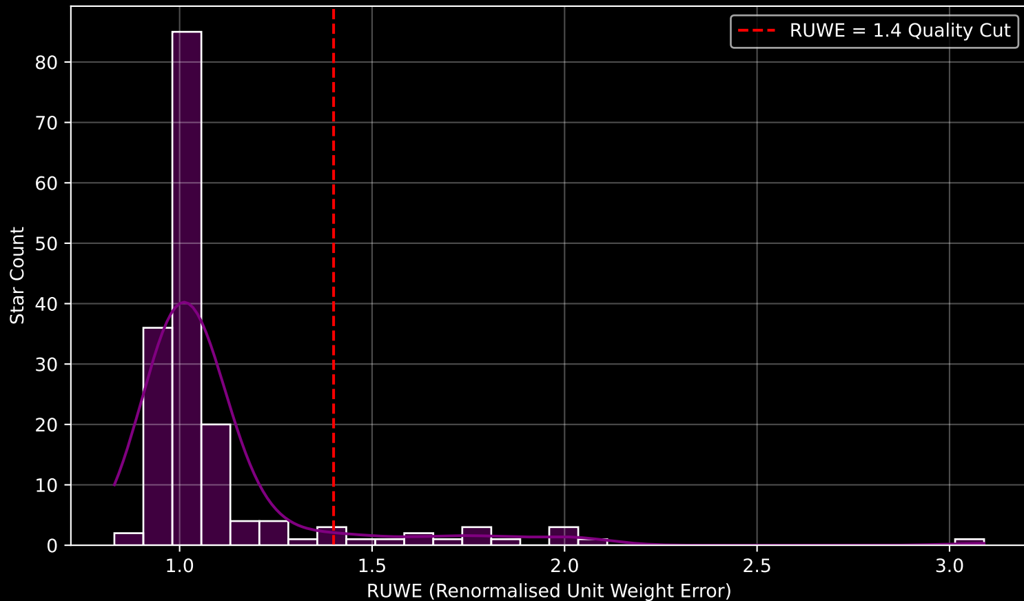
Gaia Cluster: [UPK_470] RUWE Distribution (n= 169)
