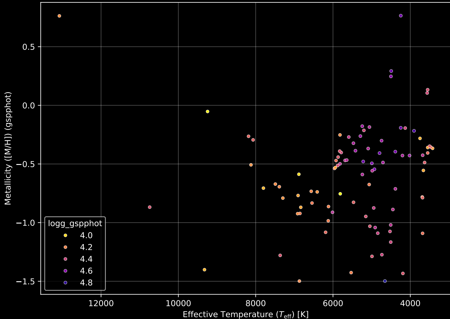
Gaia Cluster: [UPK_537] Stellar Population Parameters (n= 93)
