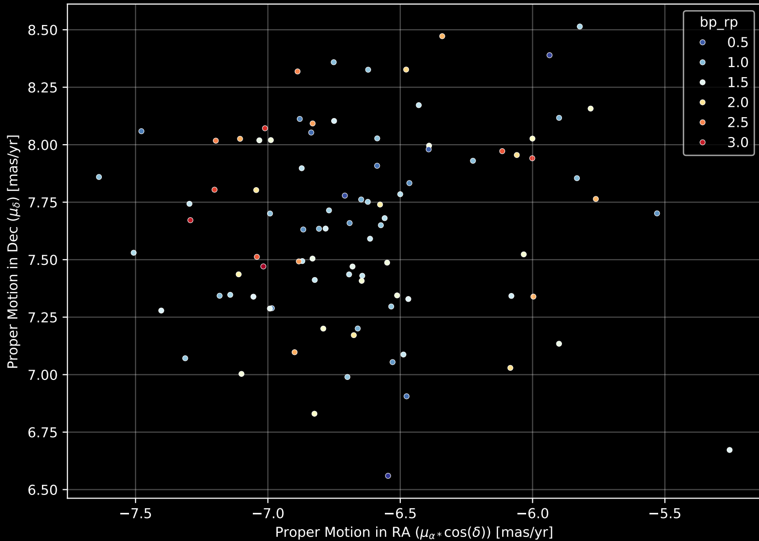
Gaia Cluster: [UPK_537] Proper Motion Diagram (n= 93)
