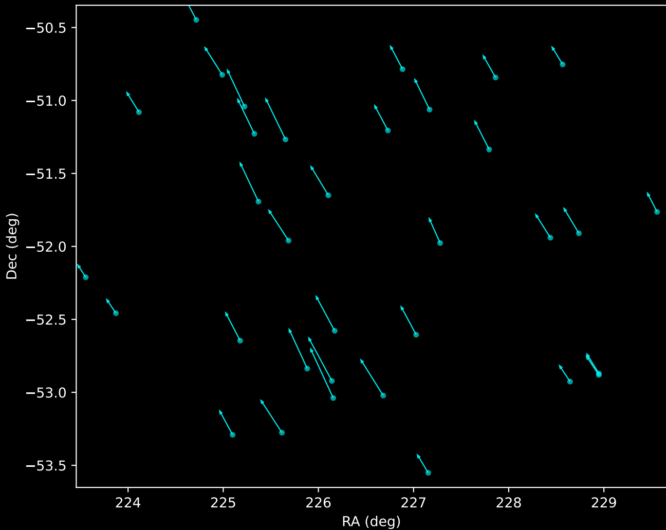
Gaia DR3 Noise Stream Proper Motion Vectors (n=34)
