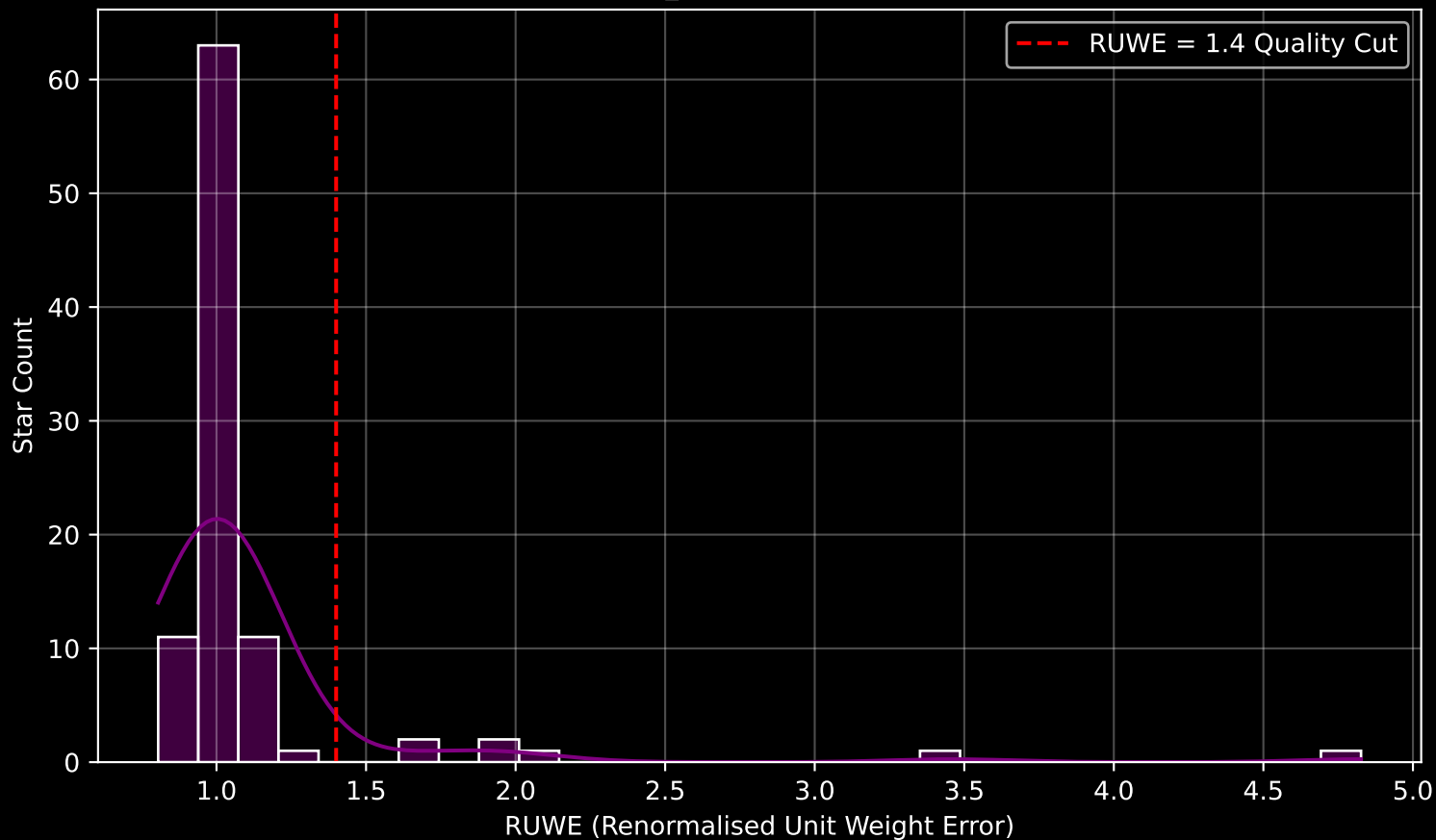
Gaia Cluster: [UPK_537] RUWE Distribution (n= 93)
