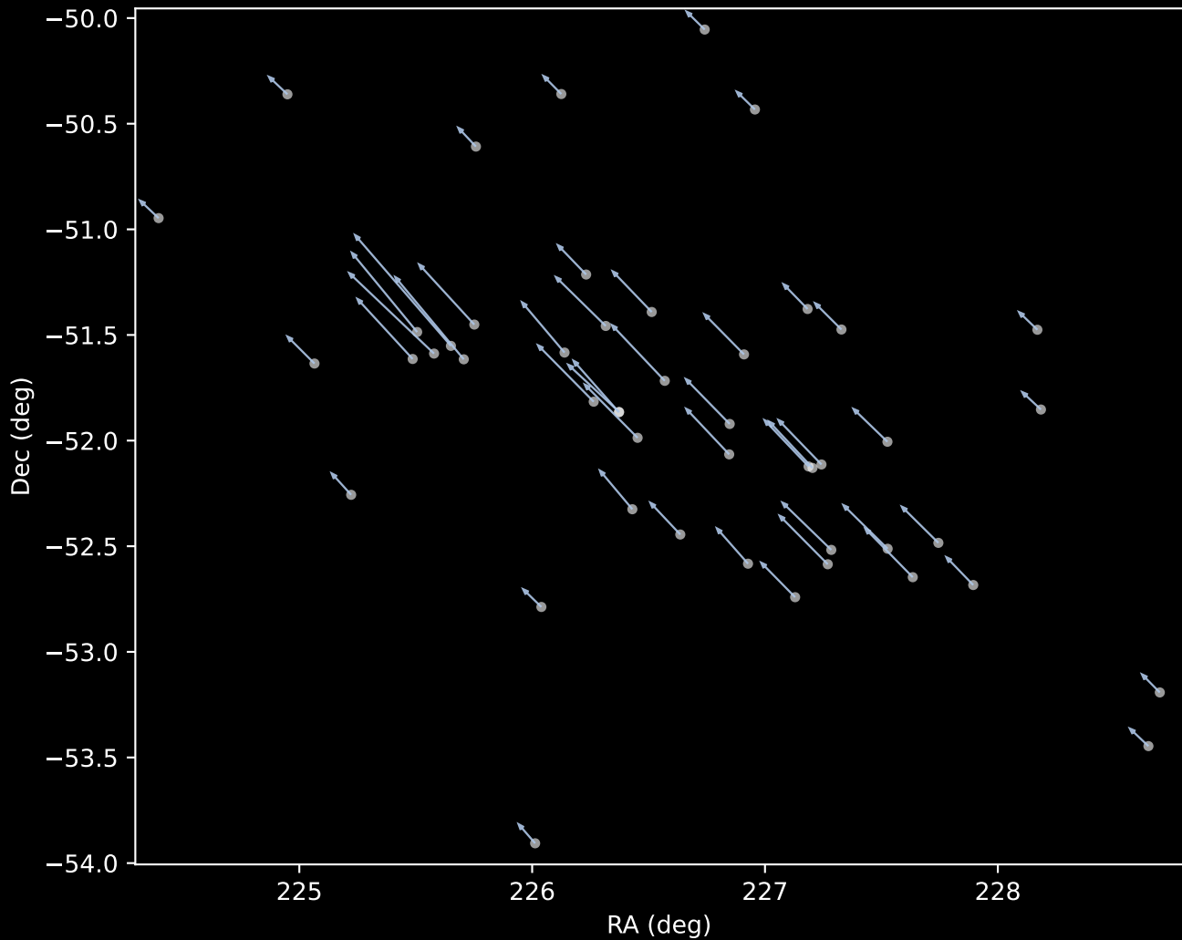
Gaia DR3 Cluster 1 Proper Motion Vectors (n=48)
