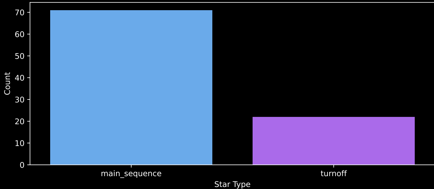
Gaia Cluster: [UPK_537] Count plot of Star Type
