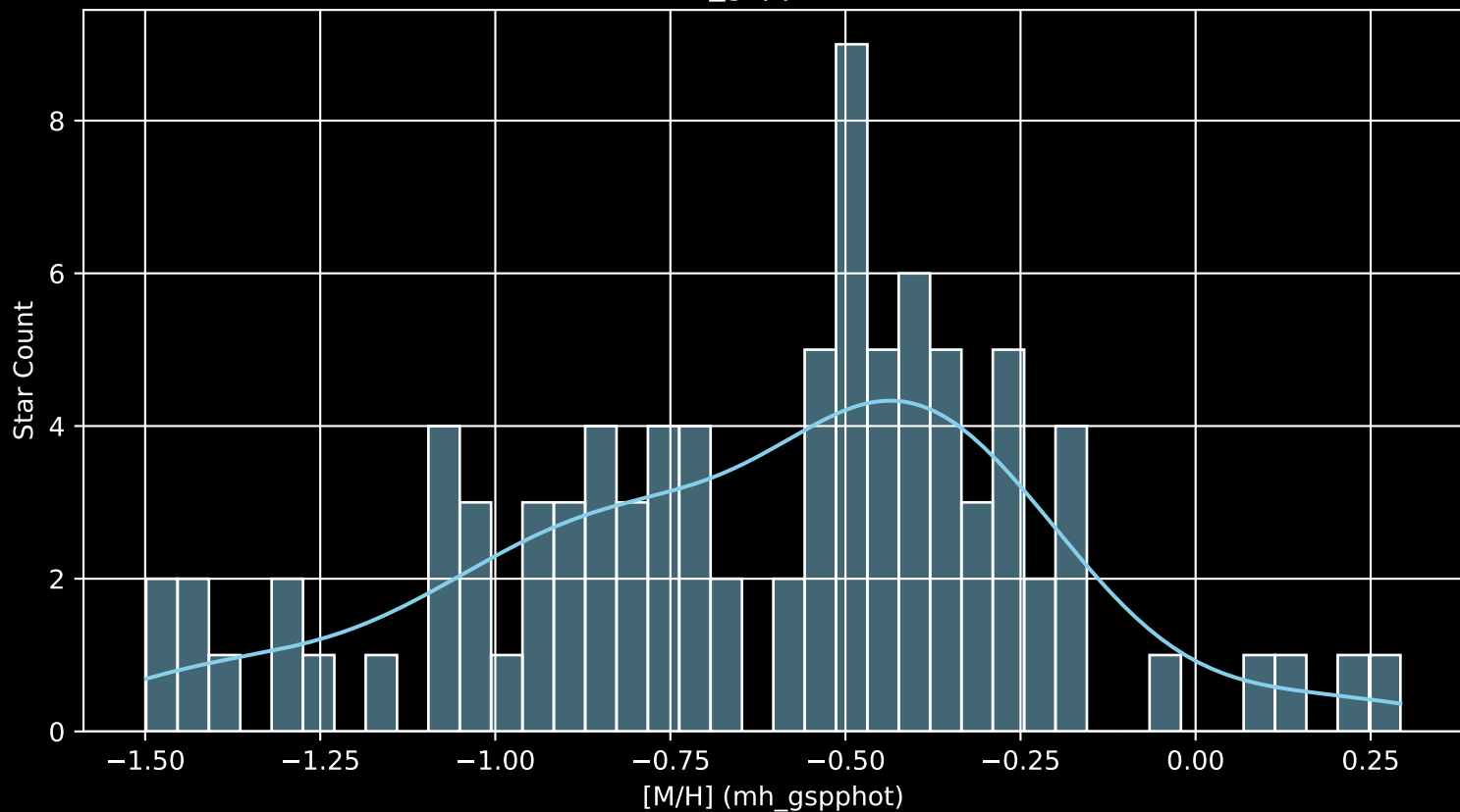
Gaia Cluster: [UPK_537 [M/H] (mh_gspphot) (n= 91)
