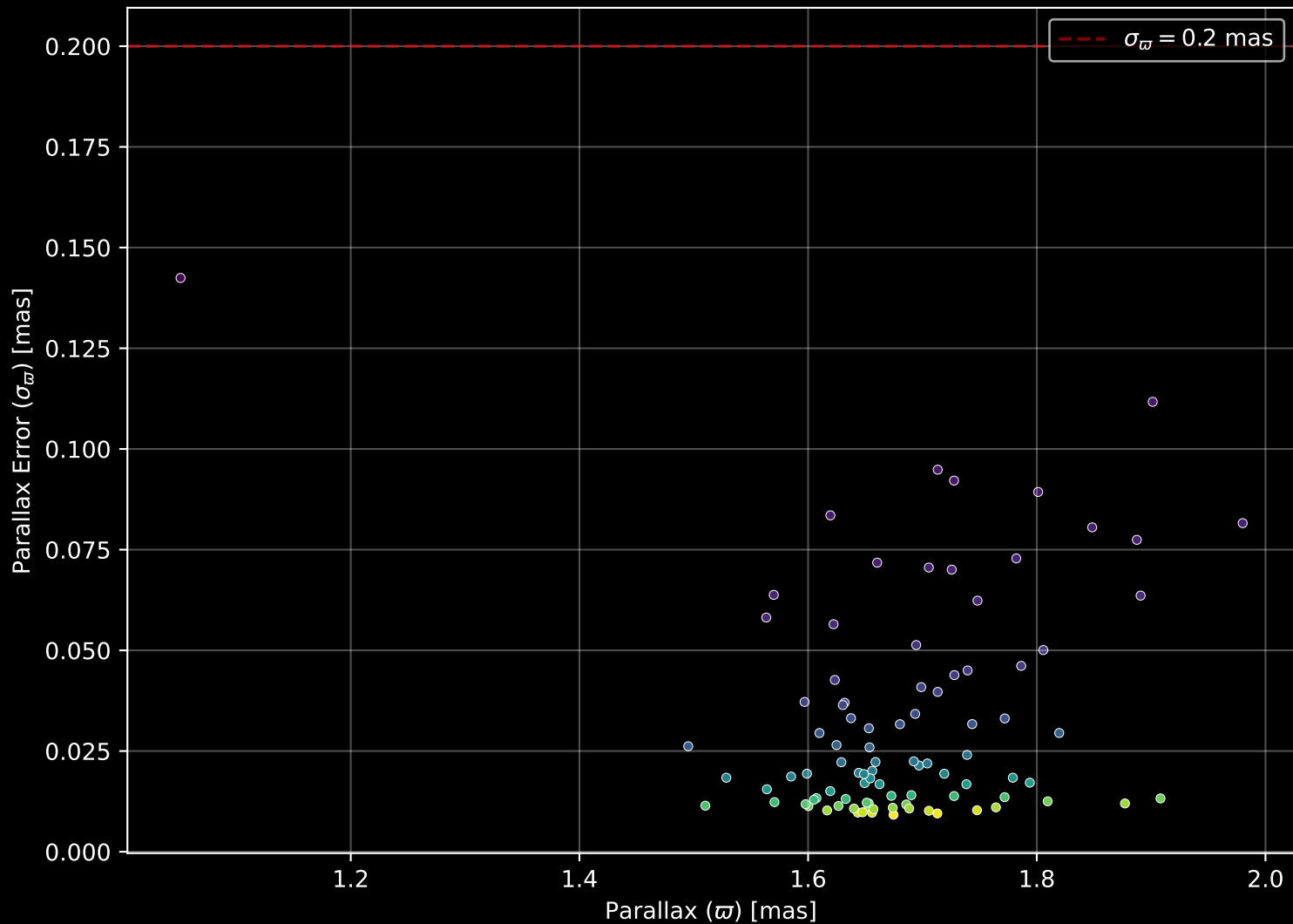
Gaia Cluster: [UPK_537] Parallax Quality (n= 93)
