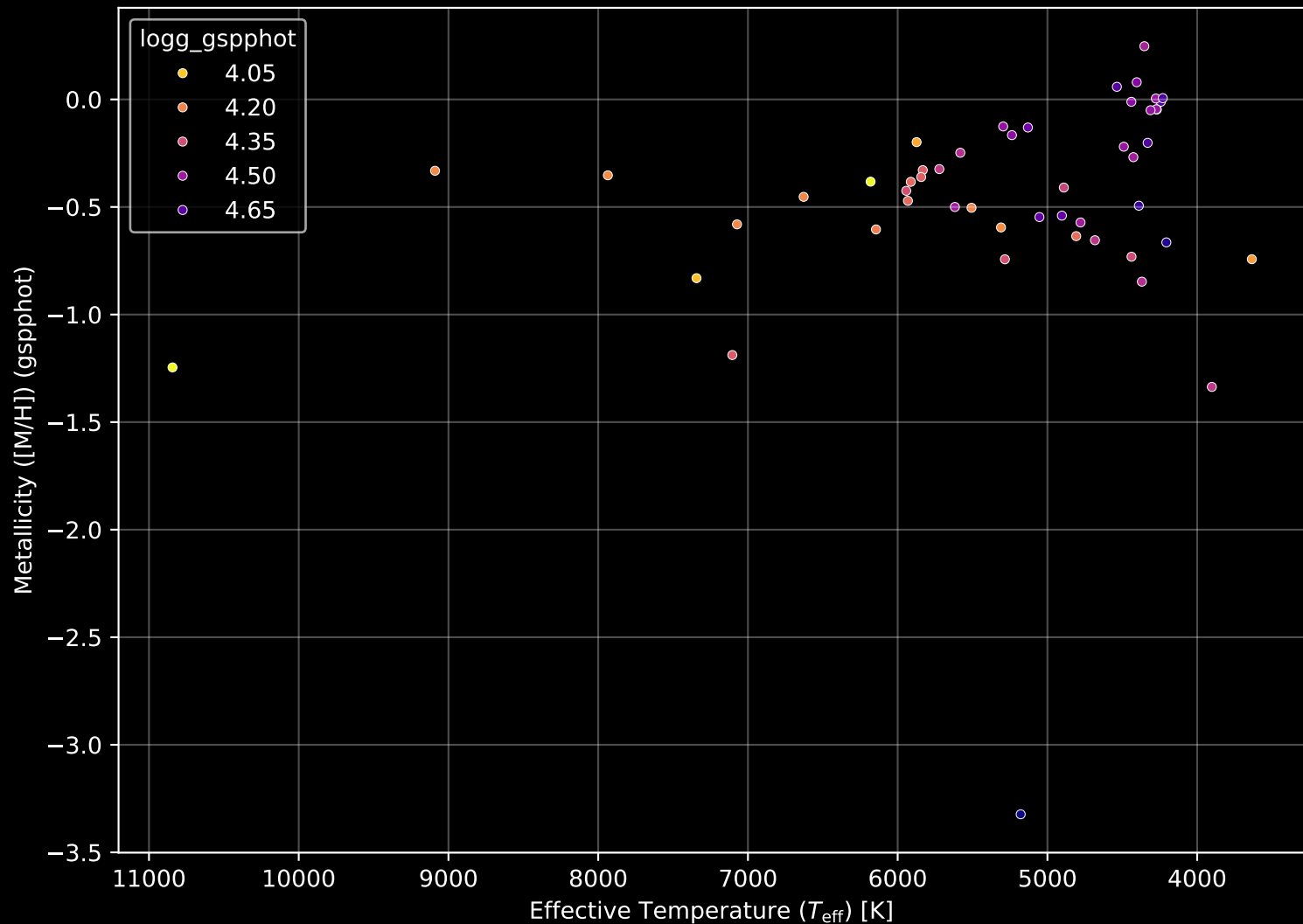
Gaia Cluster: [UPK_542] Stellar Population Parameters (n= 50)
