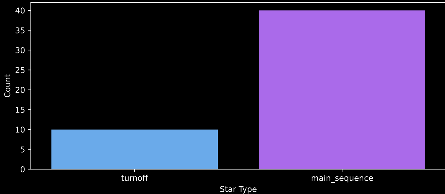
Gaia Cluster: [UPK_542] Count plot of Star Type
