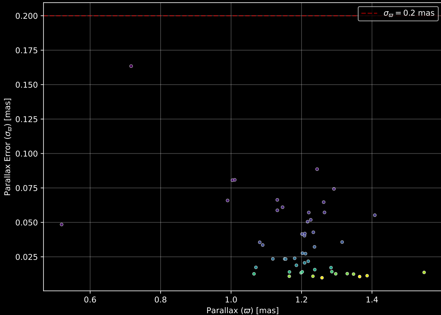
Gaia Cluster: [UPK_542] Parallax Quality (n= 50)
