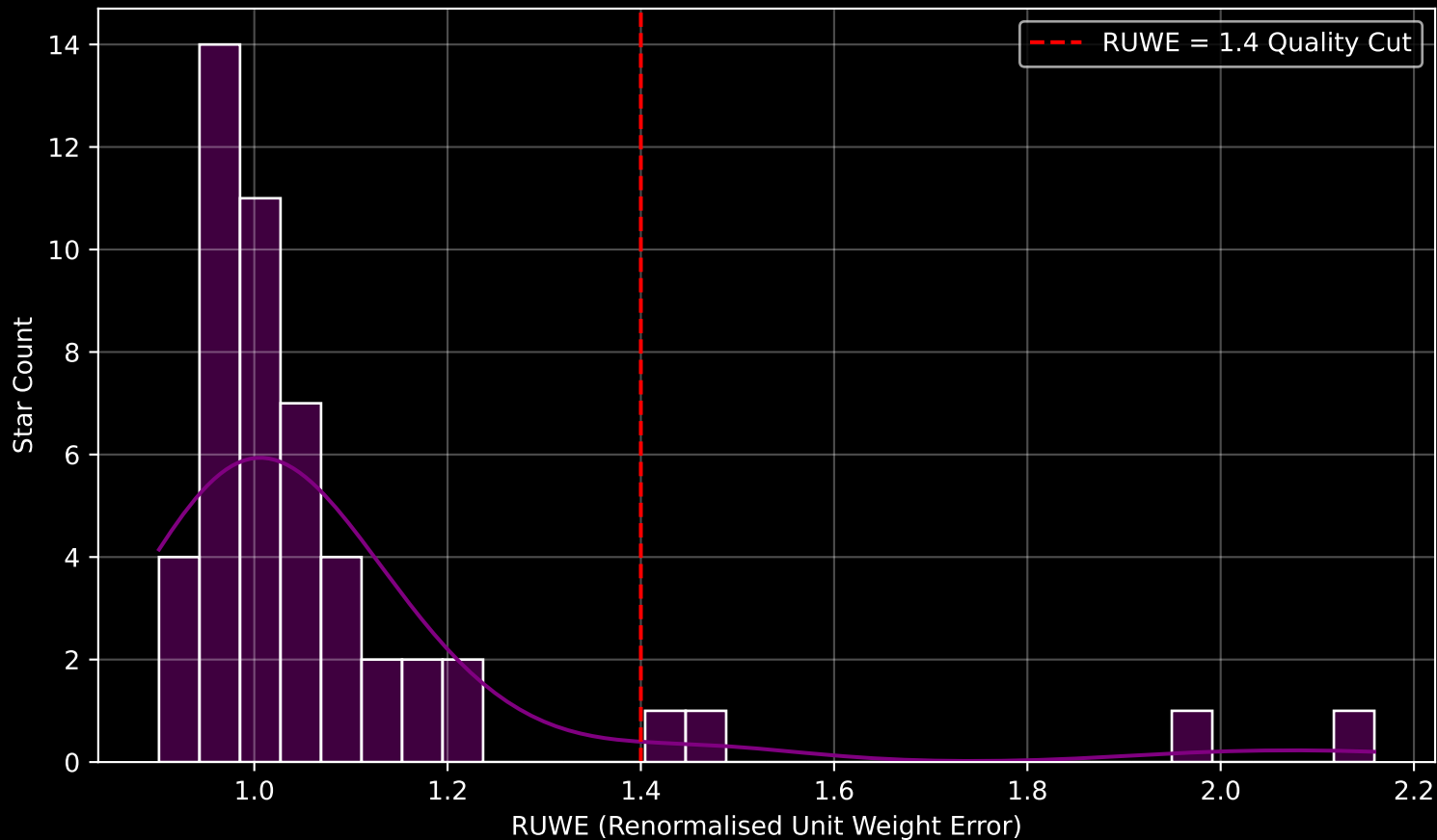
Gaia Cluster: [UPK_542] RUWE Distribution (n= 50)
