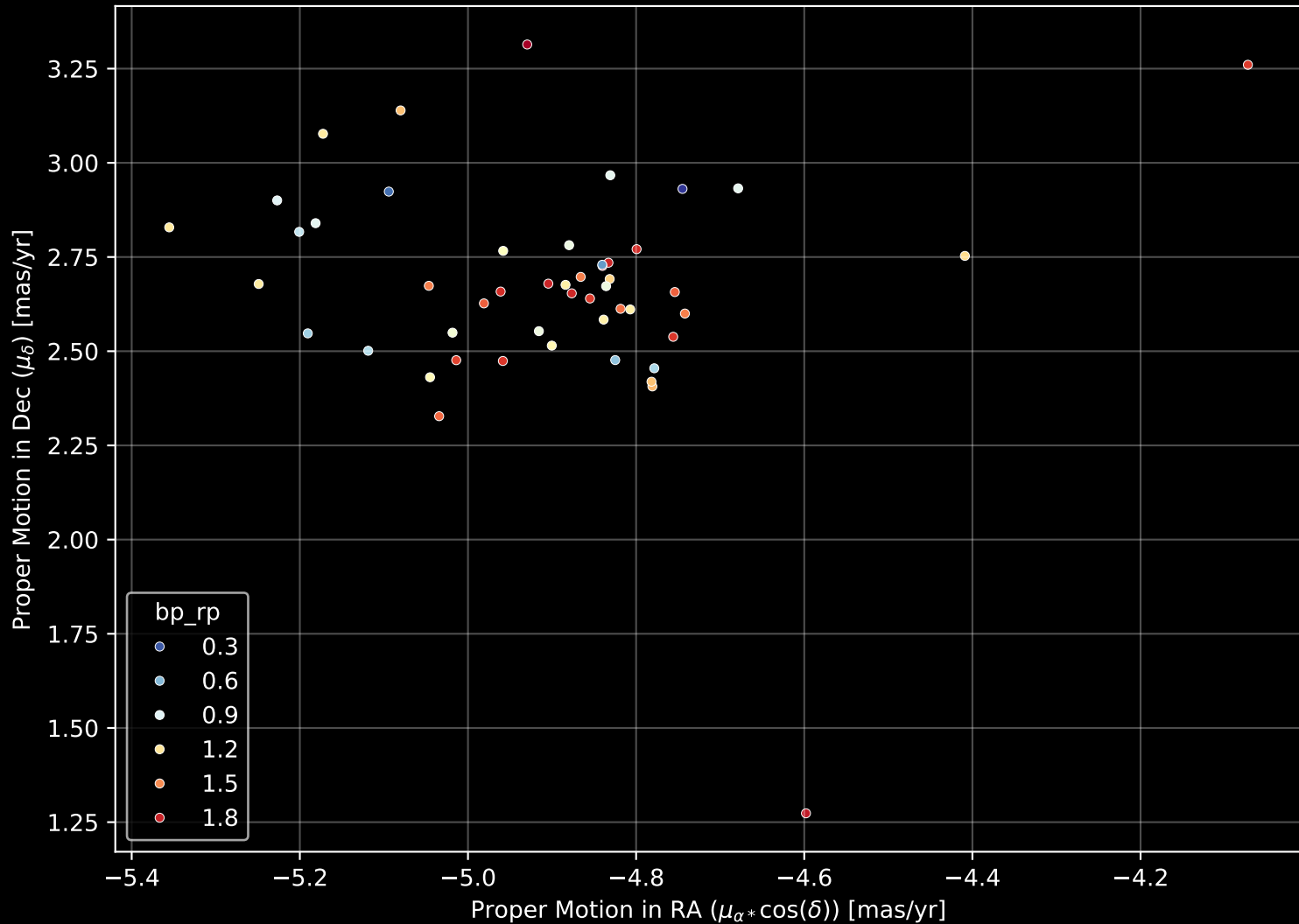
Gaia Cluster: [UPK_542] Proper Motion Diagram (n= 50)
