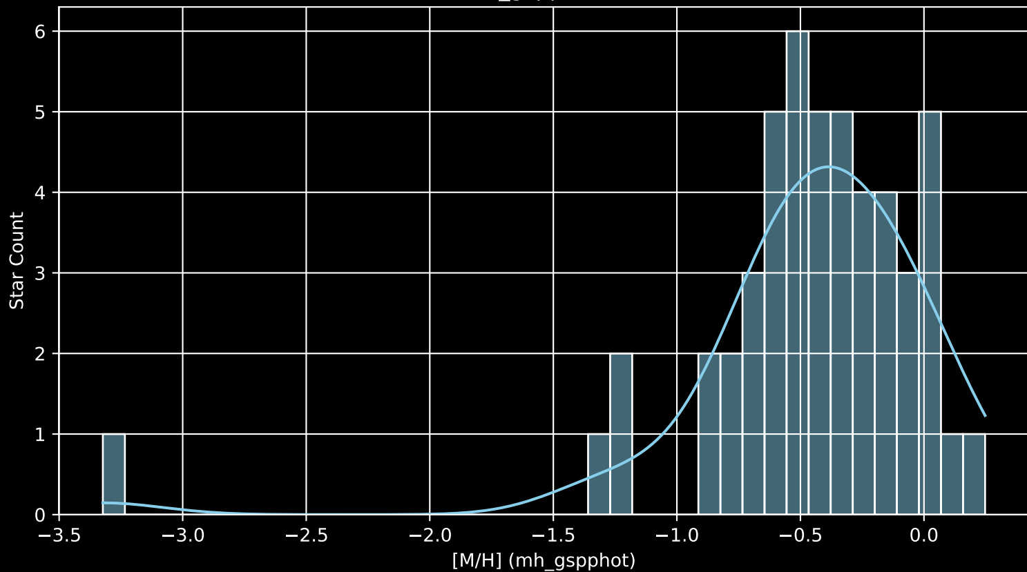
Gaia Cluster: [UPK_542 [M/H] (mh_gspphot) (n= 50)
