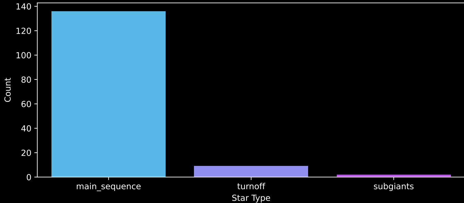
Gaia Cluster: [UPK_545] Count plot of Star Type
