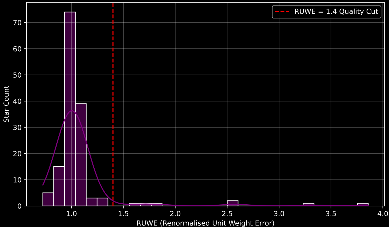
Gaia Cluster: [UPK_545] RUWE Distribution (n= 146)
