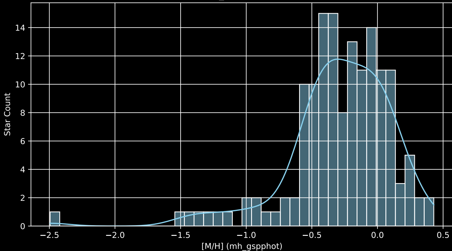
Gaia Cluster: [UPK_545 [M/H] (mh_gspphot) (n= 147)
