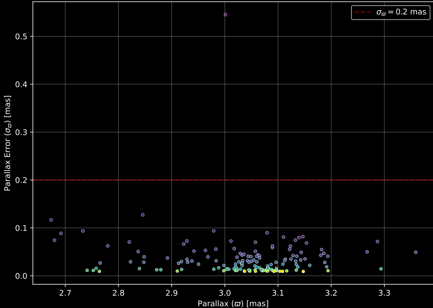
Gaia Cluster: [UPK_545] Parallax Quality (n= 147)
