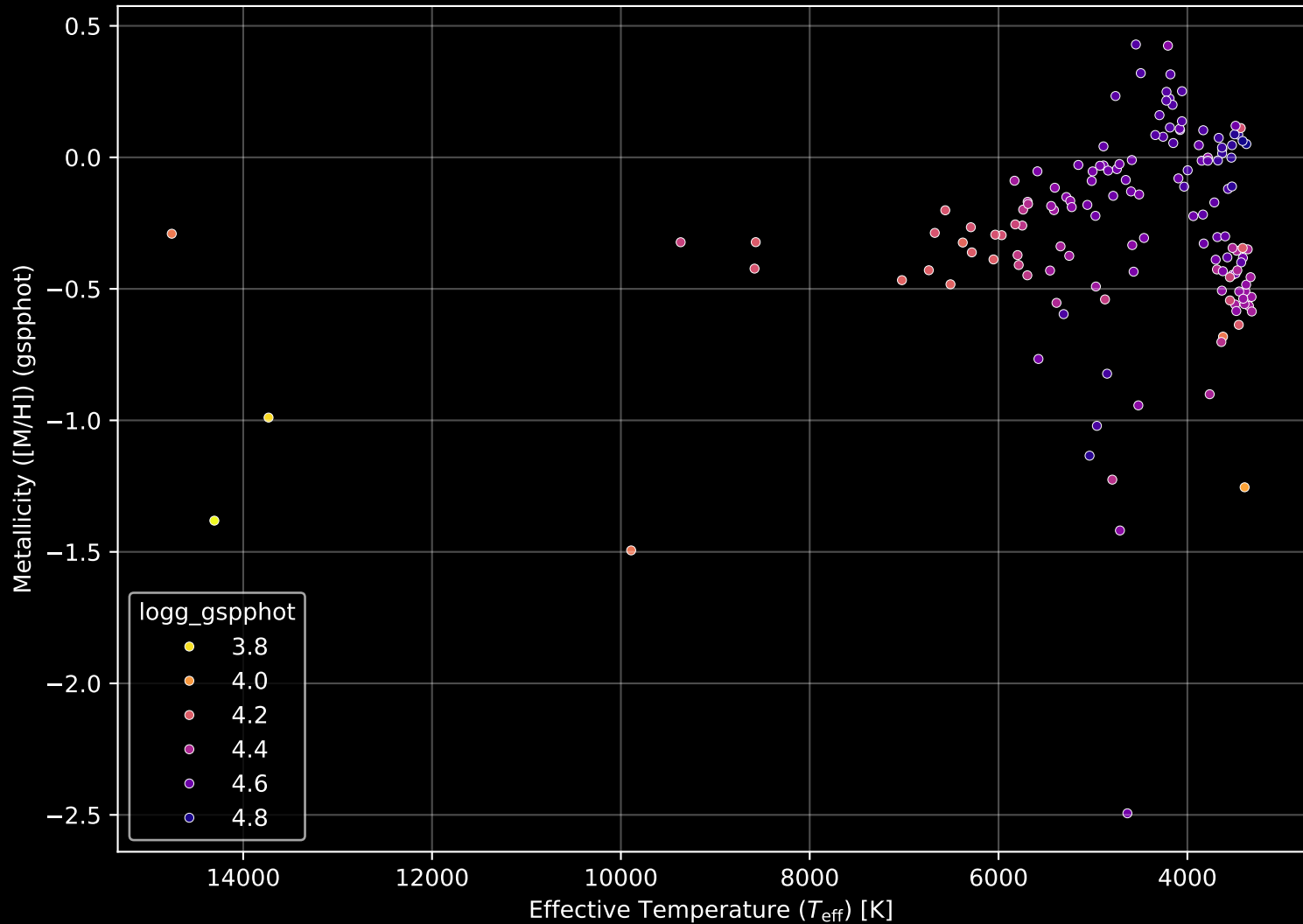
Gaia Cluster: [UPK_545] Stellar Population Parameters (n= 147)
