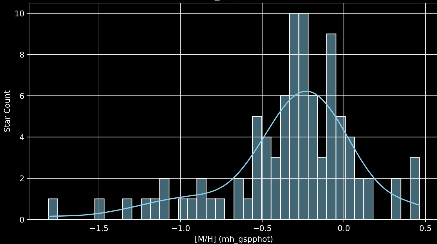
Gaia Cluster: [UPK_562 [M/H] (mh_gspphot) (n= 90)
