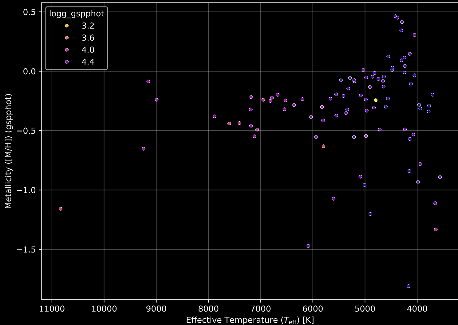
Gaia Cluster: [UPK_562] Stellar Population Parameters (n= 90)
