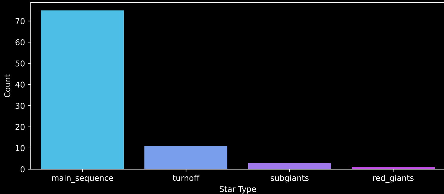
Gaia Cluster: [UPK_562] Count plot of Star Type
