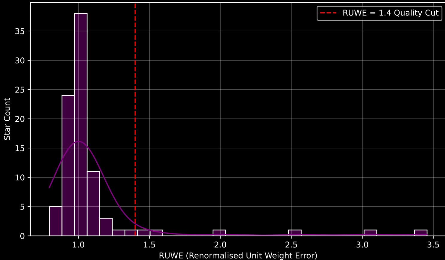
Gaia Cluster: [UPK_562] RUWE Distribution (n= 89)
