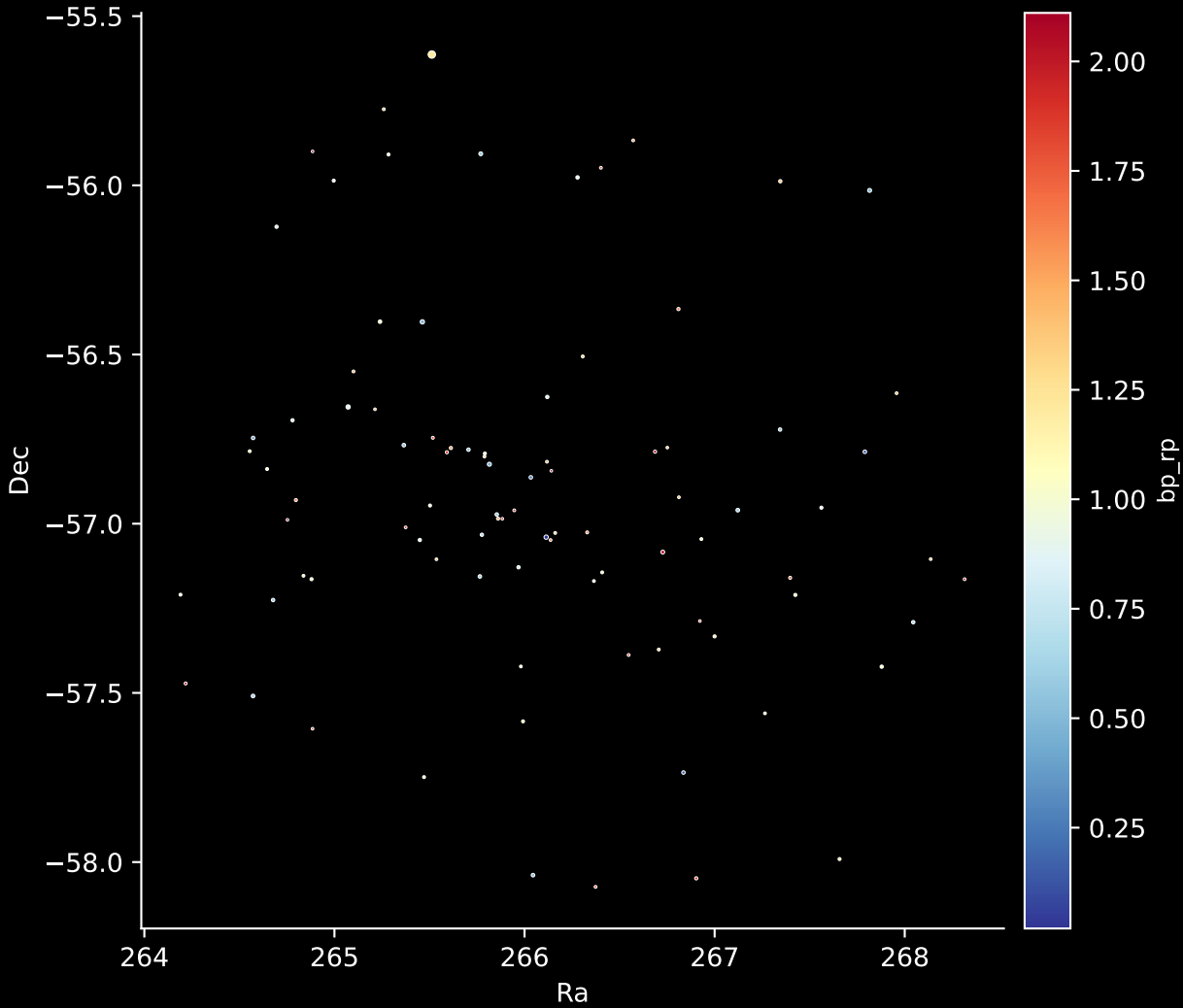
Gaia Cluster: [UPK_562] Stars: 90
