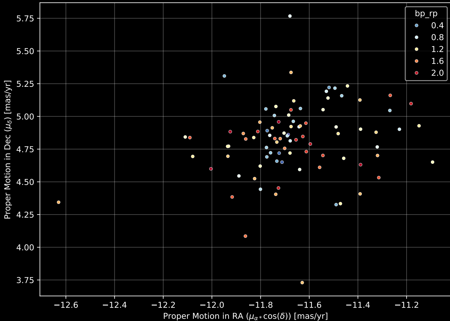
Gaia Cluster: [UPK_562] Proper Motion Diagram (n= 90)
