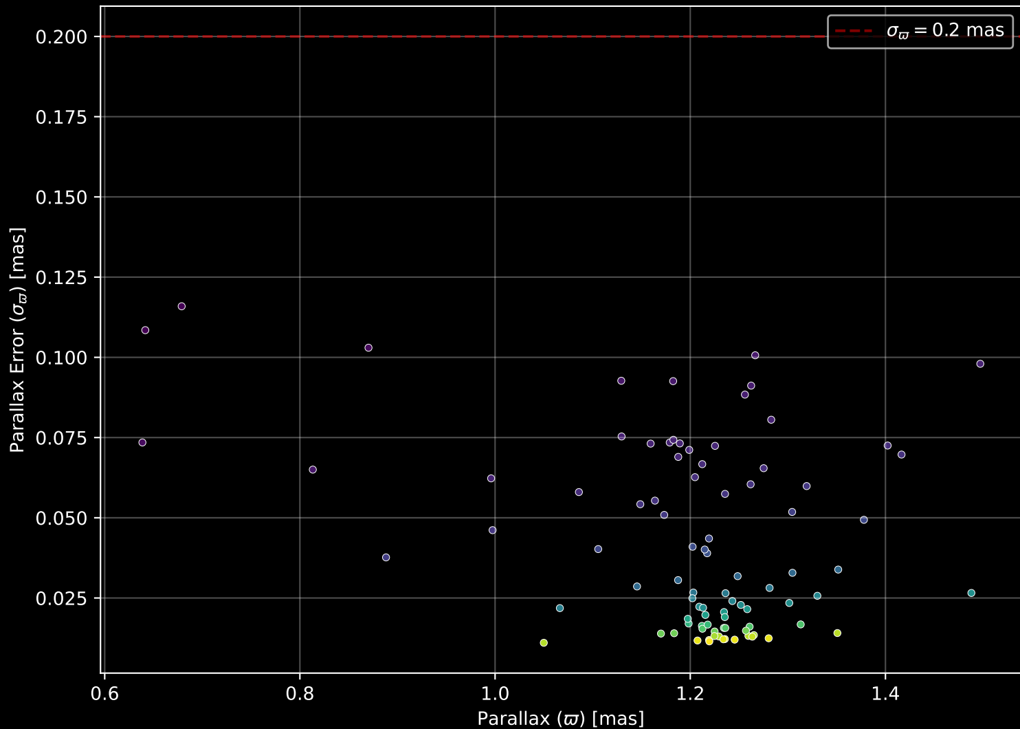
Gaia Cluster: [UPK_562] Parallax Quality (n= 90)
