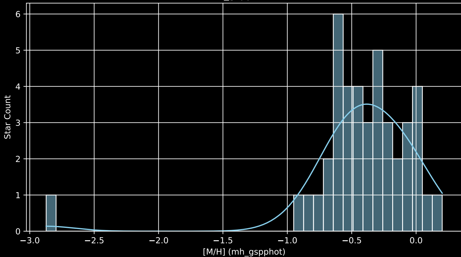
Gaia Cluster: [UPK_578 [M/H] (mh_gspphot) (n= 42)
