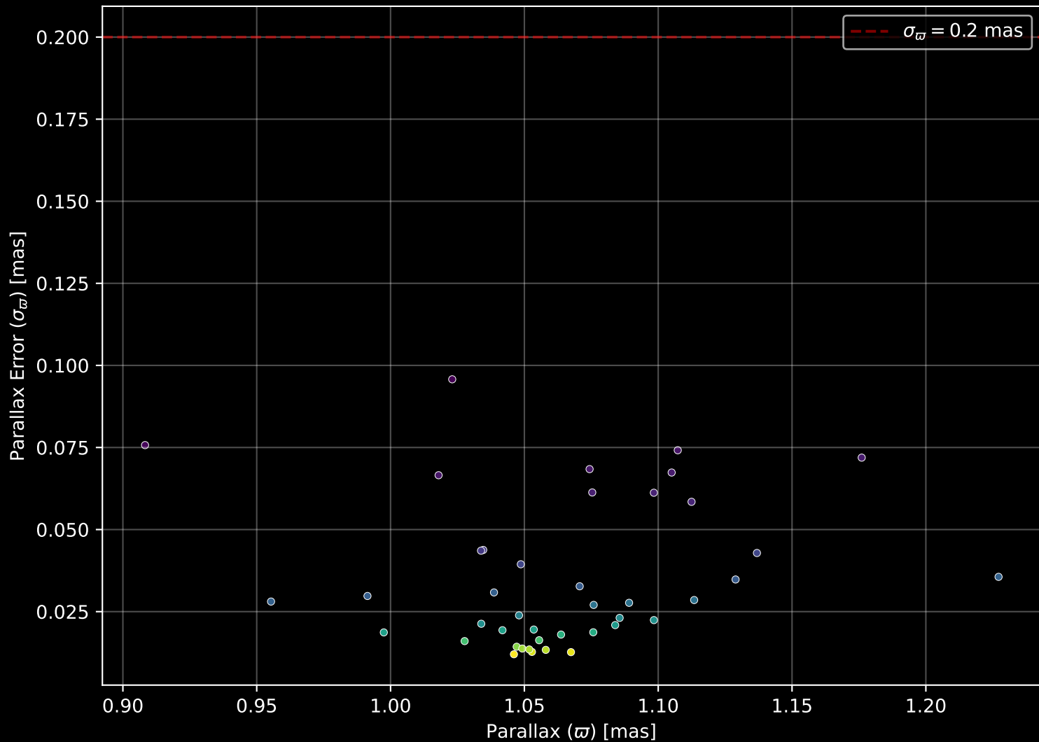
Gaia Cluster: [UPK_578] Parallax Quality (n= 42)
