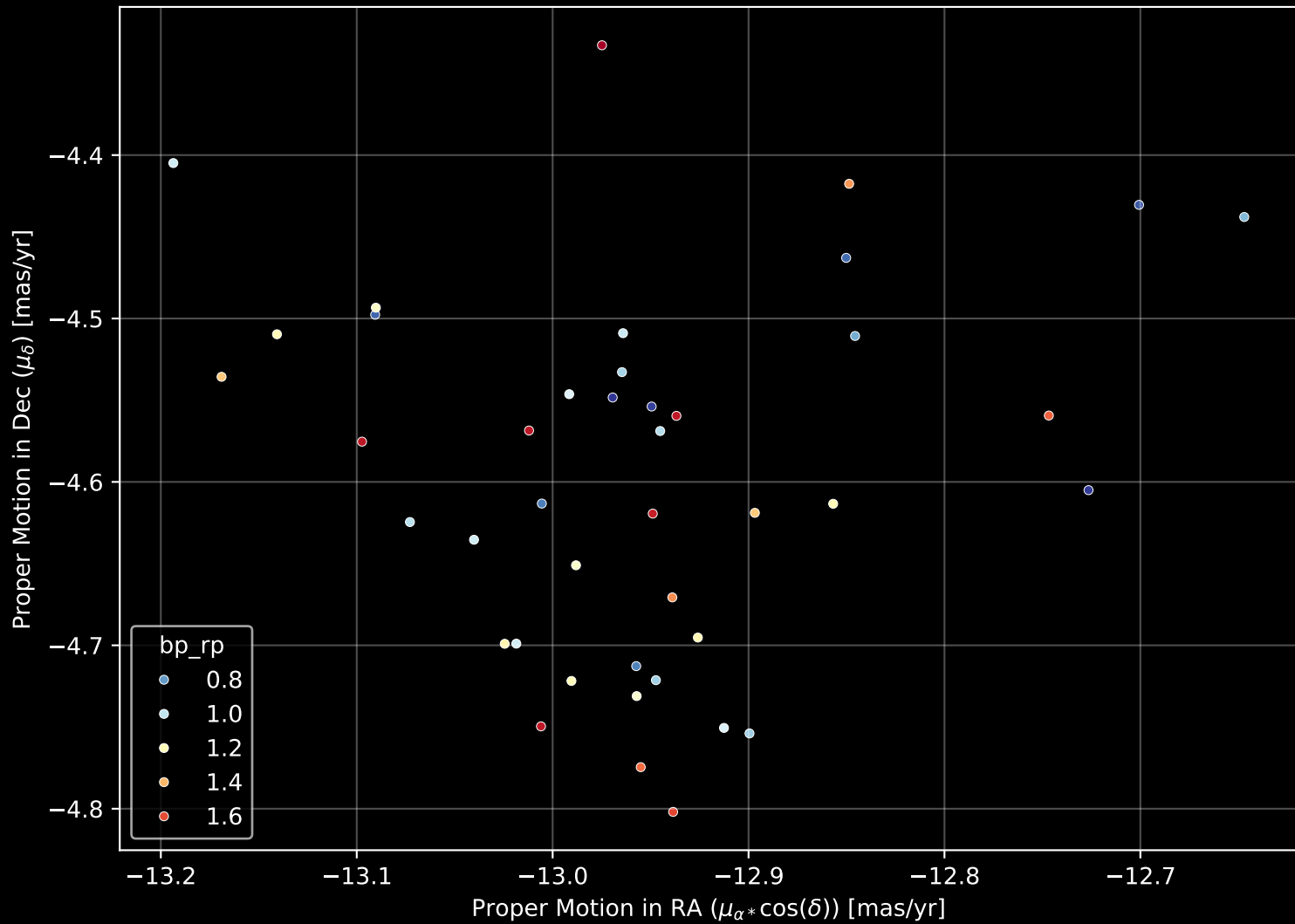
Gaia Cluster: [UPK 578] Proper Motion Diagram (n= 42)
