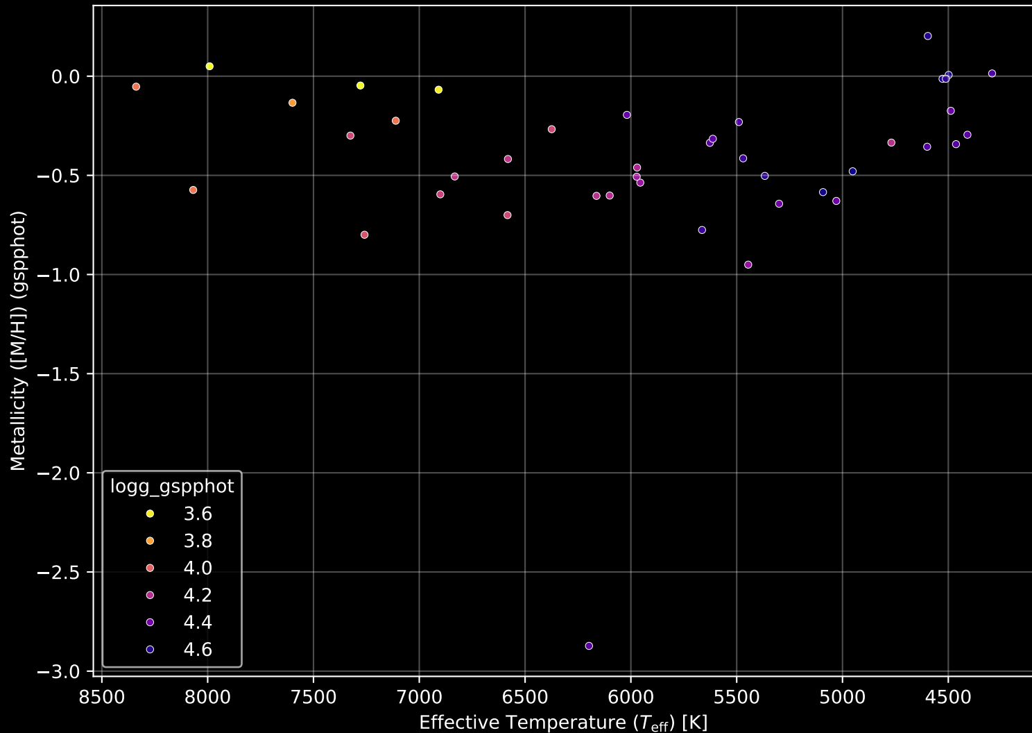
Gaia Cluster: [UPK_578] Stellar Population Parameters (n= 42)
