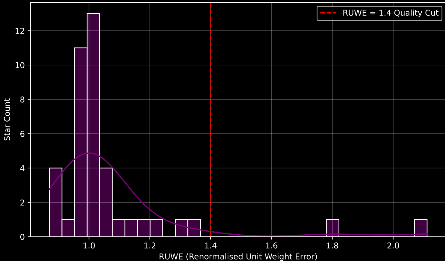
Gaia Cluster: [UPK_578] RUWE Distribution (n= 41)
