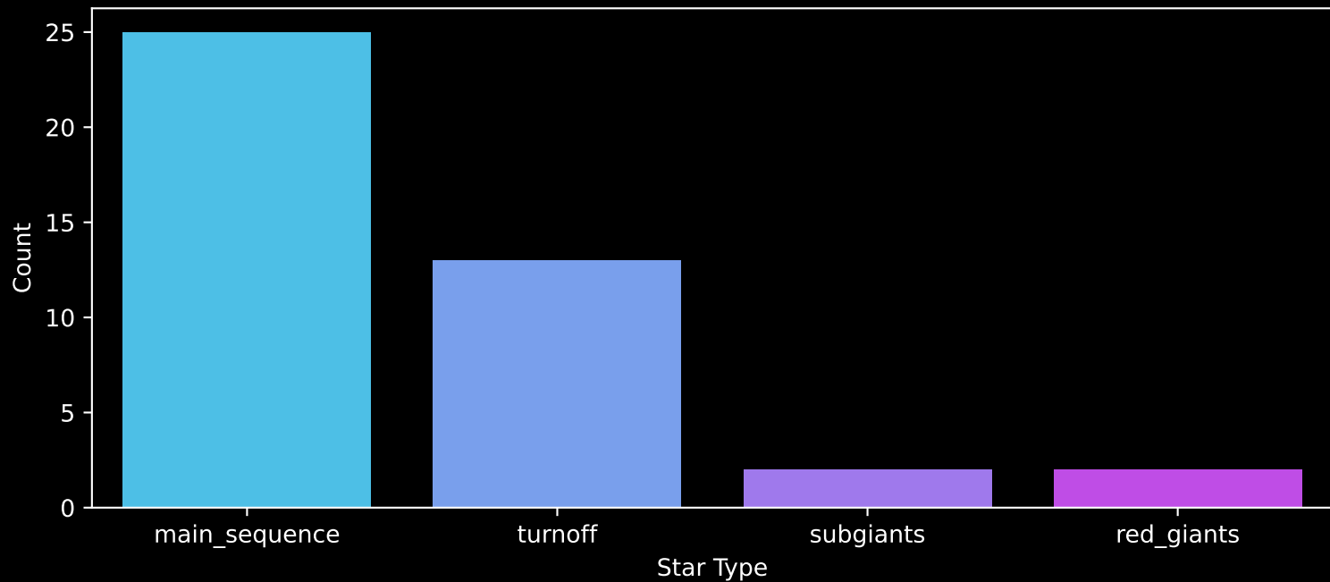
Gaia Cluster: [UPK_578] Count plot of Star Type
