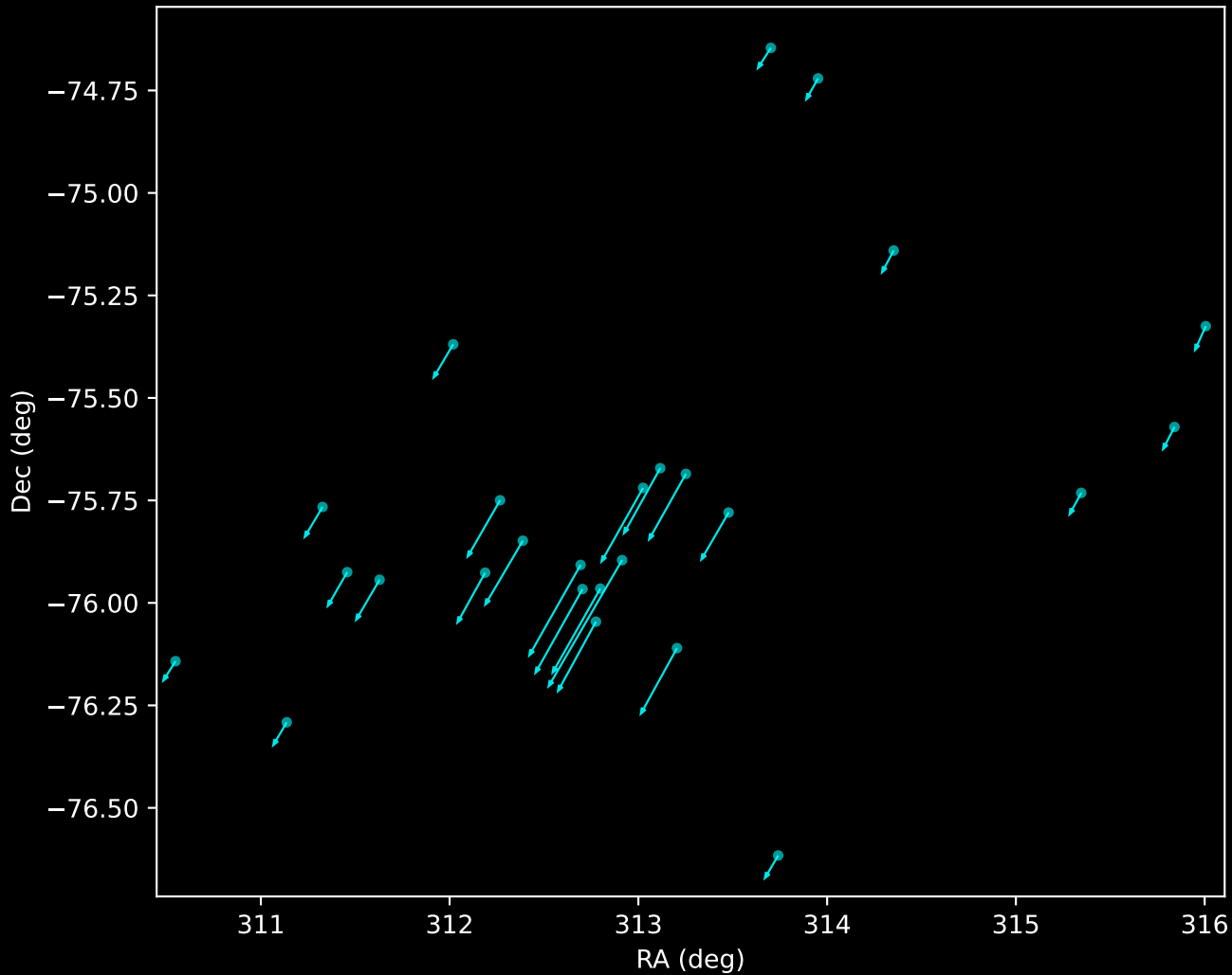
Gaia DR3 Noise Stream Proper Motion Vectors (n=26)
