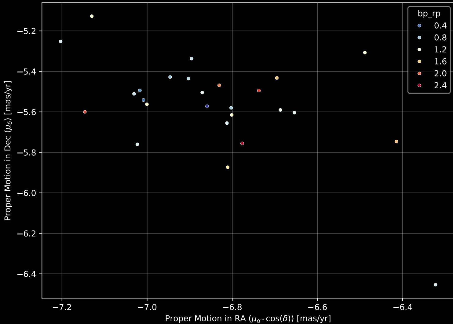
Gaia Cluster: [UPK_585] Proper Motion Diagram (n= 26)
