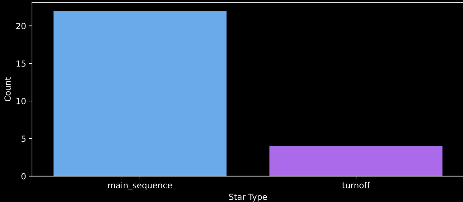
Gaia Cluster: [UPK_585] Count plot of Star Type
