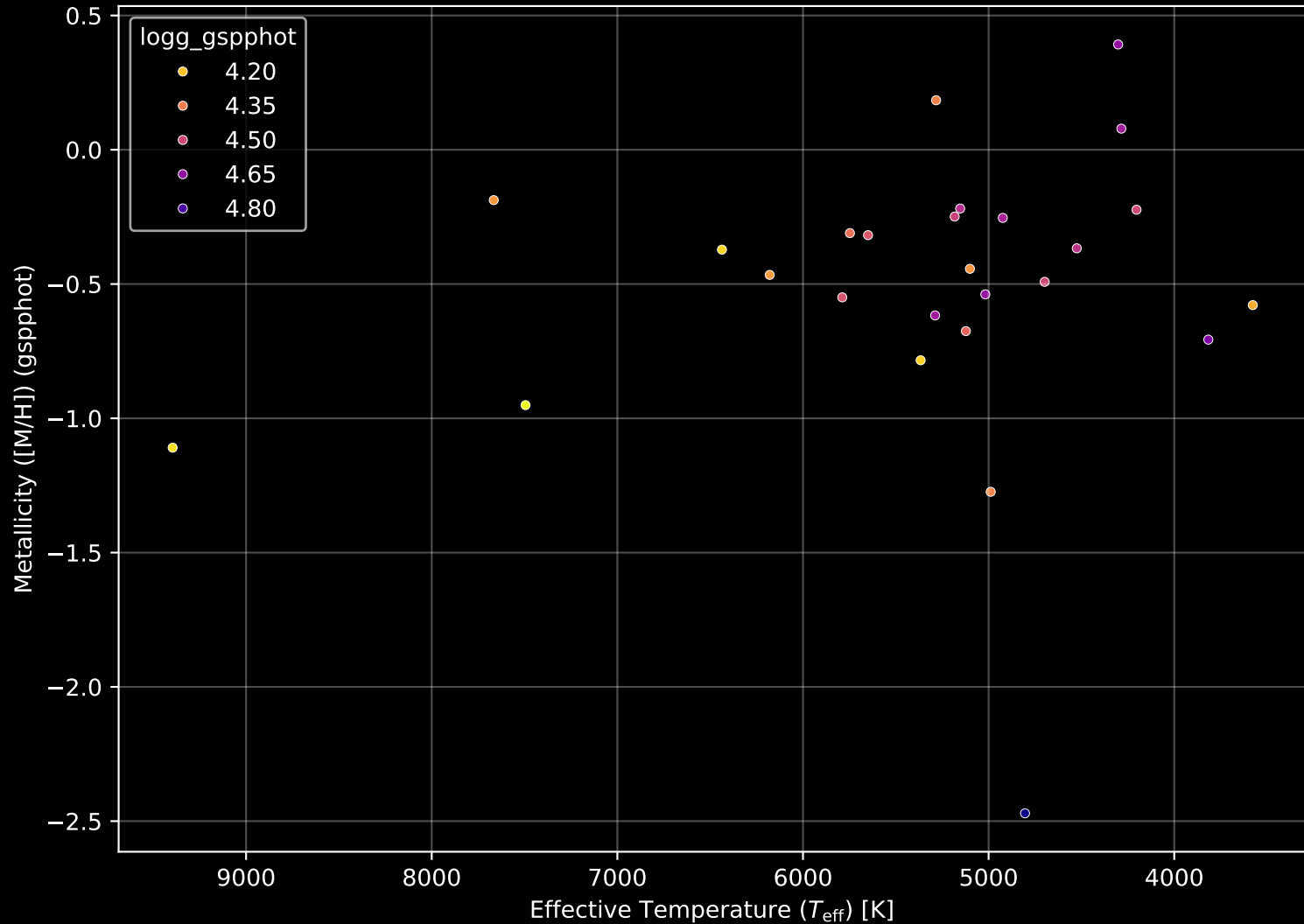
Gaia Cluster: [UPK_585] Stellar Population Parameters (n= 26)
