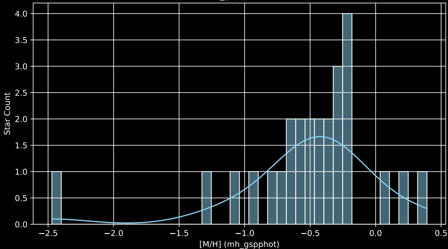
Gaia Cluster: [UPK_585 [M/H] (mh_gspphot) (n= 26)
