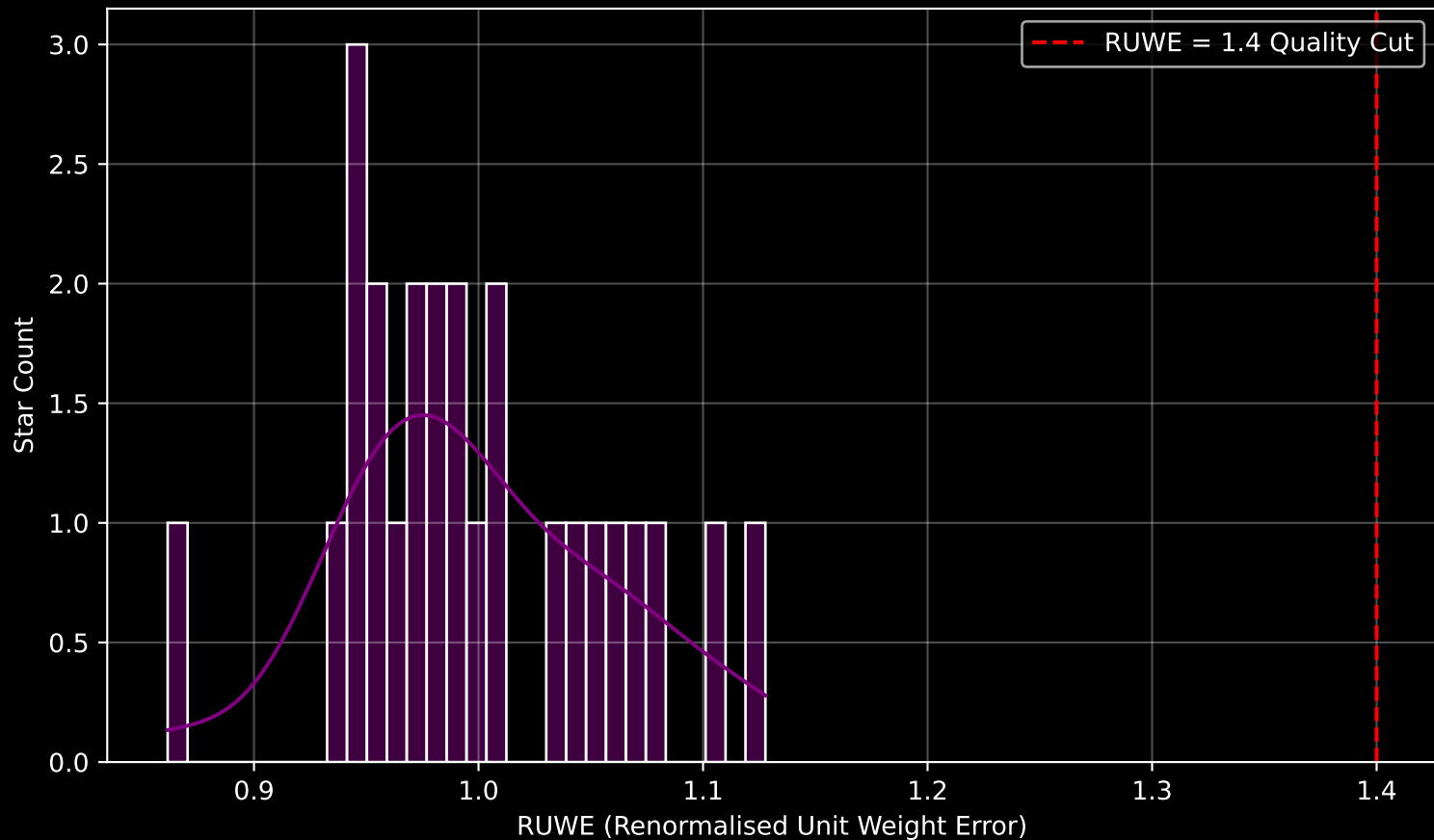
Gaia Cluster: [UPK_585] RUWE Distribution (n= 25)
