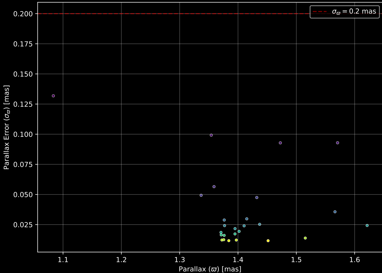
Gaia Cluster: [UPK 585] Parallax Quality (n= 26)
