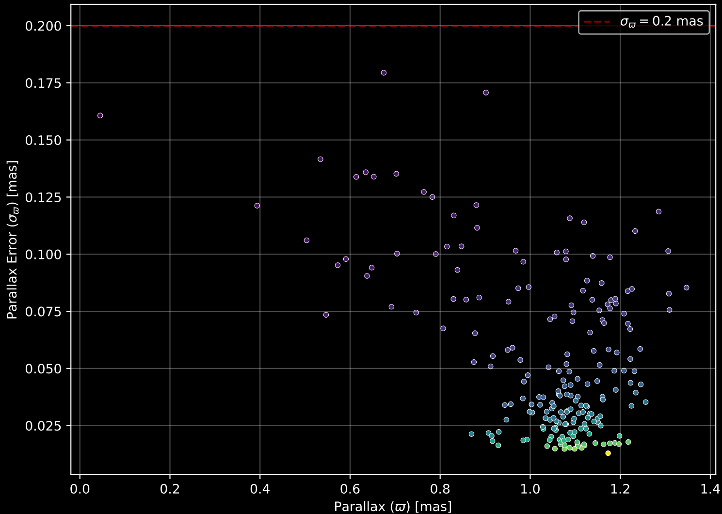
Gaia Cluster: [UPK_587] Parallax Quality (n= 205)
