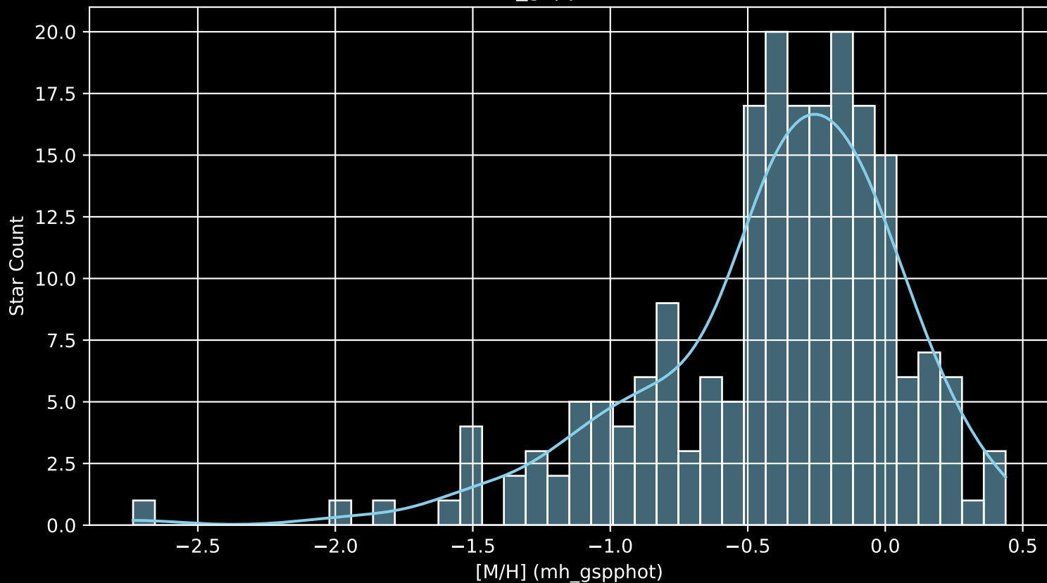
Gaia Cluster: [UPK_587 [M/H] (mh_gspphot) (n= 204)
