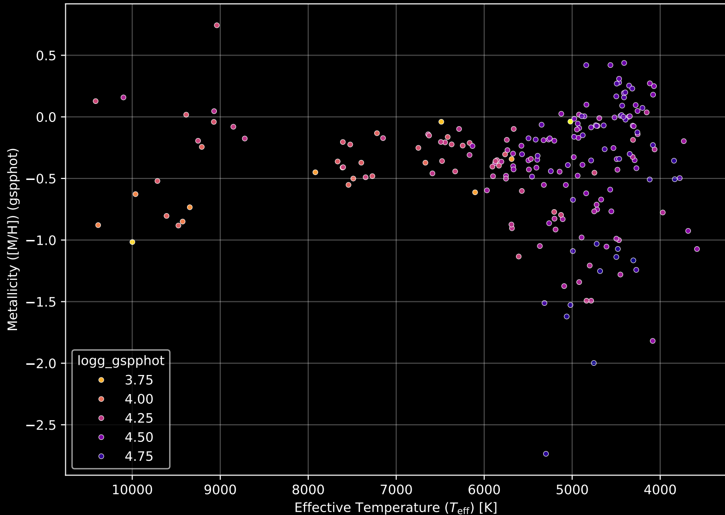
Gaia Cluster: [UPK_587] Stellar Population Parameters (n= 205)
