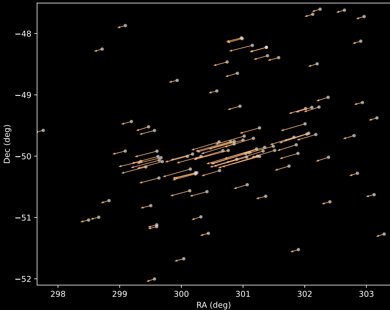
Gaia DR3 Cluster 3 Proper Motion Vectors (n=97)
