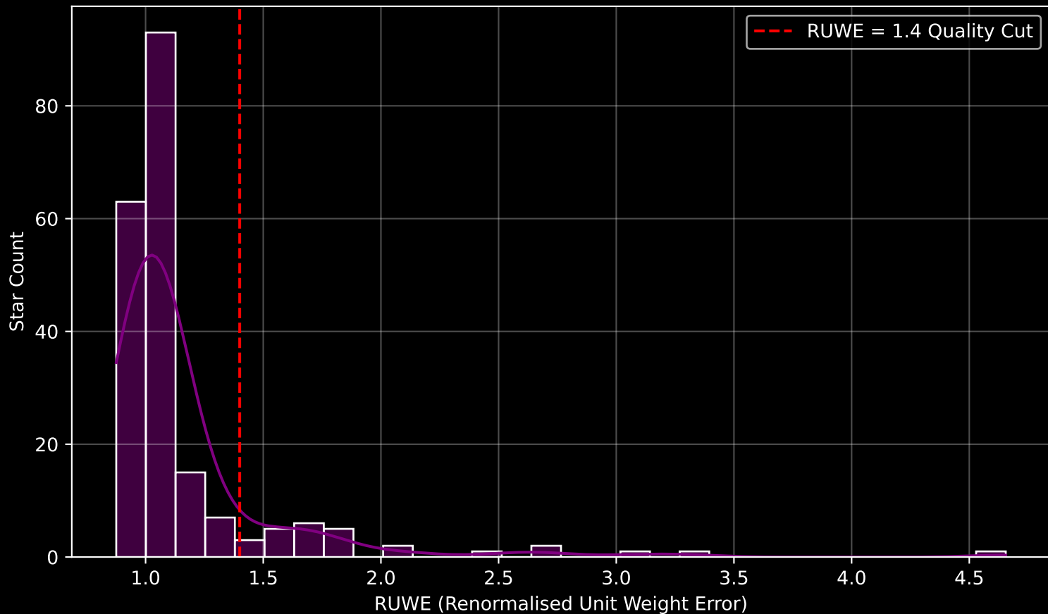
Gaia Cluster: [UPK_587] RUWE Distribution (n= 205)
