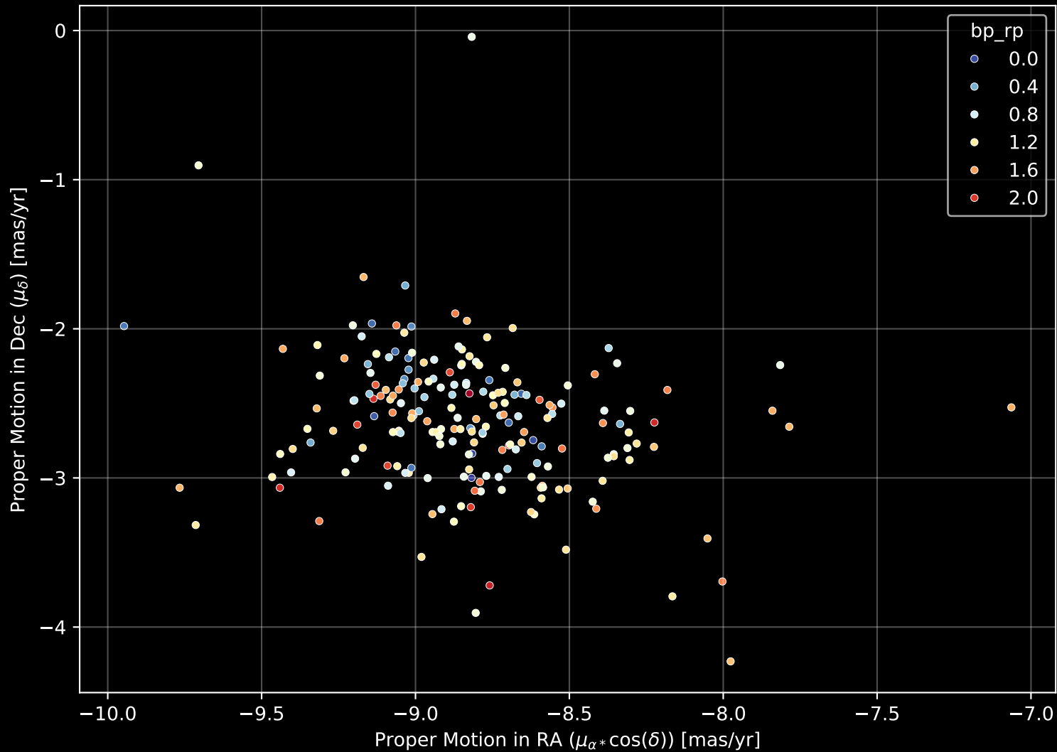
Gaia Cluster: [UPK_587] Proper Motion Diagram (n= 205)
