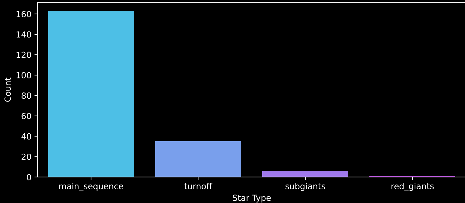
Gaia Cluster: [UPK_587] Count plot of Star Type
