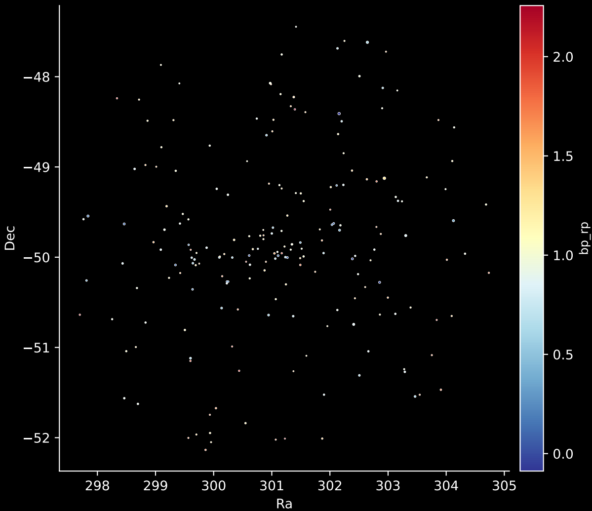
Gaia Cluster: [UPK_587] Stars: 205
