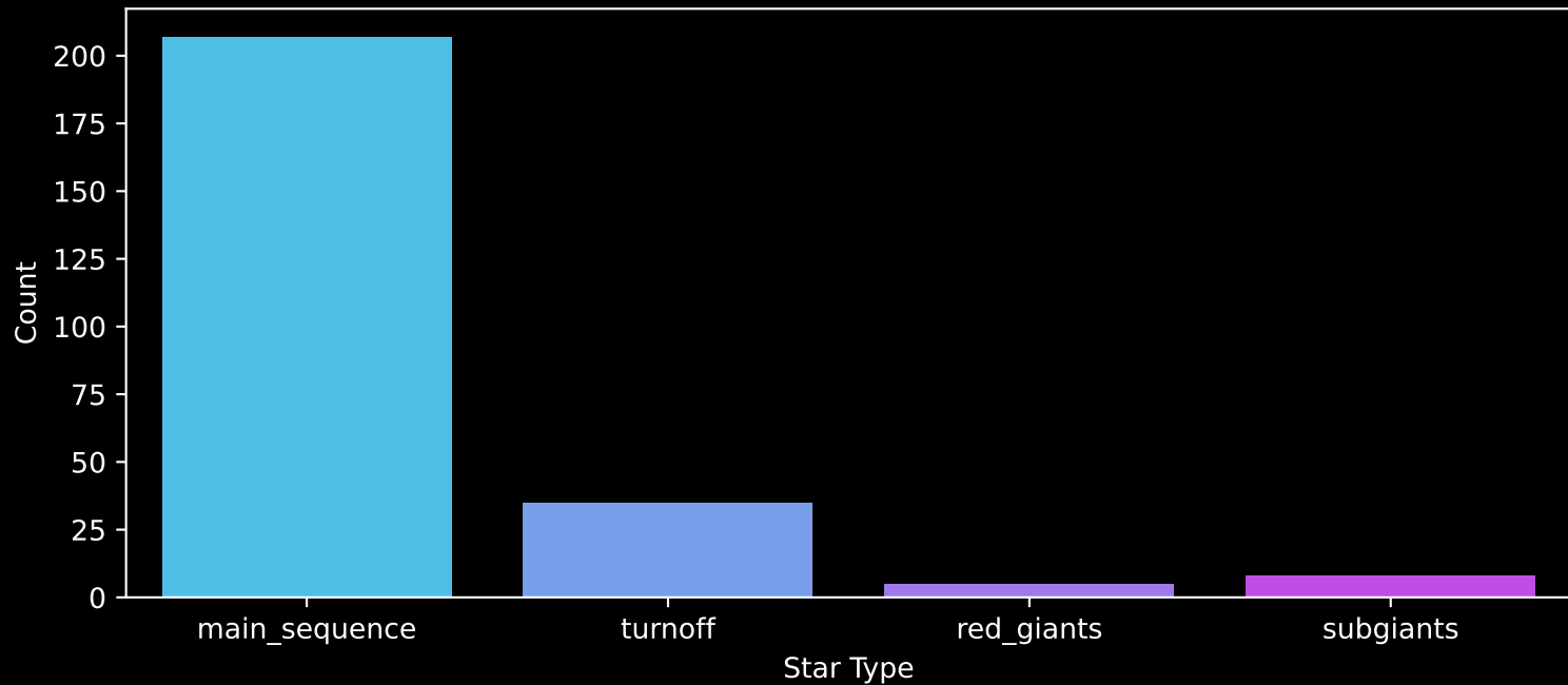
Gaia Cluster: [UPK_594] Count plot of Star Type
