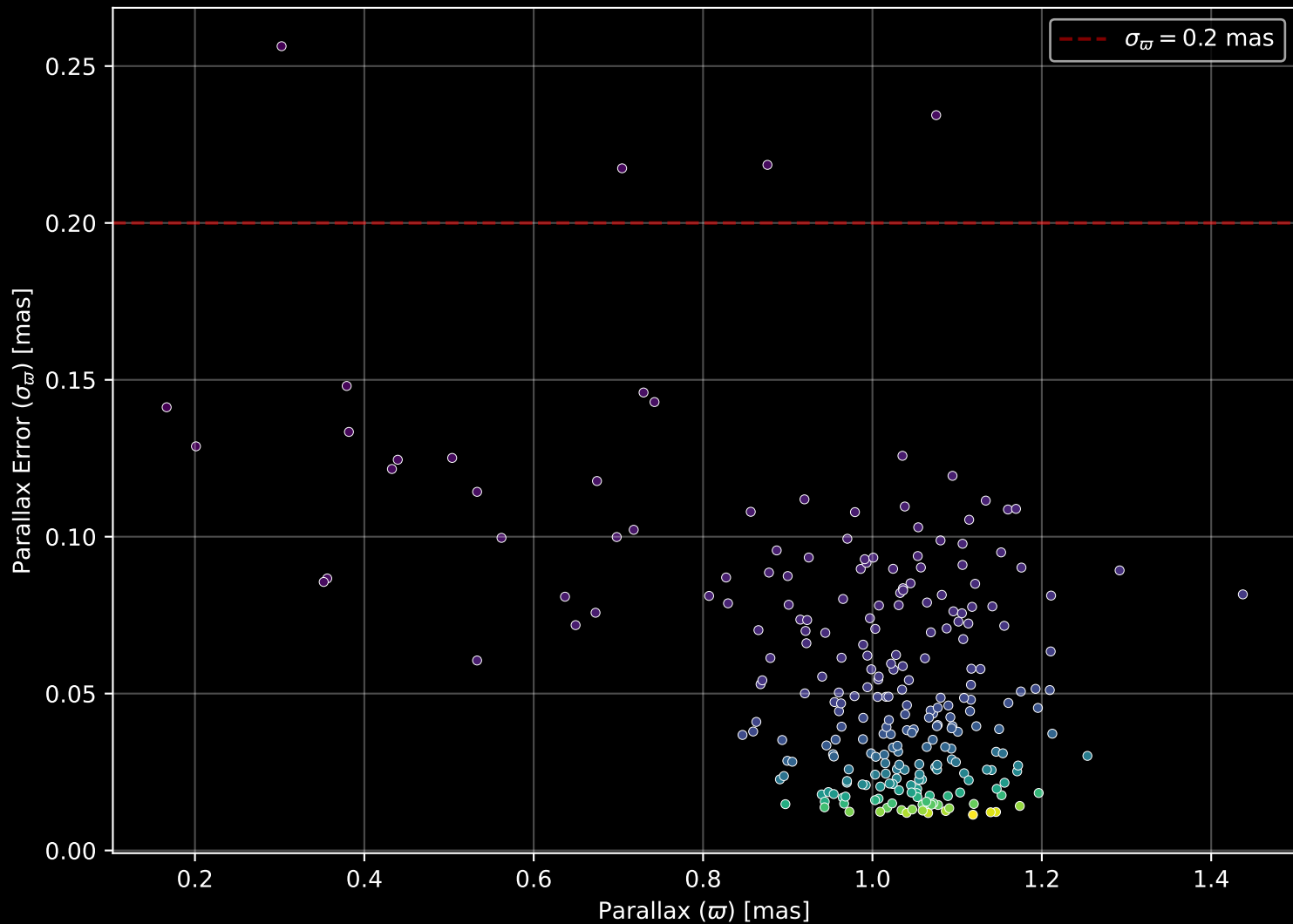
Gaia Cluster: [UPK_594] Parallax Quality (n= 255)
