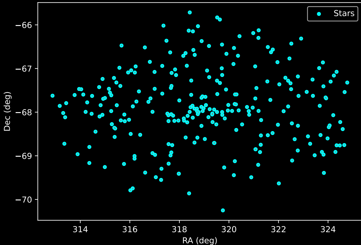
Gaia Cluster: [UPK_594] Proper Motion Vectors for Gaia Star Field (n= 255)
