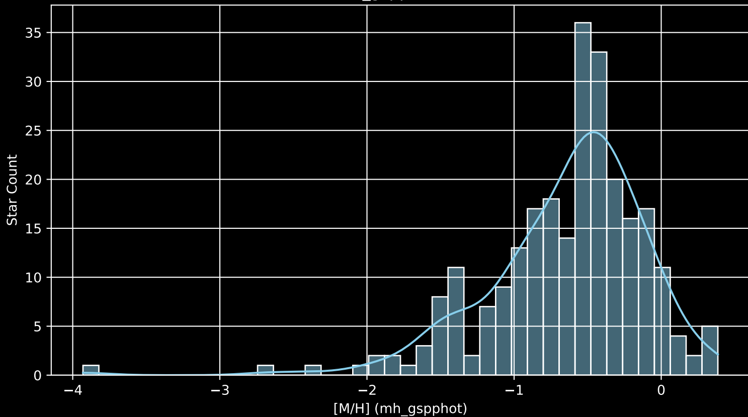
Gaia Cluster: [UPK_594 [M/H] (mh_gspphot) (n= 255)
