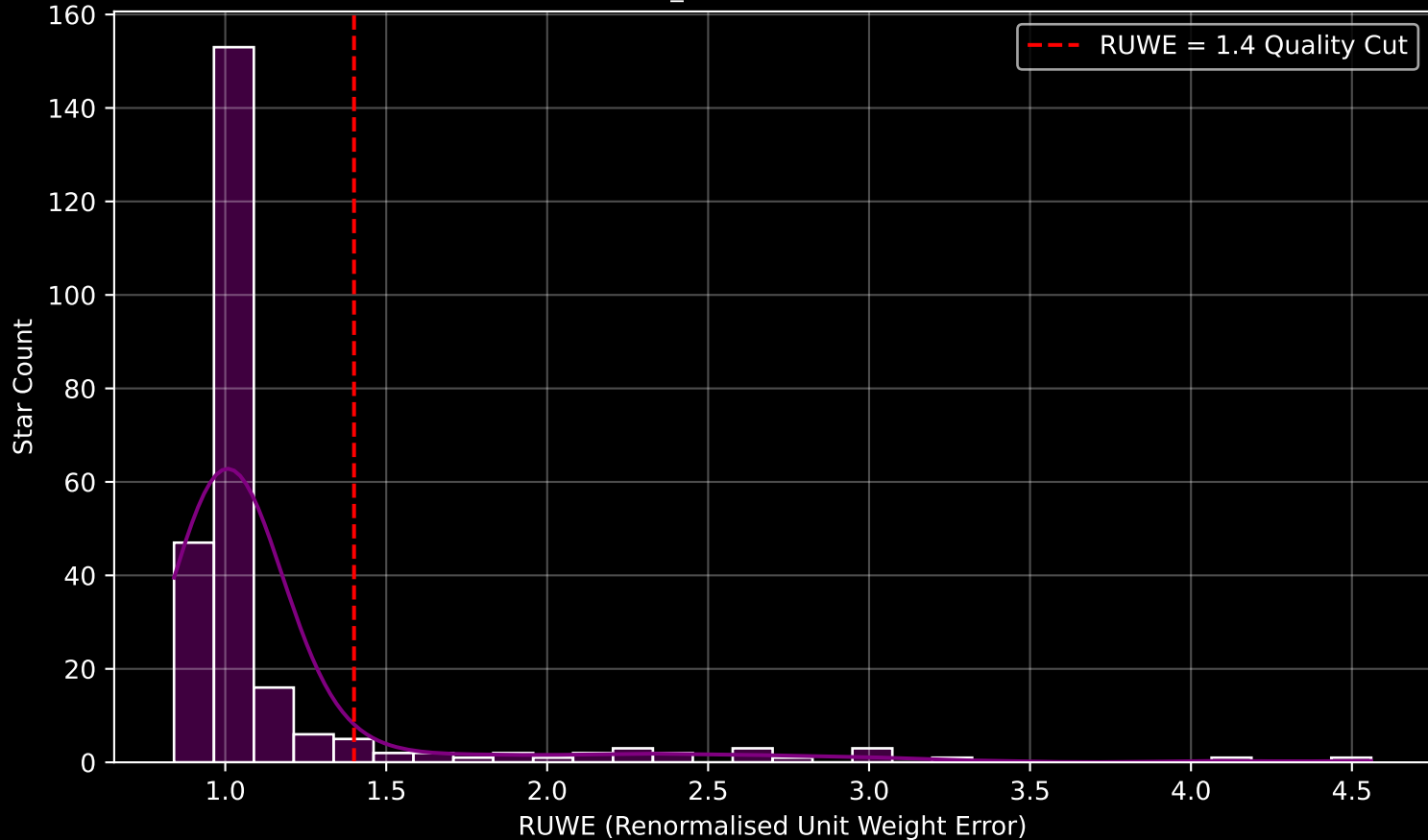
Gaia Cluster: [UPK_594] RUWE Distribution (n= 252)
