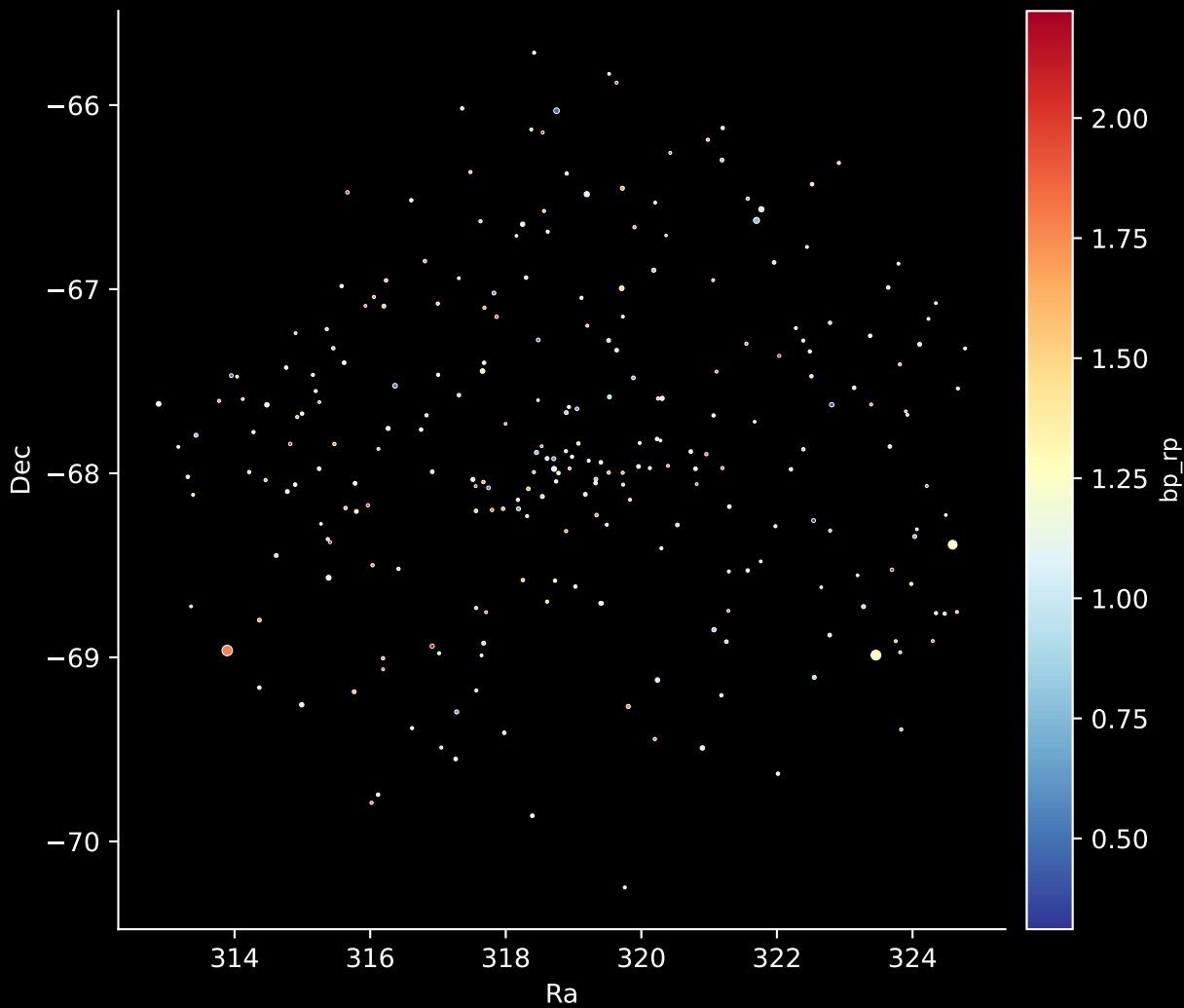
Gaia Cluster: [UPK_594] Stars: 255
