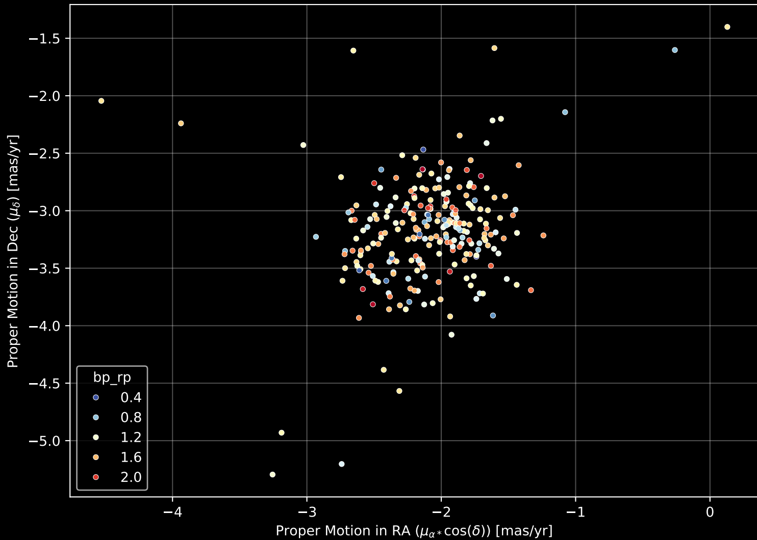
Gaia Cluster: [UPK_594] Proper Motion Diagram (n= 255)
