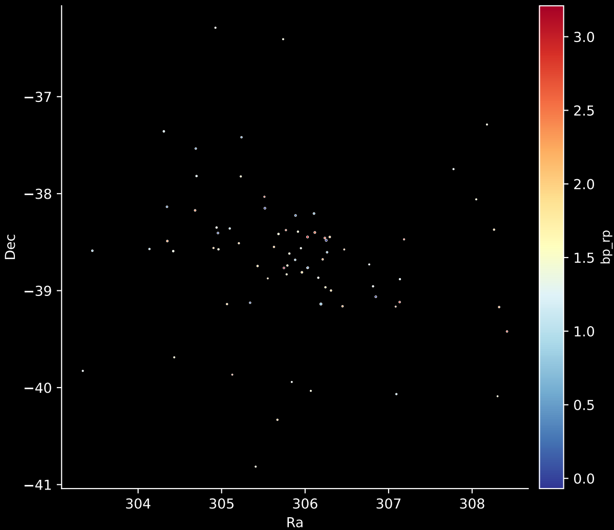
Gaia Cluster: [UPK_599] Stars: 75
