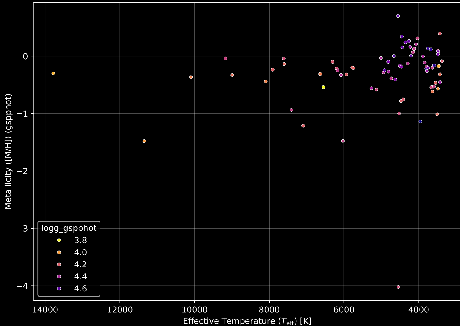
Gaia Cluster: [UPK_599] Stellar Population Parameters (n= 75)
