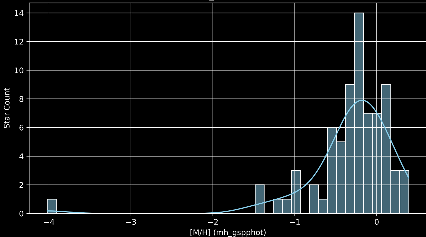
Gaia Cluster: [UPK_599 [M/H] (mh_gspphot) (n= 74)
