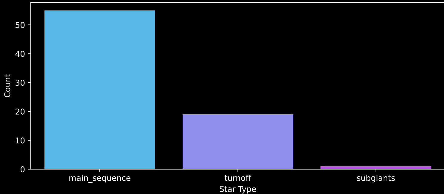
Gaia Cluster: [UPK_599] Count plot of Star Type
