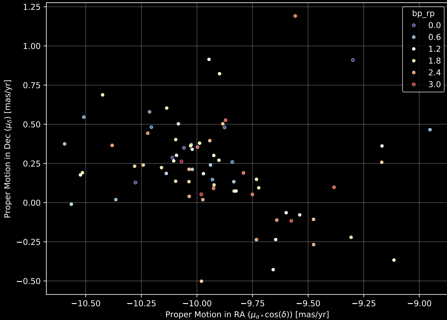
Gaia Cluster: [UPK_599] Proper Motion Diagram (n= 75)
