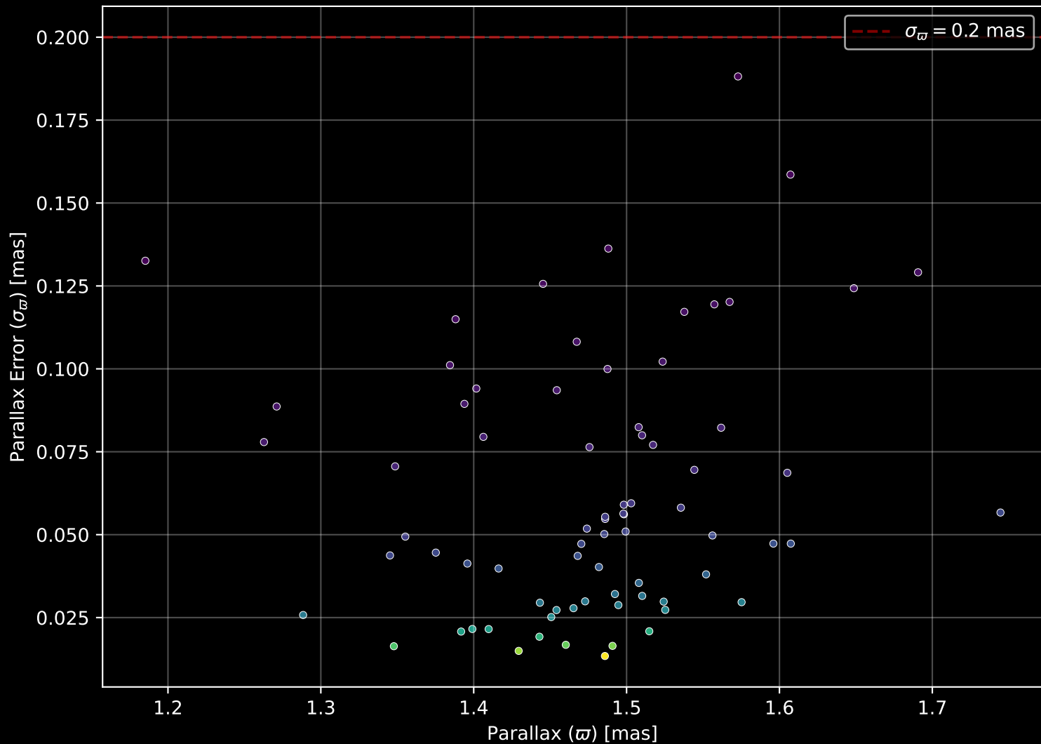
Gaia Cluster: [UPK_599] Parallax Quality (n= 75)
