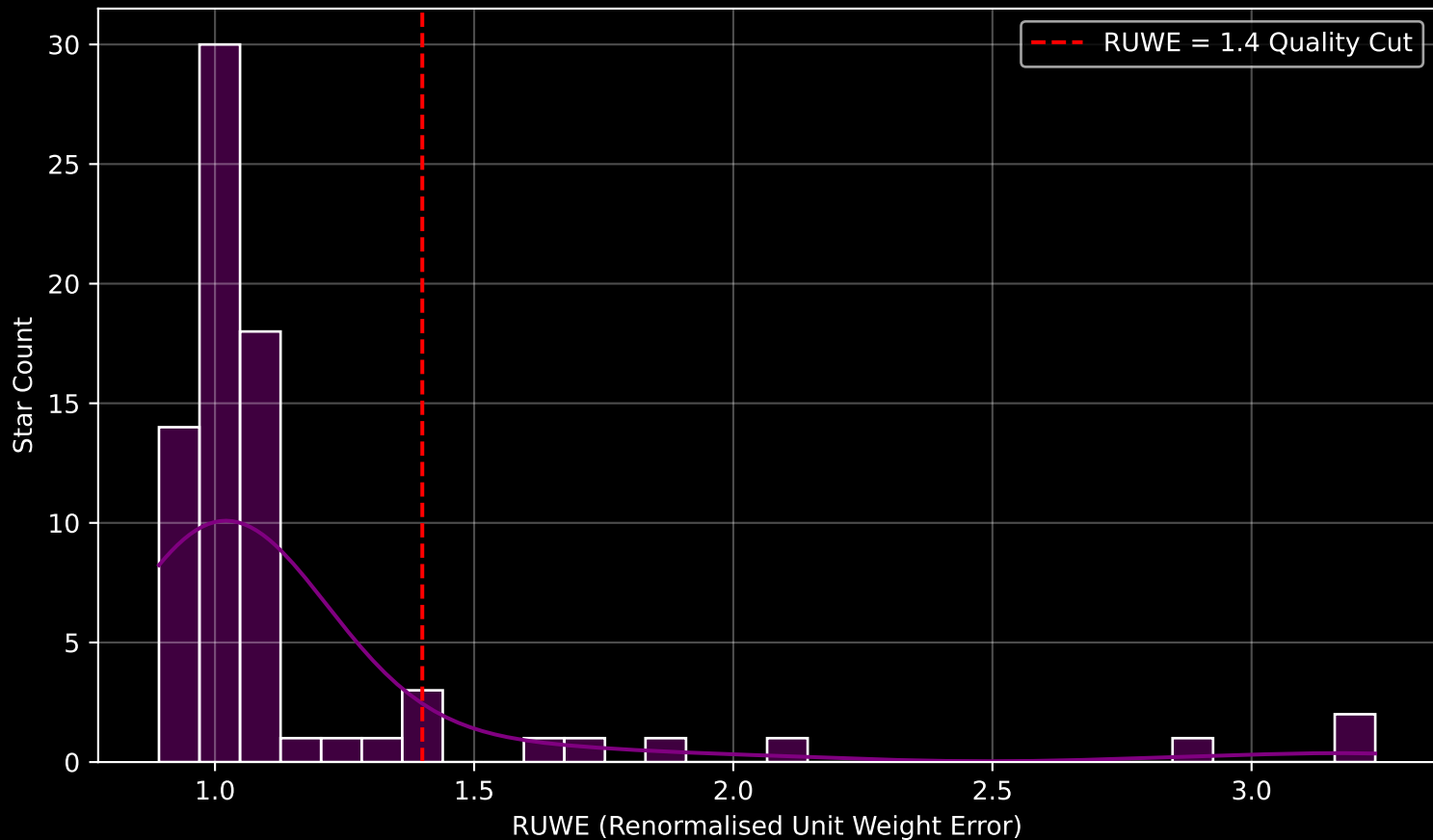
Gaia Cluster: [UPK_599] RUWE Distribution (n= 75)
