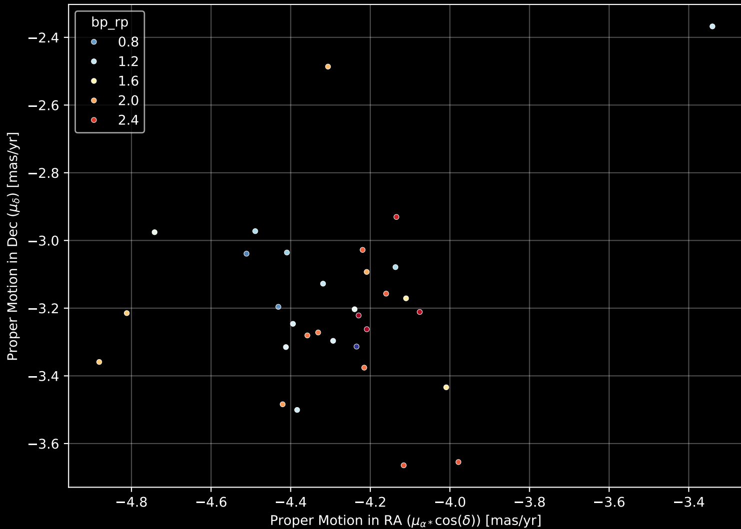
Gaia Cluster: [UPK_607] Proper Motion Diagram (n= 32)
