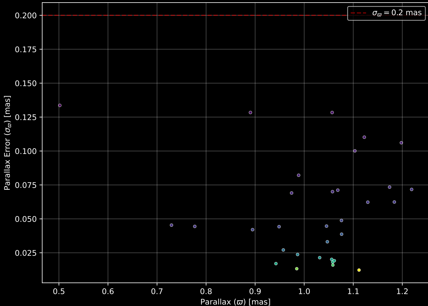
Gaia Cluster: [UPK_607] Parallax Quality (n= 32)
