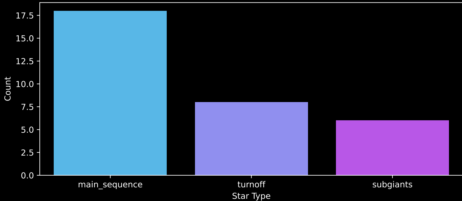
Gaia Cluster: [UPK_607] Count plot of Star Type
