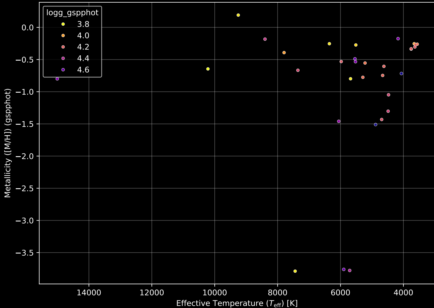
Gaia Cluster: [UPK_607] Stellar Population Parameters (n= 32)
