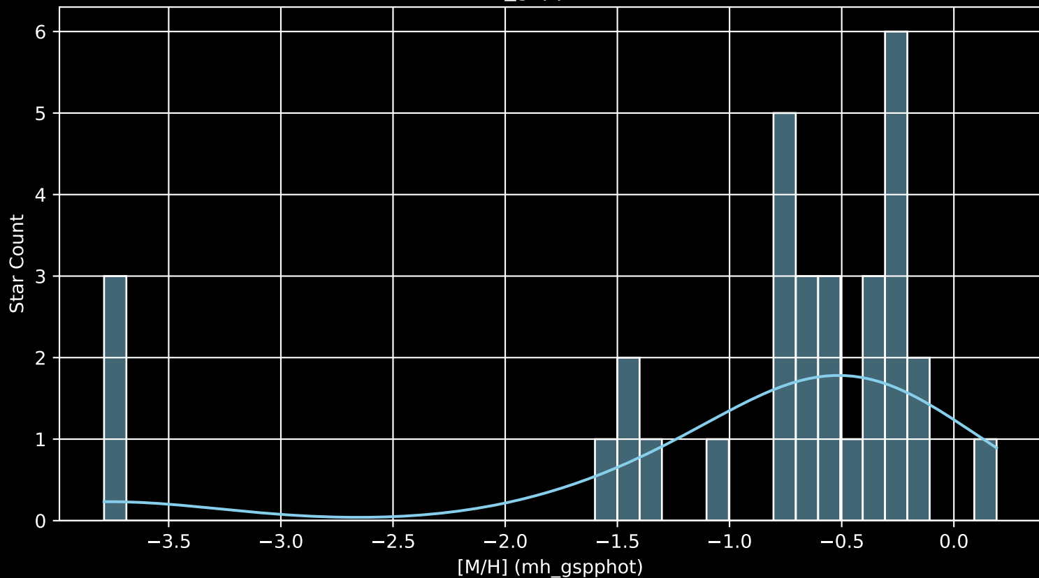
Gaia Cluster: [UPK_607 [M/H] (mh_gspphot) (n= 32)
