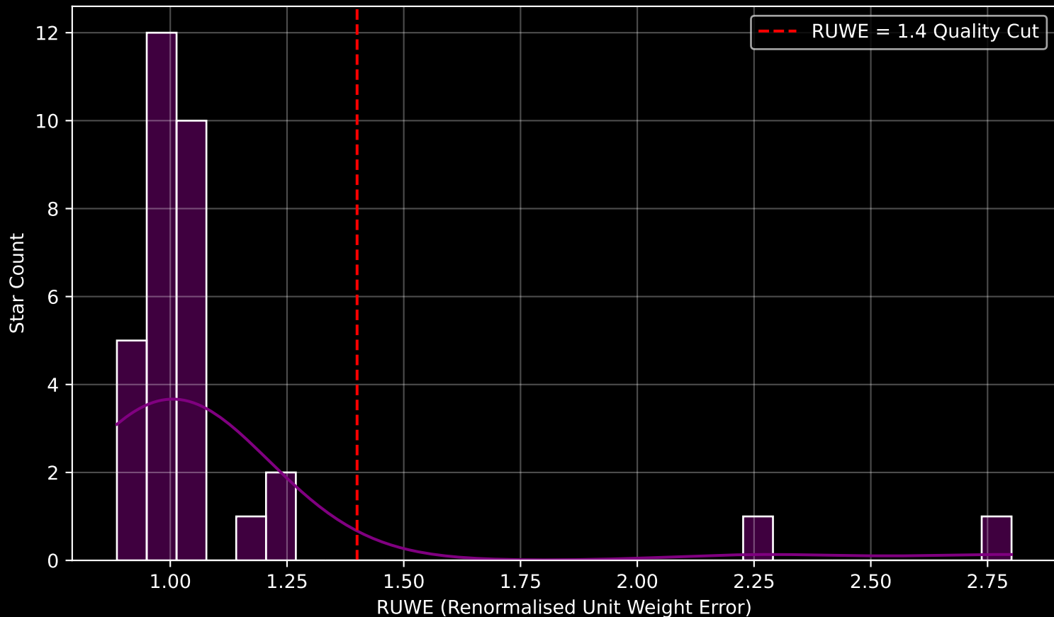
Gaia Cluster: [UPK_607] RUWE Distribution (n= 32)
