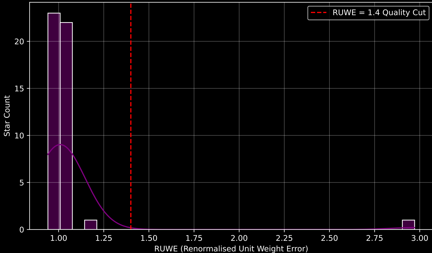
Gaia Cluster: [UPK_62] RUWE Distribution (n= 47)
