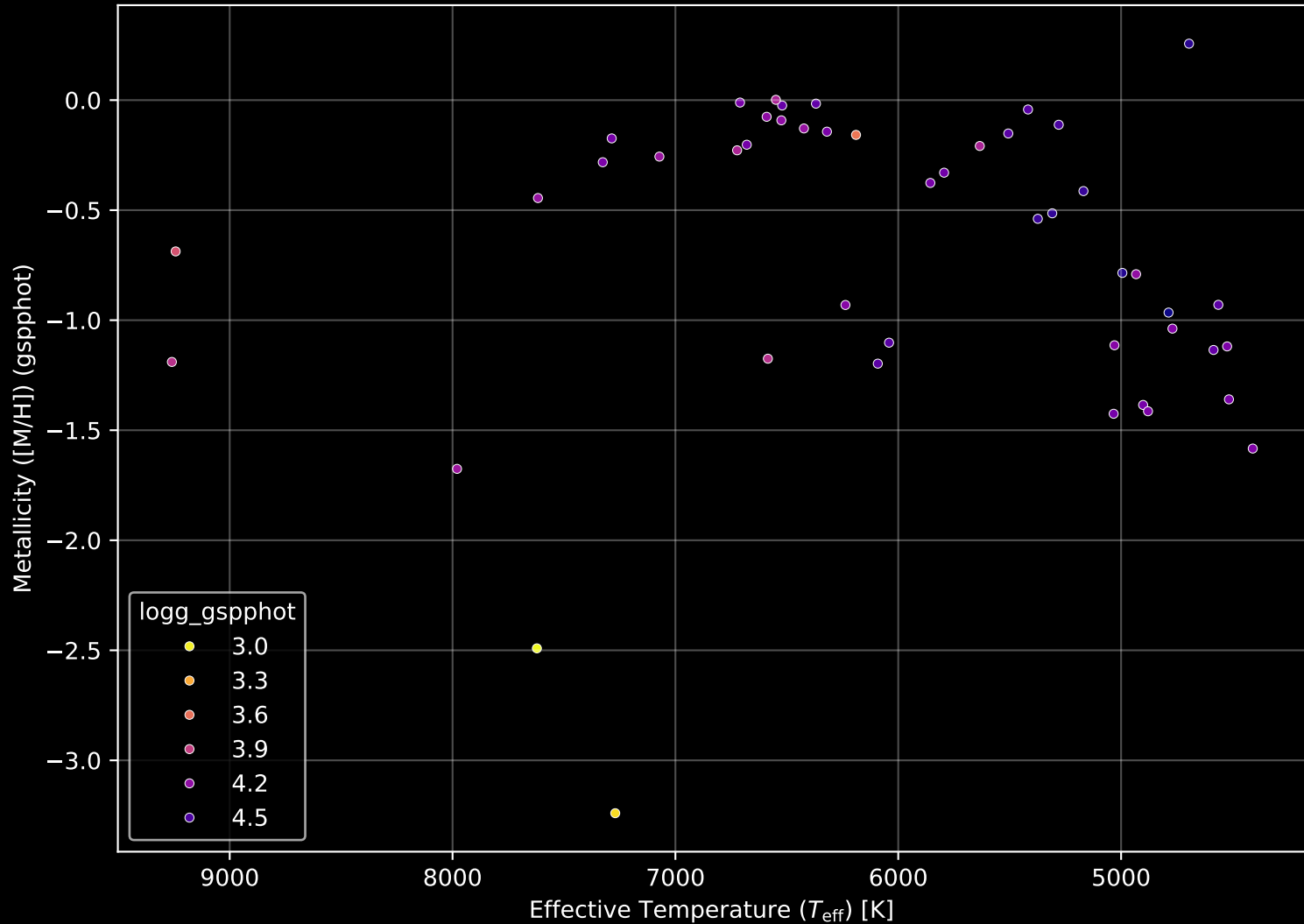
Gaia Cluster: [UPK_62] Stellar Population Parameters (n= 47)
