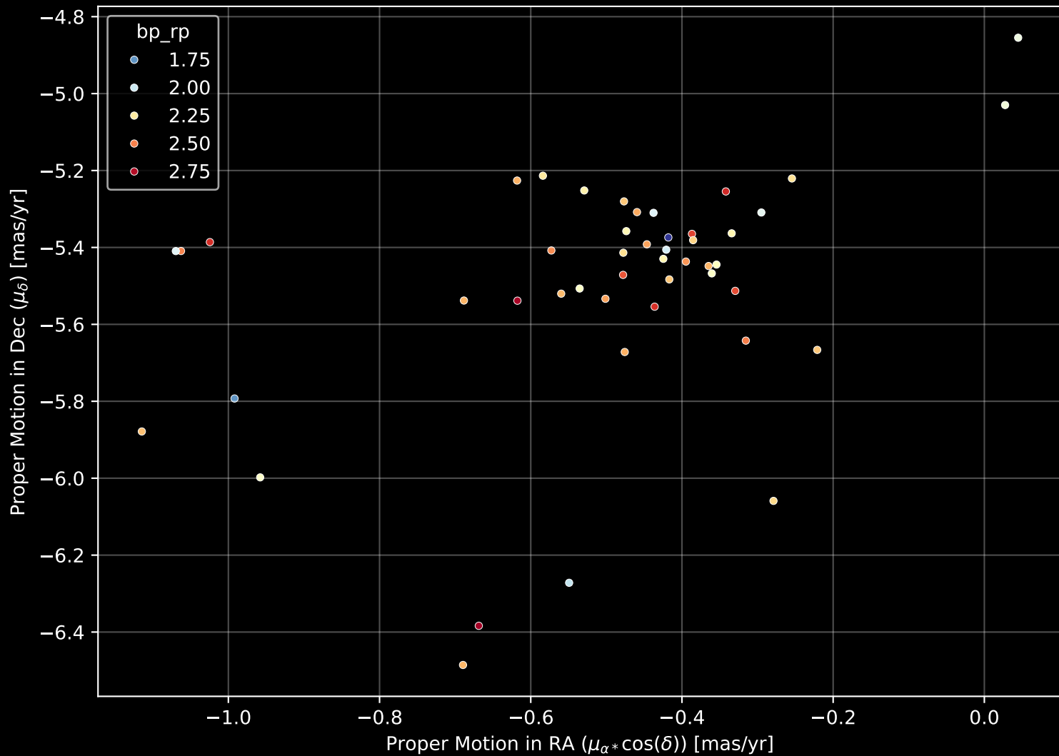
Gaia Cluster: [UPK_62] Proper Motion Diagram (n= 47)
