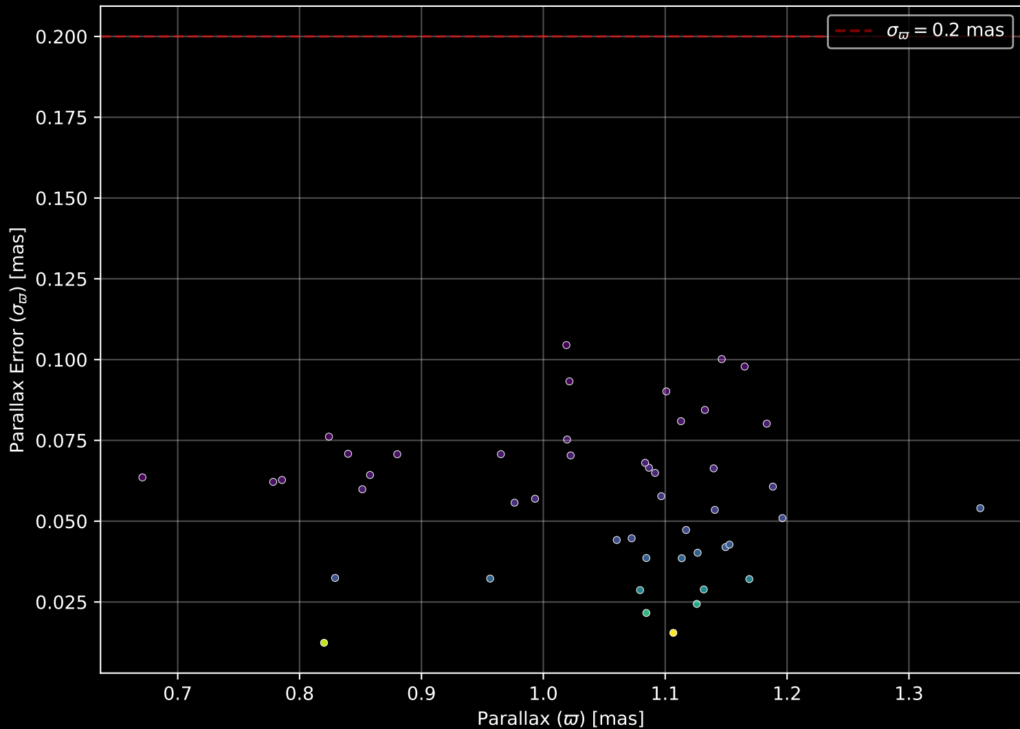
Gaia Cluster: [UPK_62] Parallax Quality (n= 47)
