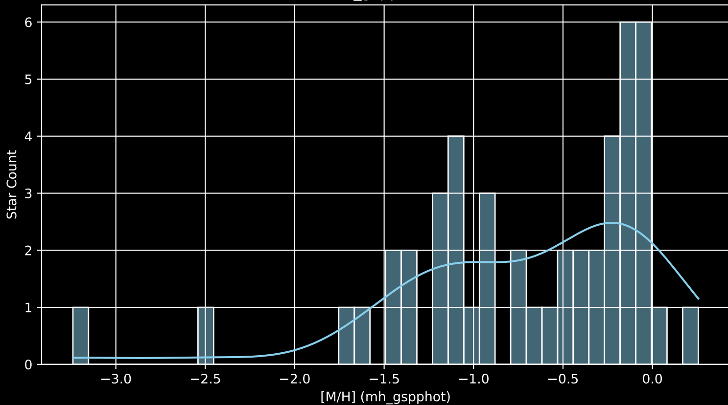
Gaia Cluster: [UPK_62 [M/H] (mh_gspphot) ( \bar{n}= 47 )
