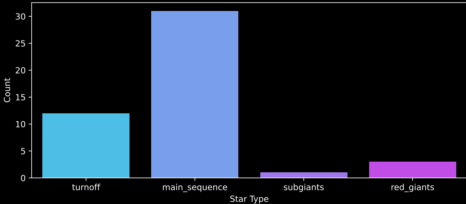
Gaia Cluster: [UPK_62] Count plot of Star Type
