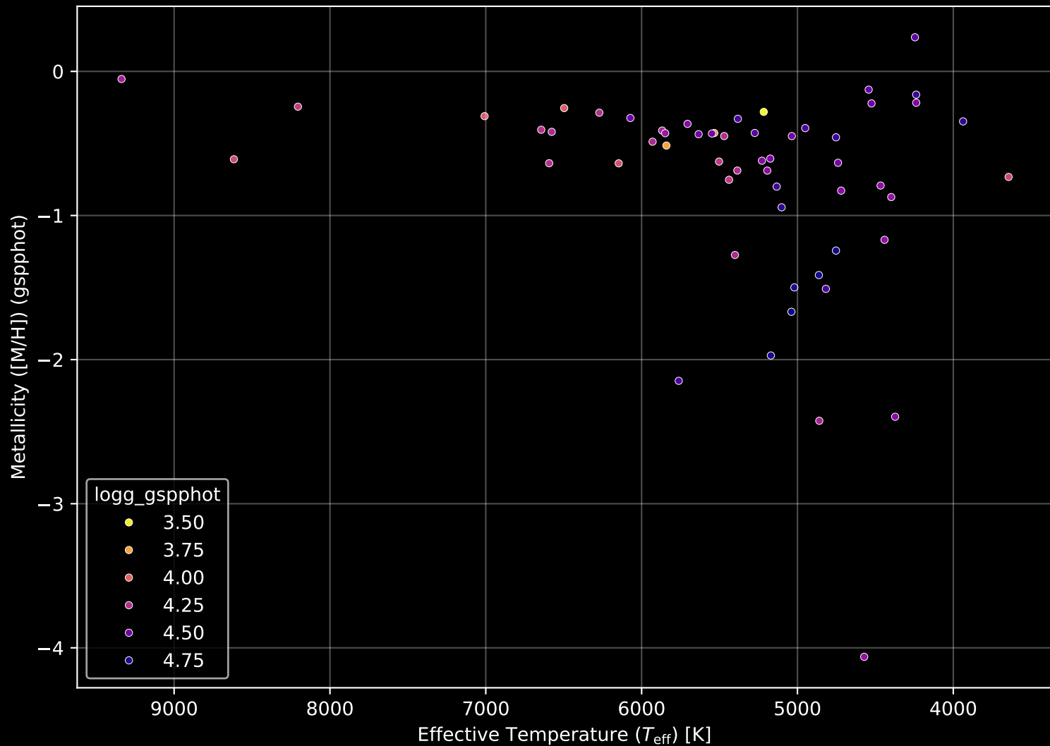
Gaia Cluster: [UPK_630] Stellar Population Parameters (n= 57)
