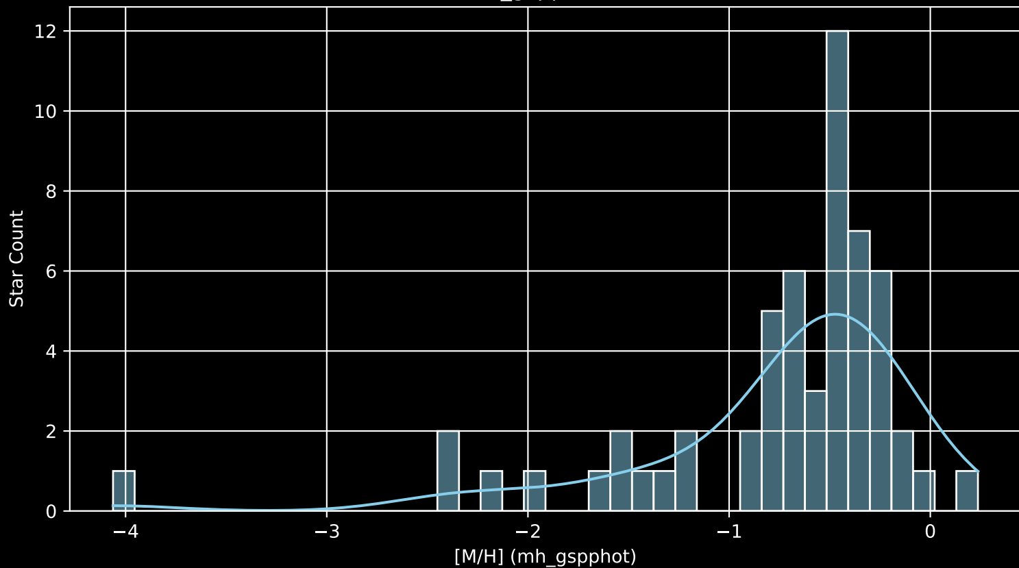
Gaia Cluster: [UPK_630 [M/H] (mh_gspphot) (n= 57)
