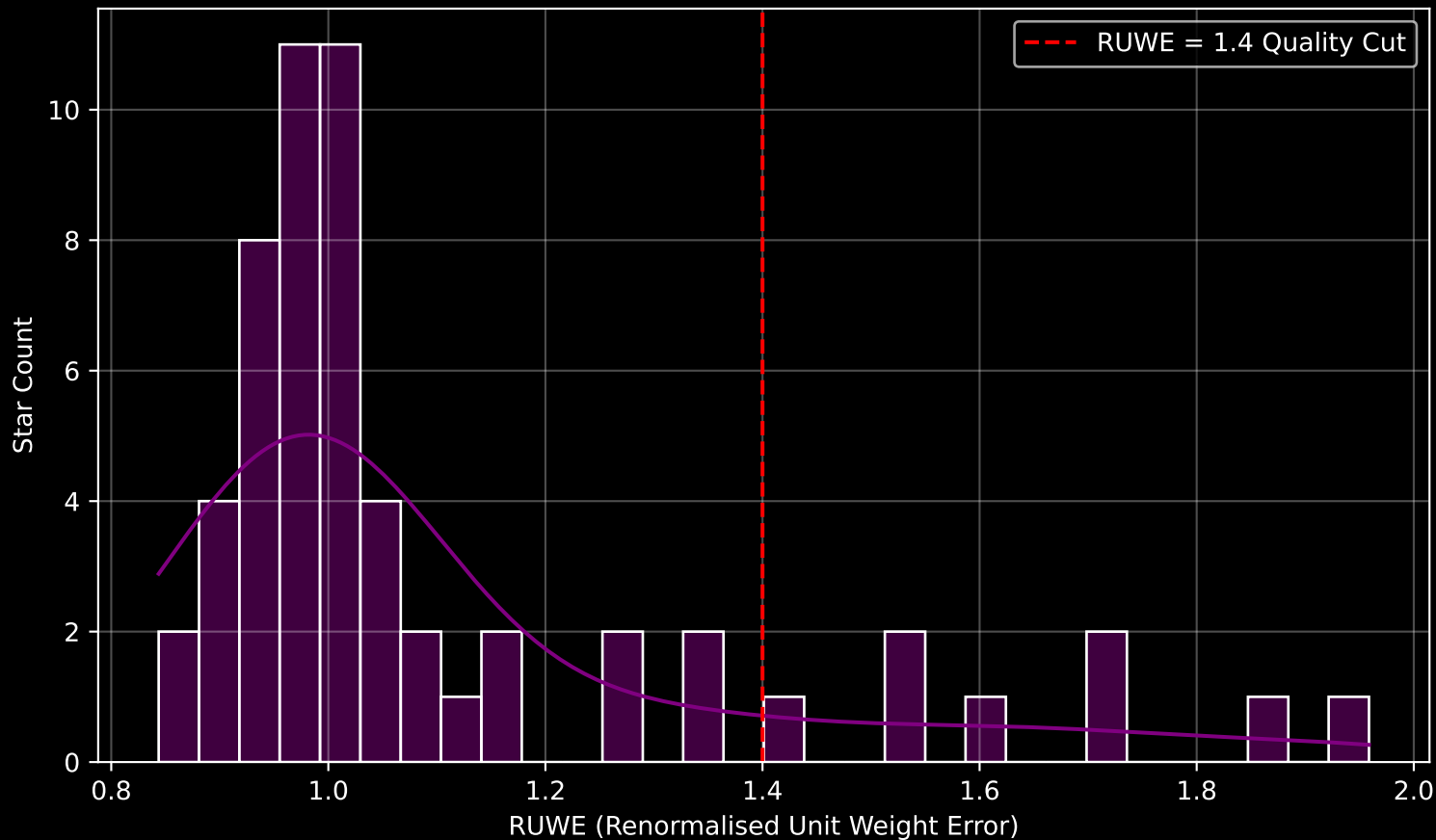
Gaia Cluster: [UPK_630] RUWE Distribution (n= 57)
