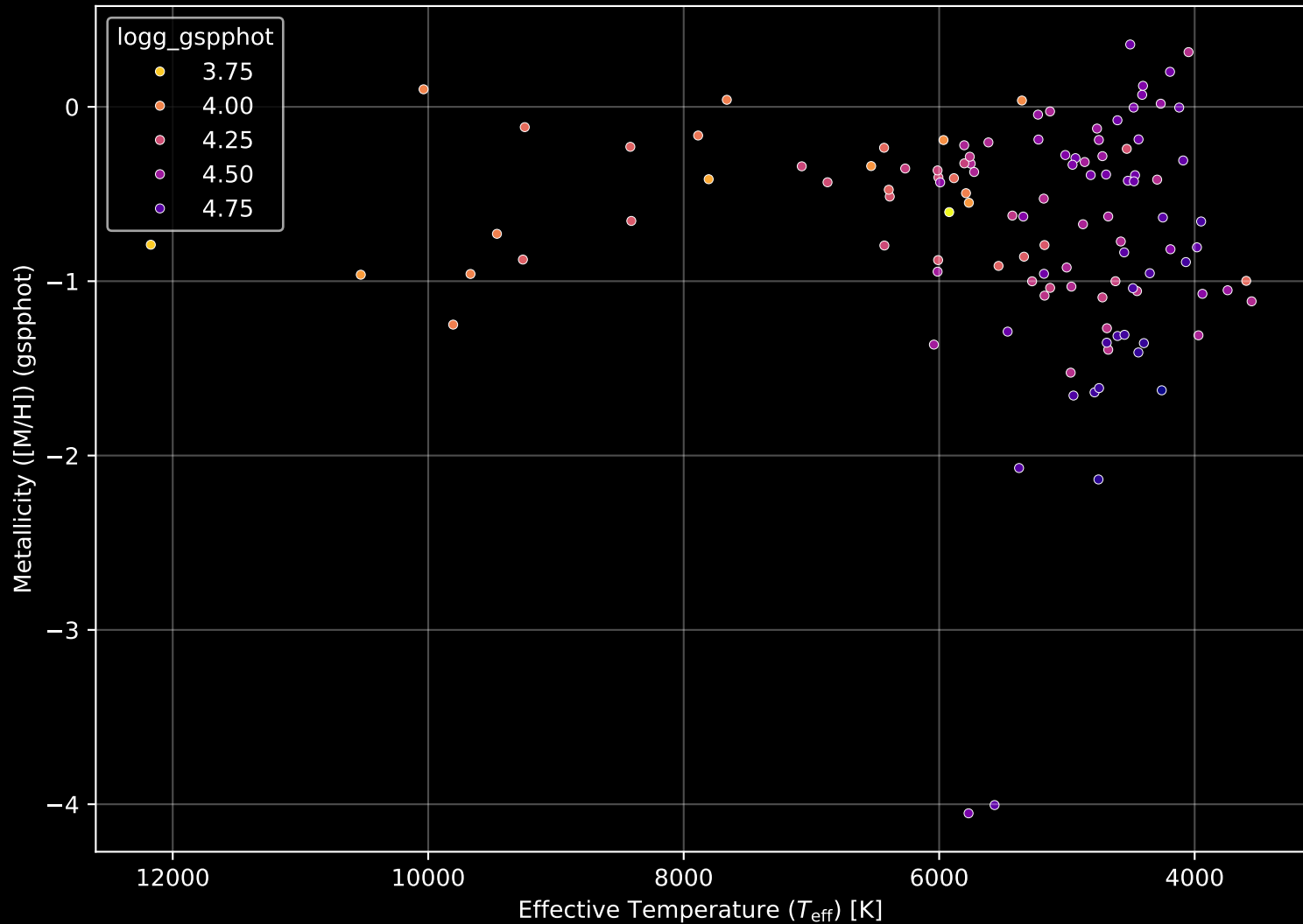
Gaia Cluster: [UPK_642] Stellar Population Parameters (n= 115)
