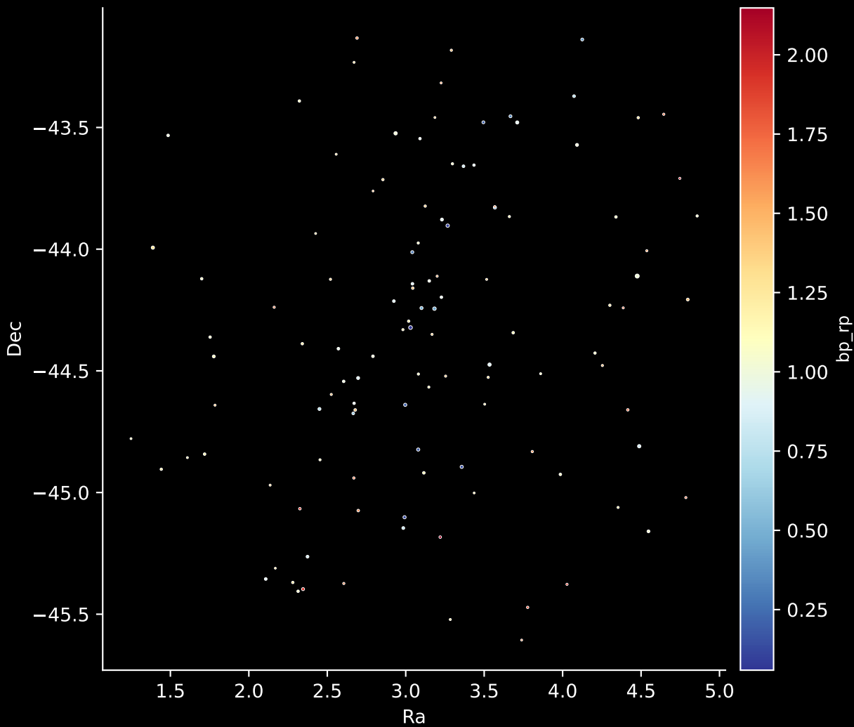
Gaia Cluster: [UPK_642] Stars: 115
