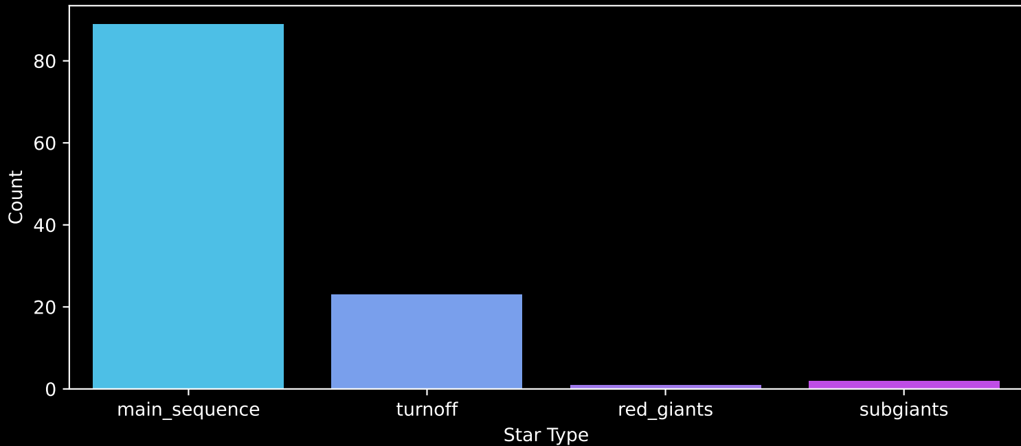
Gaia Cluster: [UPK_642] Count plot of Star Type
