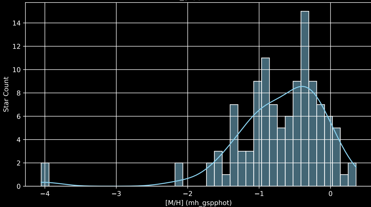
Gaia Cluster: [UPK_642 [M/H] (mh_gspphot) (n= 115)
