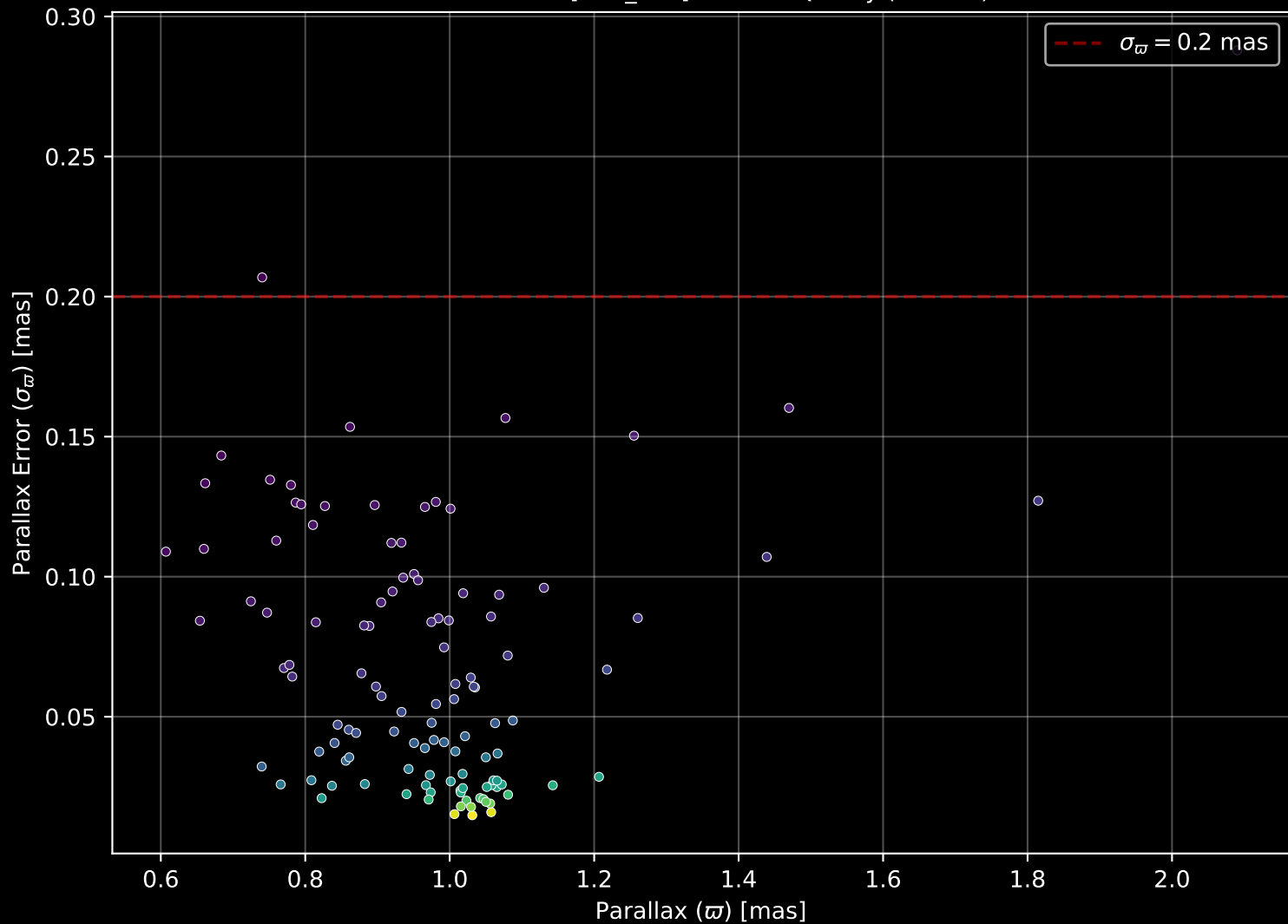
Gaia Cluster: [UPK_642] Parallax Quality (n= 115)
