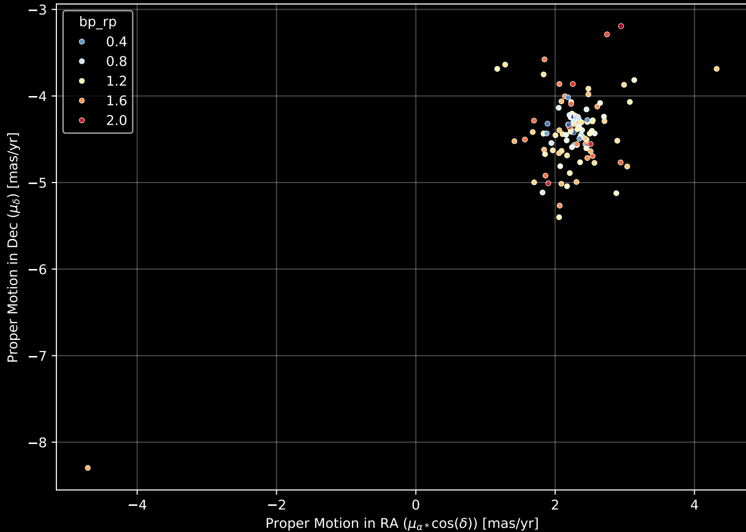
Gaia Cluster: [UPK_642] Proper Motion Diagram (n= 115)
