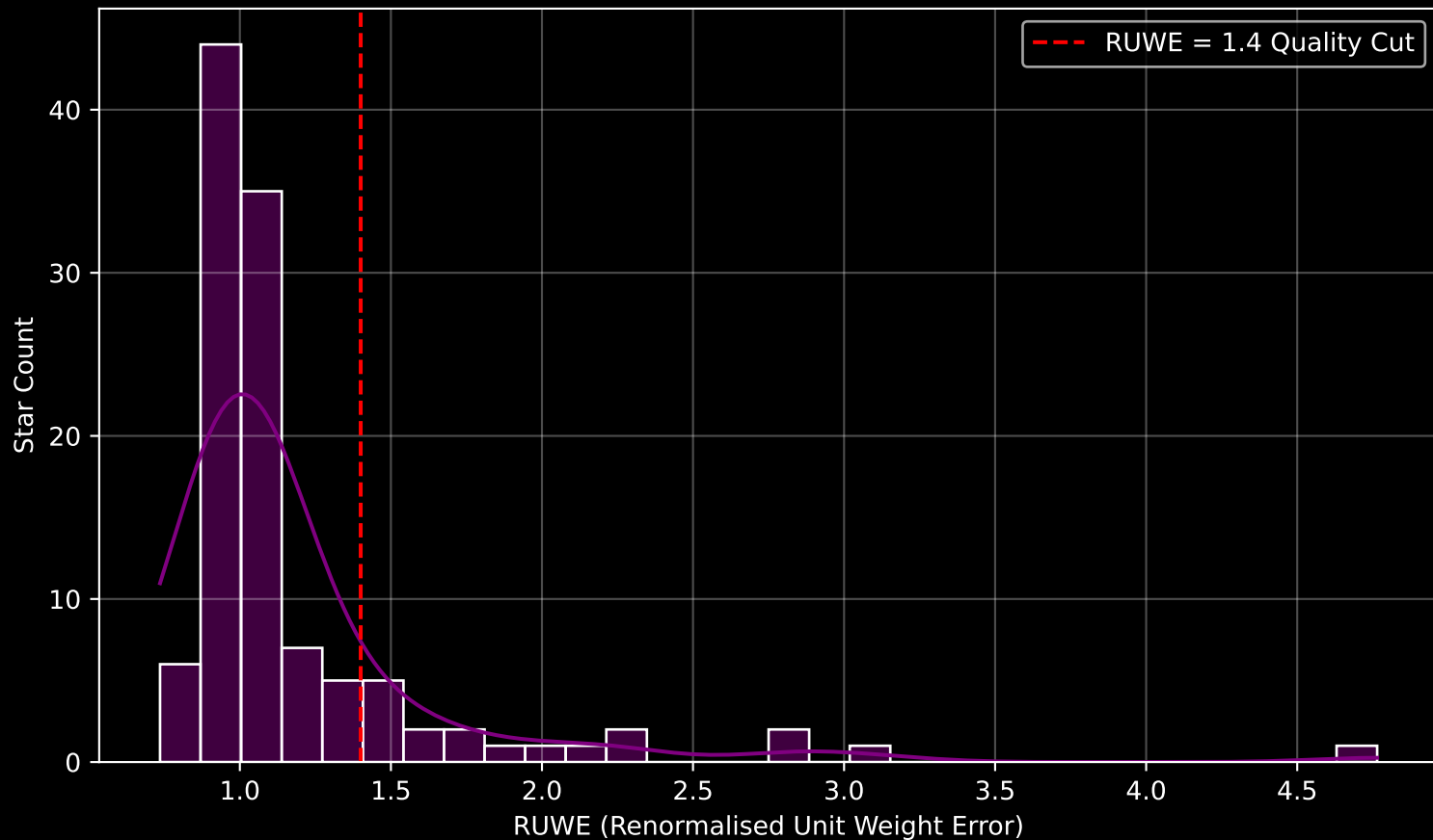
Gaia Cluster: [UPK_642] RUWE Distribution (n= 115)
