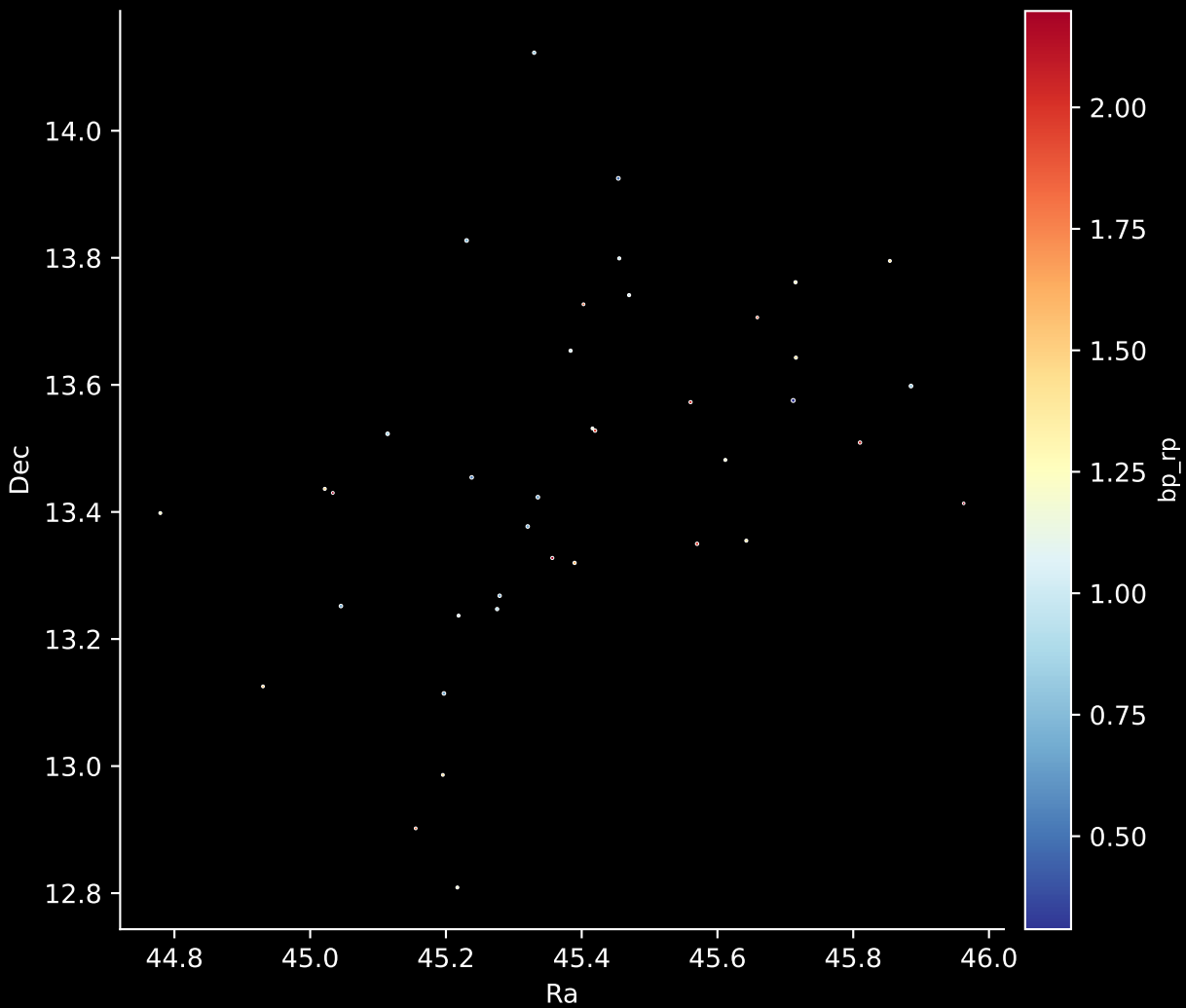
Gaia Cluster: [UPK_66] Stars: 39
