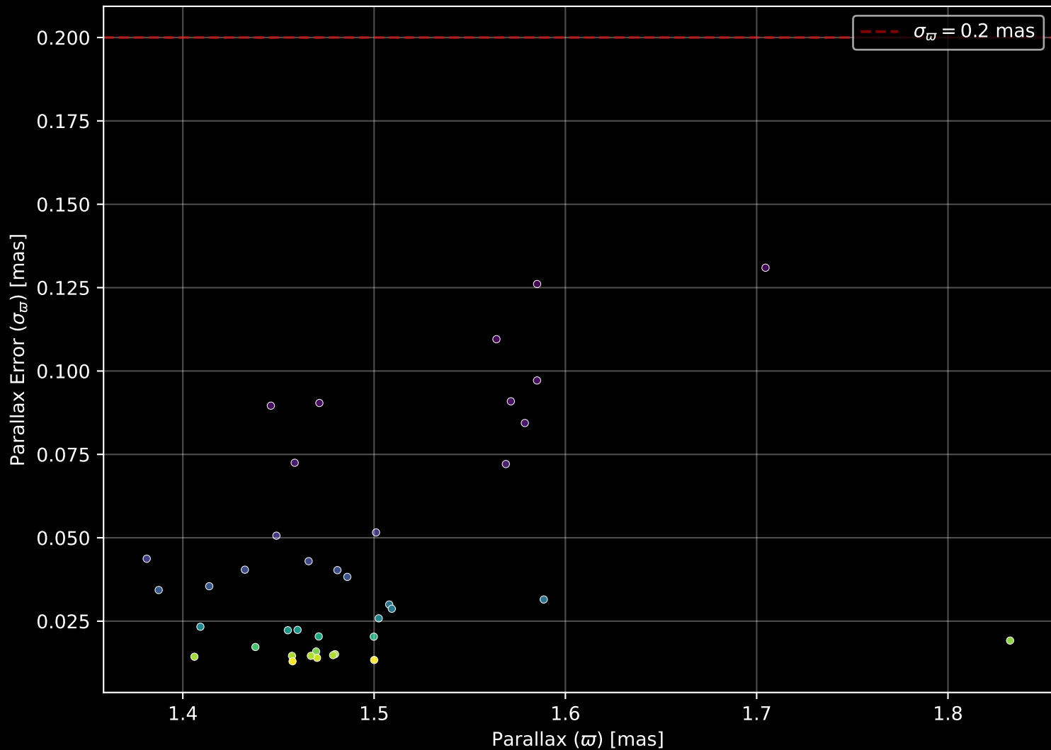
Gaia Cluster: [UPK_66] Parallax Quality (n= 39)
