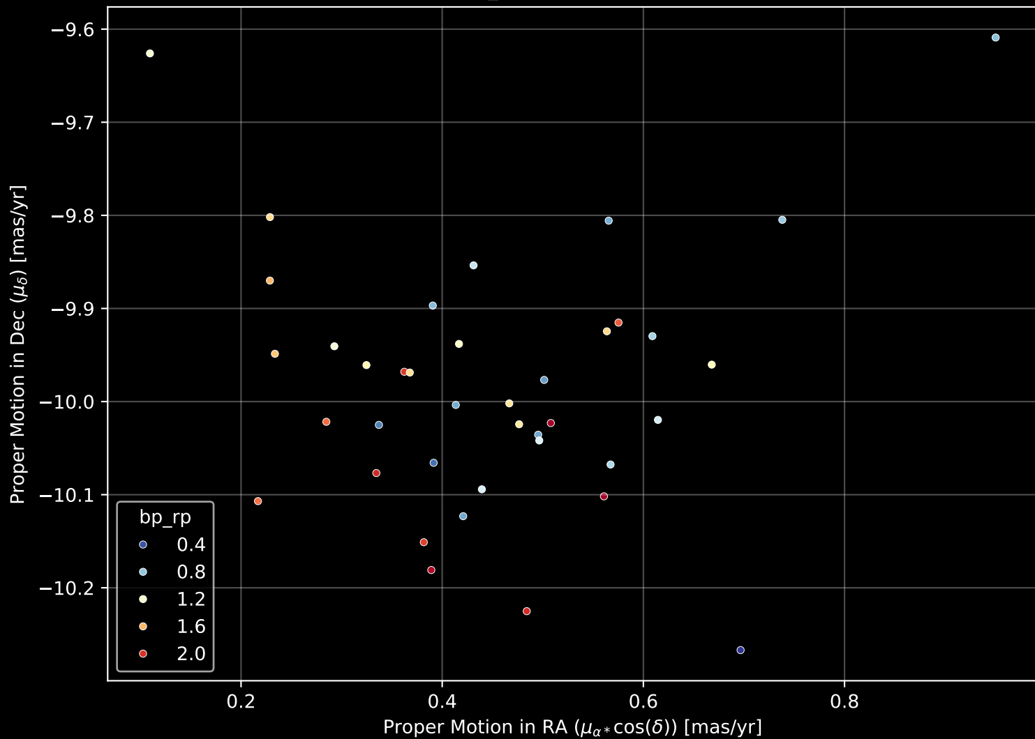
Gaia Cluster: [UPK_66] Proper Motion Diagram (n= 39)
