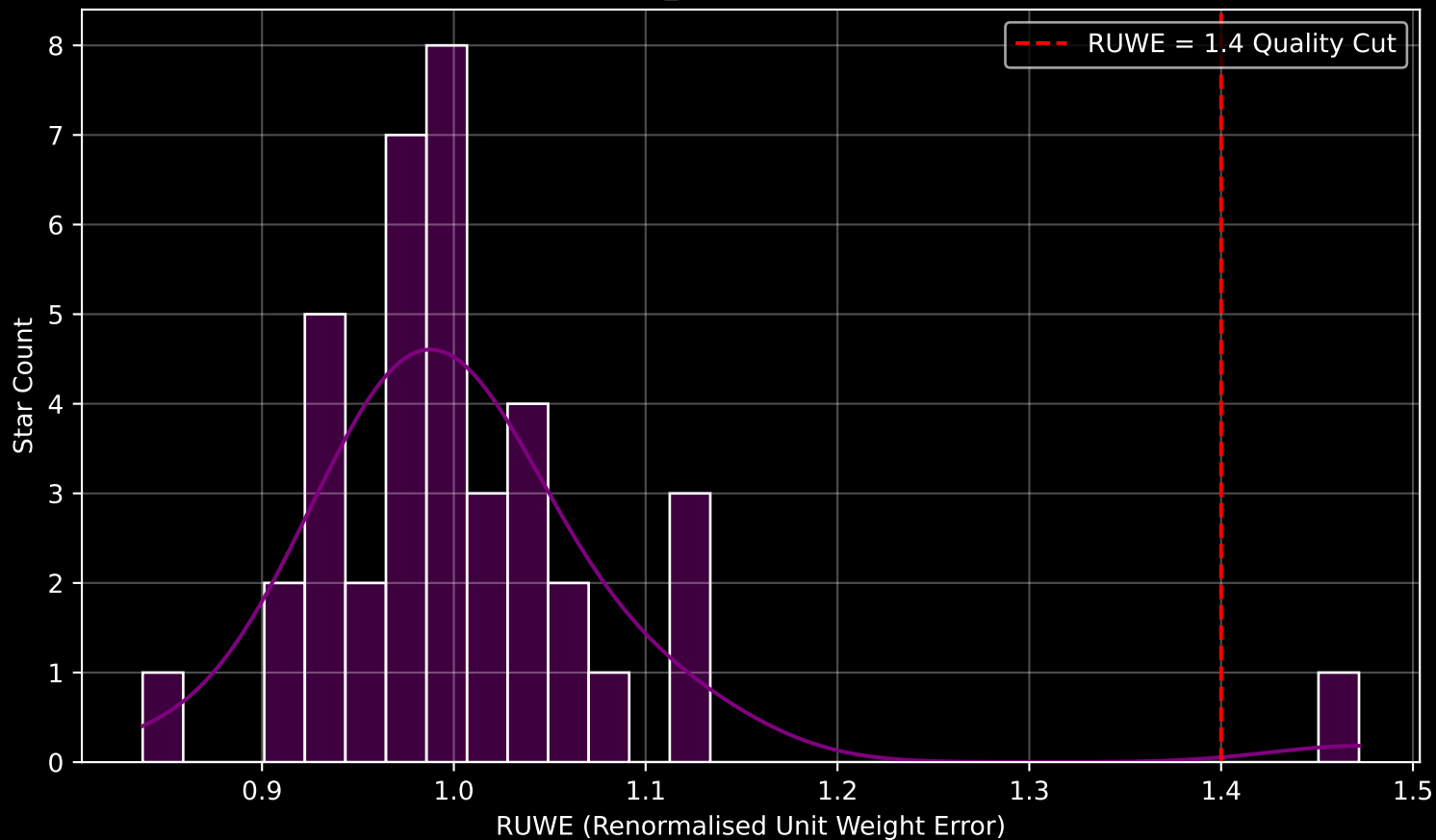
Gaia Cluster: [UPK_66] RUWE Distribution (n= 39)
