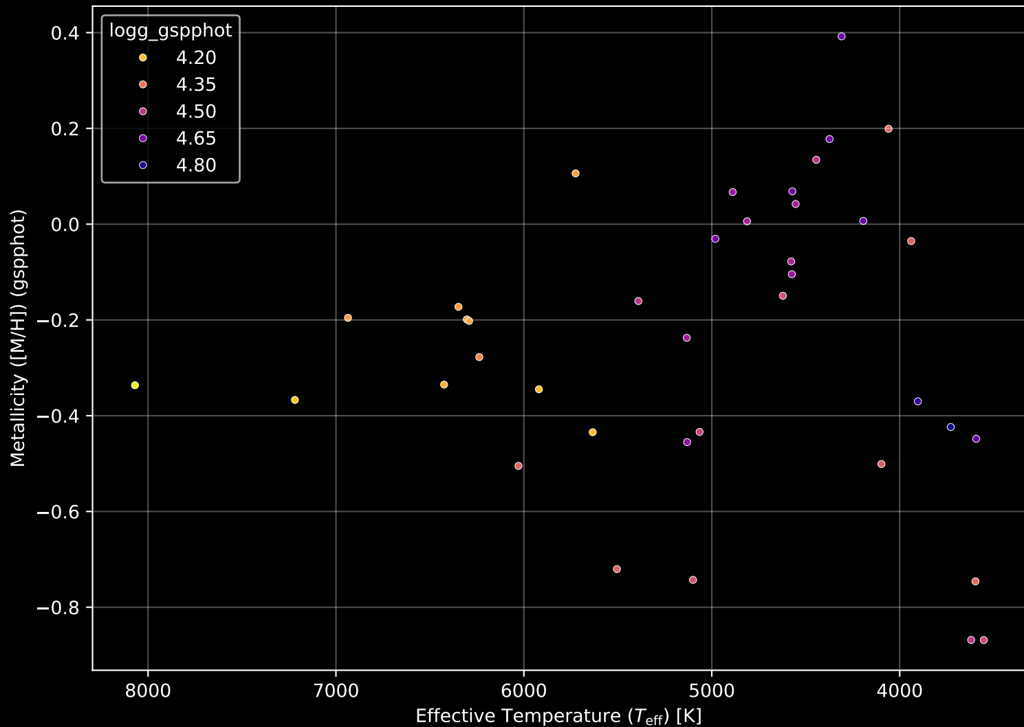
Gaia Cluster: [UPK_66] Stellar Population Parameters (n= 39)
