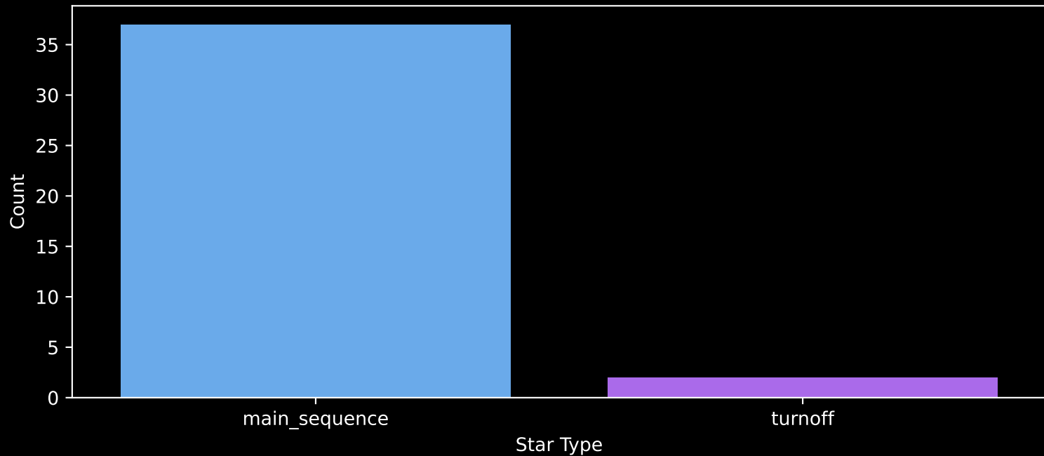
Gaia Cluster: [UPK_66] Count plot of Star Type
