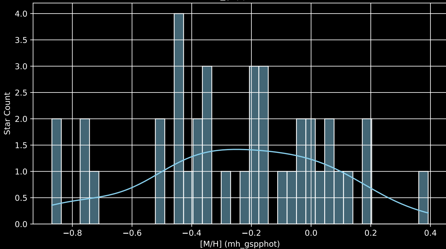
Gaia Cluster: [UPK_66 [M/H] (mh_gspphot) (n= 39)
