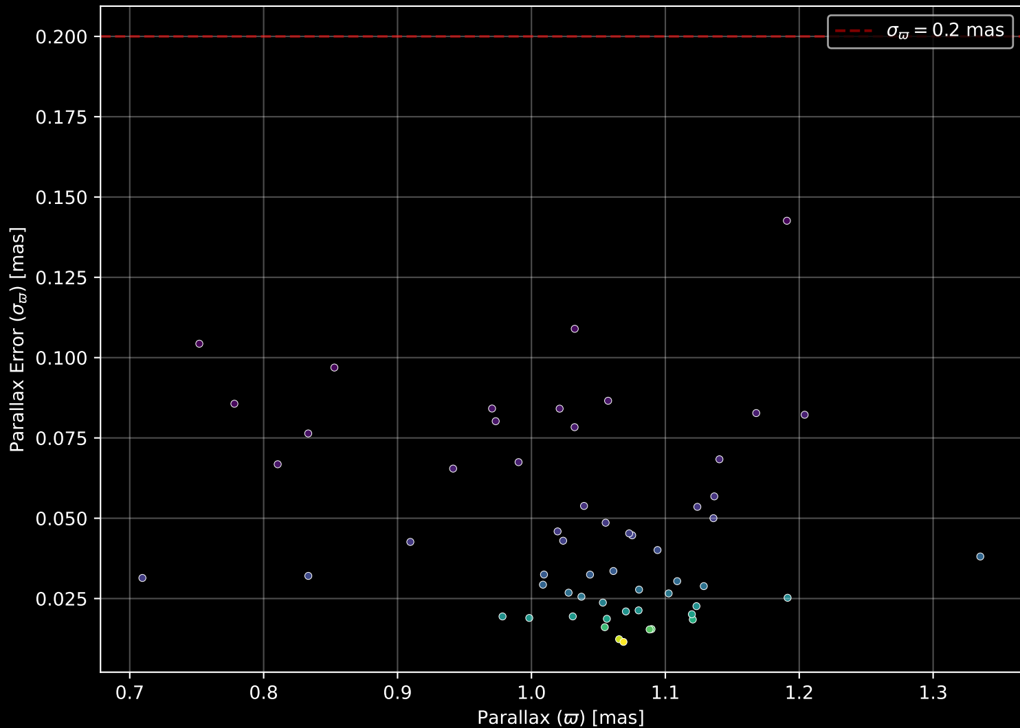
Gaia Cluster: [UPK_79] Parallax Quality (n= 57)
