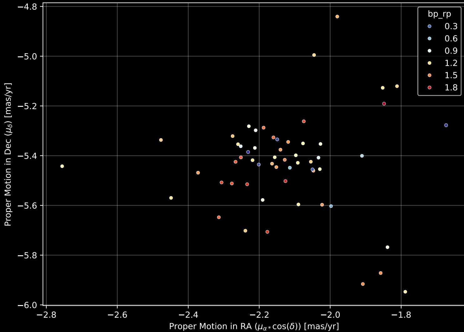
Gaia Cluster: [UPK_79] Proper Motion Diagram (n= 57)
