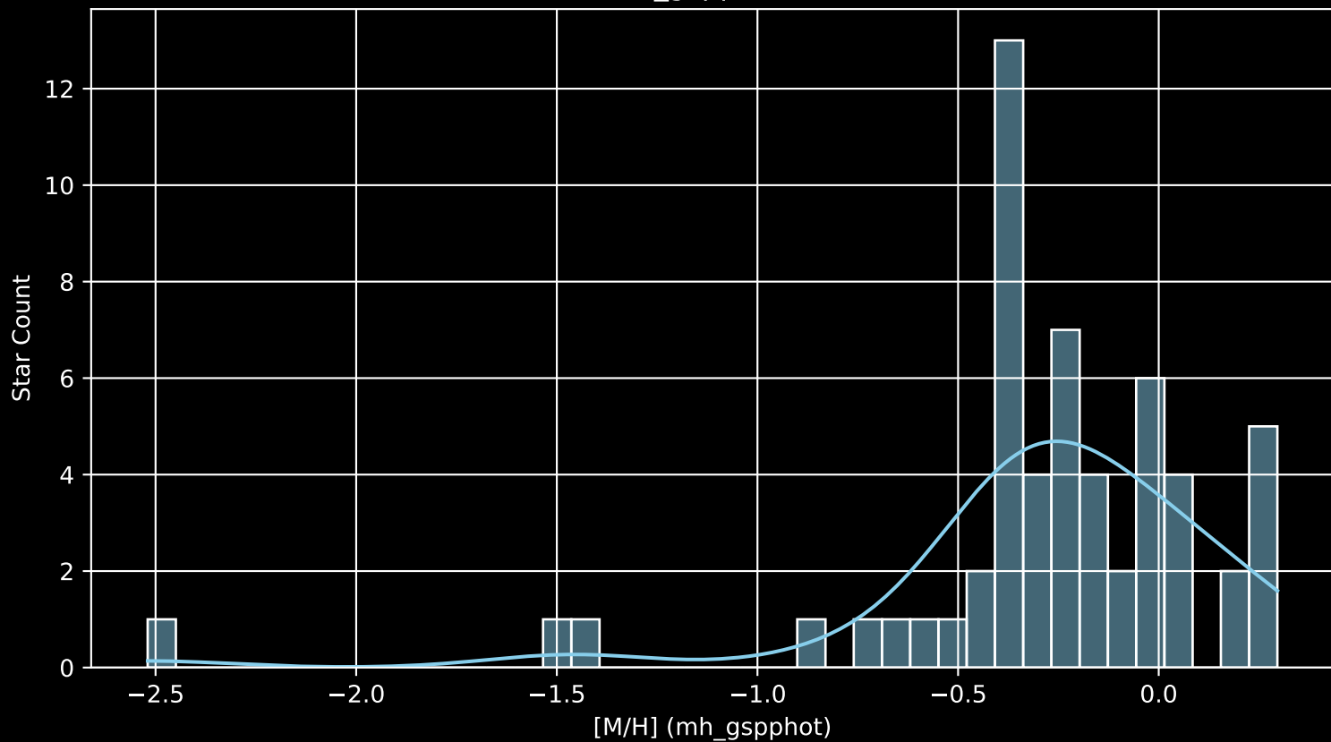
Gaia Cluster: [UPK_79 [M/H] (mh_gspphot) (n= 57)
