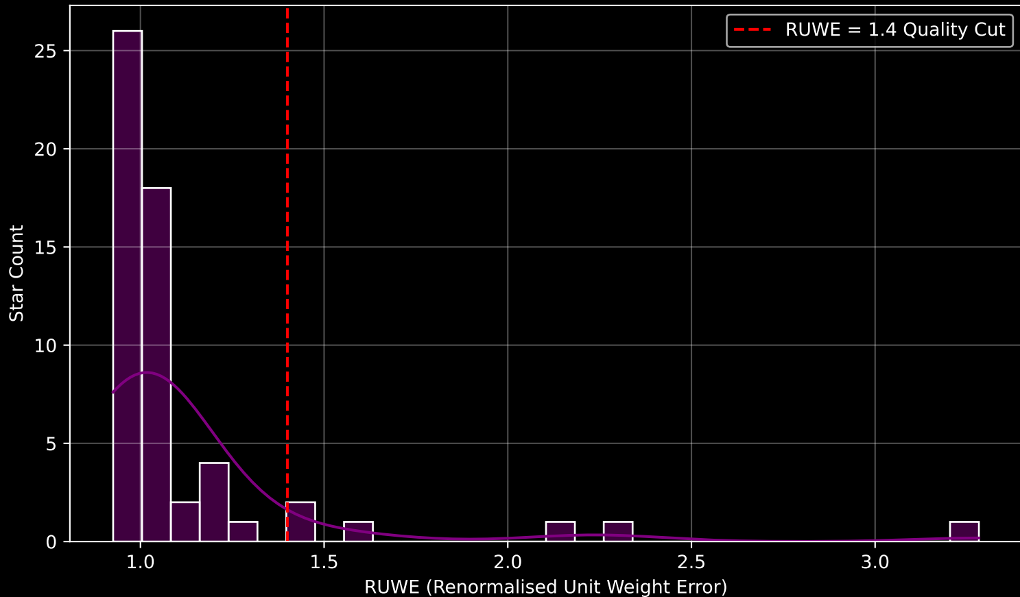
Gaia Cluster: [UPK_79] RUWE Distribution (n= 57)
