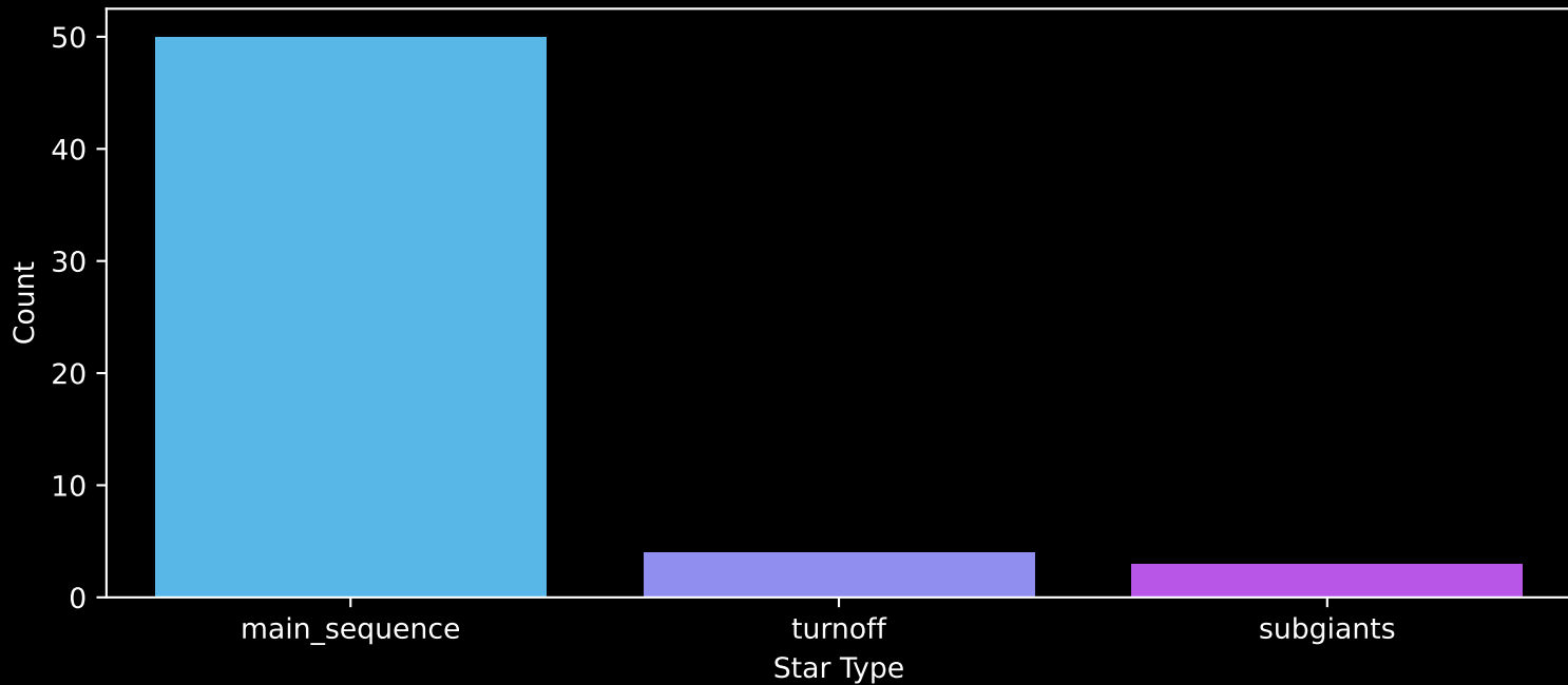
Gaia Cluster: [UPK_79] Count plot of Star Type
