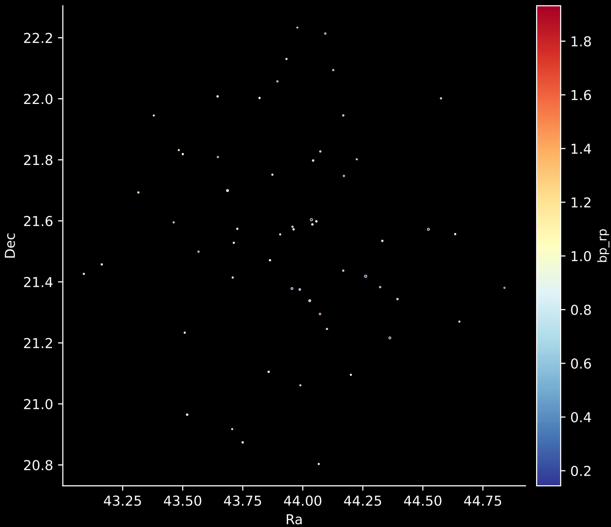
Gaia Cluster: [UPK_79] Stars: 57
