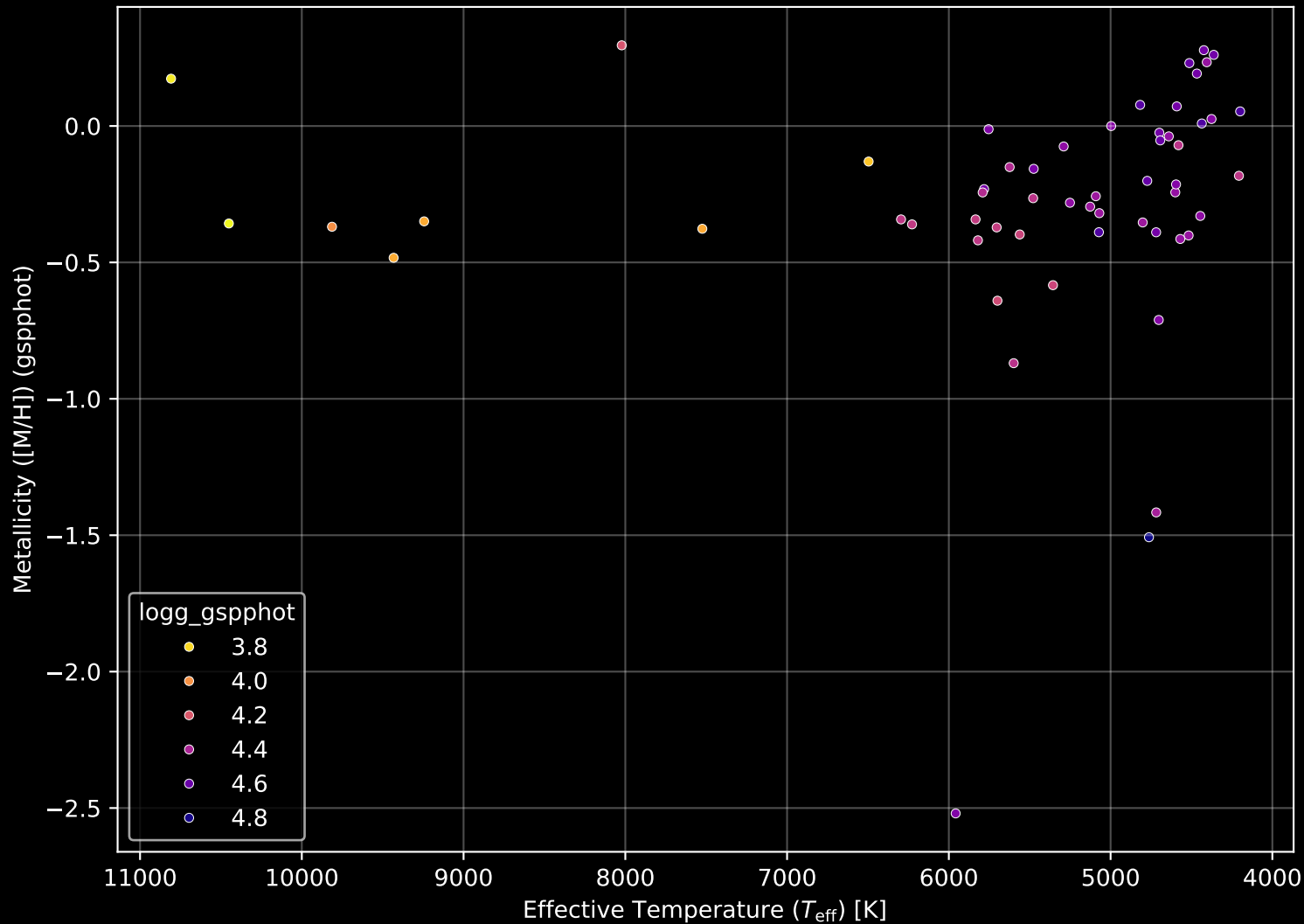
Gaia Cluster: [UPK_79] Stellar Population Parameters (n= 57)
