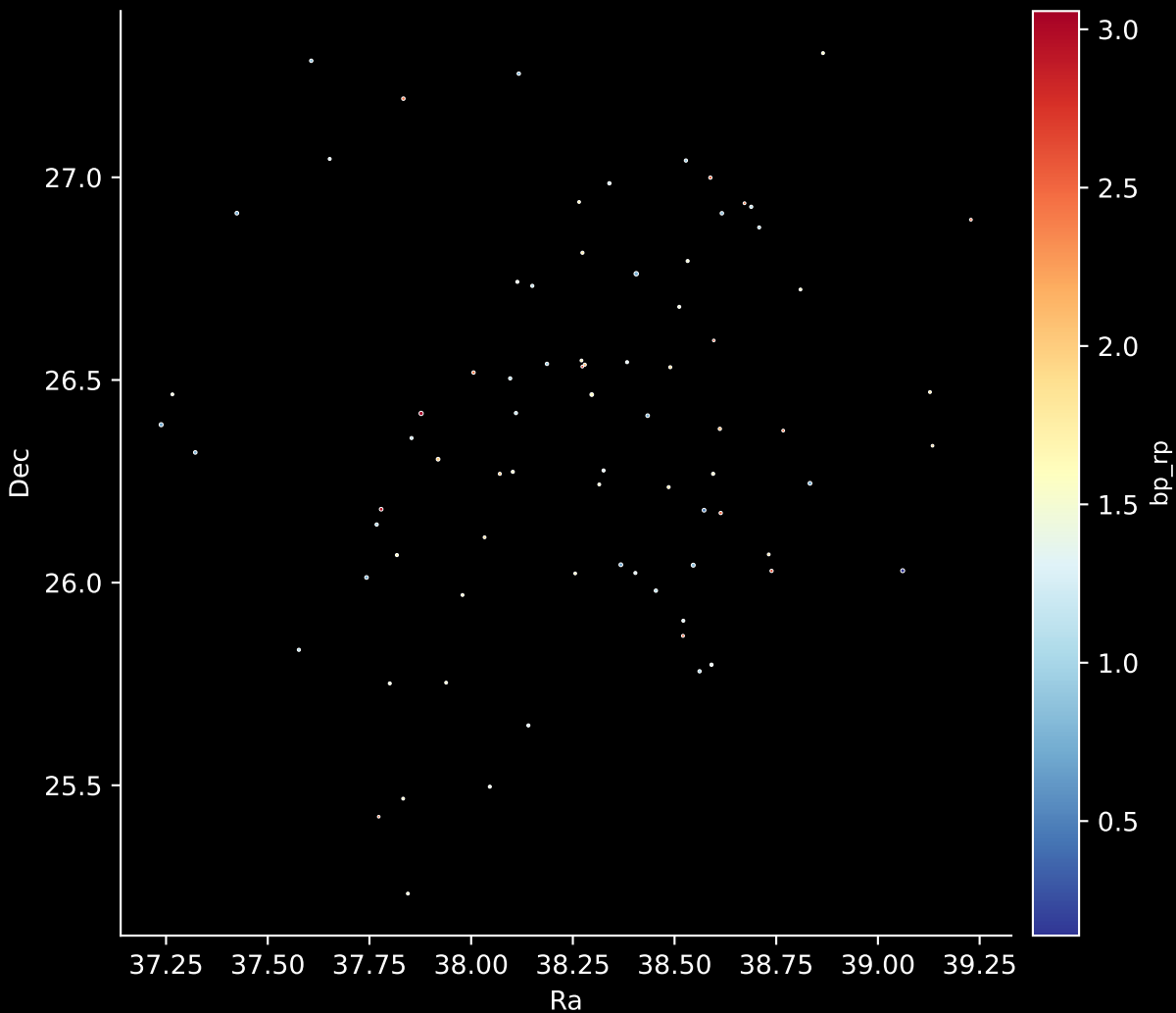
Gaia Cluster: [UPK_82] Stars: 79
