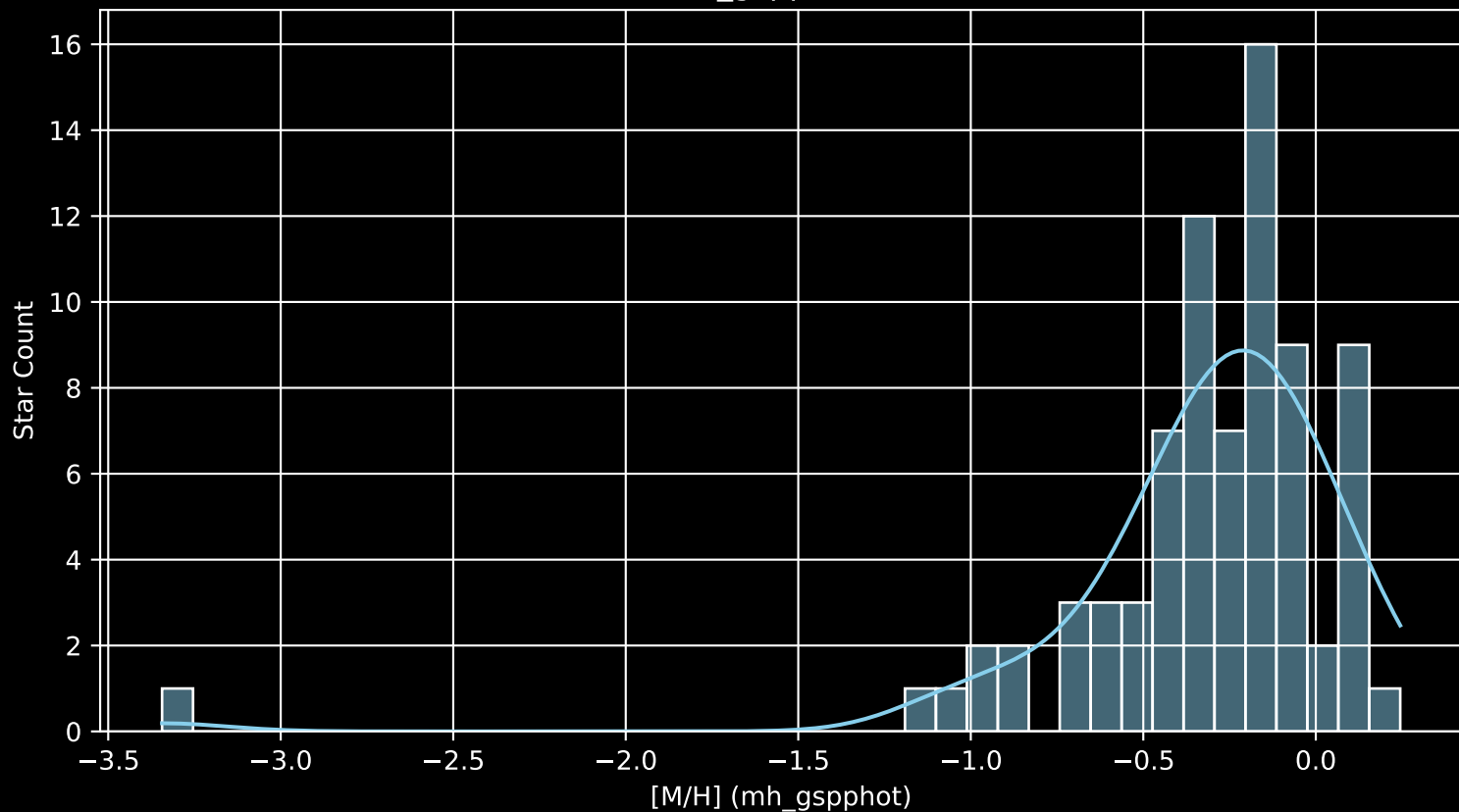
Gaia Cluster: [UPK_82 [M/H] (mh_gspphot) (n= 79)
