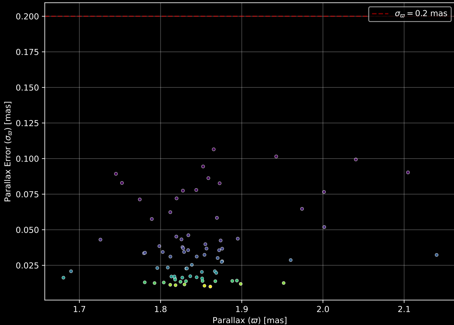
Gaia Cluster: [UPK_82] Parallax Quality (n= 79)
