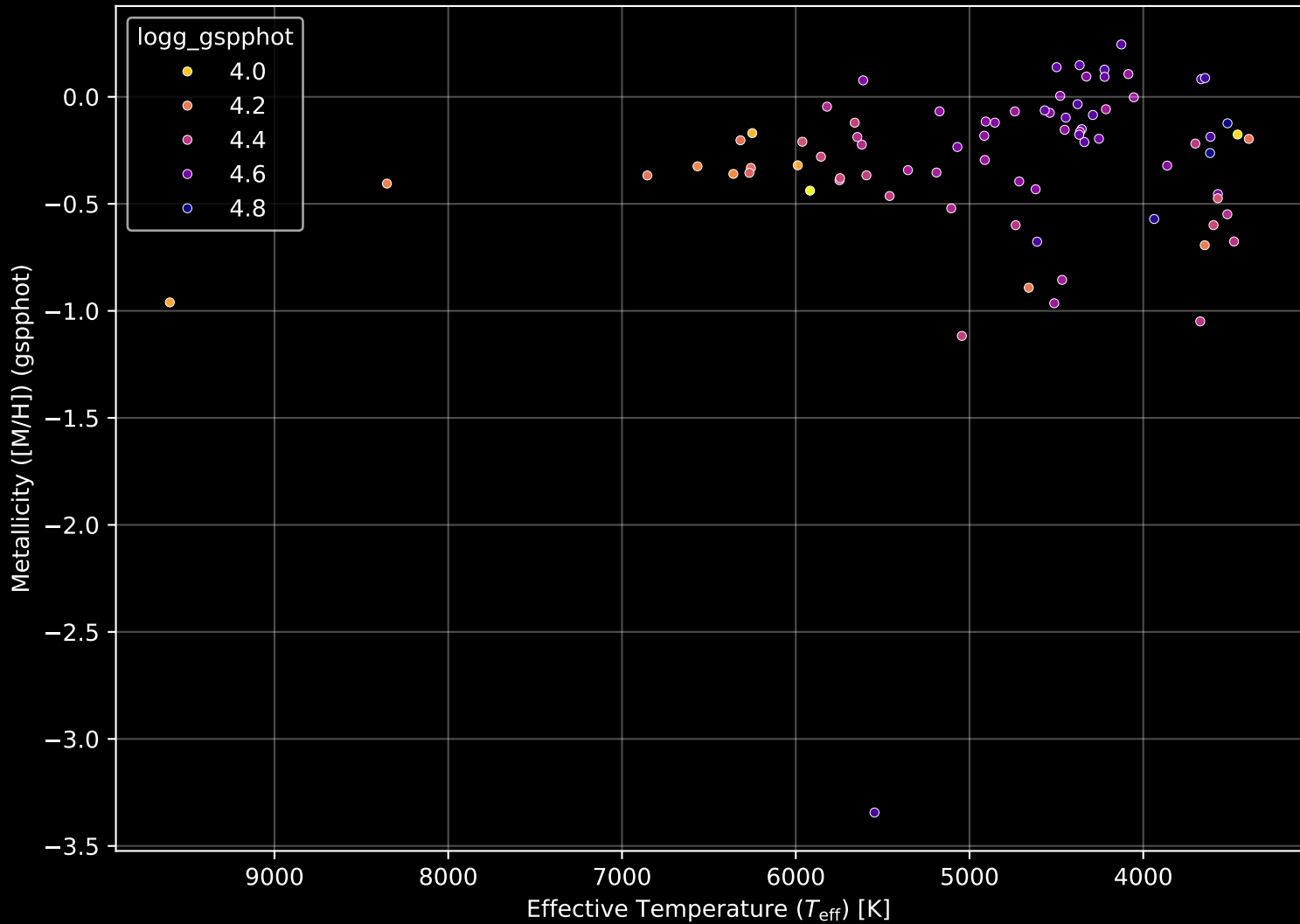
Gaia Cluster: [UPK_82] Stellar Population Parameters (n= 79)
