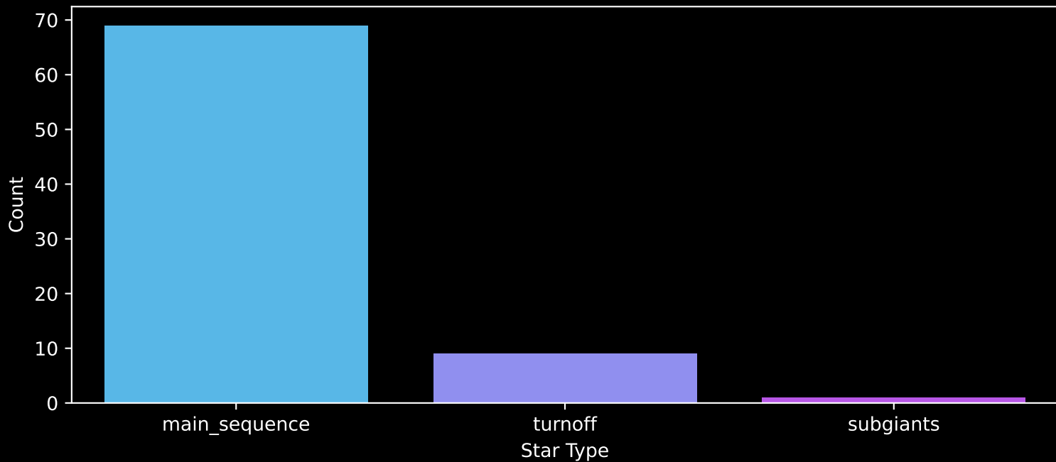
Gaia Cluster: [UPK_82] Count plot of Star Type
