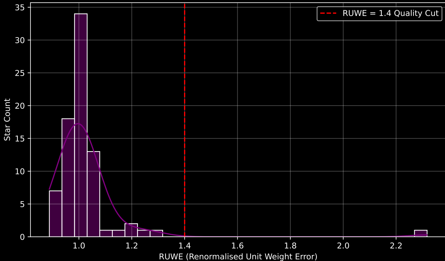
Gaia Cluster: [UPK_82] RUWE Distribution (n= 79)
