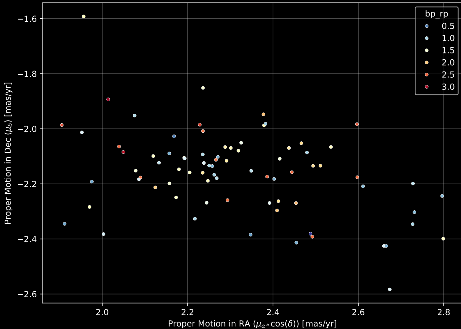
Gaia Cluster: [UPK_82] Proper Motion Diagram (n= 79)
