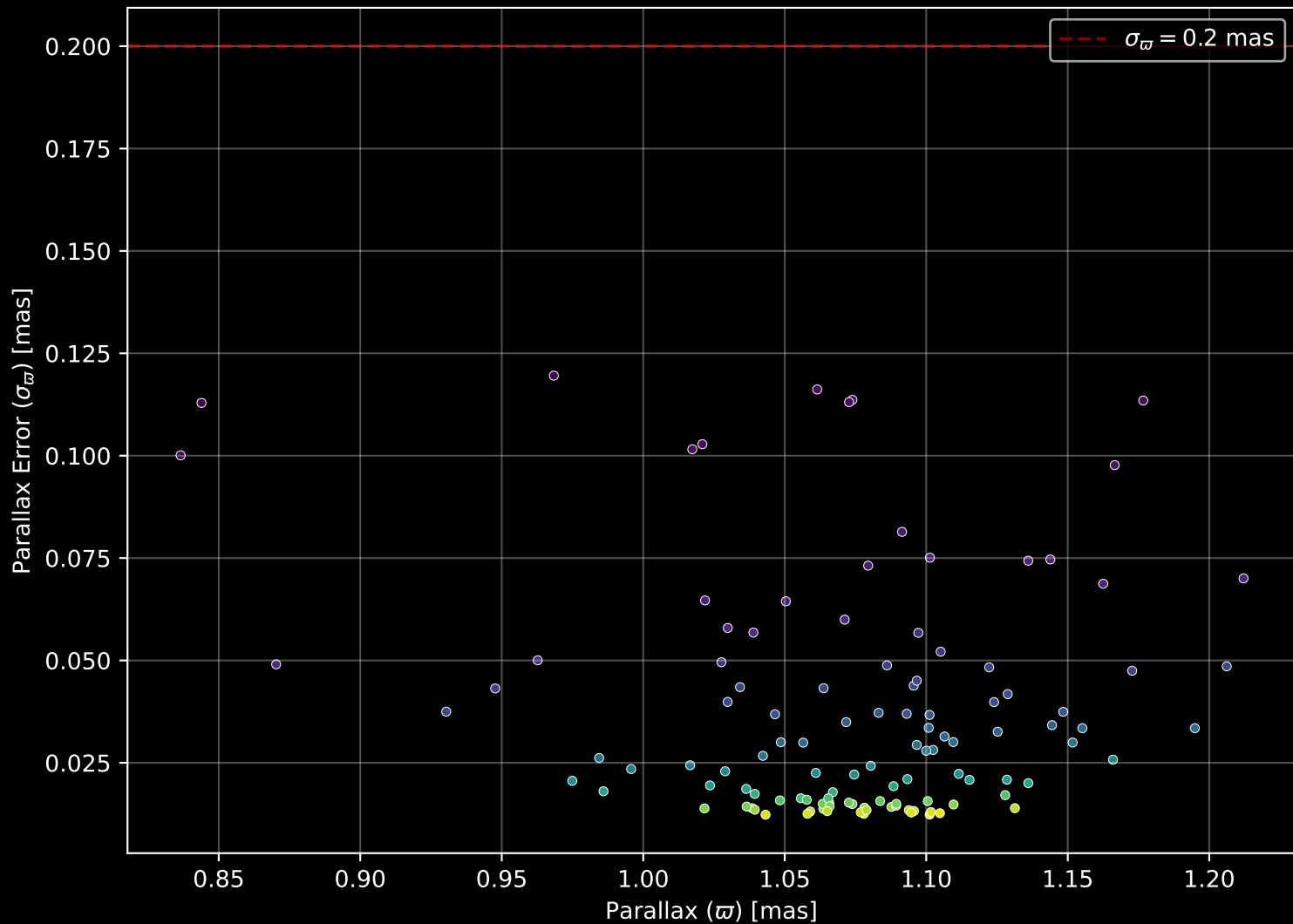
Gaia Cluster: [UPK_84] Parallax Quality (n= 116)
