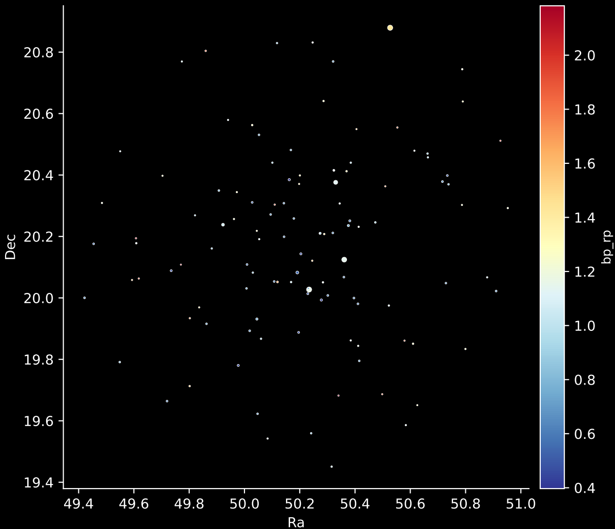
Gaia Cluster: [UPK_84] Stars: 116
