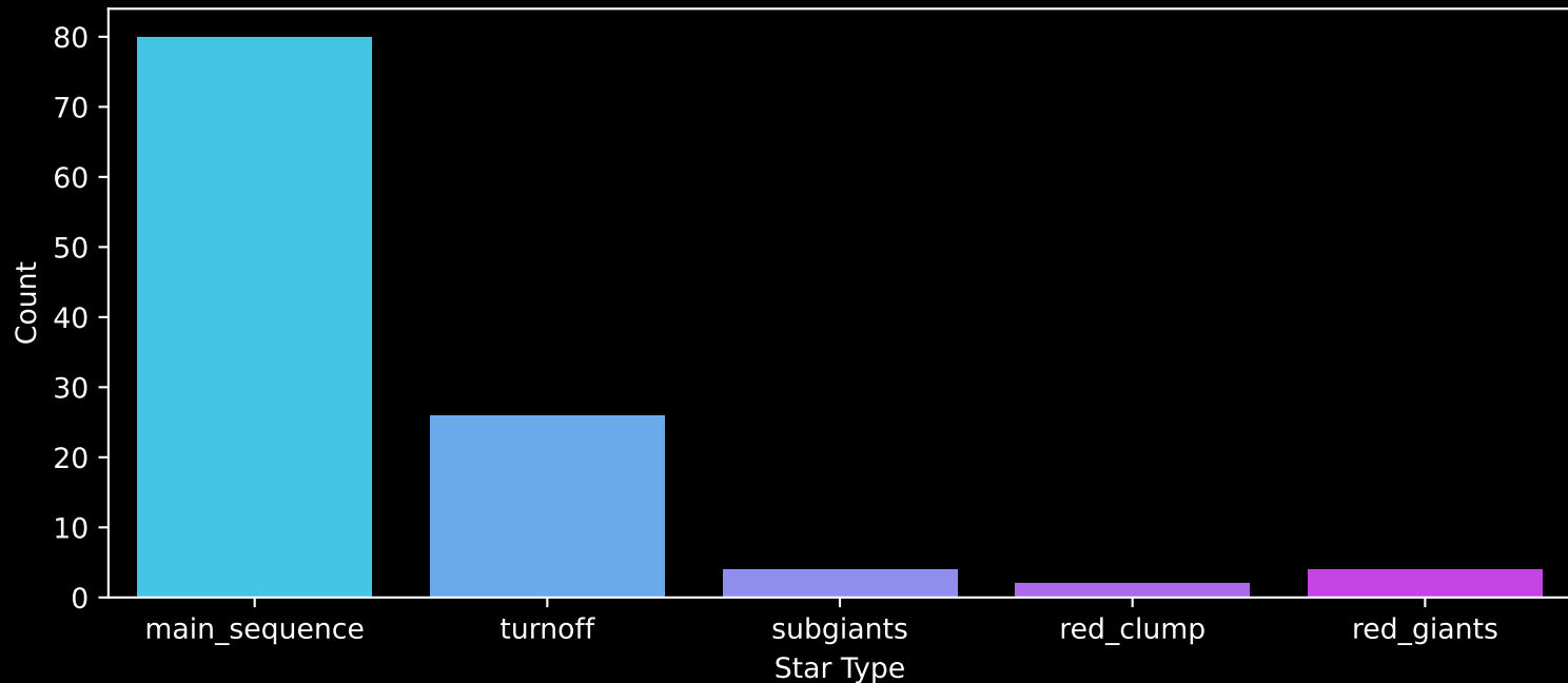
Gaia Cluster: [UPK_84] Count plot of Star Type
