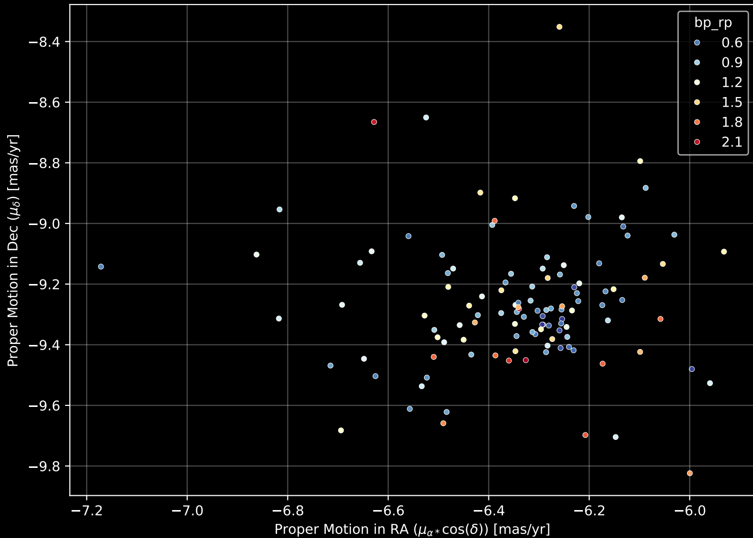
Gaia Cluster: [UPK_84] Proper Motion Diagram (n= 116)
