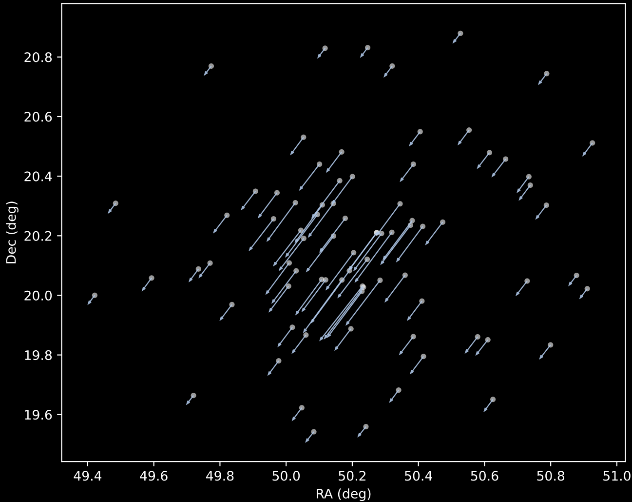
Gaia DR3 Cluster 1 Proper Motion Vectors (n=80)
