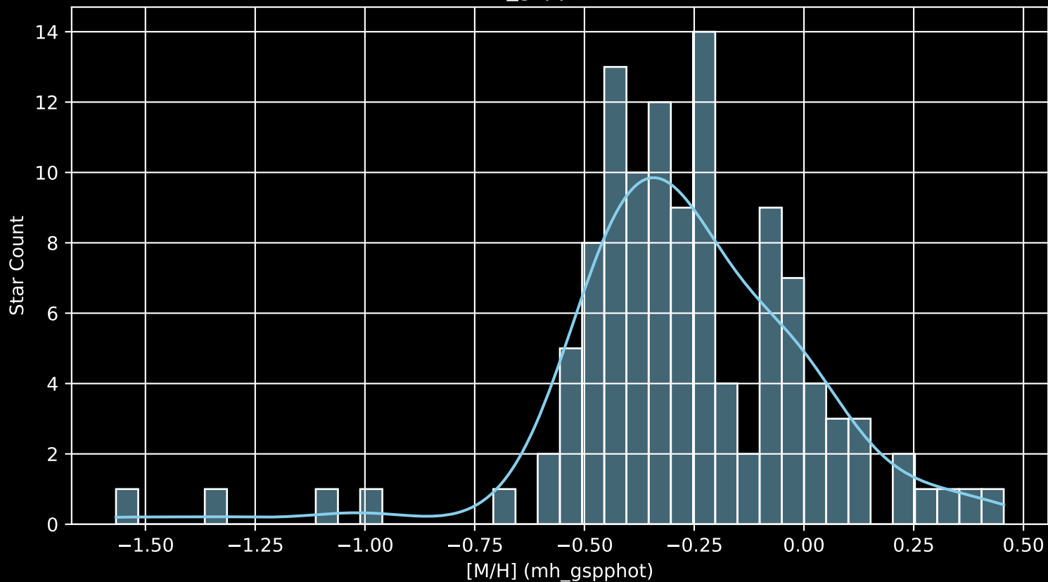
Gaia Cluster: [UPK_84 [M/H] (mh_gspphot) (n= 116)
