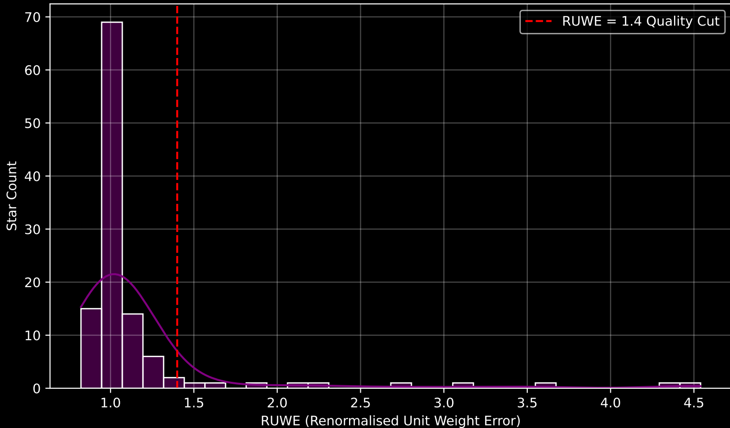
Gaia Cluster: [UPK_84] RUWE Distribution (n= 116)
