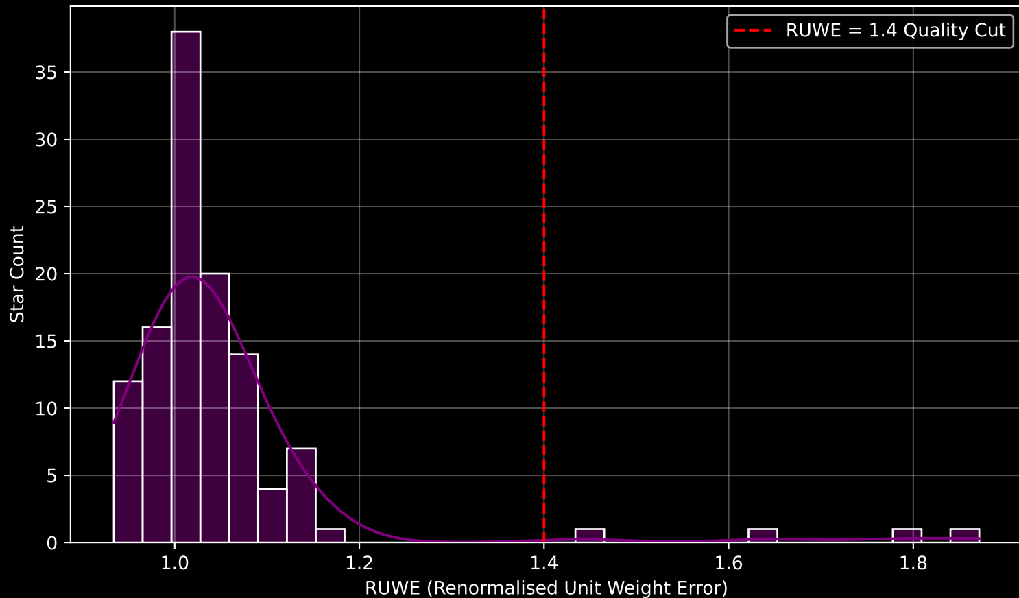
Gaia Cluster: [Waterloo_1] RUWE Distribution (n= 116)
