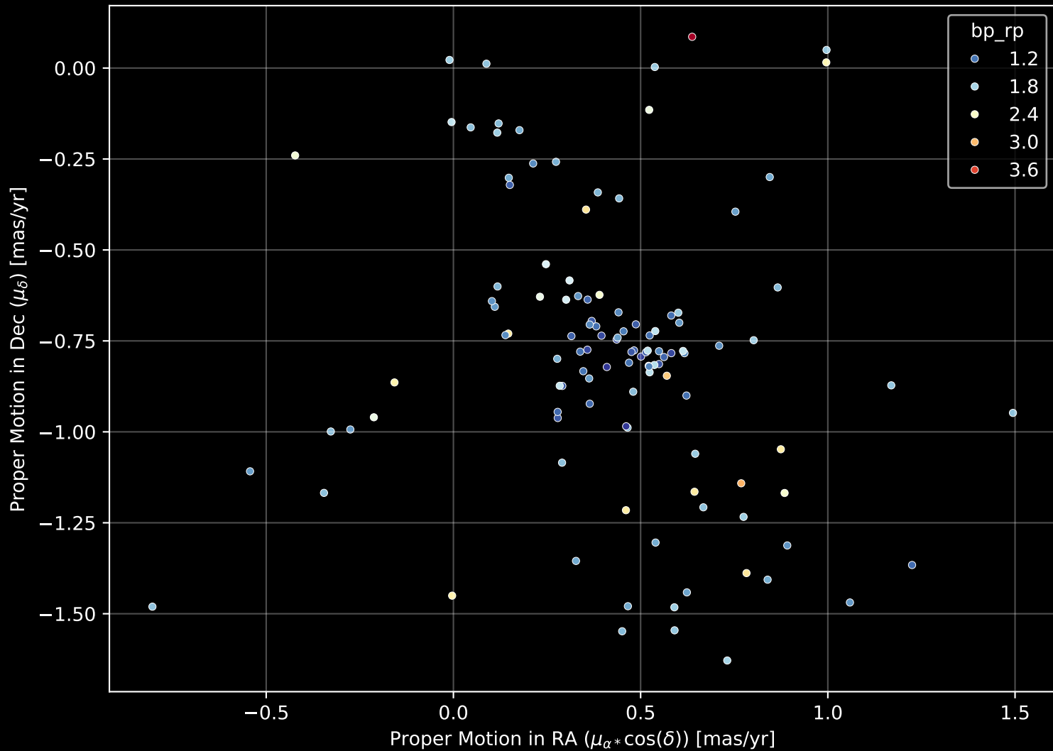
Gaia Cluster: [Waterloo_1] Proper Motion Diagram (n= 116)
