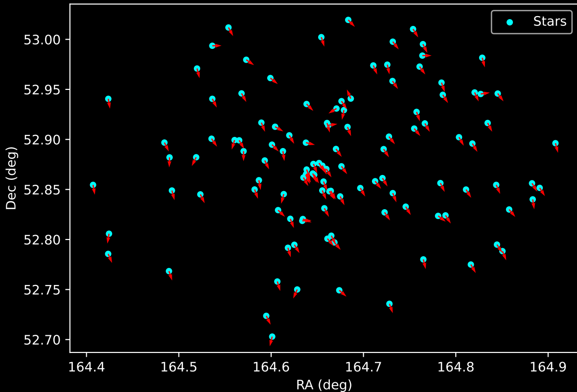
Gaia Cluster: [Waterloo_1] Proper Motion Vectors for Gaia Star Field (n= 116)
