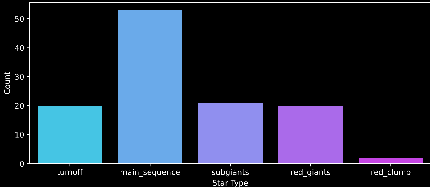
Gaia Cluster: [Waterloo_1] Count plot of Star Type
