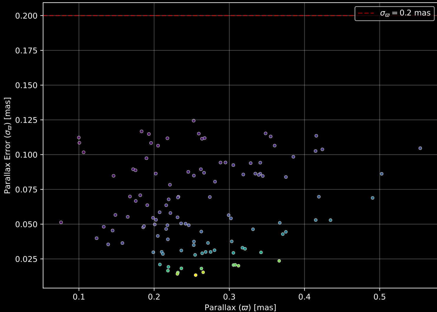
Gaia Cluster: [Waterloo_1] Parallax Quality (n= 116)
