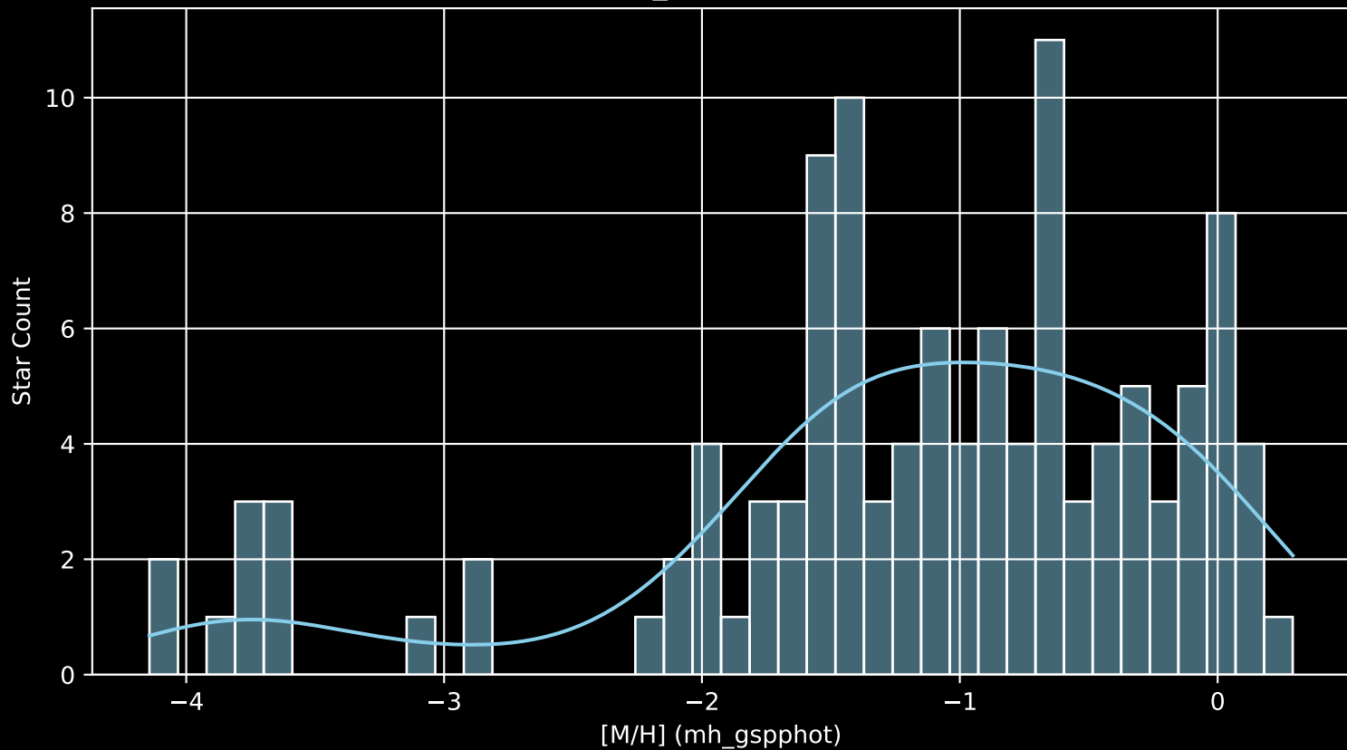
Gaia Cluster: [Waterloo_1 [M/H] (mh_gspphot) (n= 116)
