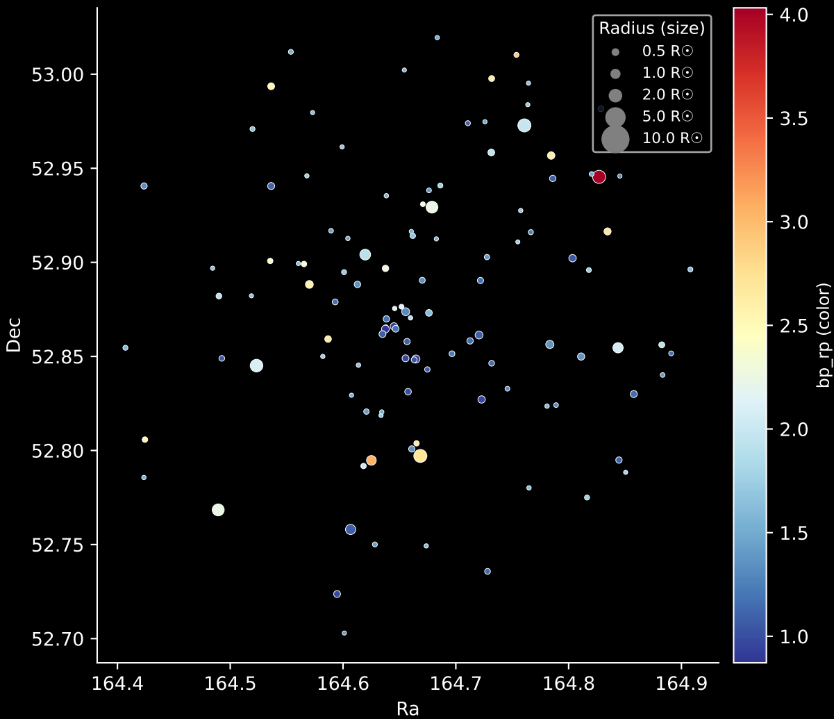
Gaia Cluster: [Waterloo_1] Stars: 116
