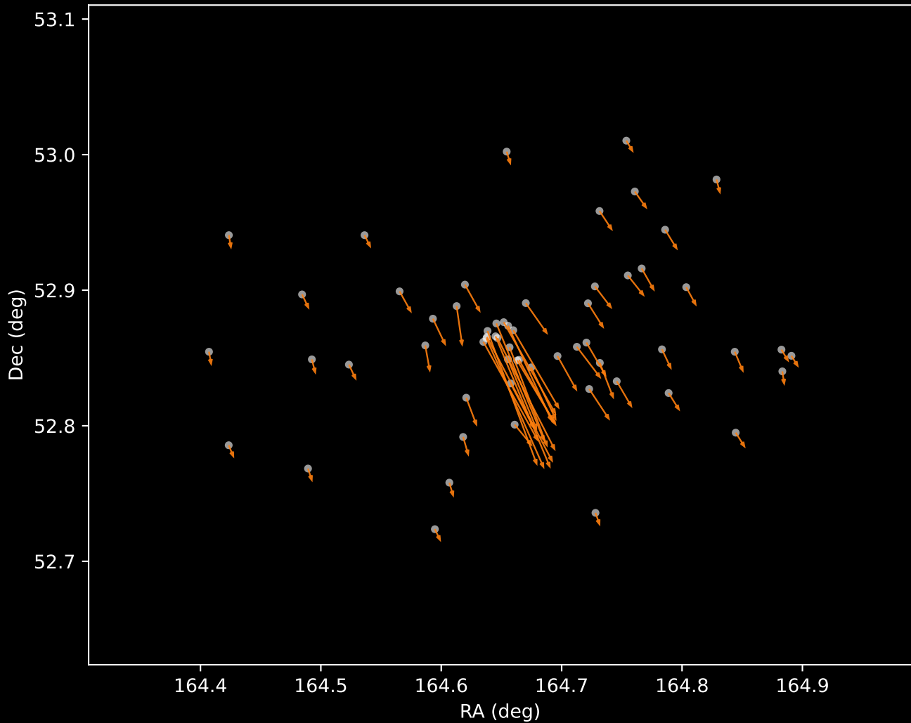
Gaia DR3 Cluster 2 Proper Motion Vectors (n=60)
