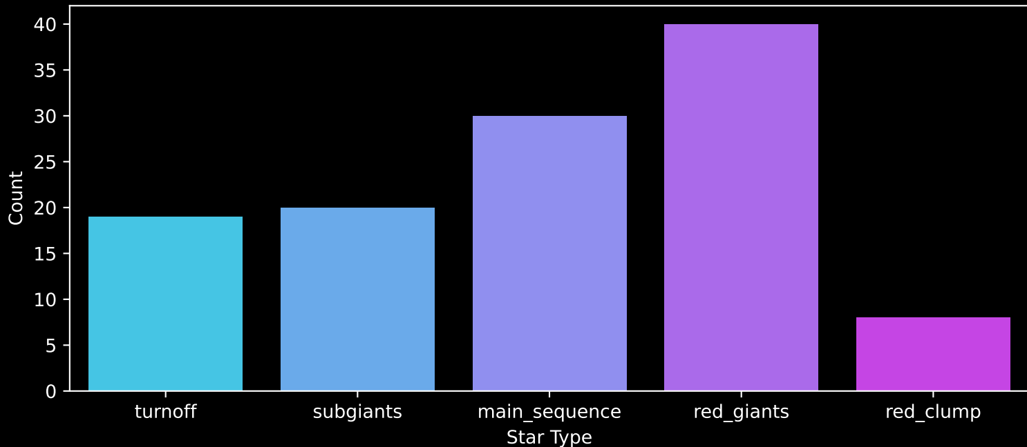
Gaia Cluster: [Westerlund_2] Count plot of Star Type
