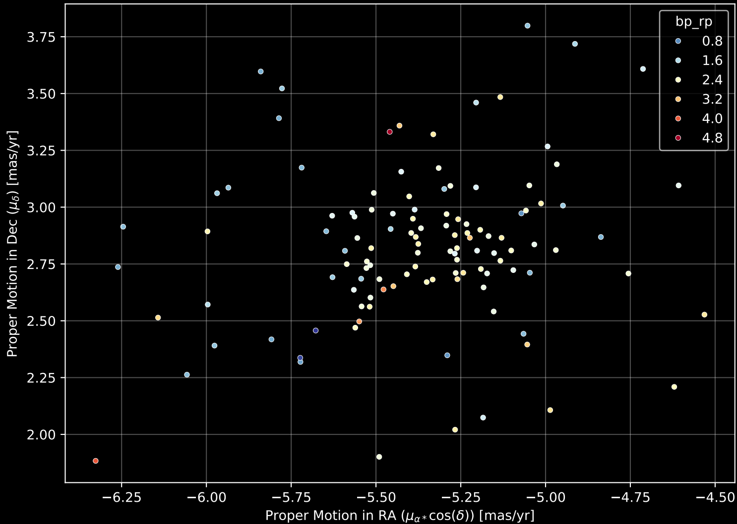
Gaia Cluster: [Westerlund_2] Proper Motion Diagram (n= 117)
