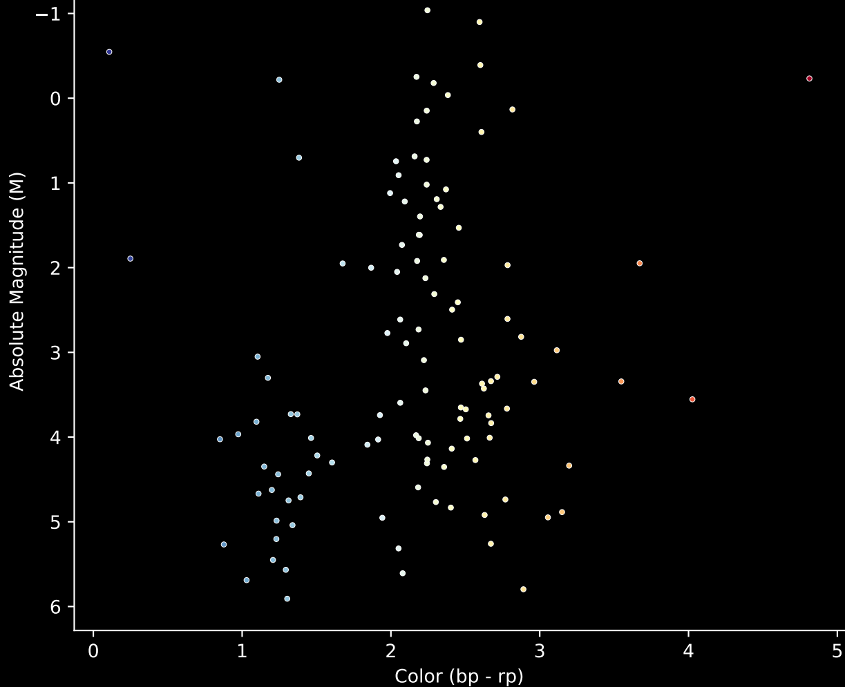
Gaia Cluster: [Westerlund_2] Stars (n= 117) Hertzsprung-Russel Diagram
