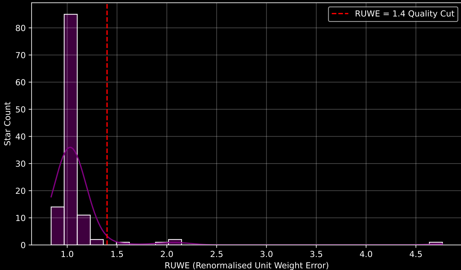
Gaia Cluster: [Westerlund_2] RUWE Distribution (n= 117)
