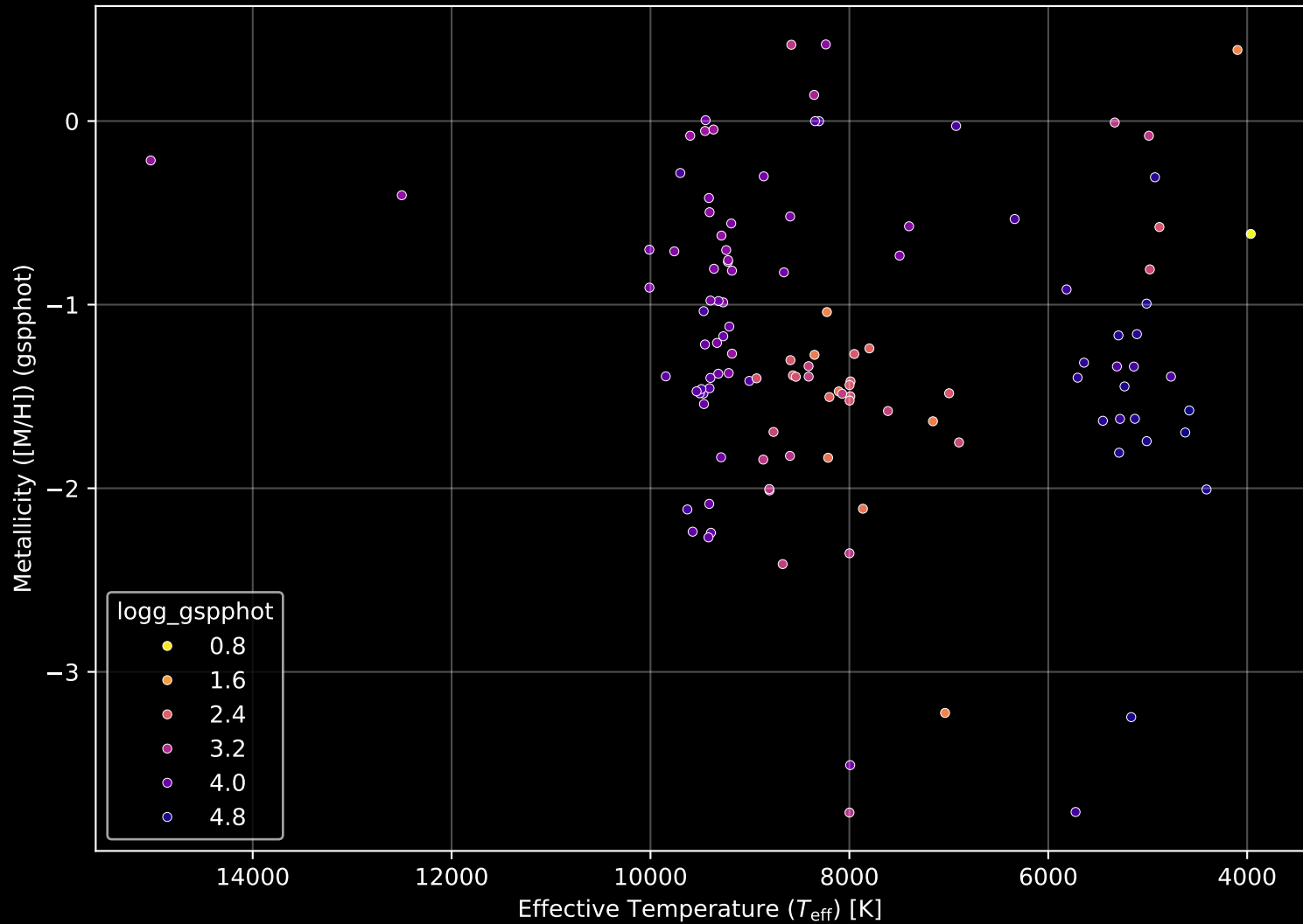
Gaia Cluster: [Westerlund_2] Stellar Population Parameters (n= 117)
