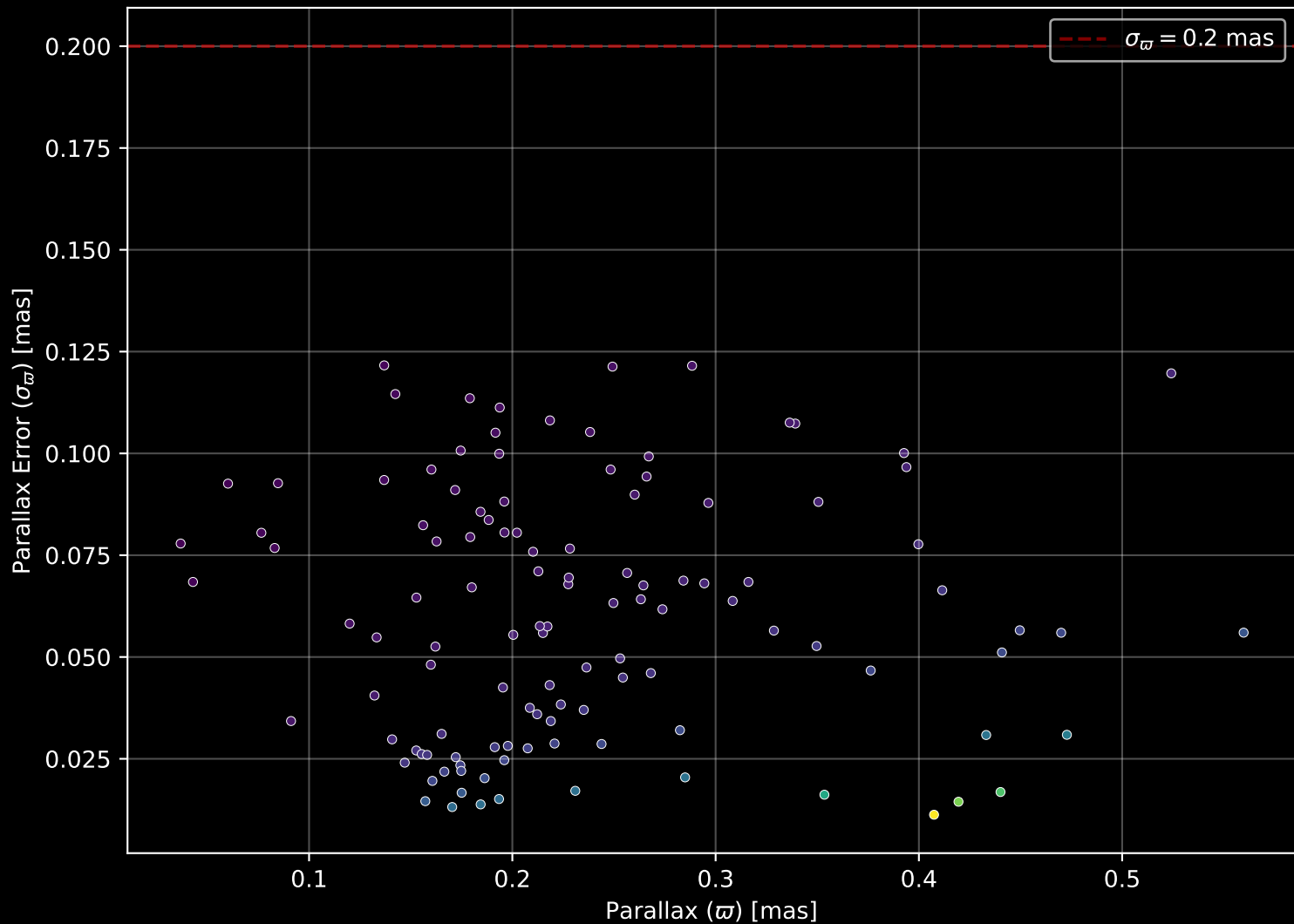
Gaia Cluster: [Westerlund_2] Parallax Quality (n= 117)
