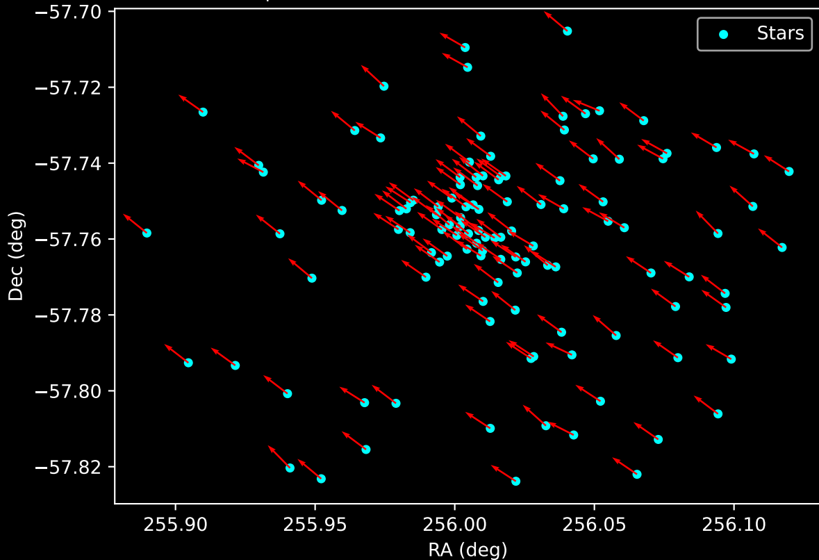
Gaia Cluster: [Westerlund_2] Proper Motion Vectors for Gaia Star Field (n= 117)
