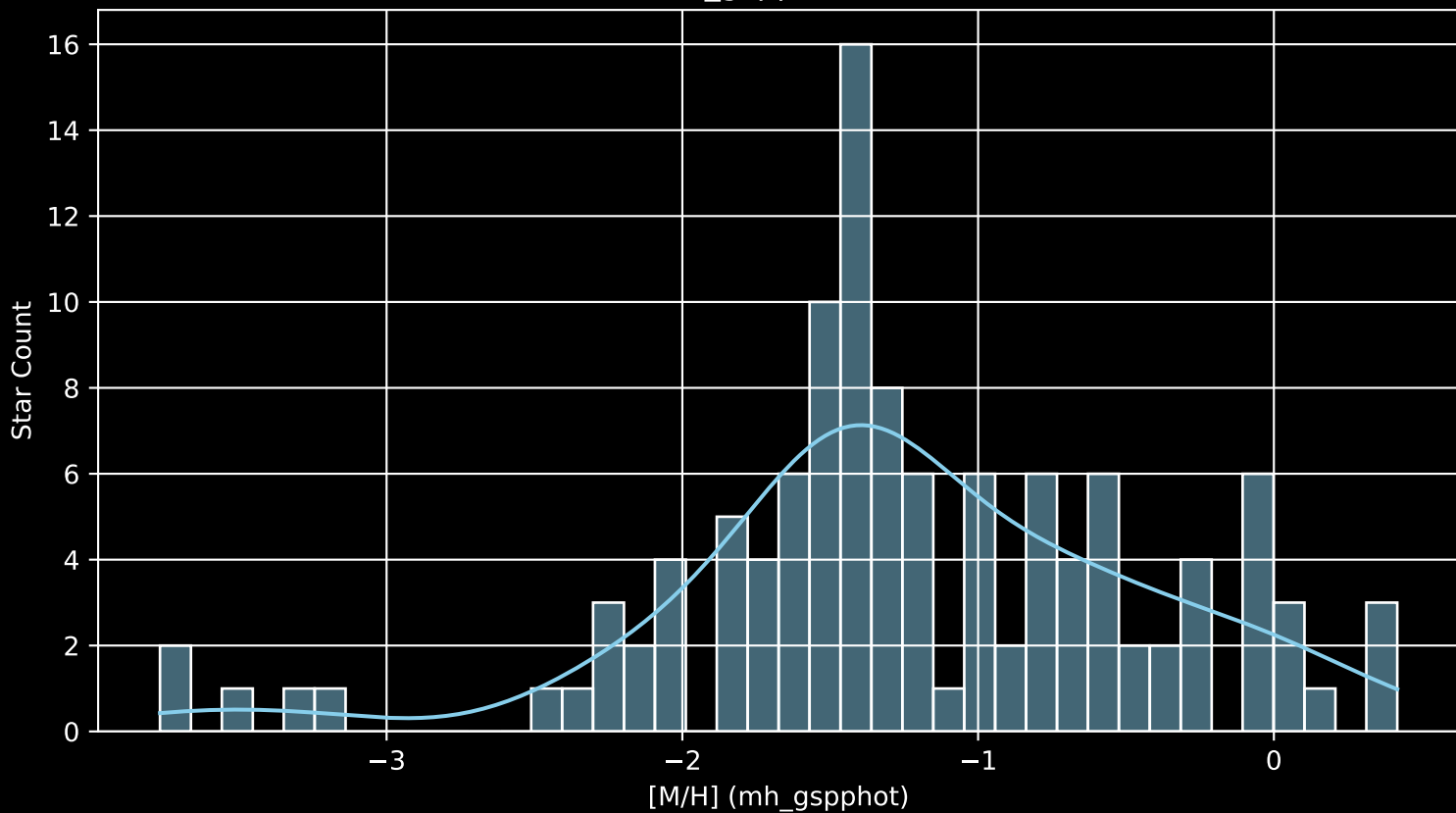
Gaia Cluster: [Westerlund_2 [M/H] (mh_gspphot) (n= 117)
