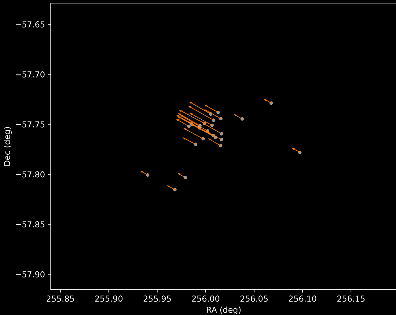
Gaia DR3 Cluster 2 Proper Motion Vectors (n=24)
