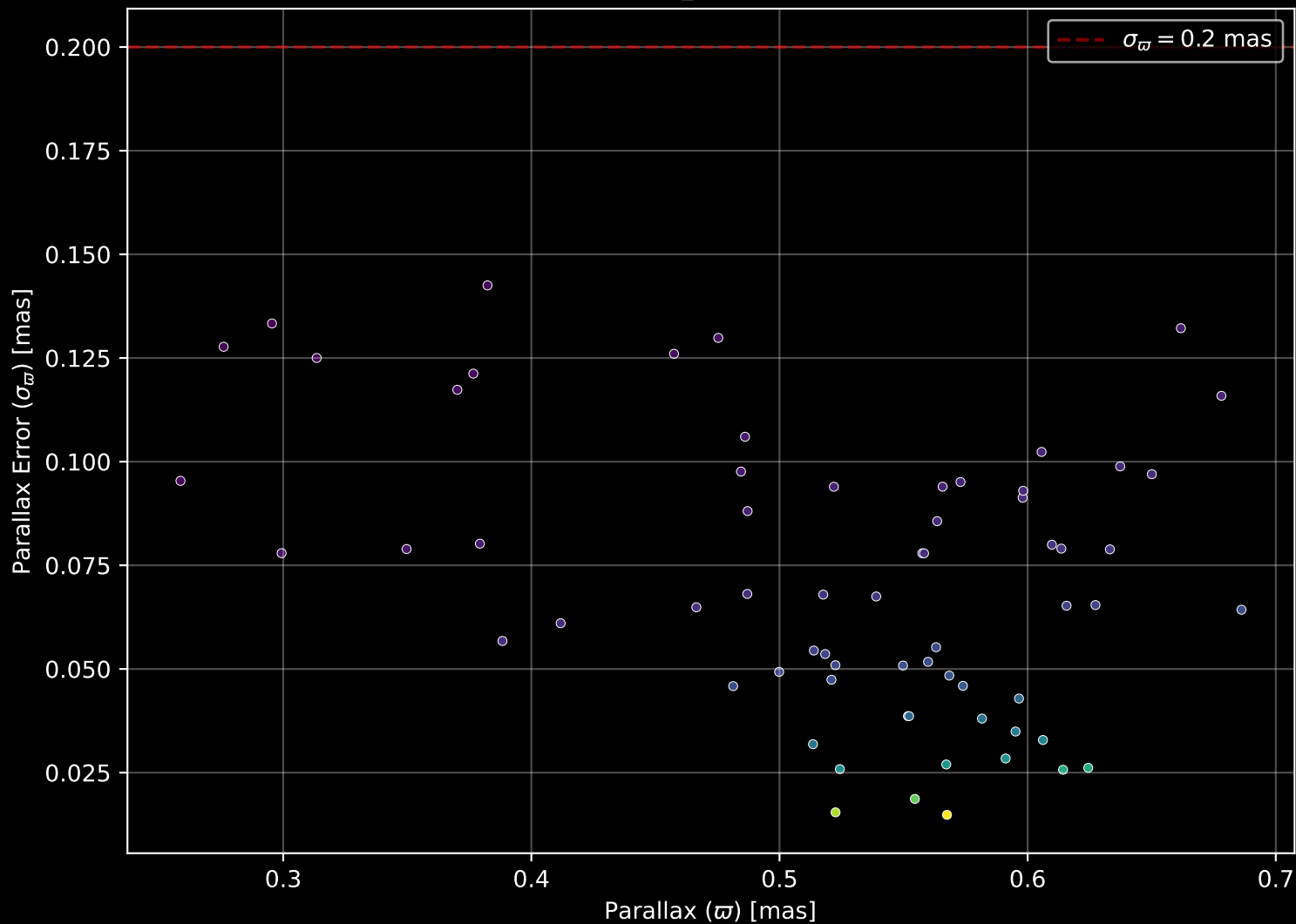
Gaia Cluster: [vdBergh_1] Parallax Quality (n= 66)
