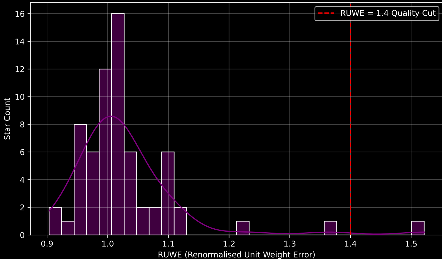
Gaia Cluster: [vdBergh_1] RUWE Distribution (n= 66)
