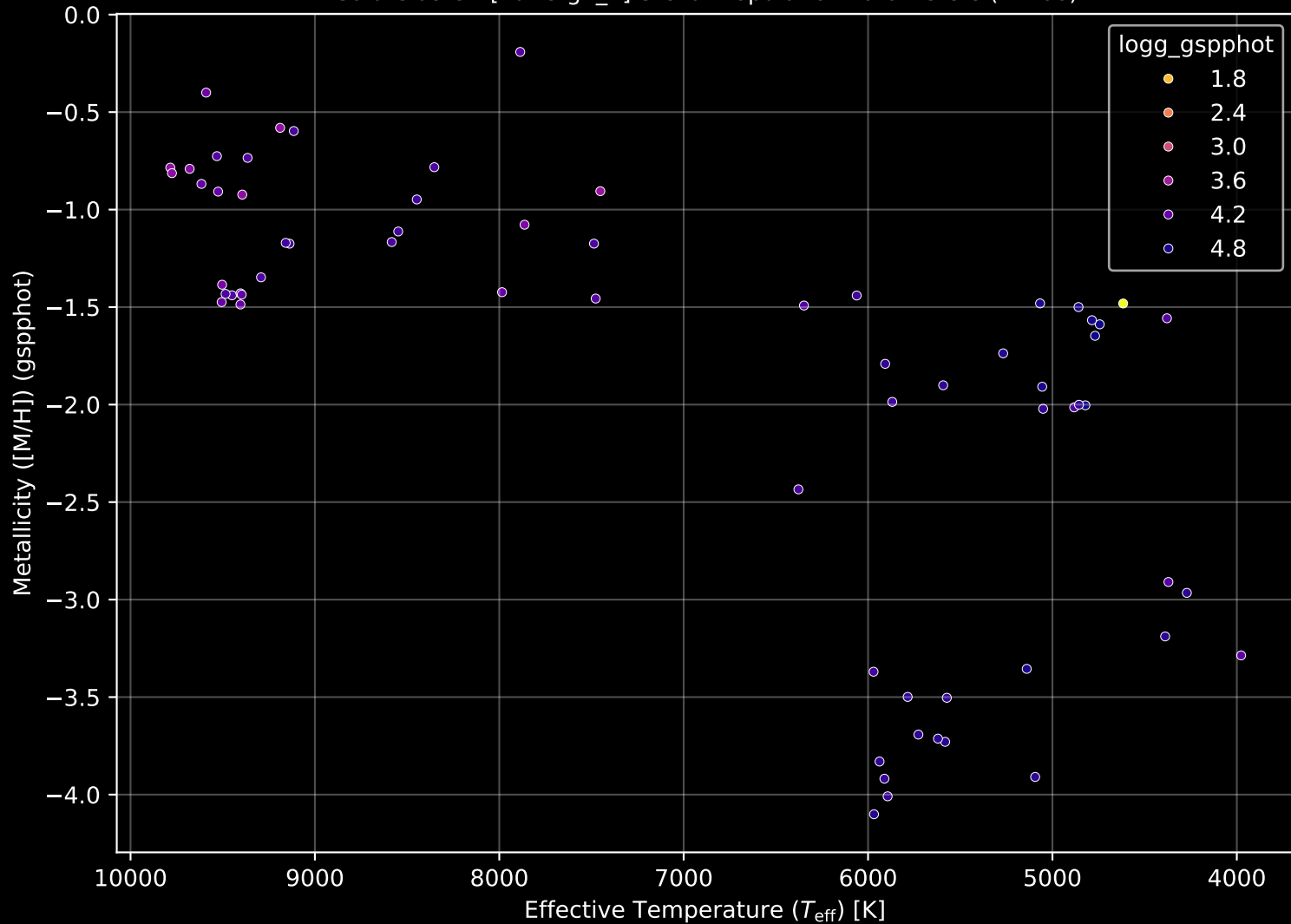
Gaia Cluster: [vdBergh_1] Stellar Population Parameters (n= 66)
