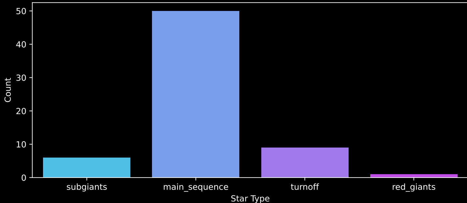
Gaia Cluster: [vdBergh_1] Count plot of Star Type
