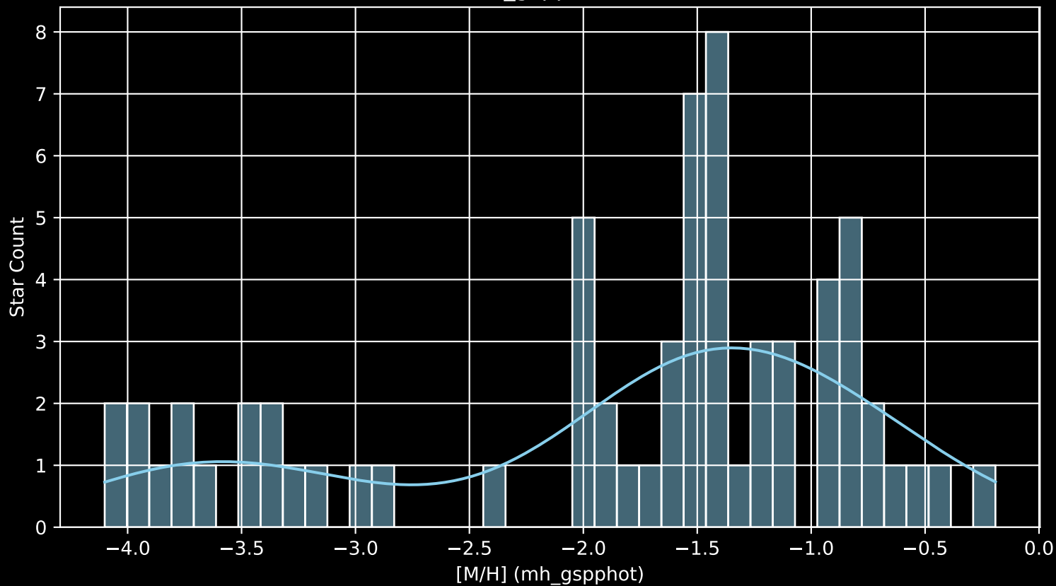
Gaia Cluster: [vdBergh_1 [M/H] (mh_gspphot) (n= 66)
