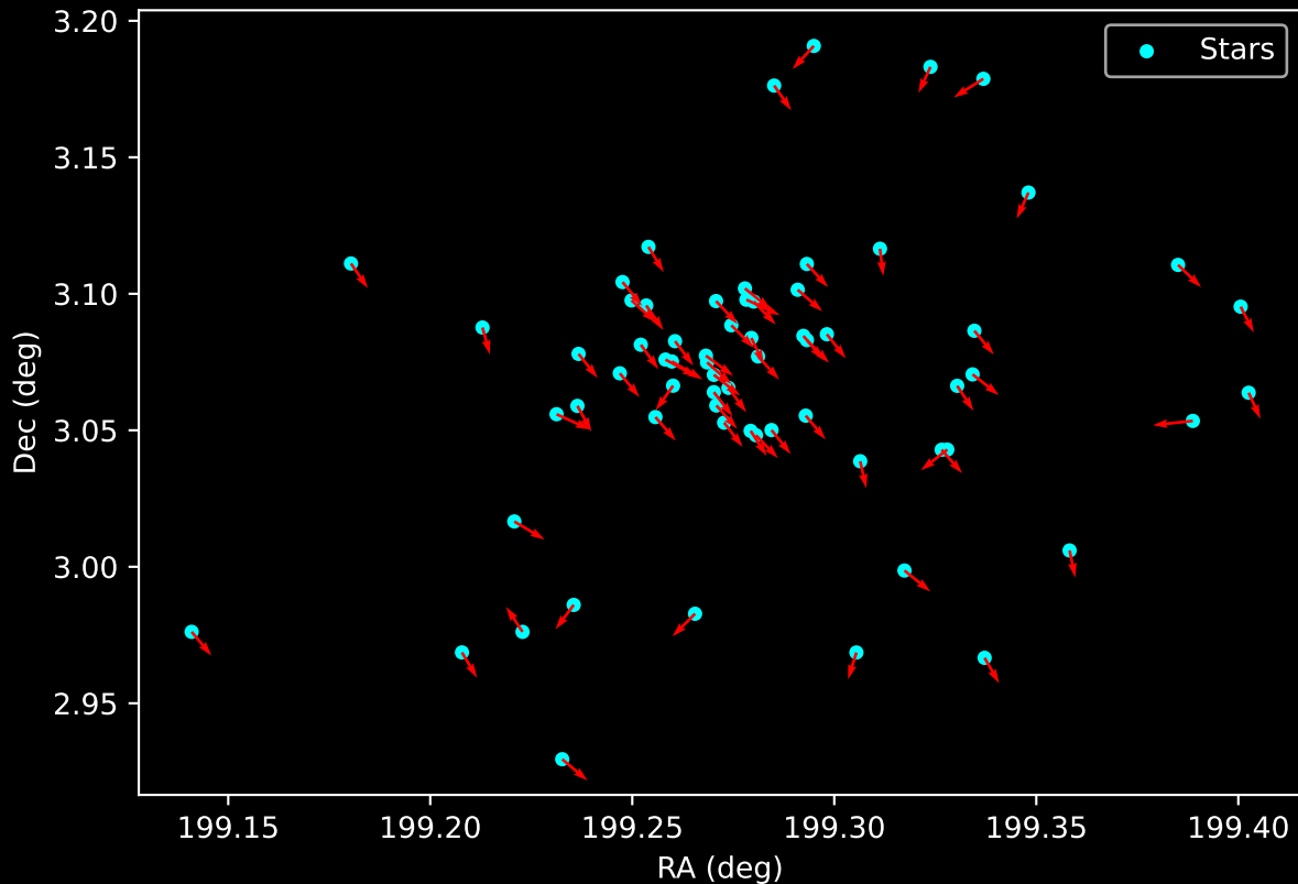
Gaia Cluster: [vdBergh_1] Proper Motion Vectors for Gaia Star Field (n= 66)
