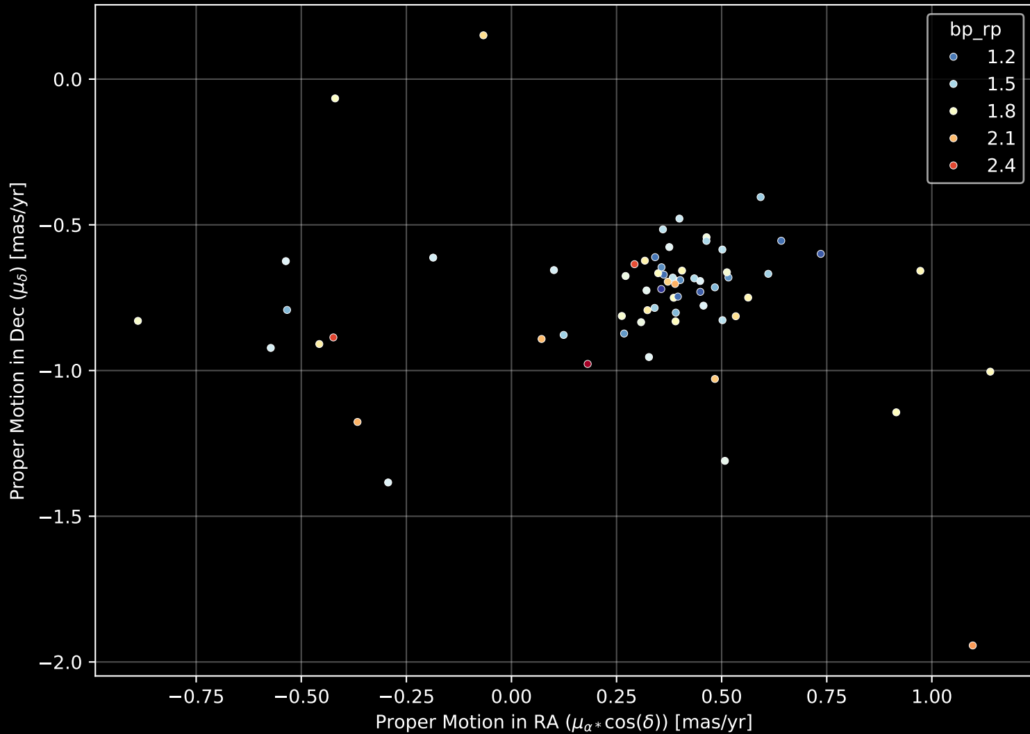
Gaia Cluster: [vdBergh_1] Proper Motion Diagram (n= 66)
