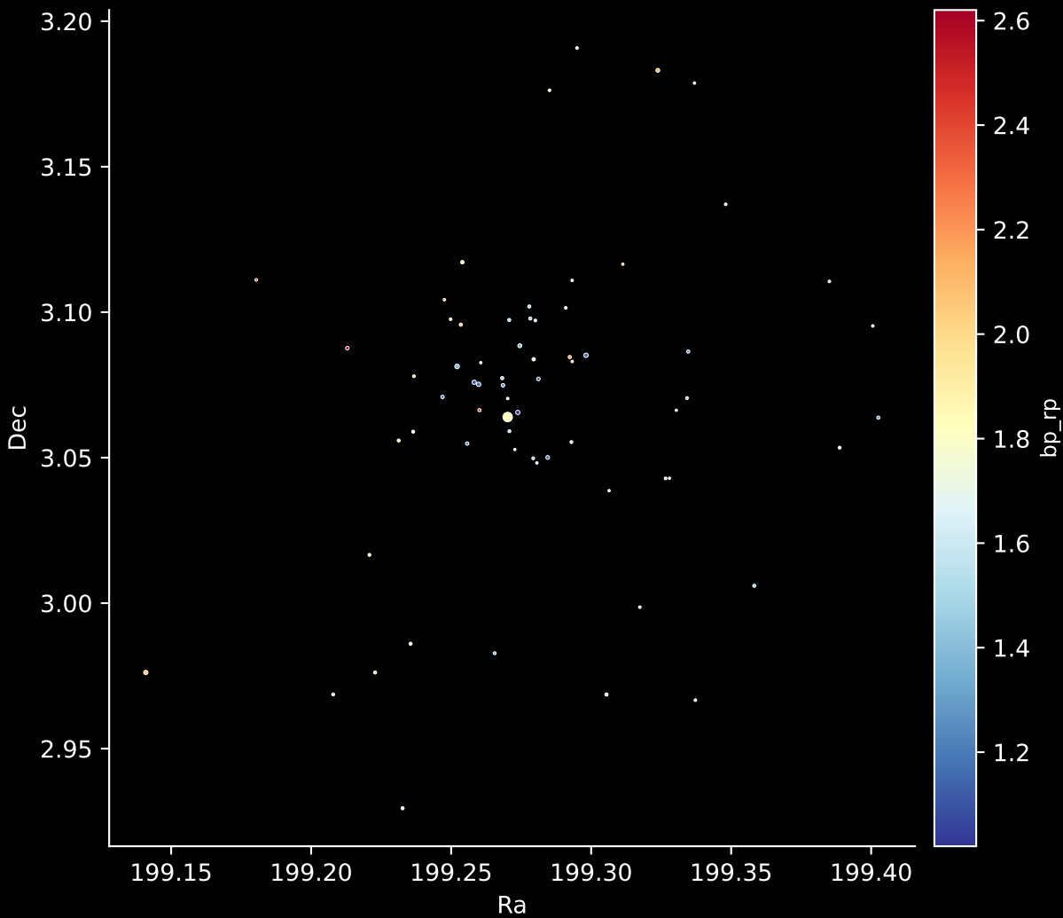
Gaia Cluster: [vdBergh_1] Stars: 66
