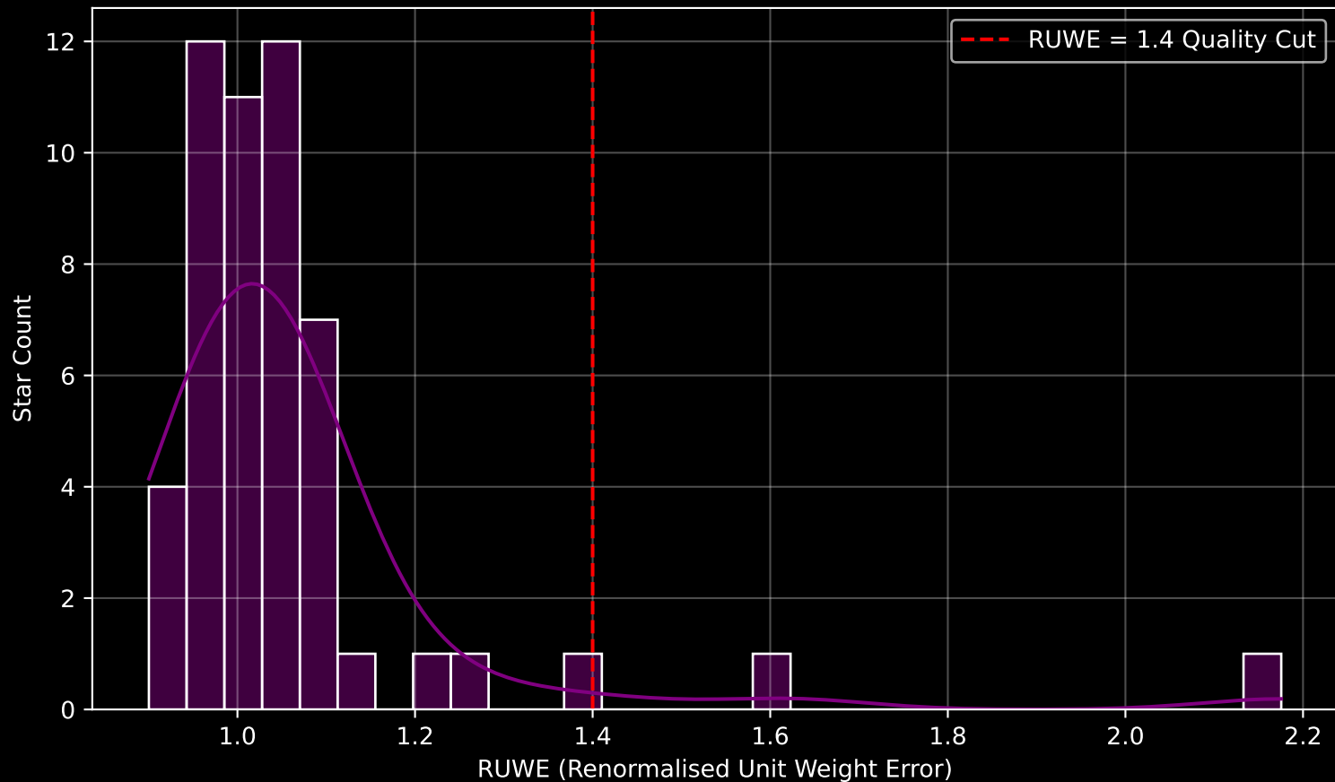
Gaia Cluster: [vdBergh_85] RUWE Distribution (n= 52)
