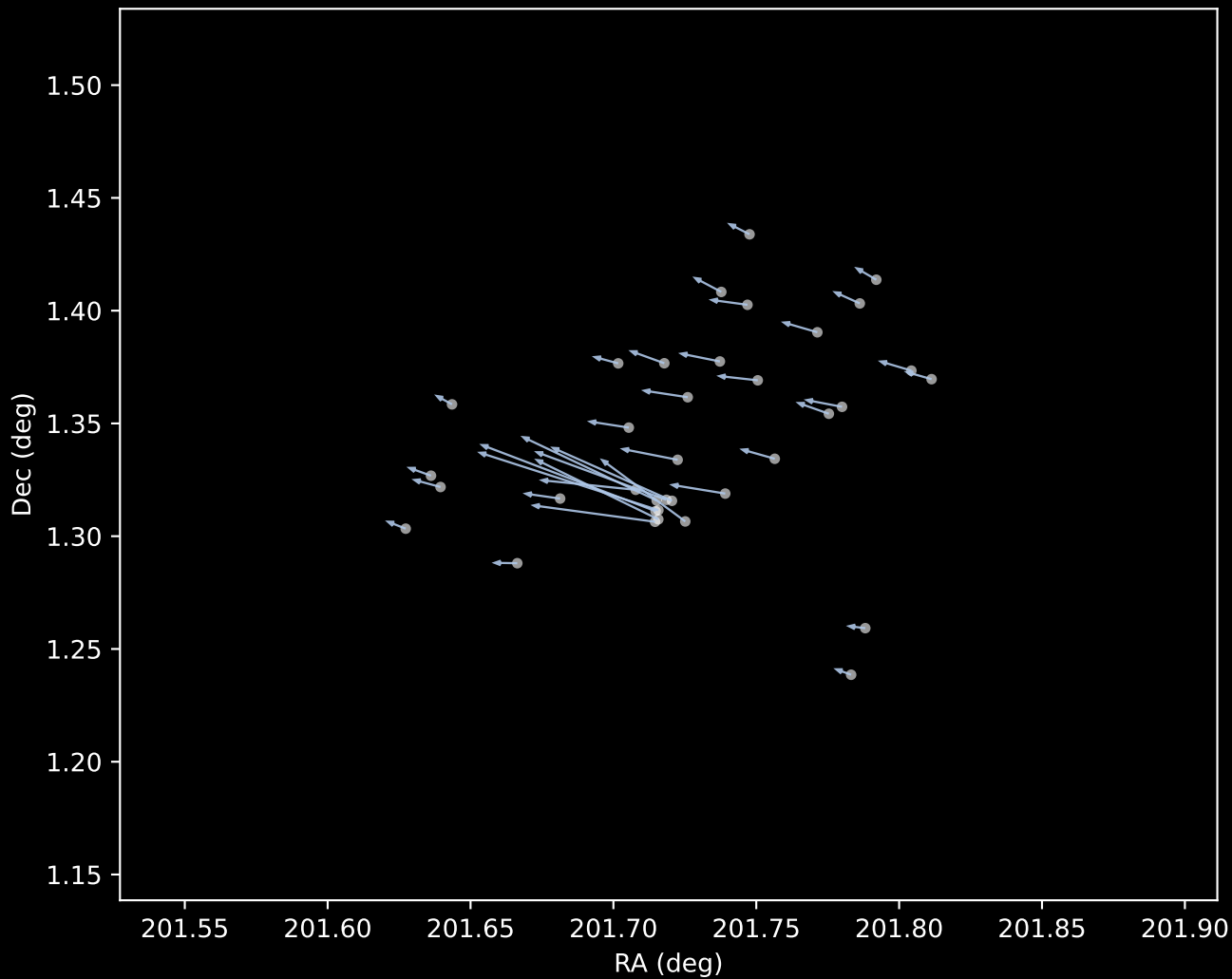
Gaia DR3 Cluster 1 Proper Motion Vectors (n=36)
