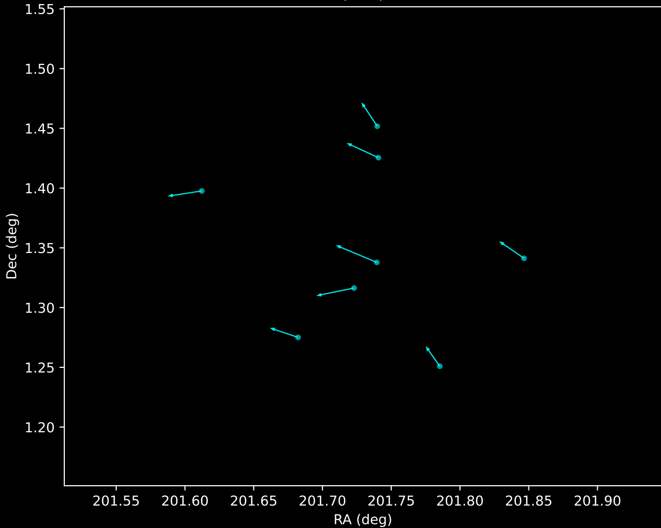
Gaia DR3 Noise Stream Proper Motion Vectors (n=8)
