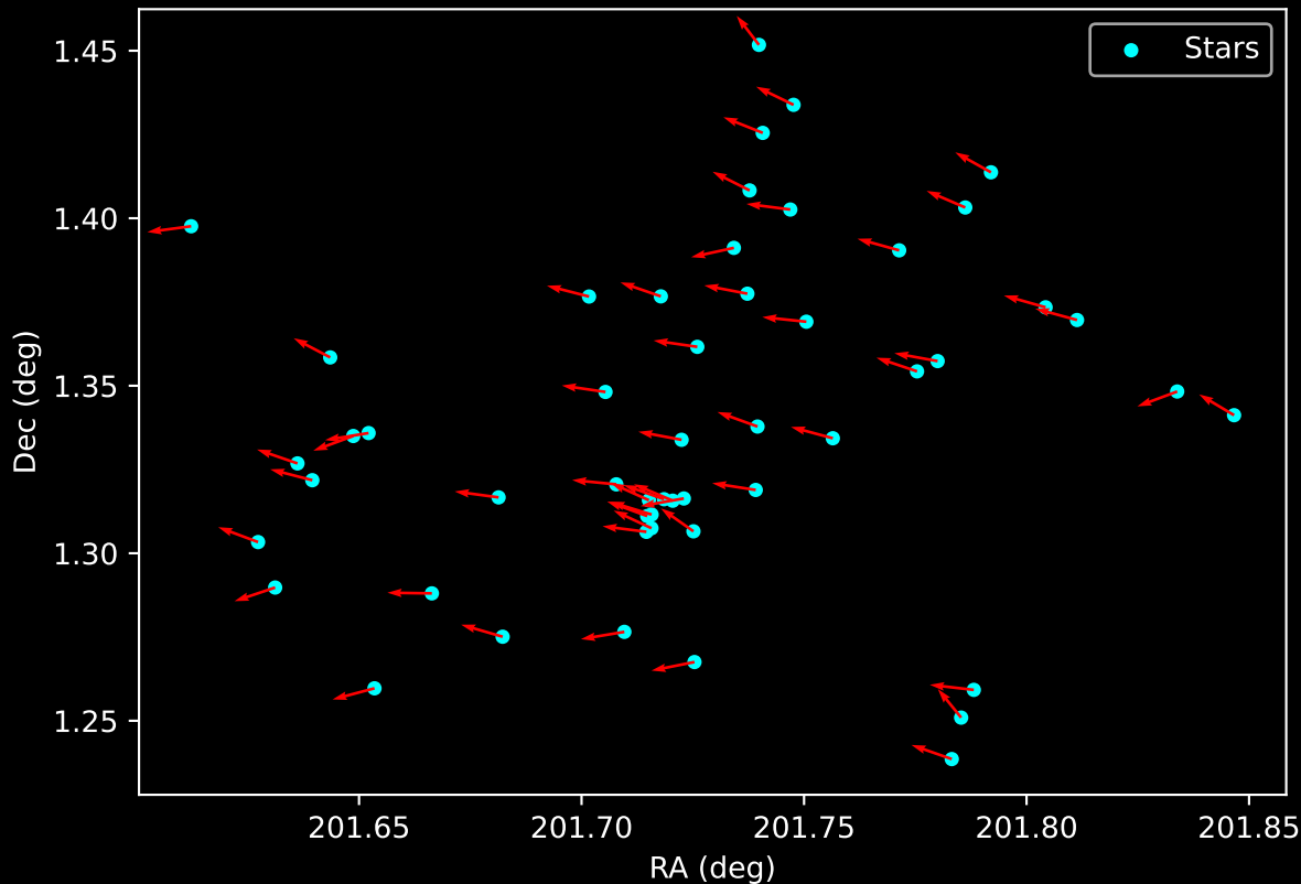
Gaia Cluster: [vdBergh_85] Proper Motion Vectors for Gaia Star Field (n= 52)
