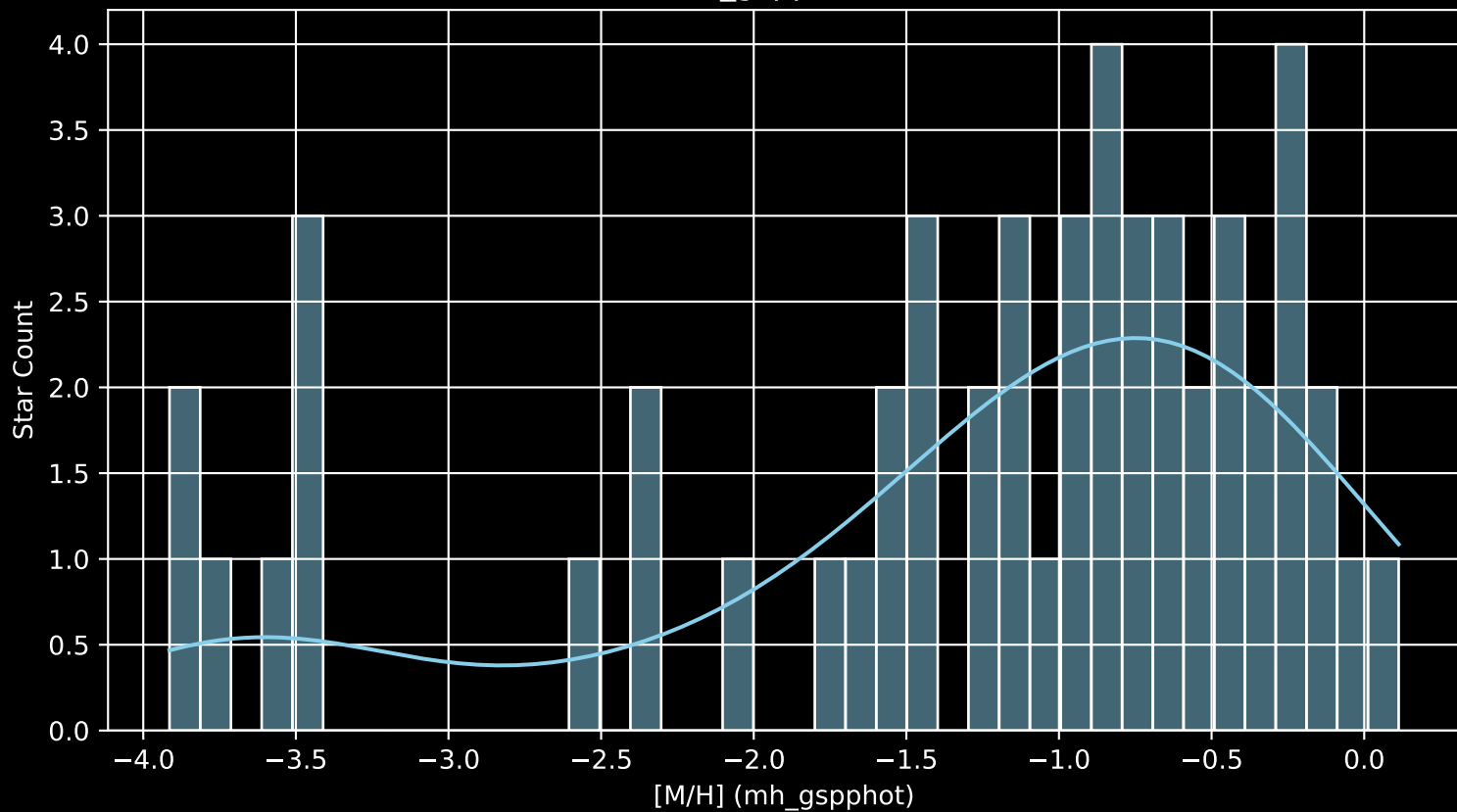
Gaia Cluster: [vdBergh_85 [M/H] (mh_gspphot) (n= 52)
