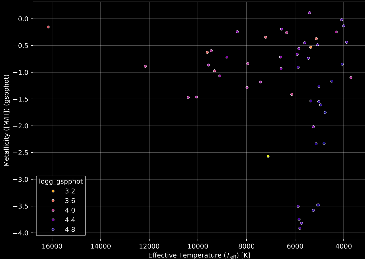
Gaia Cluster: [vdBergh_85] Stellar Population Parameters (n= 52)
