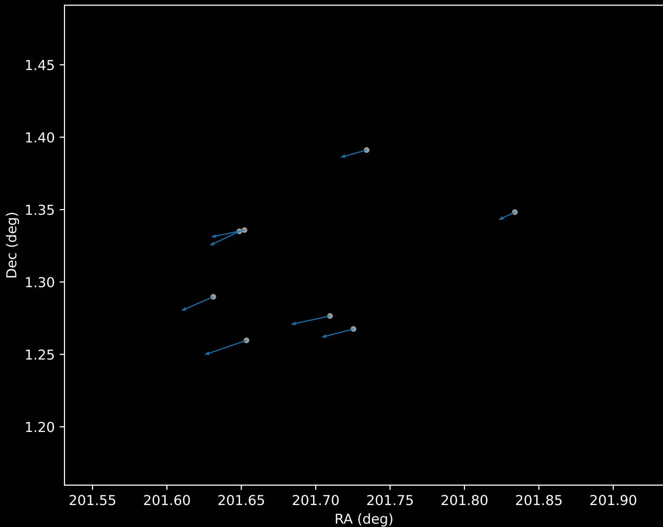
Gaia DR3 Cluster 0 Proper Motion Vectors (n=8)
