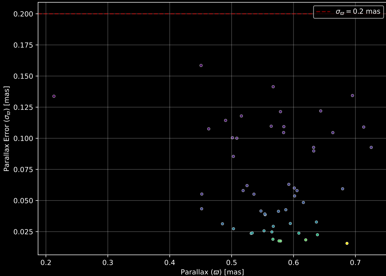
Gaia Cluster: [vdBergh_85] Parallax Quality (n= 52)
