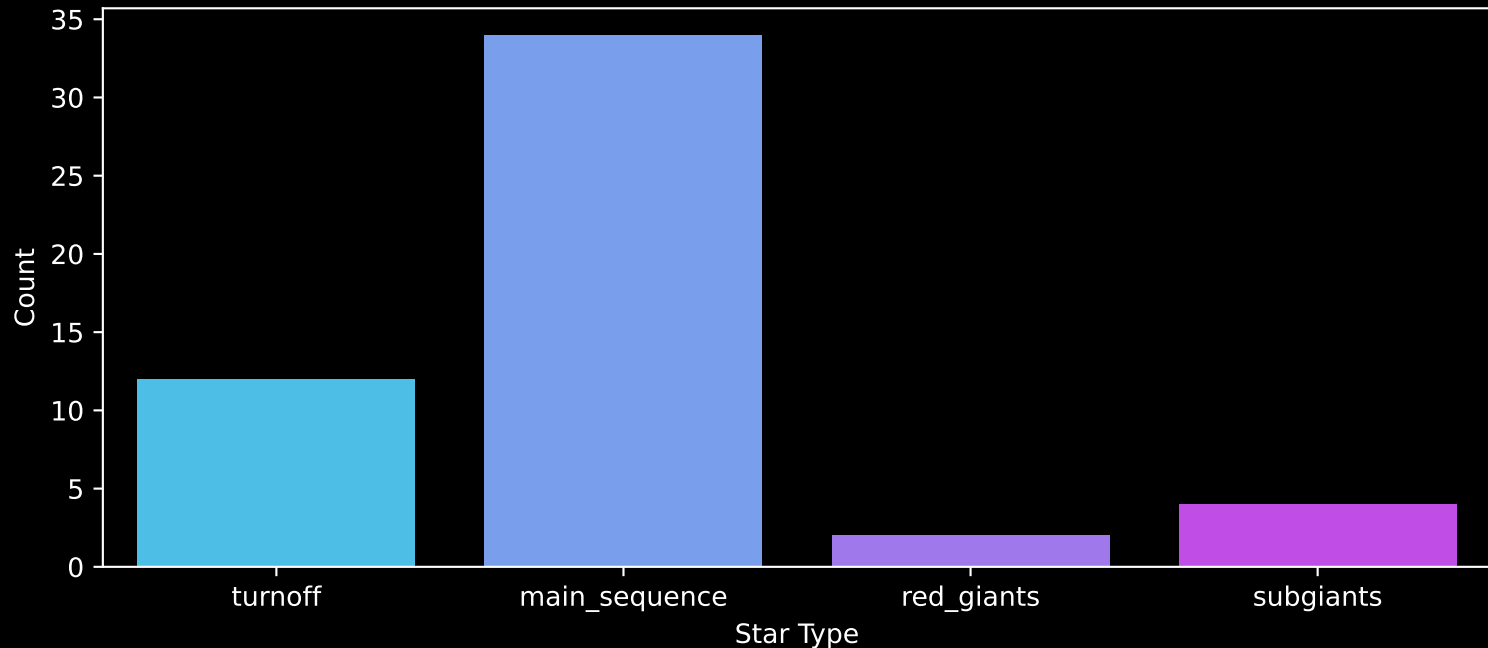
Gaia Cluster: [vdBergh_85] Count plot of Star Type
