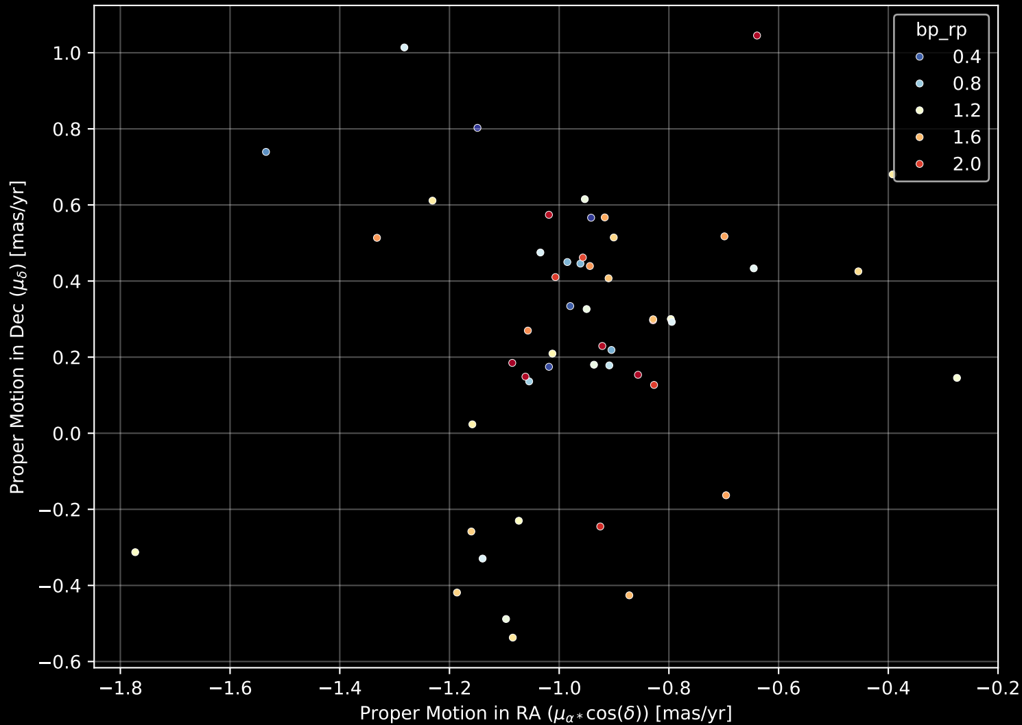
Gaia Cluster: [vdBergh_85] Proper Motion Diagram (n= 52)
