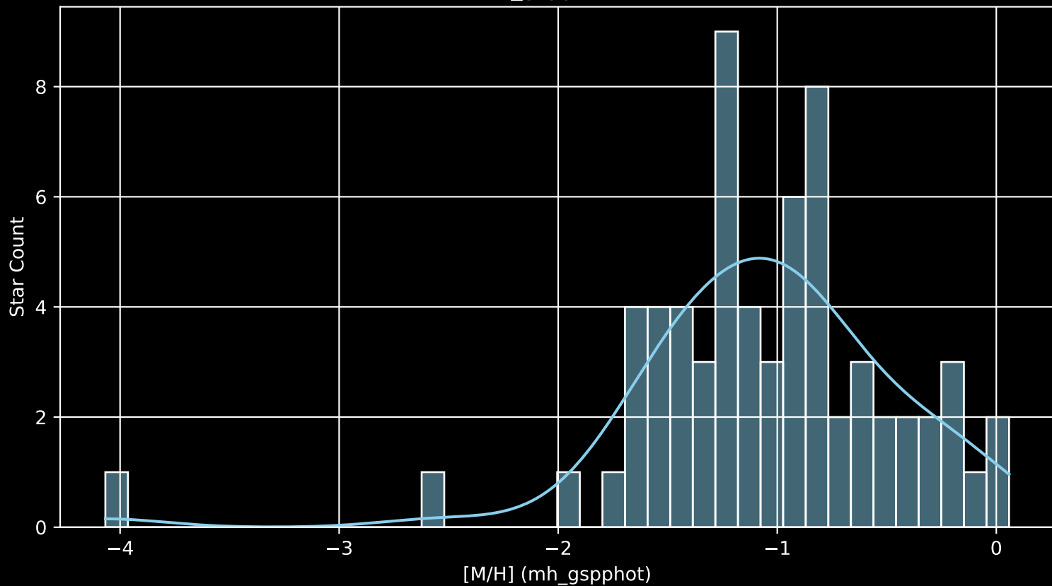
Gaia Stream: [C-10 [M/H] (mh_gspphot) (n= 66)
