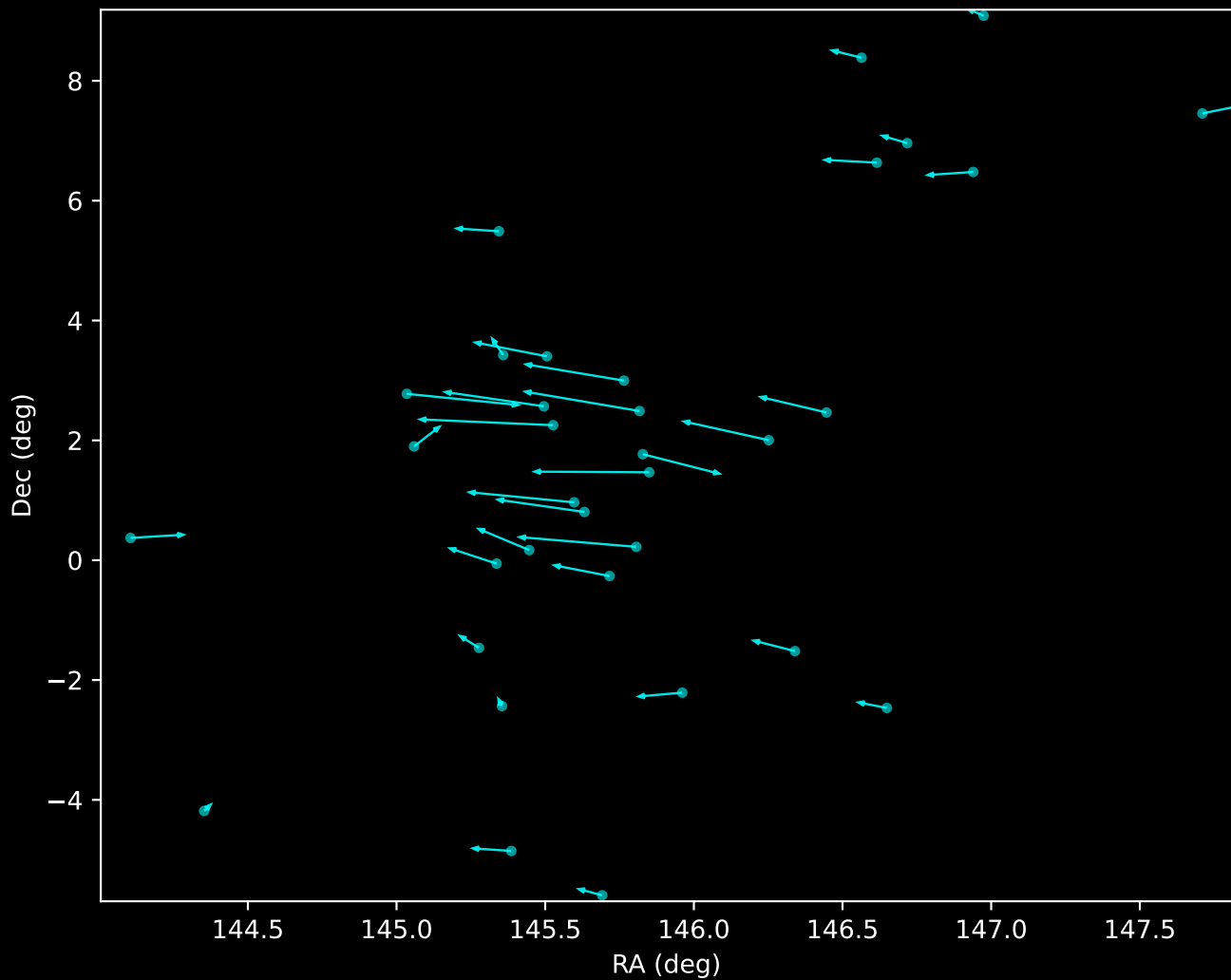
Gaia DR3 HDBSCAN 'Noise' (GD-1 Stream) (n=34)
