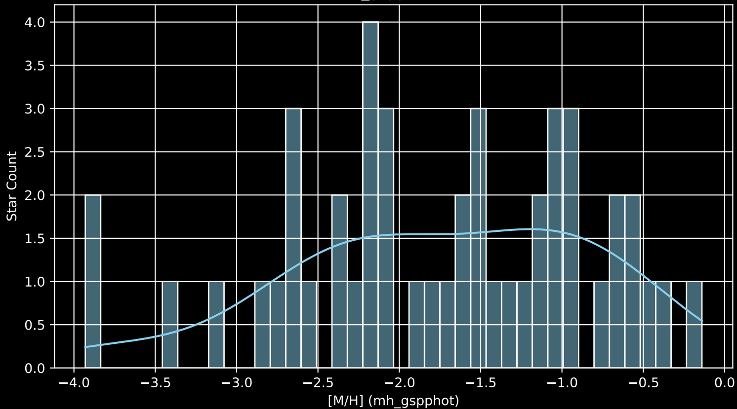
Gaia Stream: [C-11 [M/H] (mh_gspphot) (n= 47)
