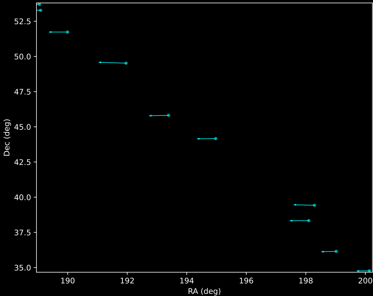
Gaia DR3 HDBSCAN 'Noise' (GD-1 Stream) (n=10)
