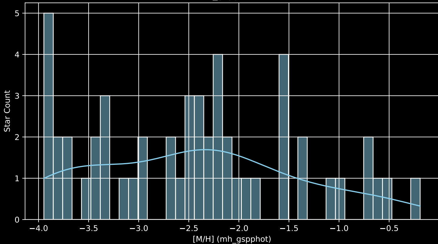
Gaia Stream: [C-25 [M/H] (mh_gspphot) (n= 52)
