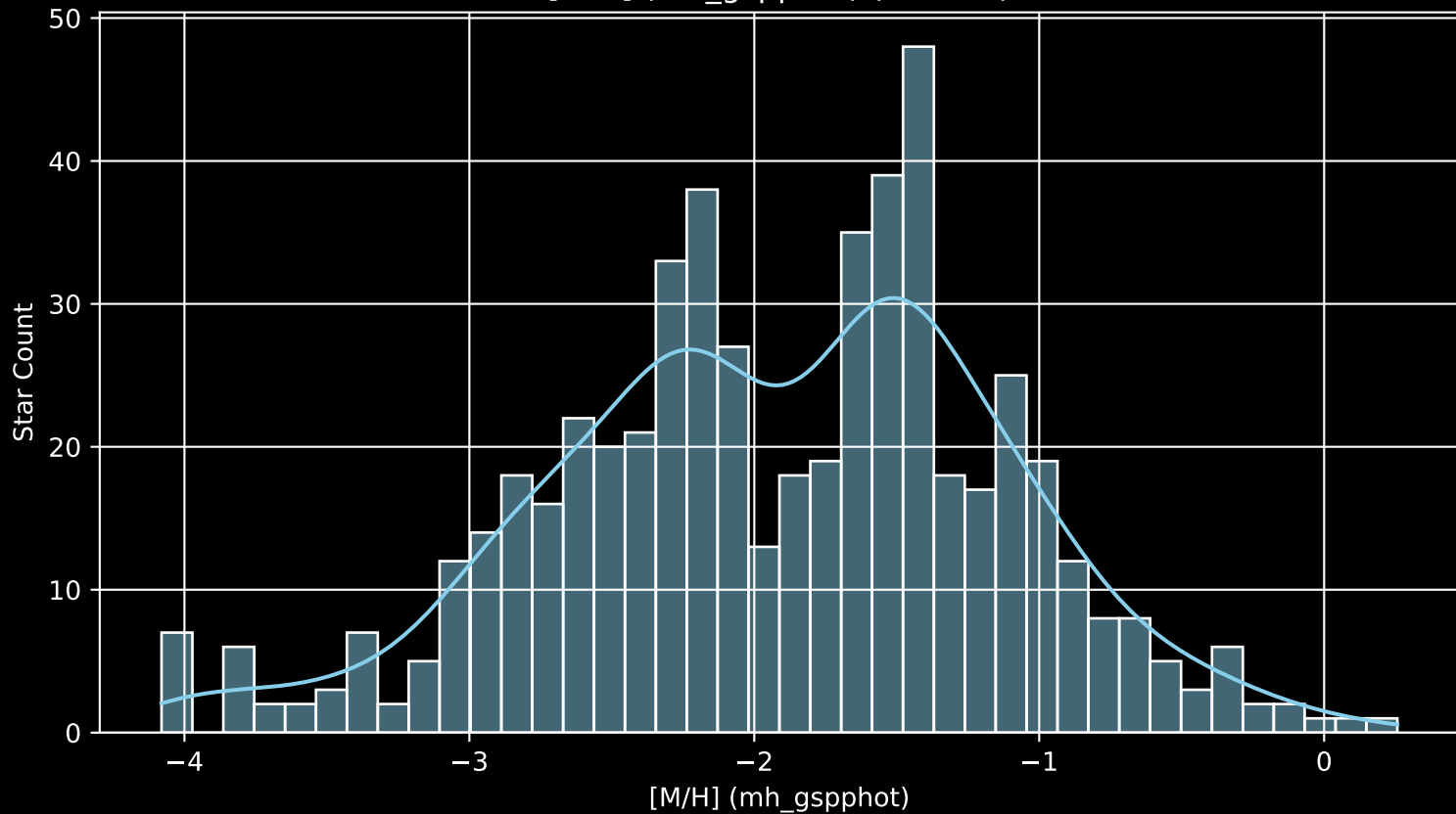
Gaia Stream: [GD-1 [M/H] (mh_gspphot) (n= 555)
