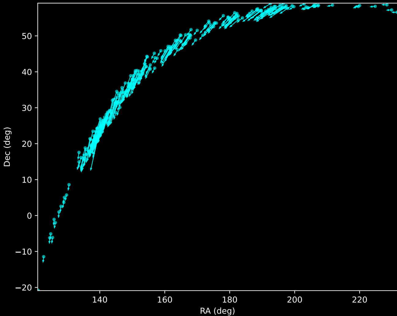
Gaia DR3 HDBSCAN 'Noise' (GD-1 Stream) (n=241)
