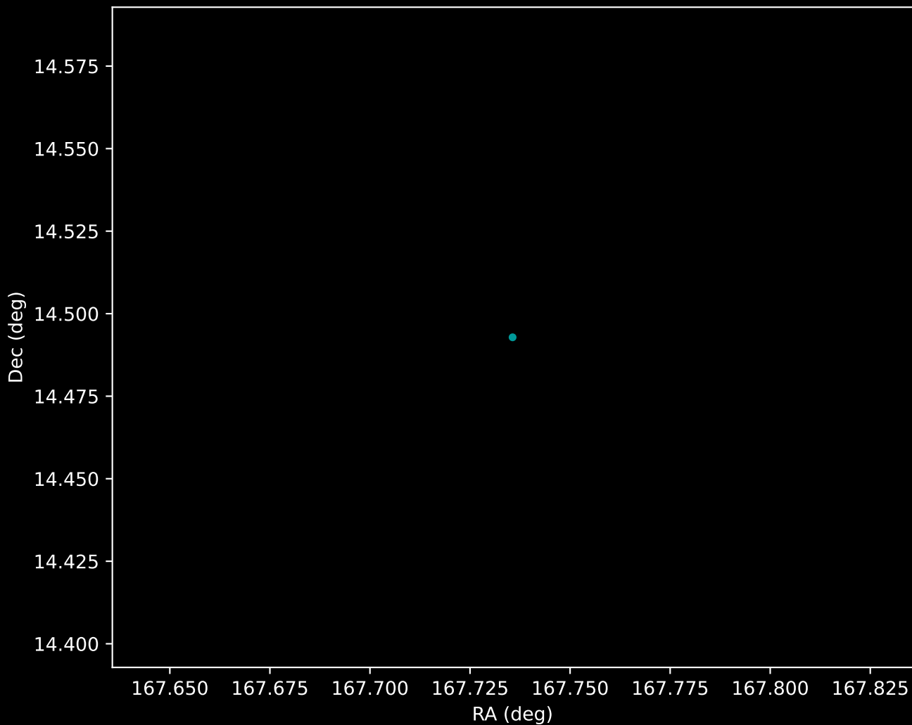
Gaia DR3 HDBSCAN 'Noise' (GD-1 Stream) (n=1)
