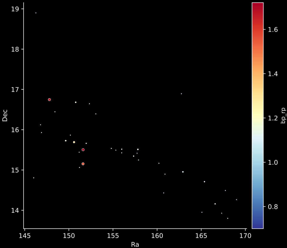
Gaia Stream: [Gaia-10] Stars: 37
