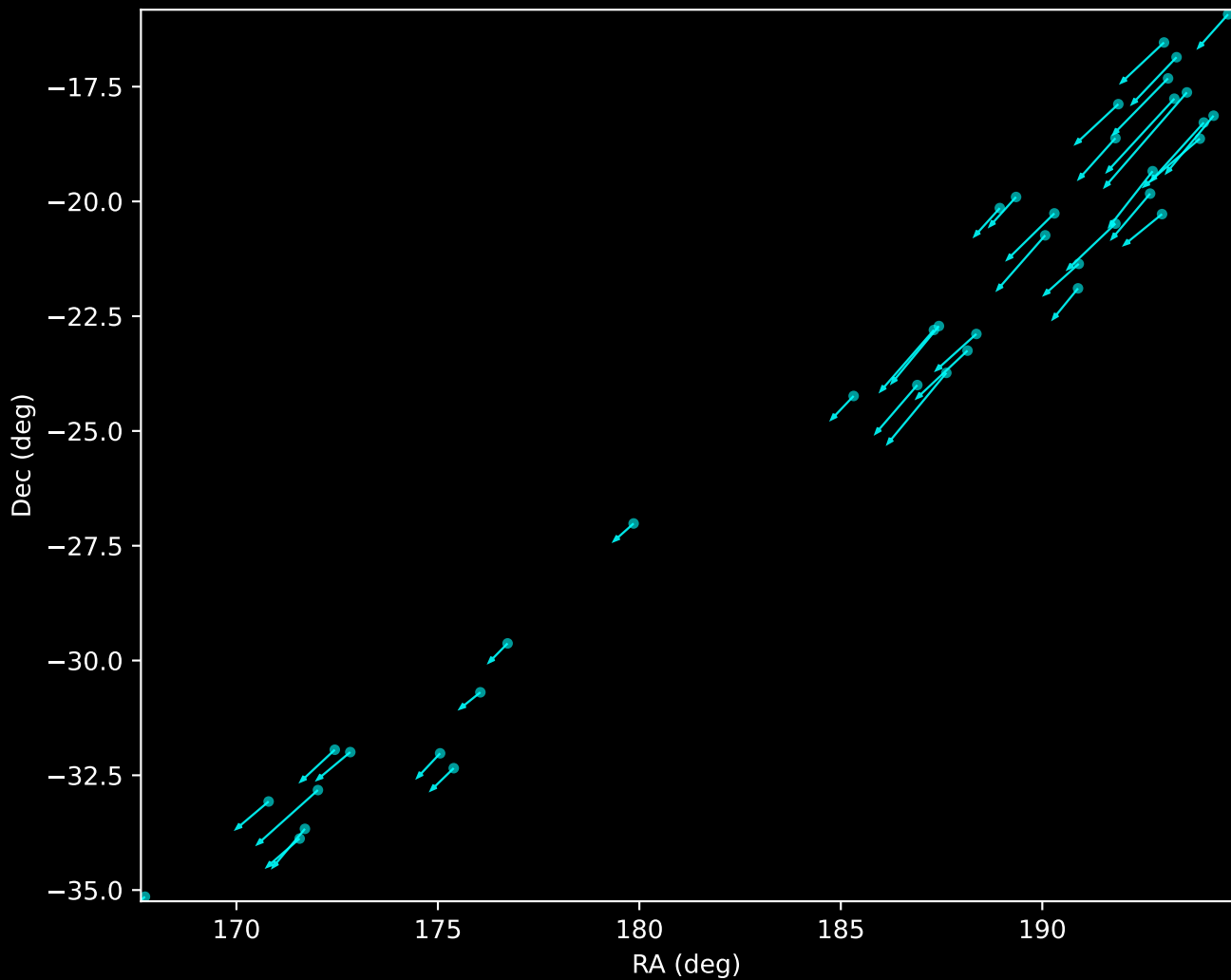
Gaia DR3 HDBSCAN 'Noise' (GD-1 Stream) (n=40)
